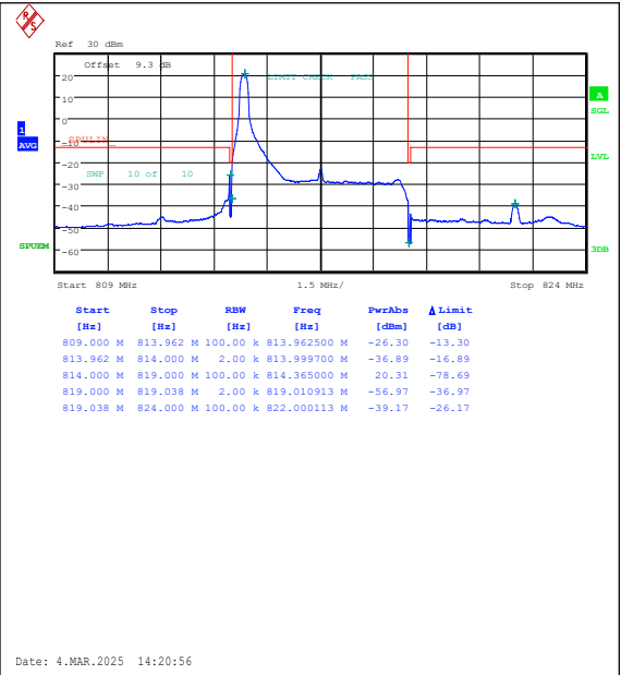
Band26(814-824)-5MHz-16QAM-26715-1RB#0-P ASS
