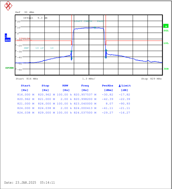
Band26(814-824)-3MHz-16QAM-26775-15RB#0-P ASS
