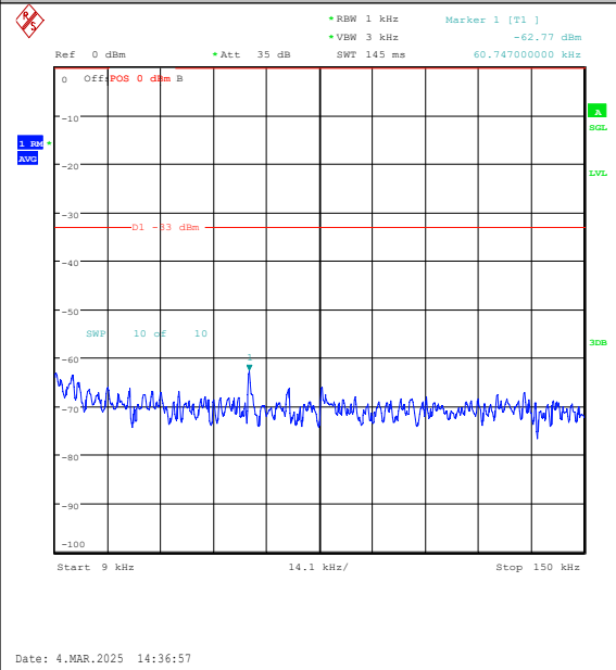
Band26(814-824)-5MHz-16QAM-26740-1RB#0-0. 009~0.15-PASS
