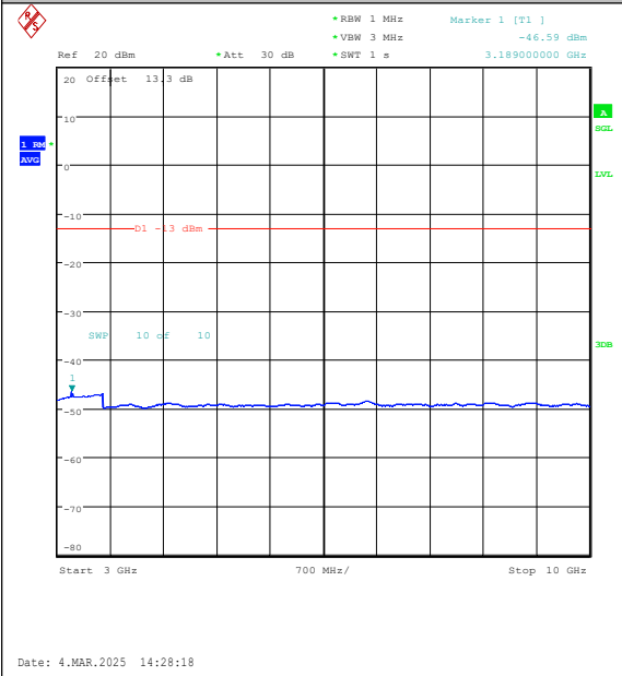
Band26(814-824)-5MHz-QPSK-26715-1RB#0-3000~10000-PASS
