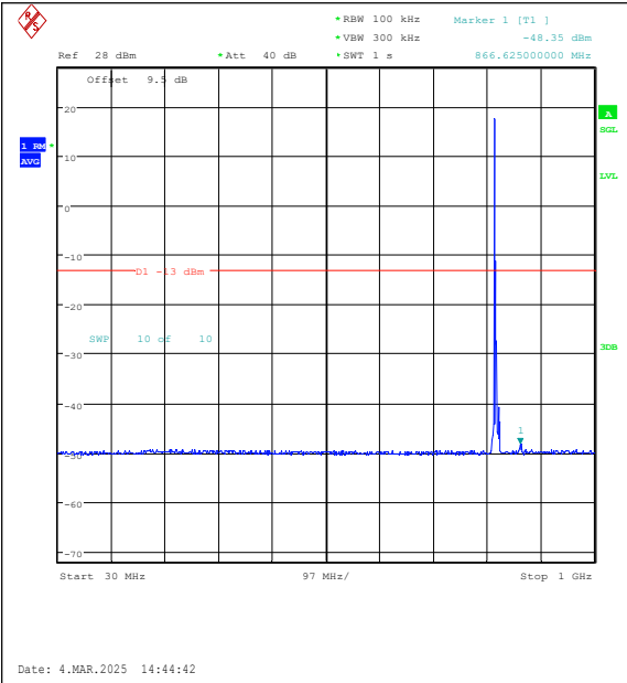
Band26(814-824)-5MHz-QPSK-26765-1RB#0-30~1000-PASS
