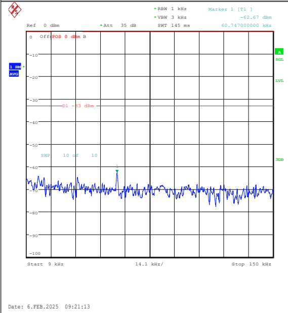
Band26(824-849)-1.4MHz-QPSK-26797-1RB#0-0.009~0.15-PASS
