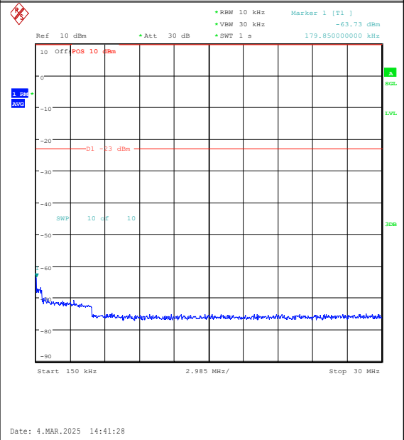
Band26(814-824)-5MHz-QPSK-26740-25RB#0-0. 15~30-PASS
