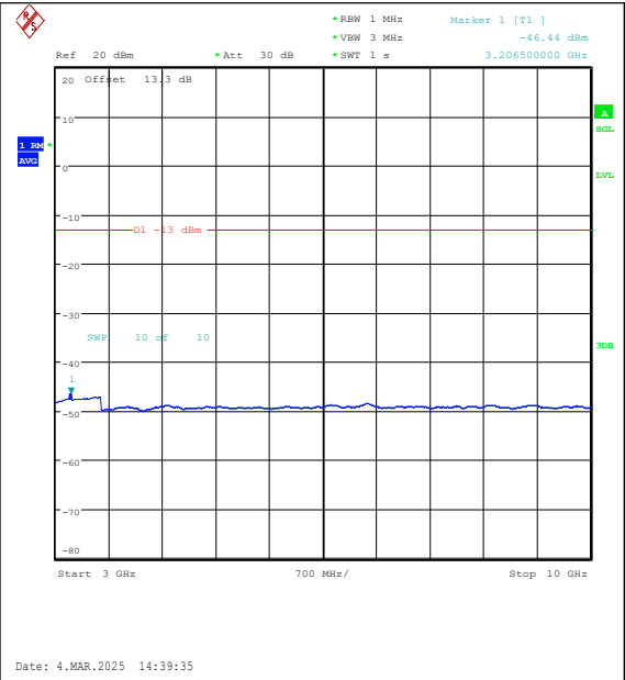
Band26(814-824)-5MHz-QPSK-26740-1RB#24-30 00~10000-PASS
