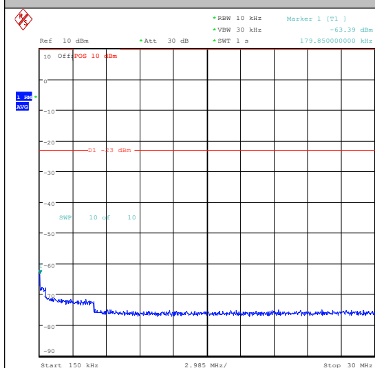
Band26(814-824)-3MHz-QPSK-26705-1RB#0-300 0~10000-PASS
