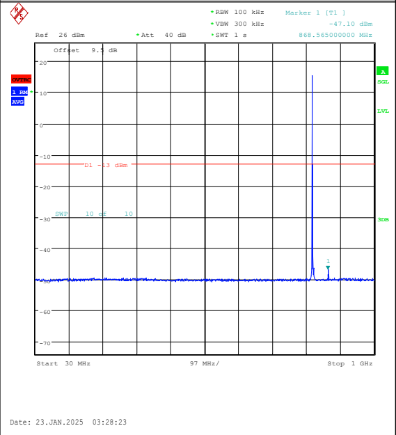
Band26(814-824)-1.4MHz-16QAM-26783-1RB#0- 30~1000-PASS
