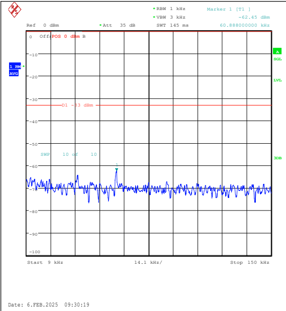
Band26(824-849)-1.4MHz-QPSK-26915-1RB#0-0.009~0.15-PASS
