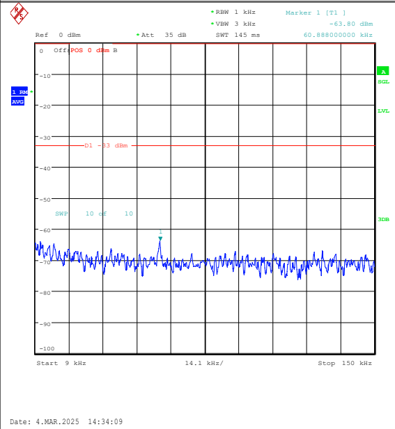
Band26(814-824)-5MHz-16QAM-26715-25RB#0-0 .009~0.15-PASS
