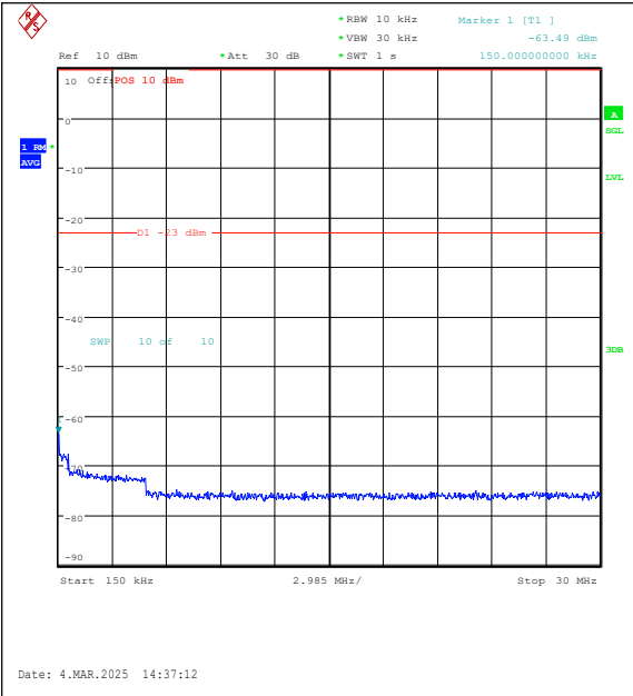
Band26(814-824)-5MHz-16QAM-26740-1RB#0-0. 15~30-PASS
