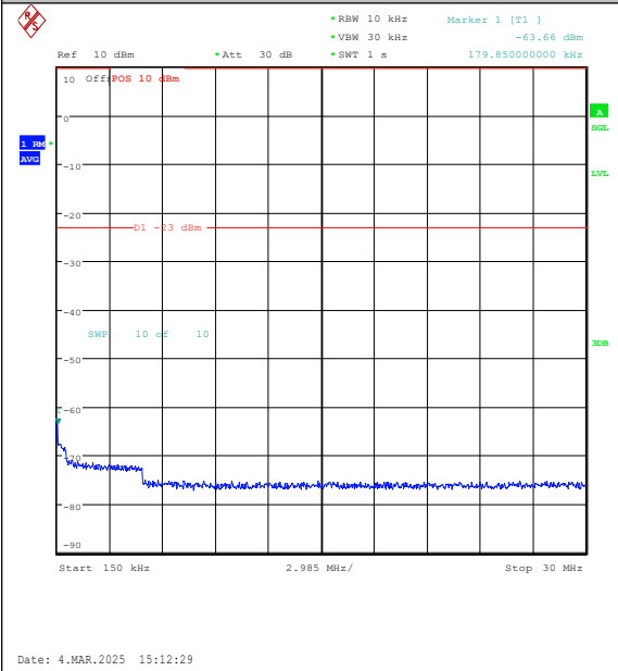
Band26(814-824)-10MHz-QPSK-26740-1RB#49-0 .15~30-PASS
