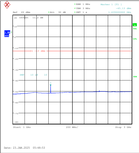
Band26(814-824)-3MHz-16QAM-26740-1RB#0-10 00~3000-PASS
