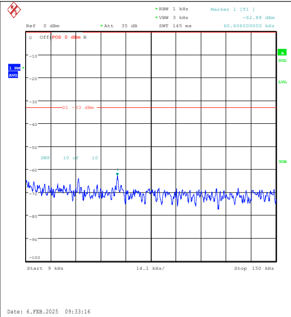
Band26(824-849)-1.4MHz-QPSK-26915-1RB#5-0. 009~0.15-PASS
