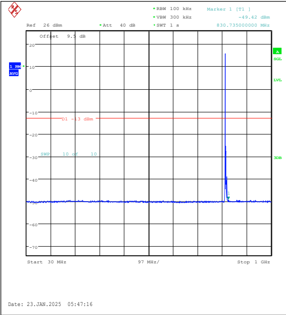
Band26(814-824)-3MHz-QPSK-26740-1RB#0-30~1000-PASS
