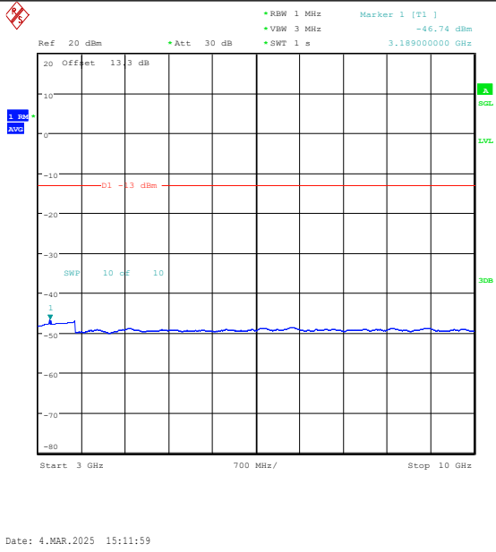
Band26(814-824)-10MHz-16QAM-26740-1RB#0-3 000~10000-PASS
