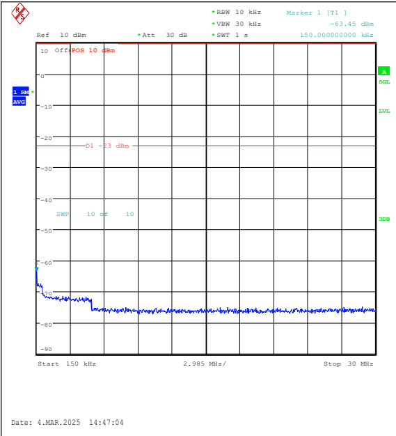
Band26(814-824)-5MHz-QPSK-26765-1RB#24-0. 15~30-PASS
