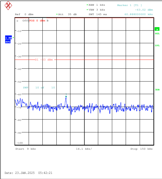
Band26(814-824)-3MHz-16QAM-26705-1RB#14-0 .009~0.15-PASS
