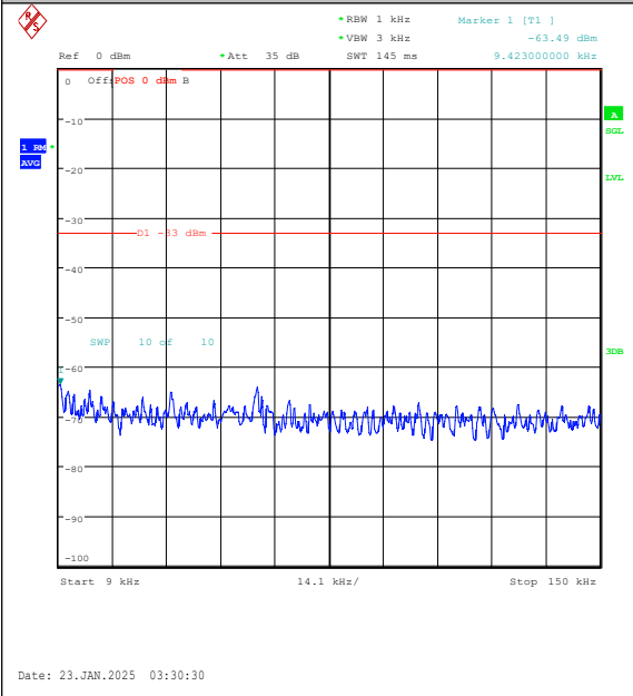
Band26(814-824)-1.4MHz-16QAM-26783-1RB#5-0.009~0.15-PASS
