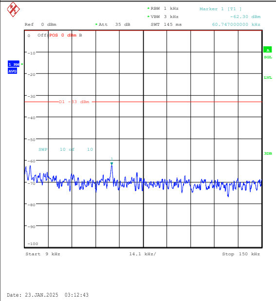
Band26(814-824)-1.4MHz-QPSK-26697-1RB#5-0. 009~0.15-PASS
