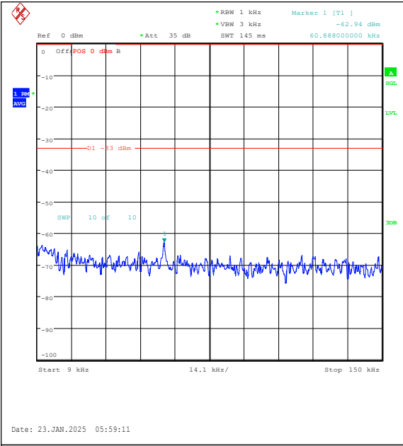
Band26(814-824)-3MHz-16QAM-26775-1RB#14-0 .009~0.15-PASS
