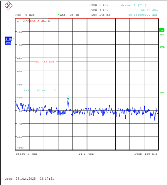
Band26(814-824)-1.4MHz-QPSK-26740-1RB#0-0.009~0.15-PASS
