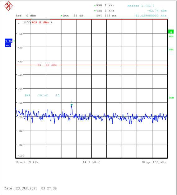
Band26(814-824)-1.4MHz-16QAM-26783-1RB#0- 0.009~0.15-PASS
