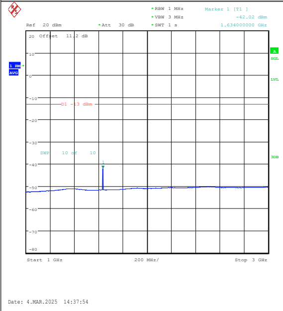
Band26(814-824)-5MHz-16QAM-26740-1RB#0-10 00~3000-PASS
