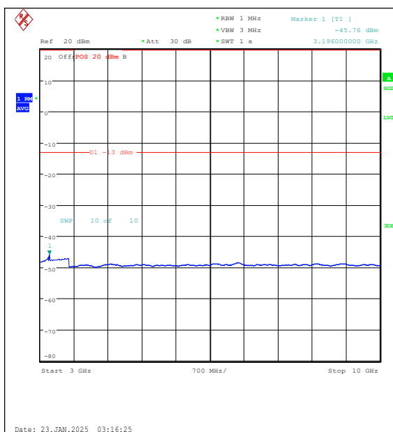
Band26(814-824)-1.4MHz-QPSK-26697-6RB#0-3 000~10000-PASS
