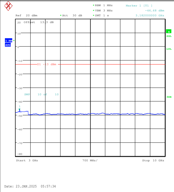
Band26(814-824)-3MHz-16QAM-26775-1RB#0-30 00~10000-PASS
