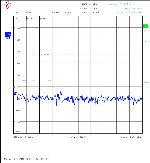
Band26(814-824)-3MHz-QPSK-26775-15RB#0-0. 009~0.15-PASS
