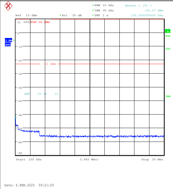
Band26(824-849)-1.4MHz-QPSK-26797-1RB#0-0.15~30-PASS
