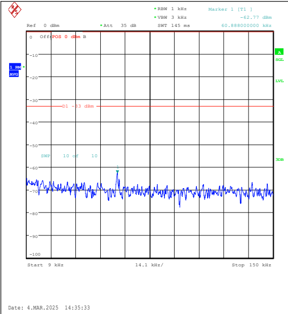
Band26(814-824)-5MHz-QPSK-26740-1RB#0-0.0 09~0.15-PASS
