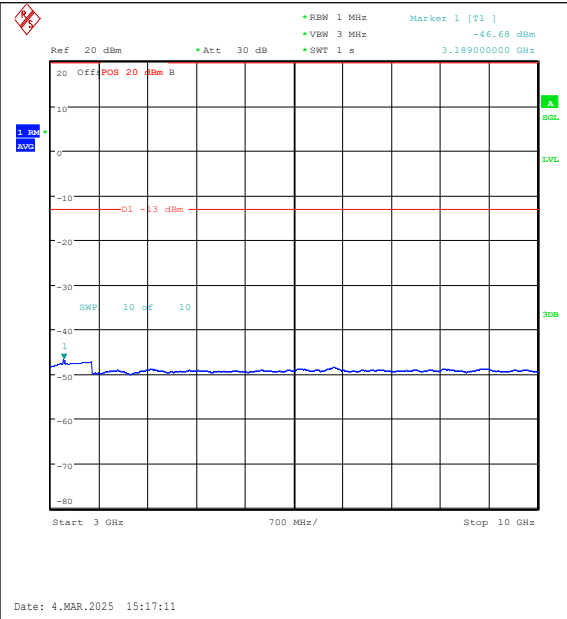
Band26(814-824)-10MHz-16QAM-26740-50RB#0-3000~10000-PASS
