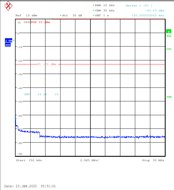
Band26(814-824)-3MHz-16QAM-26740-1RB#14-0 .15~30-PASS
