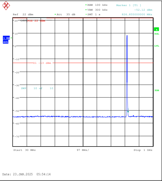
Band26(814-824)-3MHz-16QAM-26740-15RB#0-3 0~1000-PASS
