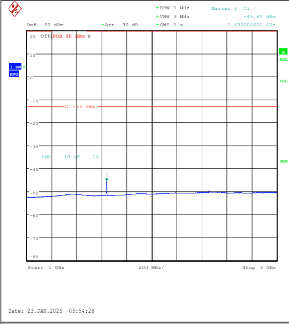
Band26(814-824)-3MHz-16QAM-26740-15RB#0-1 000~3000-PASS
