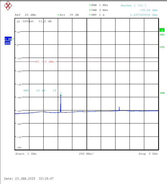
Band26(814-824)-1.4MHz-QPSK-26740-1RB#0-1000~3000-PASS
