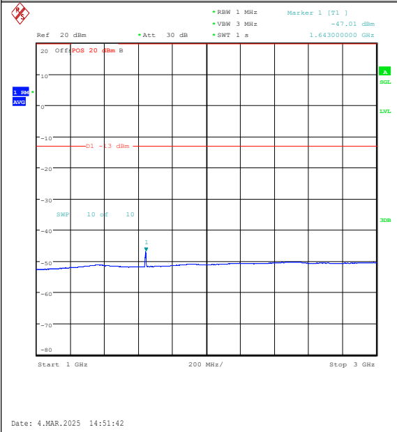
Band26(814-824)-5MHz-16QAM-26765-25RB#0-1 000~3000-PASS
