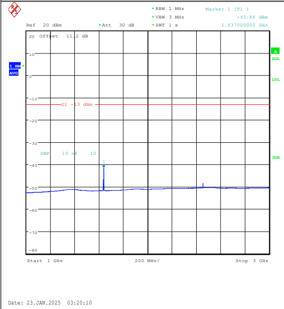
Band26(814-824)-1.4MHz-16QAM-26740-1RB#0-1000~3000-PASS
