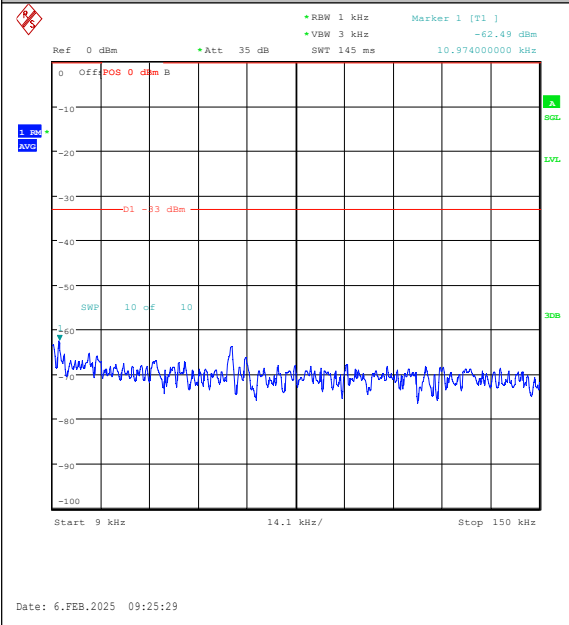
Band26(824-849)-1.4MHz-16QAM-26797-1RB#5-0.009~0.15-PASS
