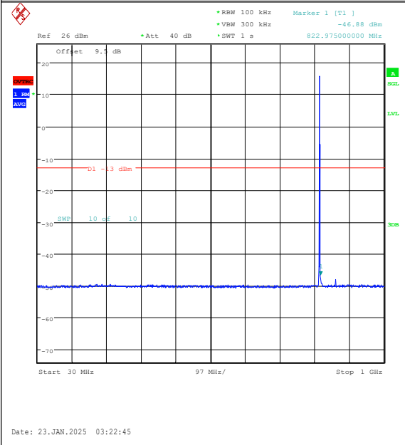
Band26(814-824)-1.4MHz-16QAM-26740-1RB#5-30~1000-PASS
