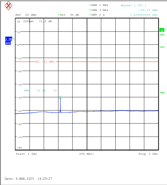
Band26(814-824)-5MHz-16QAM-26715-1RB#0-10 00~3000-PASS
