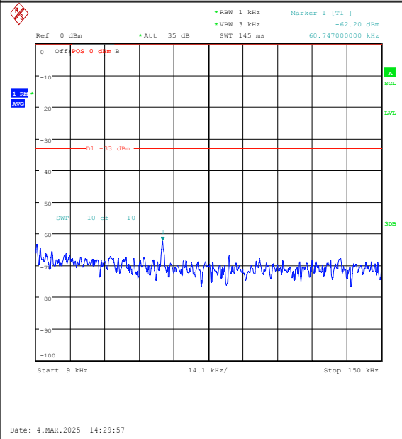
Band26(814-824)-5MHz-QPSK-26715-1RB#24-0.009~0.15-PASS
