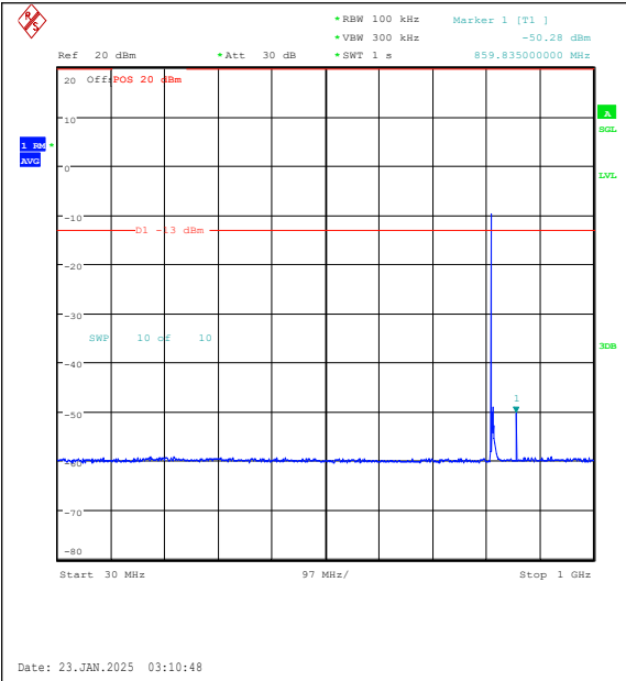
Band26(814-824)-1.4MHz-QPSK-26697-1RB#0-3 0~1000-PASS
