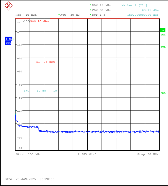
Band26(814-824)-1.4MHz-QPSK-26740-1RB#5-0. 15~30-PASS
