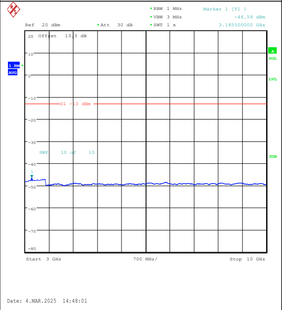
Band26(814-824)-5MHz-QPSK-26765-1RB#24-30 00~10000-PASS
