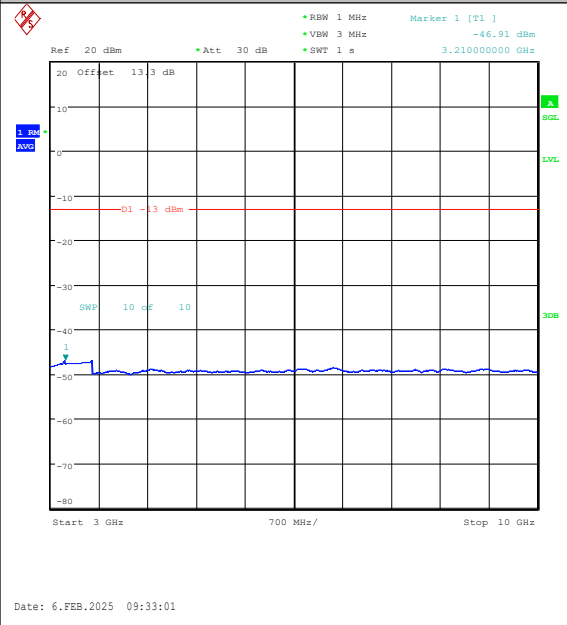
Band26(824-849)-1.4MHz-16QAM-26915-1RB#0-3000~10000-PASS
