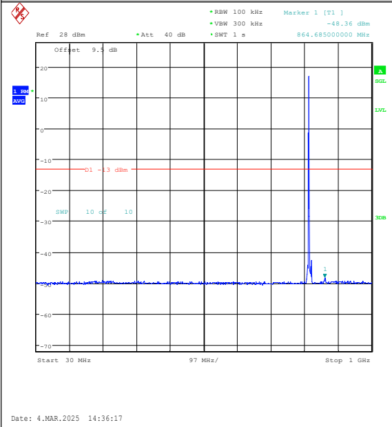
Band26(814-824)-5MHz-QPSK-26740-1RB#0-30~ 1000-PASS
