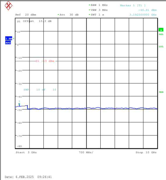
Band26(824-849)-1.4MHz-16QAM-26797-1RB#5-3000~10000-PASS
