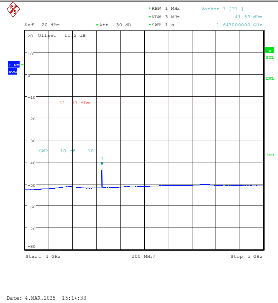
Band26(814-824)-10MHz-16QAM-26740-1RB#49-1000~3000-PASS
