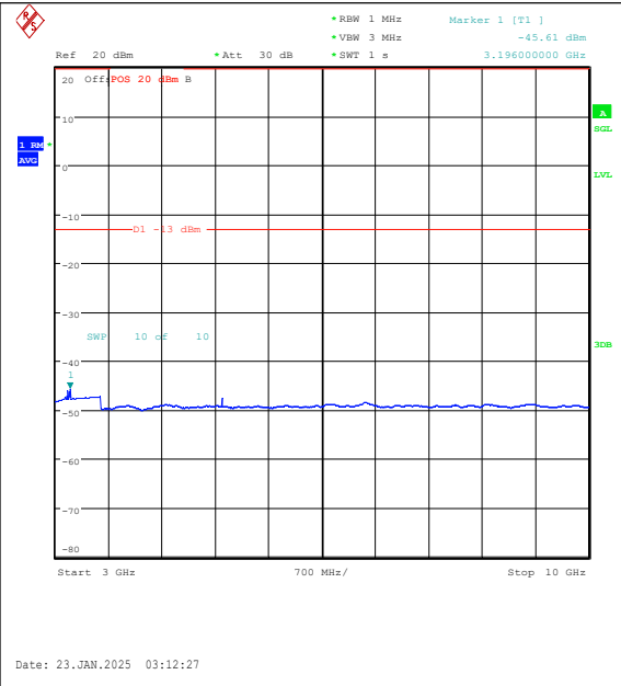
Band26(814-824)-1.4MHz-16QAM-26697-1RB#0-3000~10000-PASS
