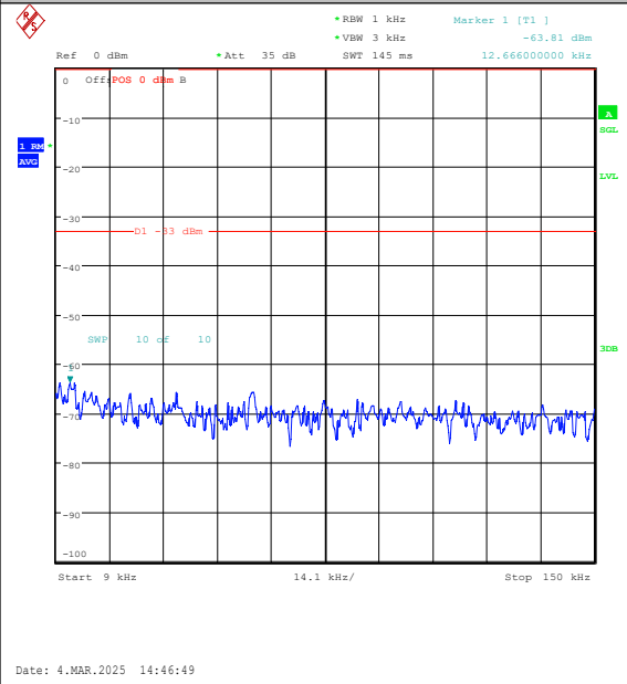
Band26(814-824)-5MHz-QPSK-26765-1RB#24-0.009~0.15-PASS
