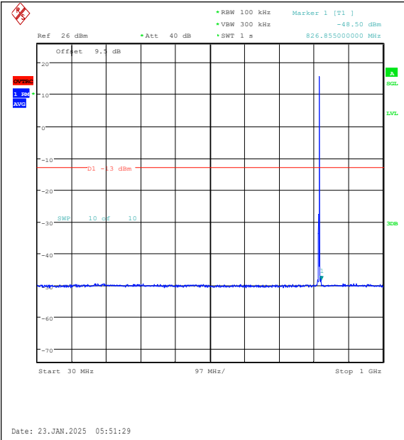
Band26(814-824)-3MHz-16QAM-26740-1RB#14-3 0~1000-PASS
