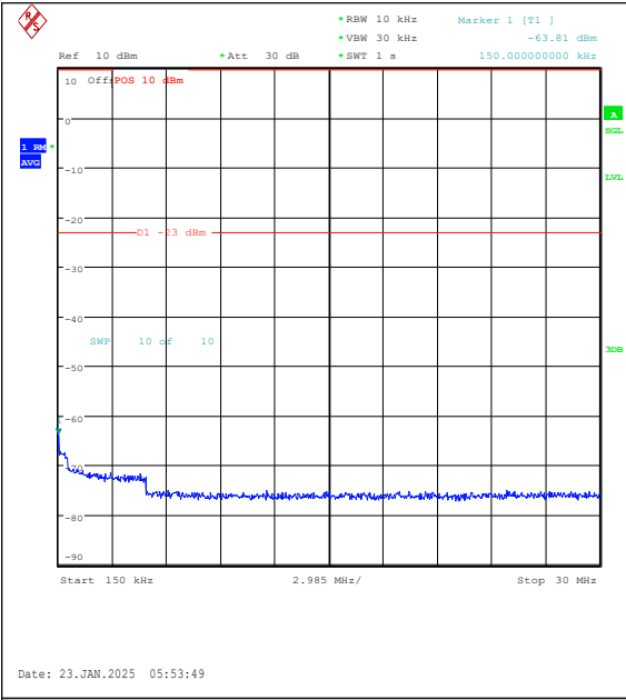
Band26(814-824)-3MHz-16QAM-26740-15RB#0-0 .15~30-PASS
