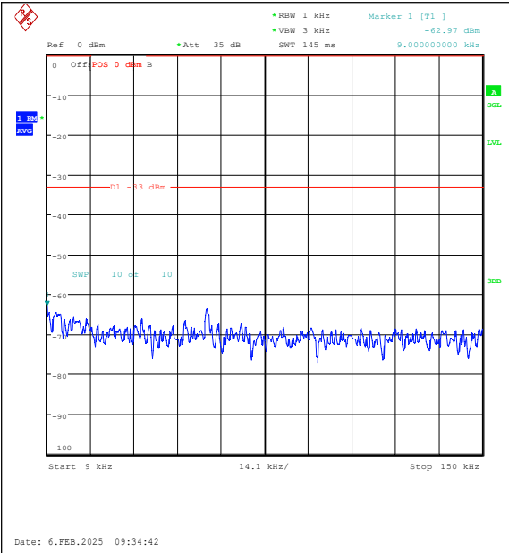
Band26(824-849)-1.4MHz-16QAM-26915-1RB#5-0.009~0.15-PASS
