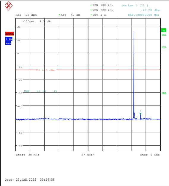
Band26(814-824)-1.4MHz-QPSK-26783-1RB#0-3 0~1000-PASS
