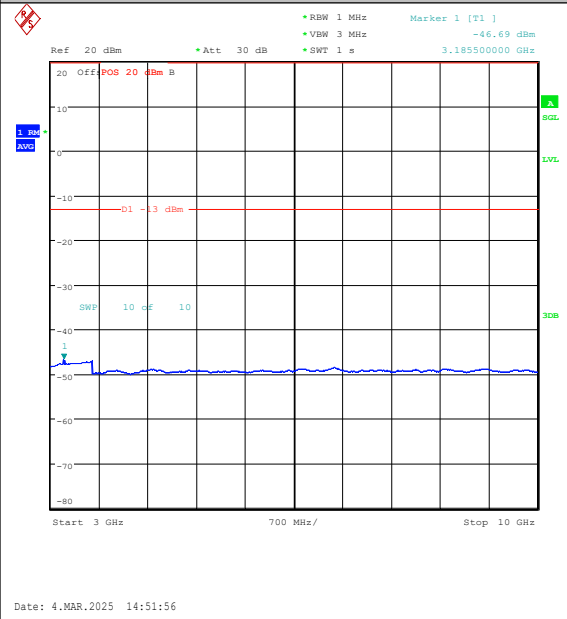
Band26(814-824)-5MHz-16QAM-26765-25RB#0-3 000~10000-PASS
