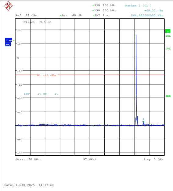
Band26(814-824)-5MHz-16QAM-26740-1RB#0-30 ~1000-PASS
