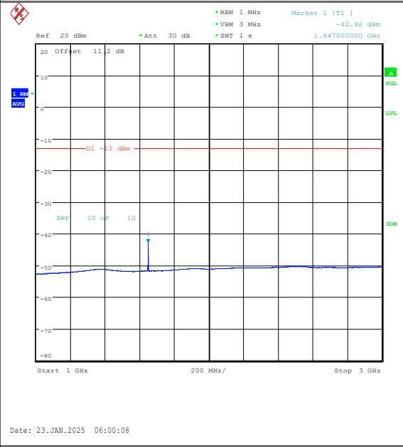
Band26(814-824)-3MHz-16QAM-26775-1RB#14-1 000~3000-PASS
