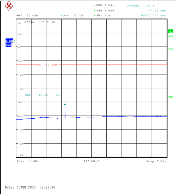
Band26(824-849)-1.4MHz-16QAM-26797-1RB#0-1000~3000-PASS
