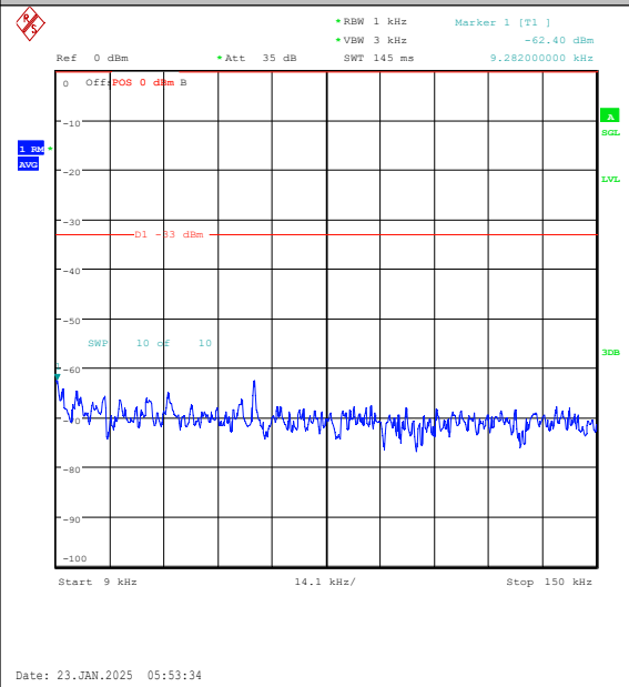
Band26(814-824)-3MHz-16QAM-26740-15RB#0-0 .009~0.15-PASS
