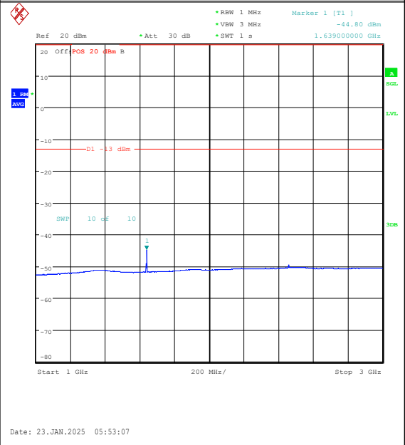
Band26(814-824)-3MHz-QPSK-26740-15RB#0-10 00~3000-PASS
