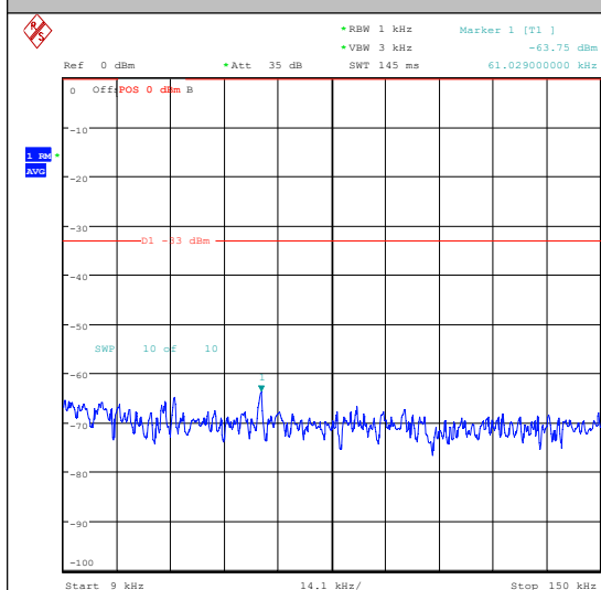
Band26(814-824)-3MHz-16QAM-26705-15RB#0-1 000~3000-PASS
