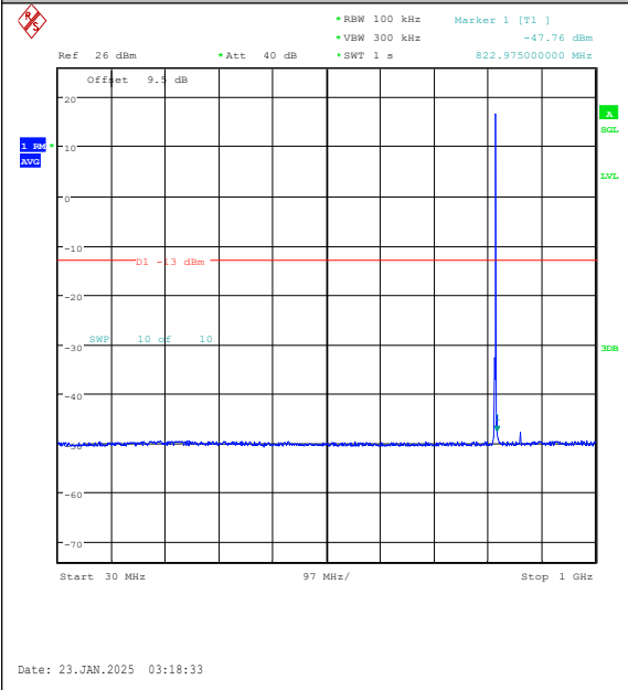
Band26(814-824)-1.4MHz-QPSK-26740-1RB#0-30~1000-PASS
