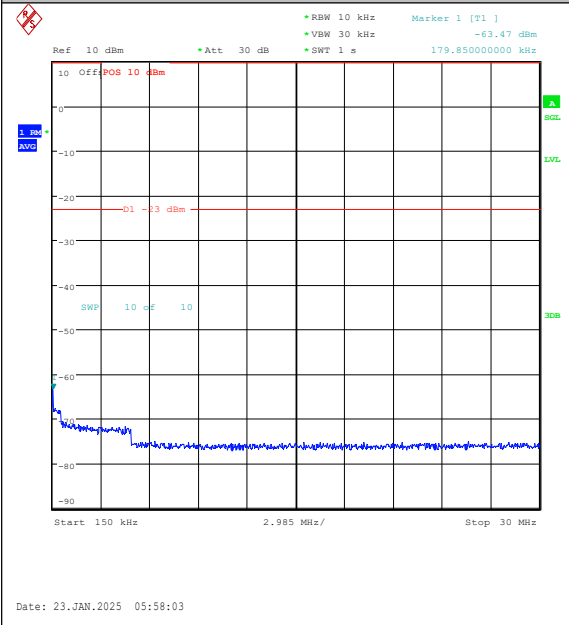
Band26(814-824)-3MHz-QPSK-26775-1RB#14-0. 15~30-PASS
