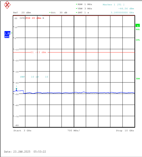
Band26(814-824)-3MHz-QPSK-26740-15RB#0-30 00~10000-PASS
