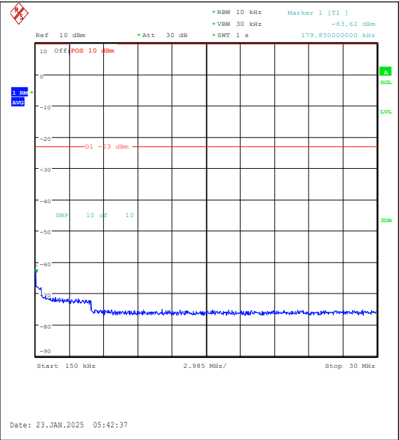
Band26(814-824)-3MHz-16QAM-26705-1RB#14-0 .15~30-PASS
