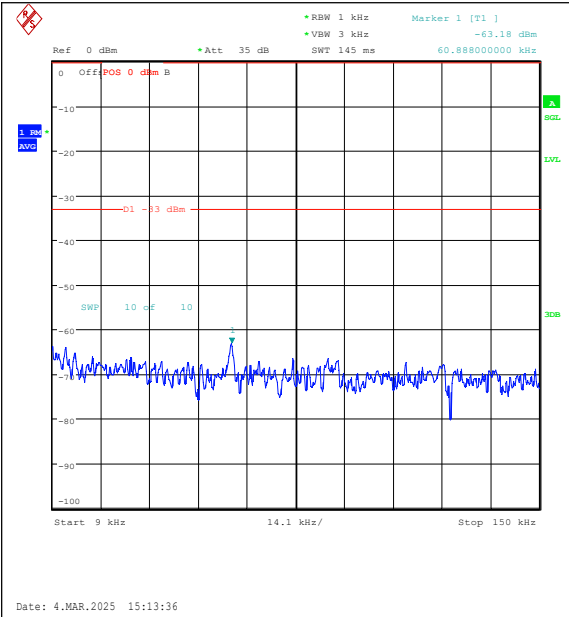
Band26(814-824)-10MHz-16QAM-26740-1RB#49-0.009~0.15-PASS
