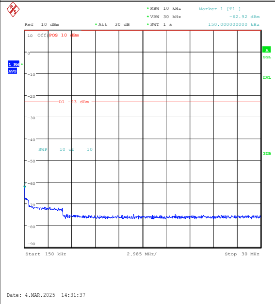
Band26(814-824)-5MHz-16QAM-26715-1RB#24-0 .15~30-PASS
