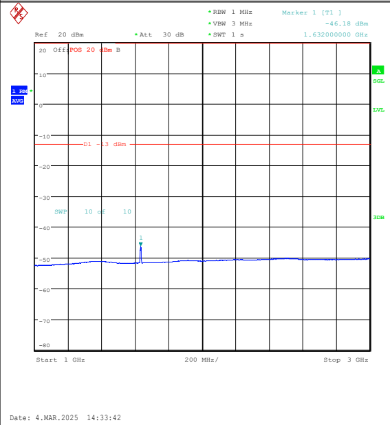
Band26(814-824)-5MHz-QPSK-26715-25RB#0-1000~3000-PASS
