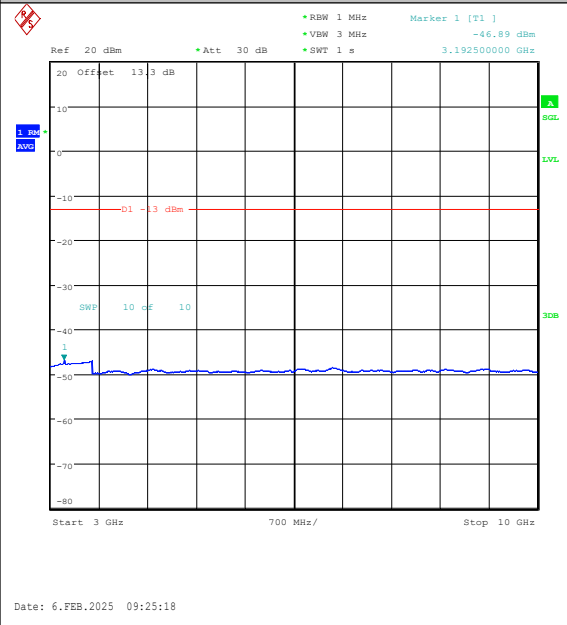
Band26(824-849)-1.4MHz-QPSK-26797-1RB#5-3 000~10000-PASS
