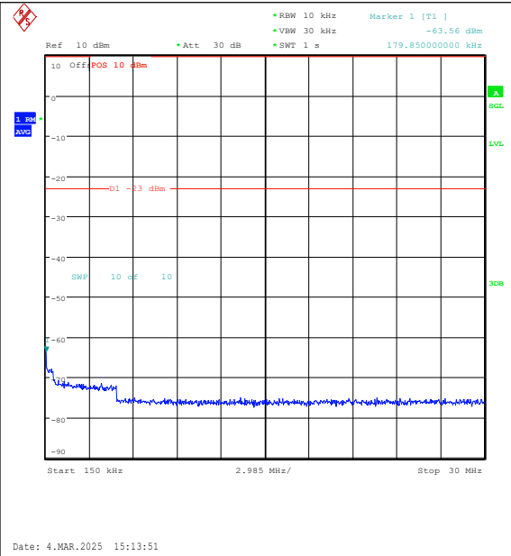
Band26(814-824)-10MHz-16QAM-26740-1RB#49-0.15~30-PASS
