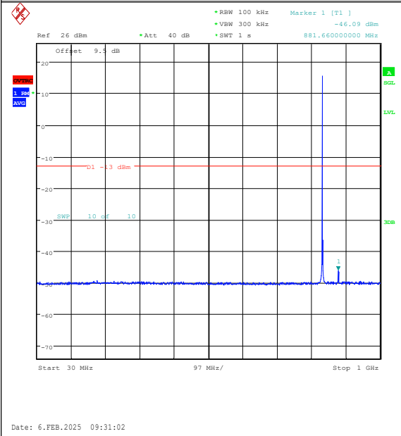
Band26(824-849)-1.4MHz-QPSK-26915-1RB#0-30~1000-PASS
