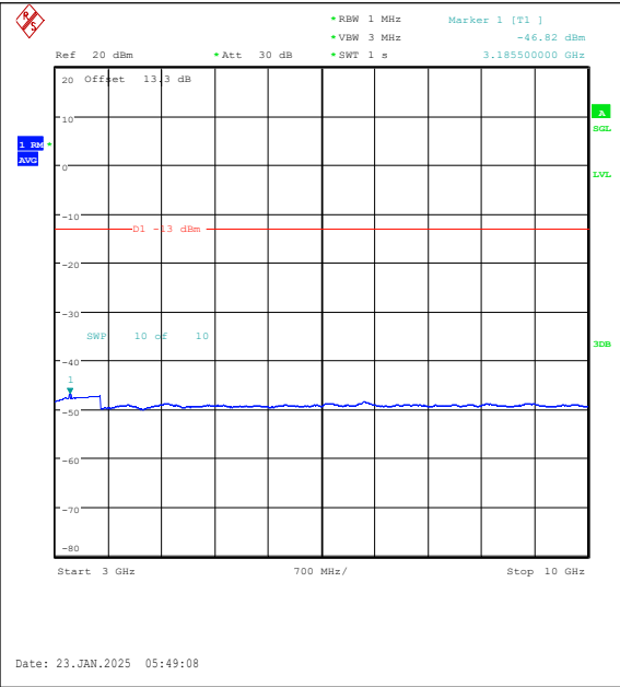
Band26(814-824)-3MHz-16QAM-26740-1RB#0-30 00~10000-PASS
