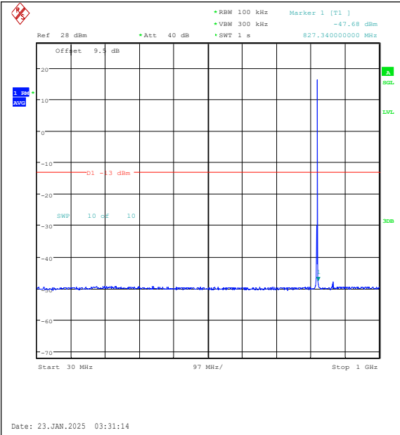
Band26(814-824)-1.4MHz-16QAM-26783-1RB#5-30~1000-PASS
