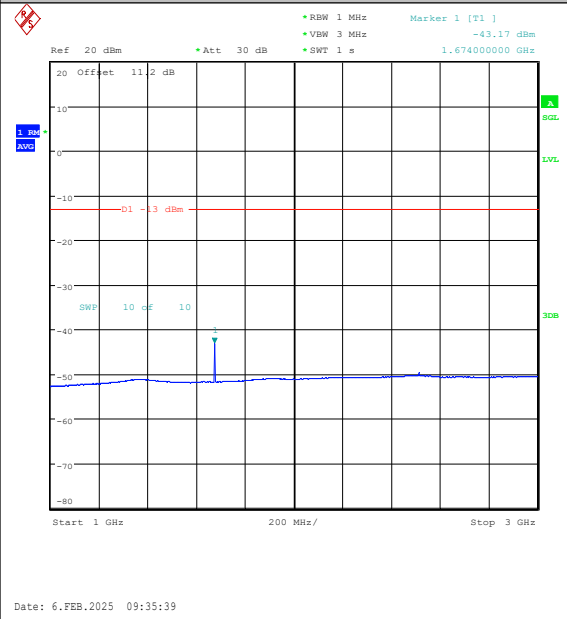
Band26(824-849)-1.4MHz-16QAM-26915-1RB#5-1000~3000-PASS
