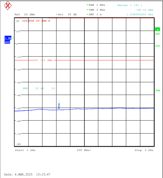
Band26(814-824)-10MHz-QPSK-26740-50RB#0-1 000~3000-PASS
