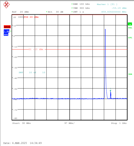
Band26(814-824)-5MHz-16QAM-26715-25RB#0-3 0~1000-PASS
