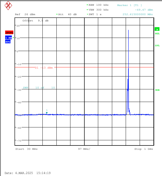
Band26(814-824)-10MHz-16QAM-26740-1RB#49-30~1000-PASS
