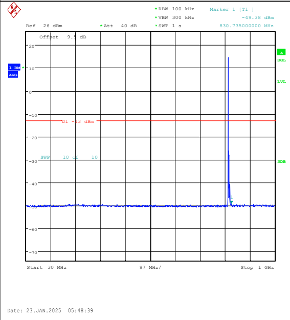
Band26(814-824)-3MHz-16QAM-26740-1RB#0-30 ~1000-PASS
