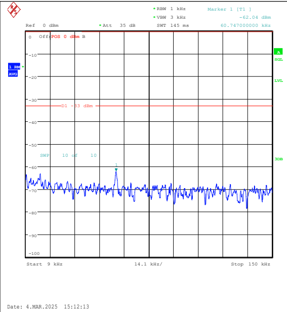
Band26(814-824)-10MHz-QPSK-26740-1RB#49-0 .009~0.15-PASS
