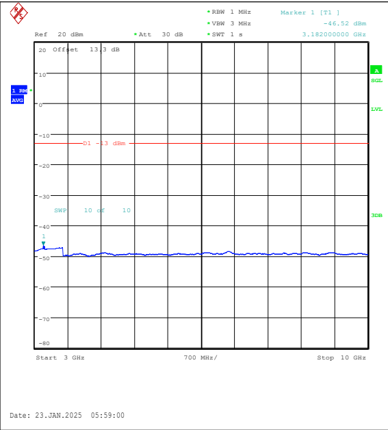
Band26(814-824)-3MHz-QPSK-26775-1RB#14-30 00~10000-PASS
