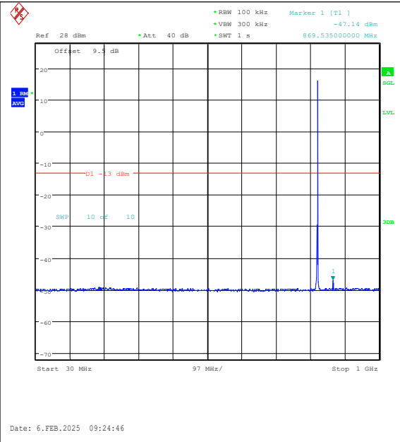
Band26(824-849)-1.4MHz-QPSK-26797-1RB#5-3 0~1000-PASS
