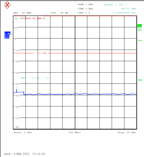
Band26(814-824)-10MHz-QPSK-26740-50RB#0-3 000~10000-PASS
