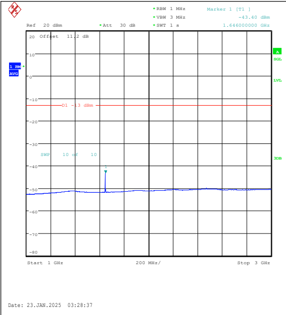
Band26(814-824)-1.4MHz-16QAM-26783-1RB#0-1000~3000-PASS
