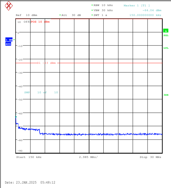
Band26(814-824)-3MHz-16QAM-26740-1RB#0-0. 15~30-PASS
