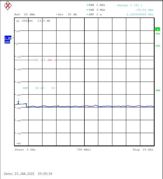
Band26(814-824)-3MHz-QPSK-26740-1RB#14-30 00~10000-PASS
