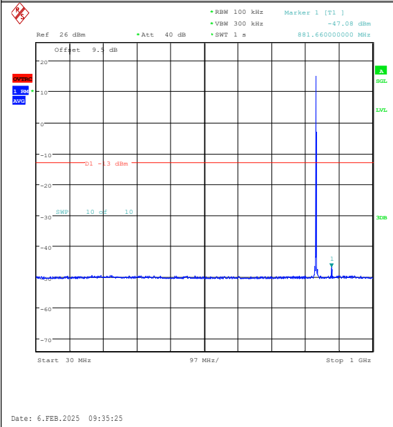
Band26(824-849)-1.4MHz-16QAM-26915-1RB#5-30~1000-PASS
