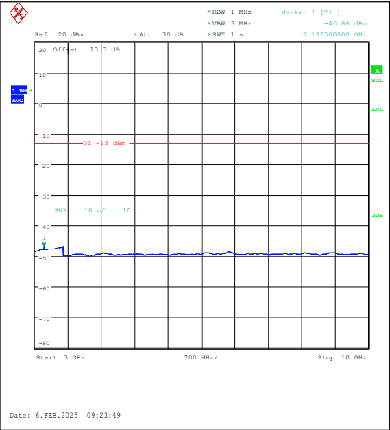
Band26(824-849)-1.4MHz-16QAM-26797-1RB#0-3000~10000-PASS
