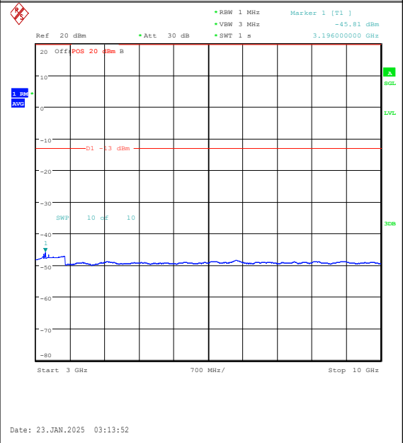
Band26(814-824)-1.4MHz-QPSK-26697-1RB#5-3 000~10000-PASS
