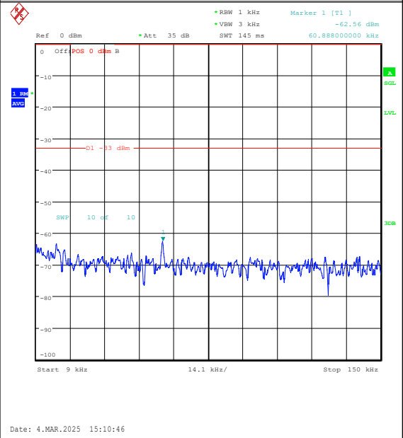
Band26(814-824)-10MHz-16QAM-26740-1RB#0-0 .009~0.15-PASS
