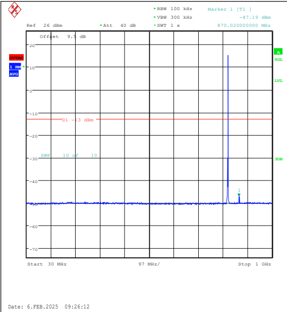
Band26(824-849)-1.4MHz-16QAM-26797-1RB#5-30~1000-PASS
