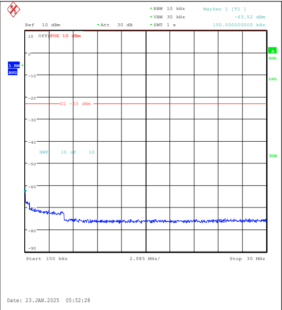
Band26(814-824)-3MHz-QPSK-26740-15RB#0-0. 15~30-PASS
