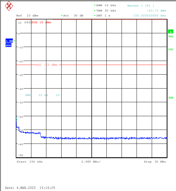
Band26(814-824)-10MHz-16QAM-26740-50RB#0-0.15~30-PASS
