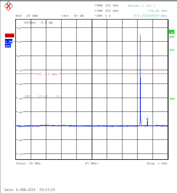
Band26(824-849)-1.4MHz-16QAM-26797-1RB#0- 30~1000-PASS
