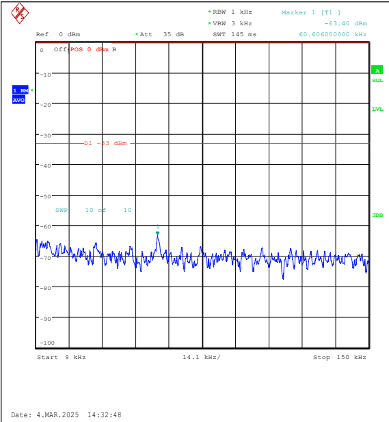
Band26(814-824)-5MHz-QPSK-26715-25RB#0-0.009~0.15-PASS
