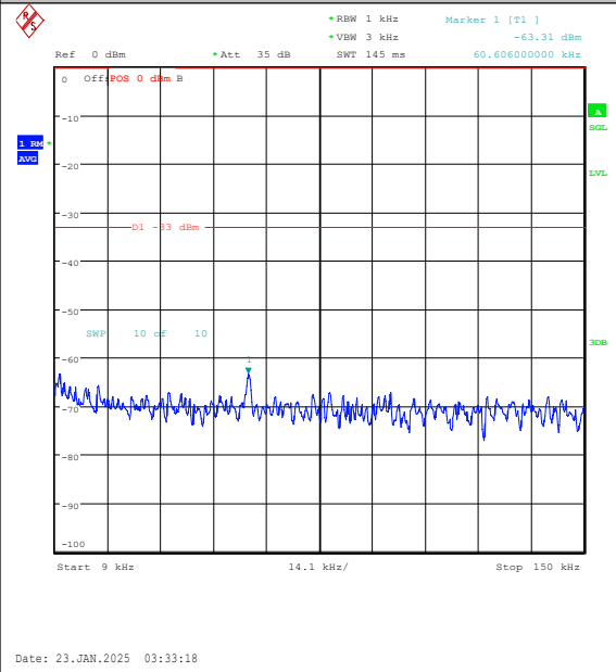
Band26(814-824)-1.4MHz-16QAM-26783-6RB#0-0.009~0.15-PASS
