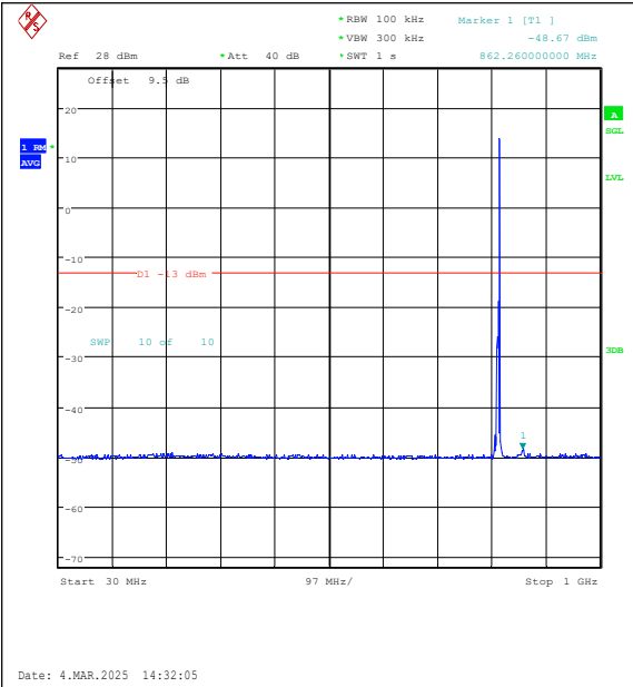
Band26(814-824)-5MHz-16QAM-26715-1RB#24-3 0~1000-PASS
