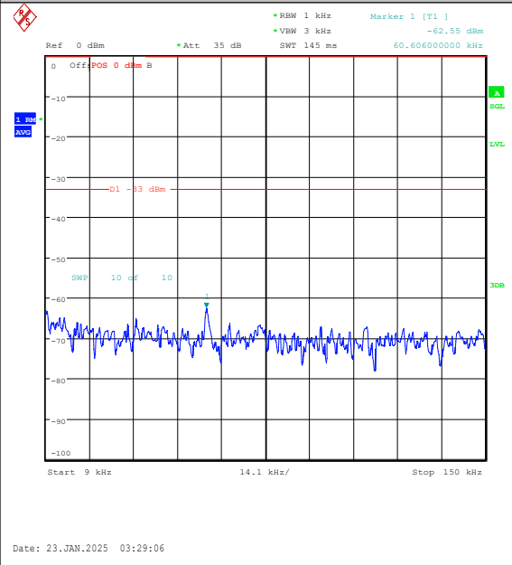
Band26(814-824)-1.4MHz-QPSK-26783-1RB#5-0. 009~0.15-PASS
