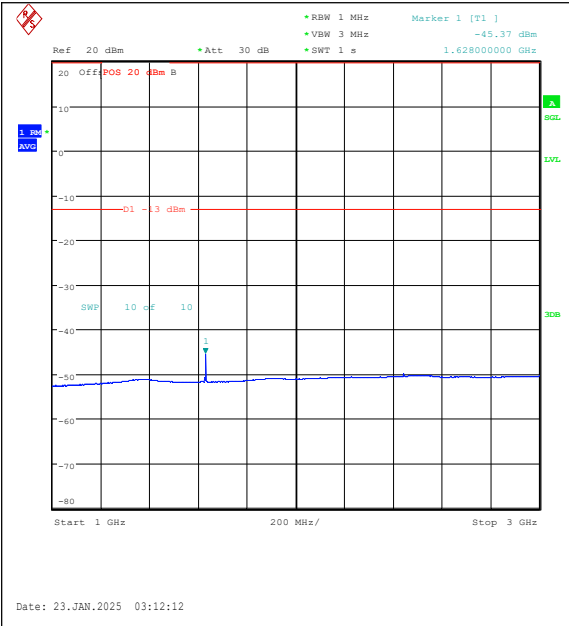
Band26(814-824)-1.4MHz-16QAM-26697-1RB#0-1000~3000-PASS
