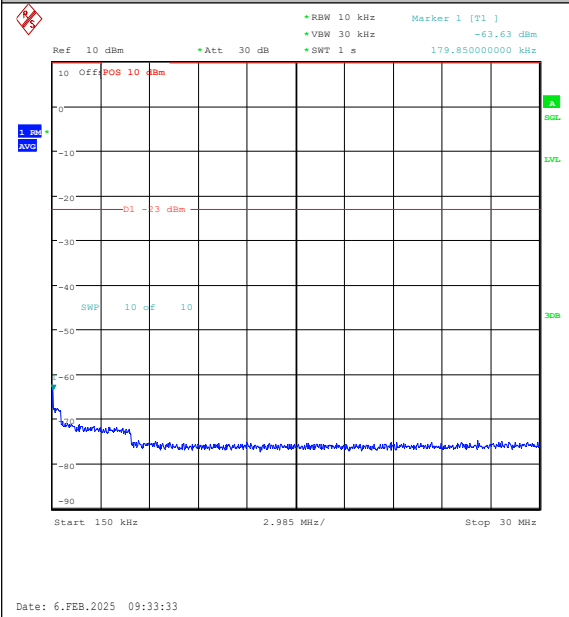
Band26(824-849)-1.4MHz-QPSK-26915-1RB#5-0. 15~30-PASS
