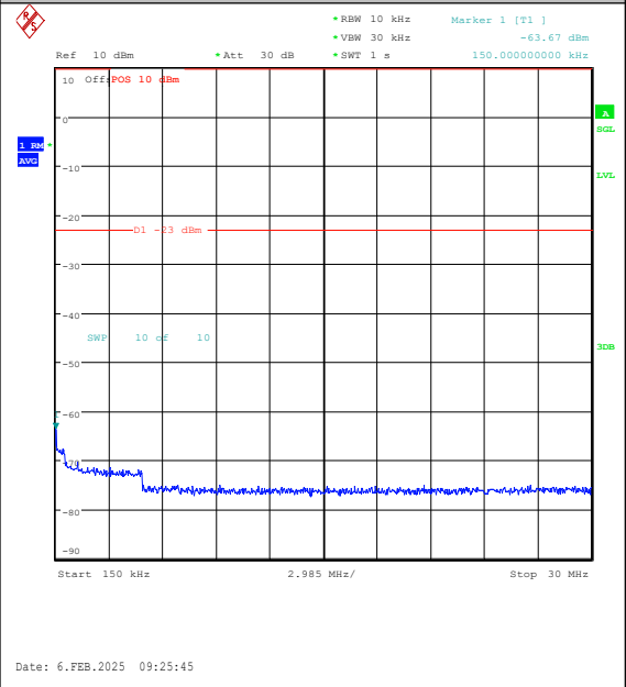
Band26(824-849)-1.4MHz-16QAM-26797-1RB#5-0.15~30-PASS
