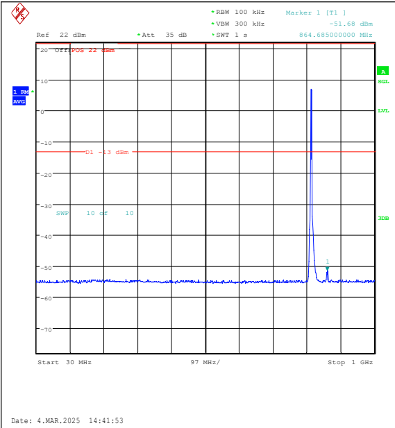
Band26(814-824)-5MHz-QPSK-26740-25RB#0-30 ~1000-PASS
