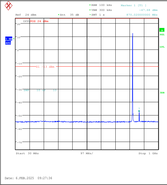
Band26(824-849)-1.4MHz-QPSK-26797-6RB#0-3 0~1000-PASS
