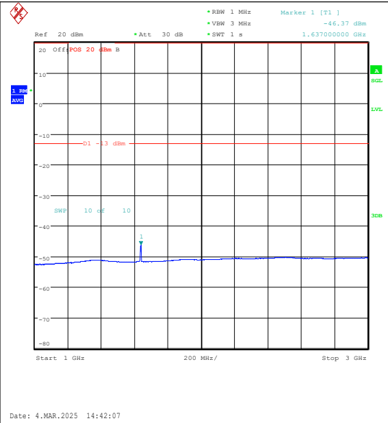
Band26(814-824)-5MHz-QPSK-26740-25RB#0-10 00~3000-PASS
