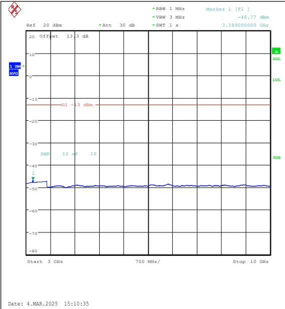
Band26(814-824)-10MHz-QPSK-26740-1RB#0-30 00~10000-PASS
