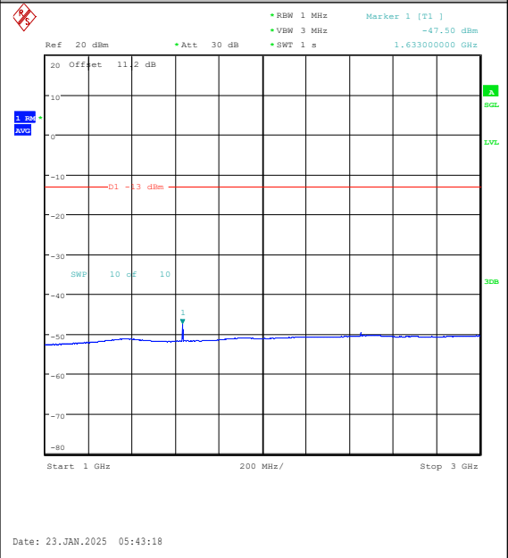
Band26(814-824)-3MHz-16QAM-26705-1RB#14-1 000~3000-PASS
