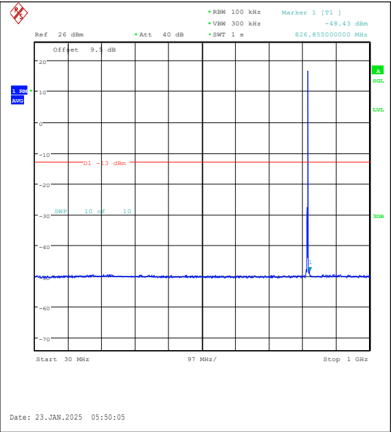
Band26(814-824)-3MHz-QPSK-26740-1RB#14-30 ~1000-PASS
