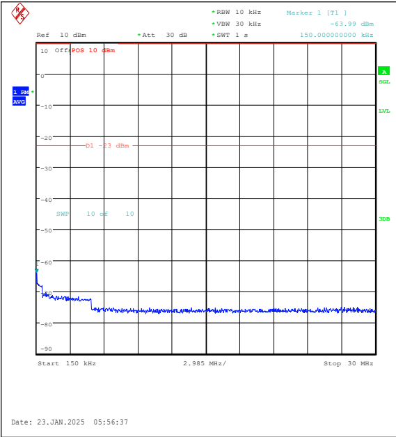
Band26(814-824)-3MHz-16QAM-26775-1RB#0-0. 15~30-PASS
