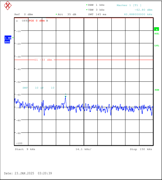
Band26(814-824)-1.4MHz-QPSK-26740-1RB#5-0. 009~0.15-PASS
