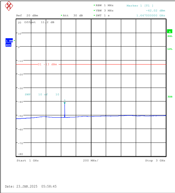
Band26(814-824)-3MHz-QPSK-26775-1RB#14-10 00~3000-PASS
