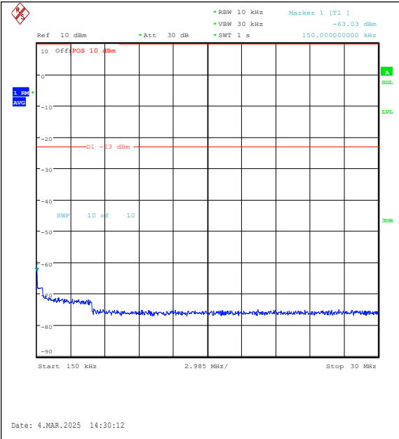
Band26(814-824)-5MHz-QPSK-26715-1RB#24-0. 15~30-PASS
