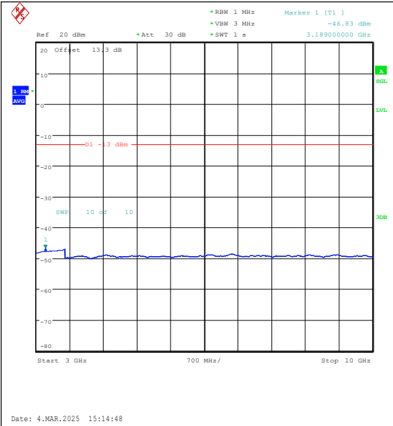
Band26(814-824)-10MHz-16QAM-26740-1RB#49-3000~10000-PASS
