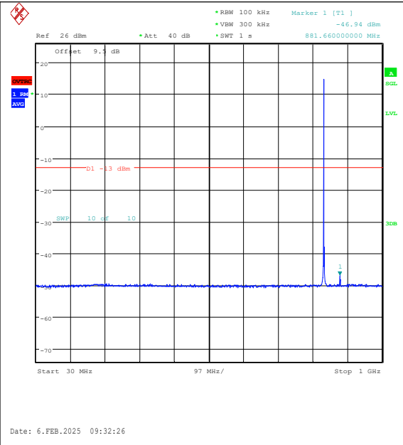
Band26(824-849)-1.4MHz-16QAM-26915-1RB#0-30~1000-PASS
