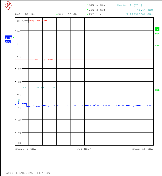
Band26(814-824)-5MHz-QPSK-26740-25RB#0-30 00~10000-PASS
