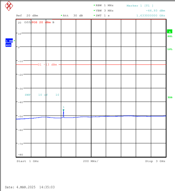
Band26(814-824)-5MHz-16QAM-26715-25RB#0-1 000~3000-PASS
