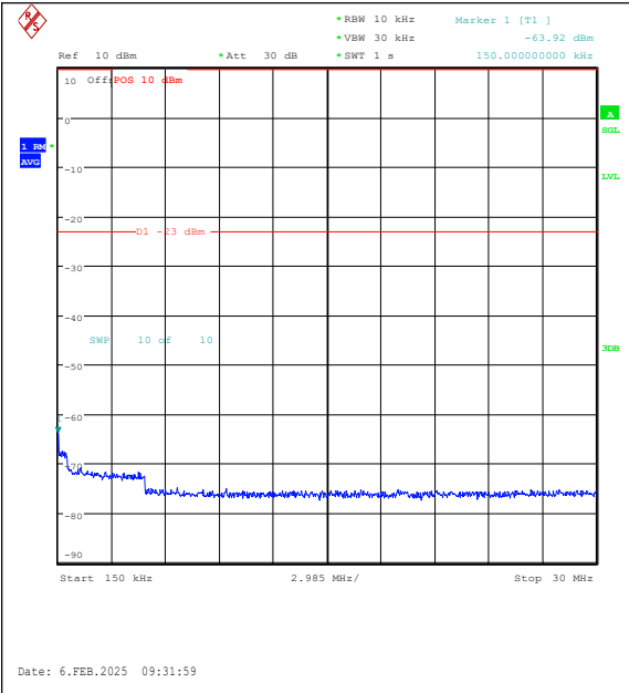
Band26(824-849)-1.4MHz-16QAM-26915-1RB#0-0.15~30-PASS
