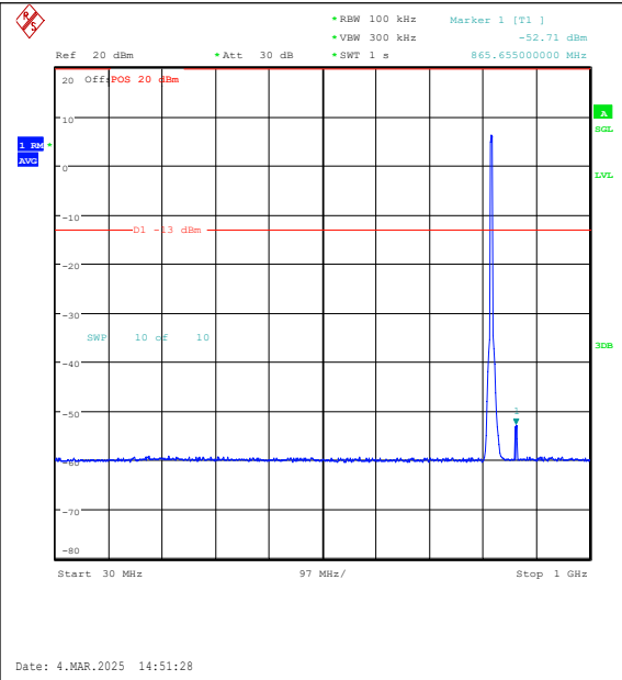
Band26(814-824)-5MHz-16QAM-26765-25RB#0-3 0~1000-PASS
