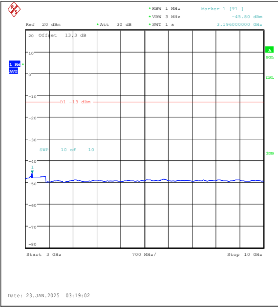
Band26(814-824)-1.4MHz-QPSK-26740-1RB#0-3 000~10000-PASS
