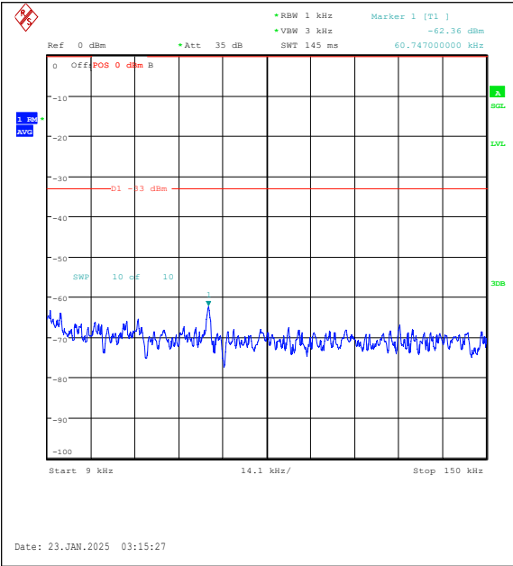
Band26(814-824)-1.4MHz-QPSK-26697-6RB#0-0.009~0.15-PASS
