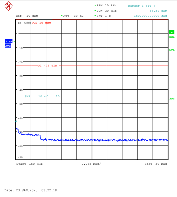
Band26(814-824)-1.4MHz-16QAM-26740-1RB#5-0.15~30-PASS
