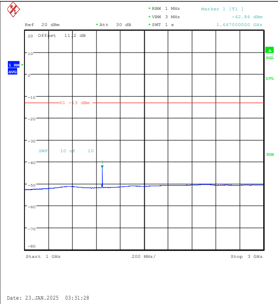
Band26(814-824)-1.4MHz-16QAM-26783-1RB#5-1000~3000-PASS
