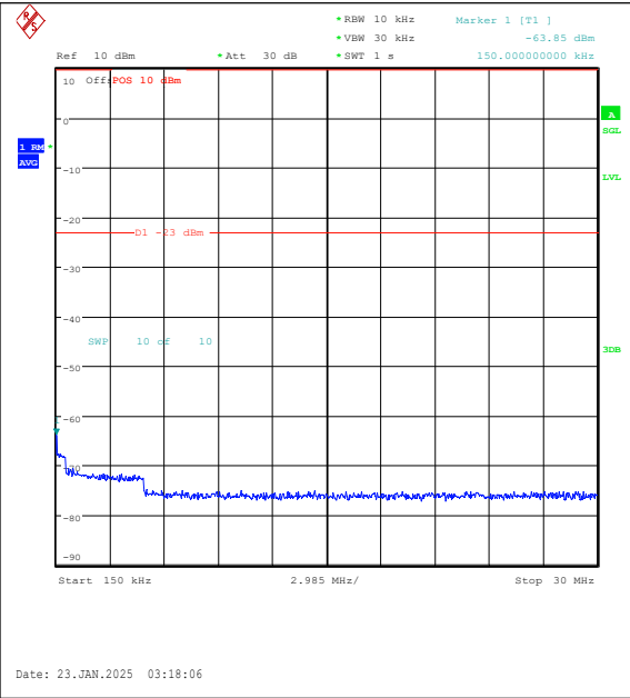
Band26(814-824)-1.4MHz-QPSK-26740-1RB#0-0.15~30-PASS
