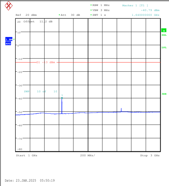
Band26(814-824)-3MHz-QPSK-26740-1RB#14-10 00~3000-PASS
