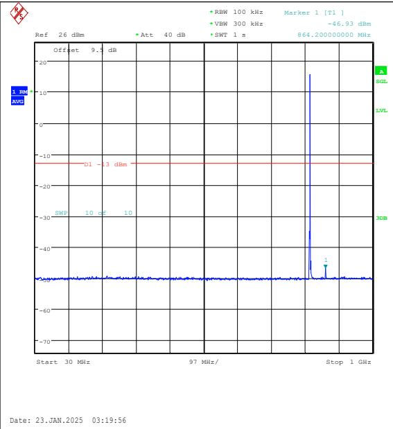
Band26(814-824)-1.4MHz-16QAM-26740-1RB#0-30~1000-PASS
