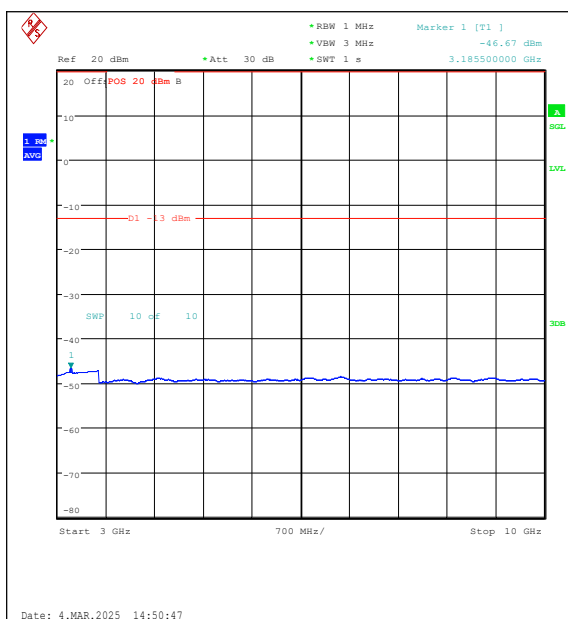
Band26(814-824)-5MHz-QPSK-26765-25RB#0-30 00~10000-PASS
