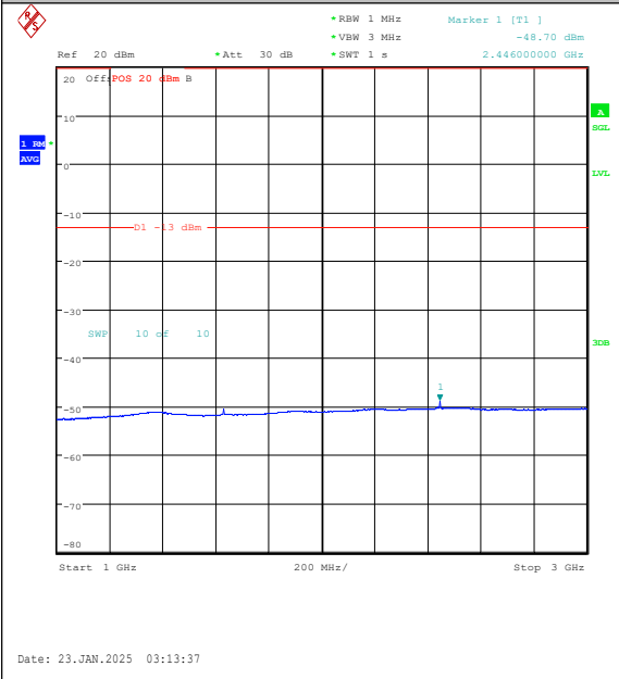
Band26(814-824)-1.4MHz-QPSK-26697-1RB#5-1 000~3000-PASS
