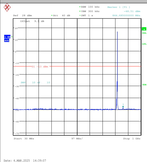
Band26(814-824)-5MHz-QPSK-26740-1RB#24-30 ~1000-PASS
