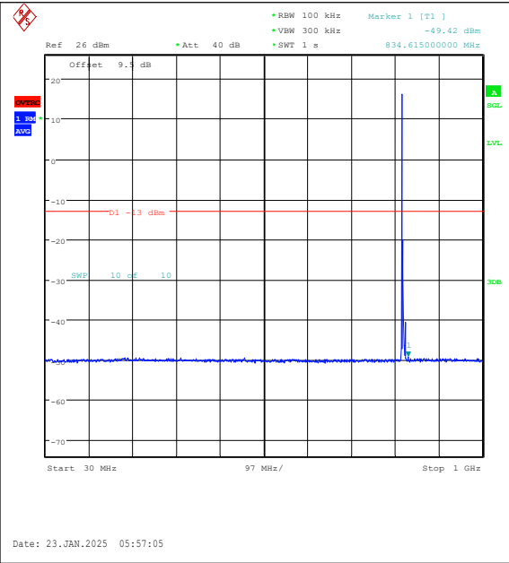
Band26(814-824)-3MHz-16QAM-26775-1RB#0-30 ~1000-PASS
