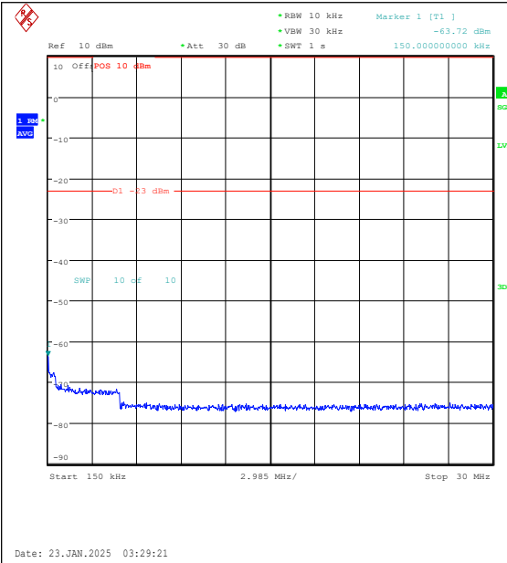
Band26(814-824)-1.4MHz-QPSK-26783-1RB#5-0. 15~30-PASS
