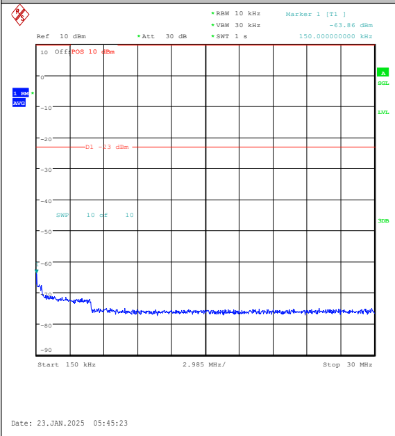
Band26(814-824)-3MHz-16QAM-26705-15RB#0-0 .15~30-PASS
