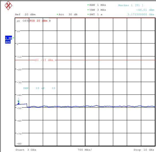
Band26(814-824)-1.4MHz-QPSK-26740-6RB#0-3 0~1000-PASS
