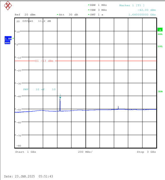
Band26(814-824)-3MHz-16QAM-26740-1RB#14-1 000~3000-PASS
