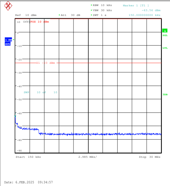
Band26(824-849)-1.4MHz-16QAM-26915-1RB#5-0.15~30-PASS
