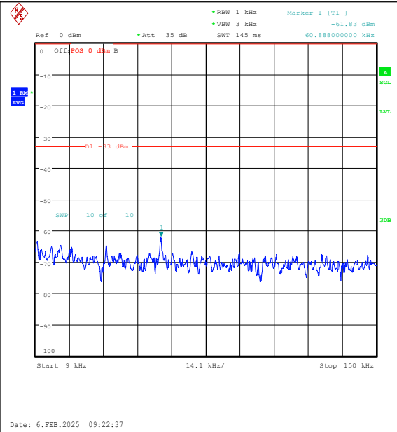
Band26(824-849)-1.4MHz-16QAM-26797-1RB#0- 0.009~0.15-PASS
