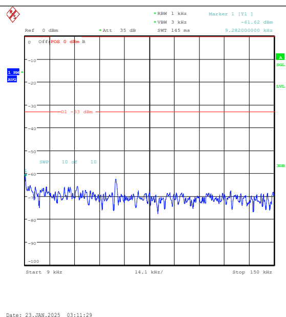
Band26(814-824)-1.4MHz-16QAM-26697-1RB#0- 0.009~0.15-PASS
