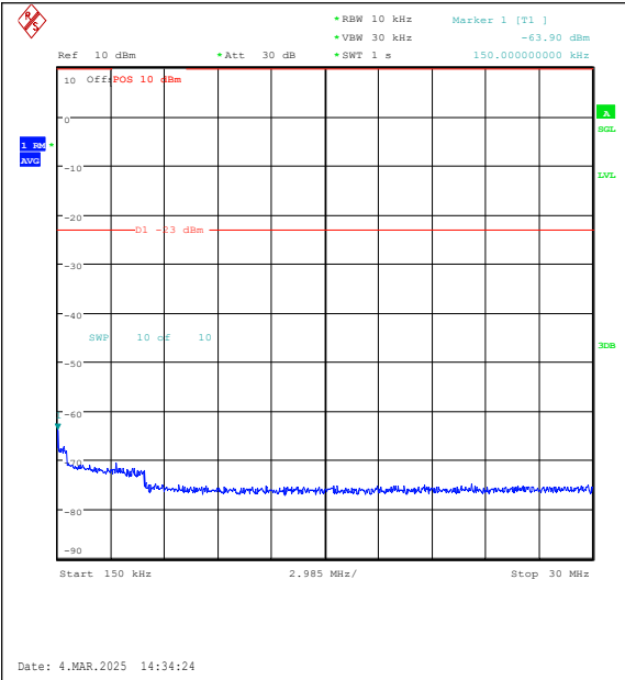
Band26(814-824)-5MHz-16QAM-26715-25RB#0-0 .15~30-PASS
