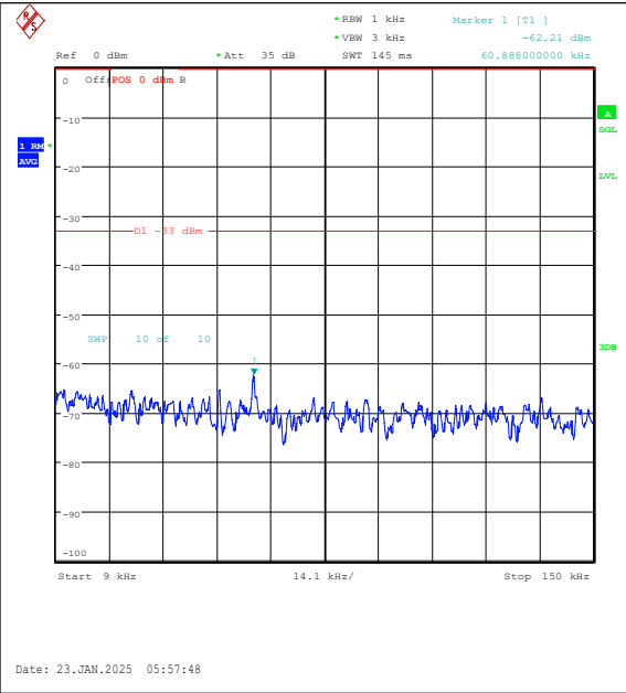
Band26(814-824)-3MHz-QPSK-26775-1RB#14-0. 009~0.15-PASS
