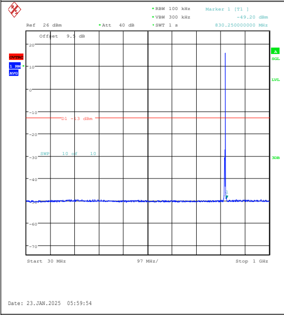
Band26(814-824)-3MHz-16QAM-26775-1RB#14-3 0~1000-PASS
