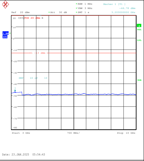
Band26(814-824)-3MHz-16QAM-26740-15RB#0-3 000~10000-PASS
