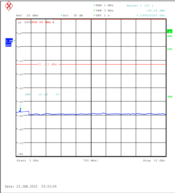
Band26(814-824)-1.4MHz-QPSK-26783-6RB#0-3 000~10000-PASS
