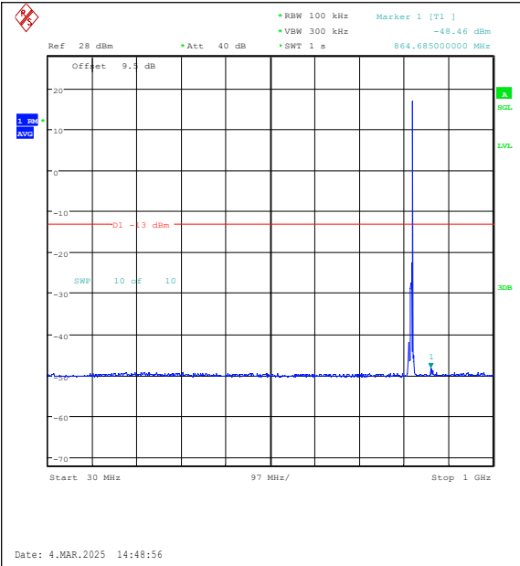
Band26(814-824)-5MHz-16QAM-26765-1RB#24-3 0~1000-PASS
