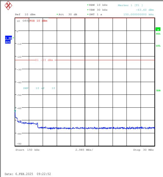
Band26(824-849)-1.4MHz-16QAM-26797-1RB#0- 0.15~30-PASS
