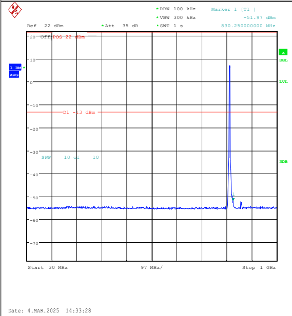
Band26(814-824)-5MHz-QPSK-26715-25RB#0-30~1000-PASS
