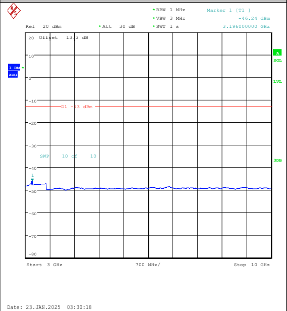
Band26(814-824)-1.4MHz-QPSK-26783-1RB#5-3 000~10000-PASS
