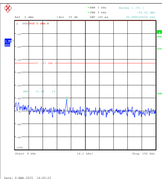
Band26(814-824)-5MHz-16QAM-26765-1RB#0-0. 009~0.15-PASS
