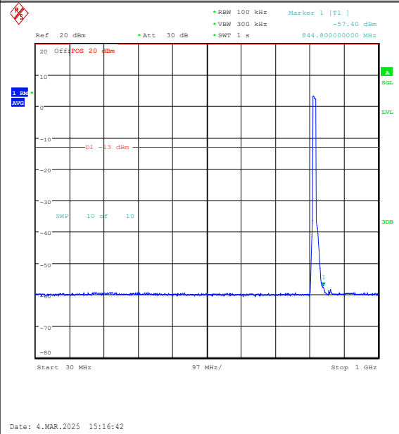
Band26(814-824)-10MHz-16QAM-26740-50RB#0-30~1000-PASS
