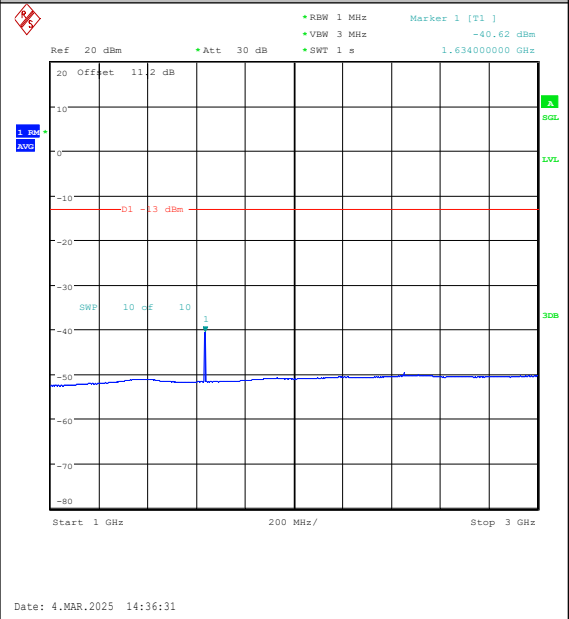
Band26(814-824)-5MHz-QPSK-26740-1RB#0-100 0~3000-PASS
