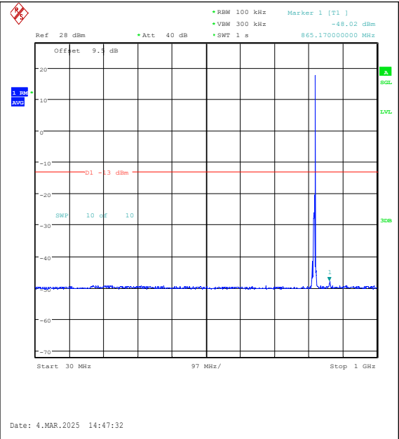
Band26(814-824)-5MHz-QPSK-26765-1RB#24-30 ~1000-PASS
