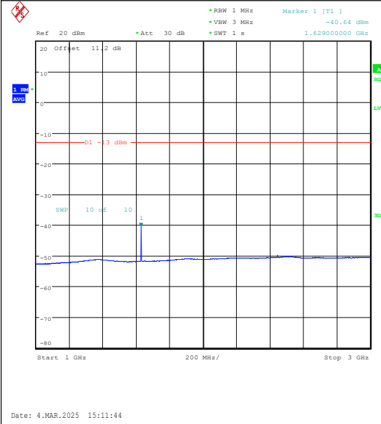
Band26(814-824)-10MHz-16QAM-26740-1RB#0-1 000~3000-PASS
