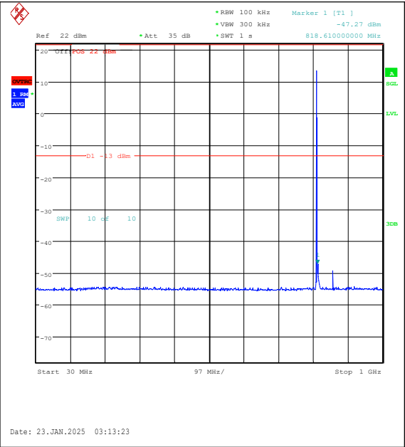
Band26(814-824)-1.4MHz-QPSK-26697-1RB#5-3 0~1000-PASS
