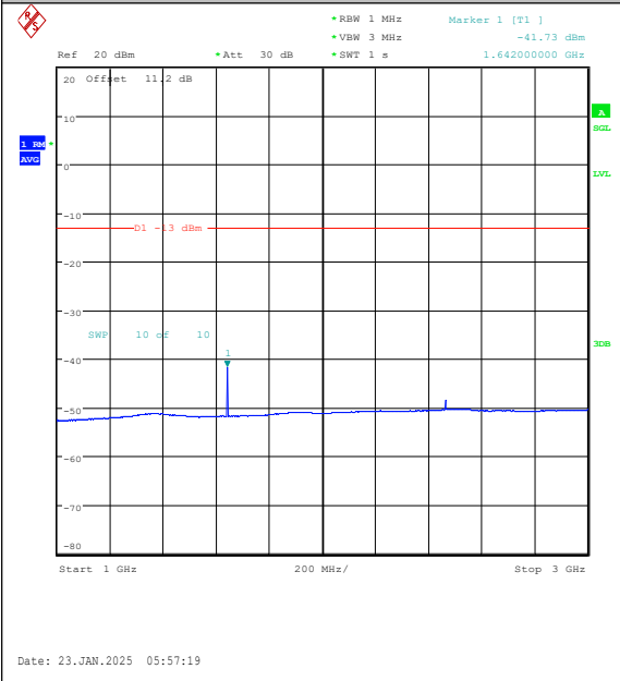
Band26(814-824)-3MHz-16QAM-26775-1RB#0-10 00~3000-PASS
