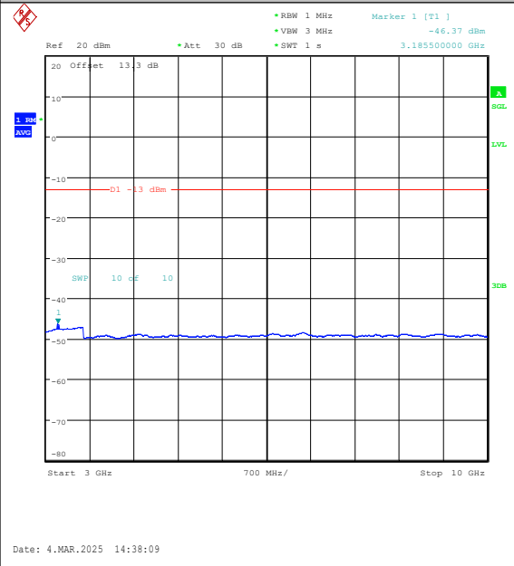
Band26(814-824)-5MHz-16QAM-26740-1RB#0-30 00~10000-PASS
