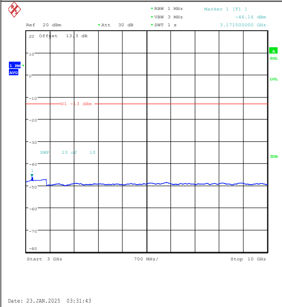
Band26(814-824)-1.4MHz-16QAM-26783-1RB#5-3000~10000-PASS
