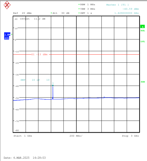
Band26(814-824)-5MHz-QPSK-26715-1RB#0-1000~3000-PASS
