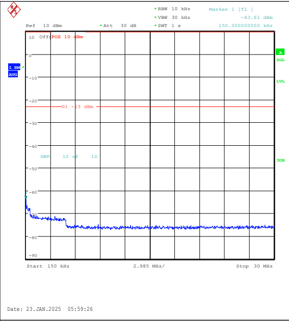
Band26(814-824)-3MHz-16QAM-26775-1RB#14-0 .15~30-PASS
