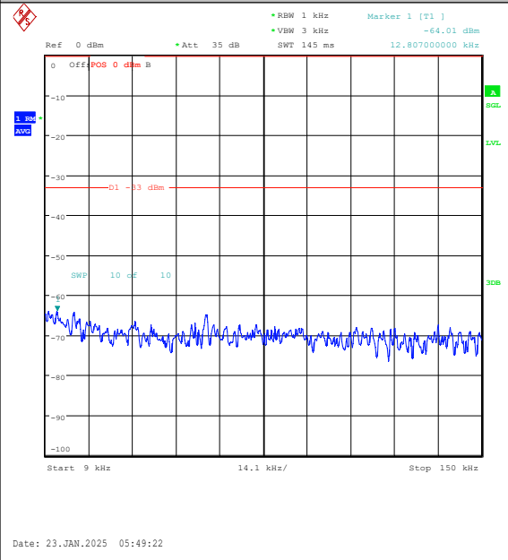
Band26(814-824)-3MHz-QPSK-26740-1RB#14-0.009~0.15-PASS
