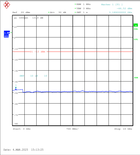
Band26(814-824)-10MHz-QPSK-26740-1RB#49-3 000~10000-PASS
