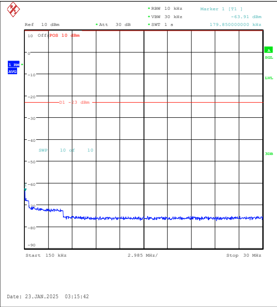
Band26(814-824)-1.4MHz-QPSK-26697-6RB#0-0.15~30-PASS
