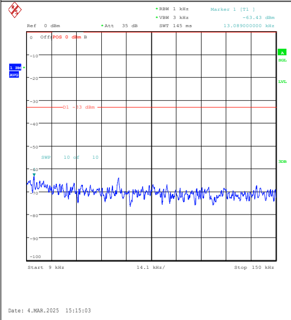
Band26(814-824)-10MHz-QPSK-26740-50RB#0-0 .009~0.15-PASS
