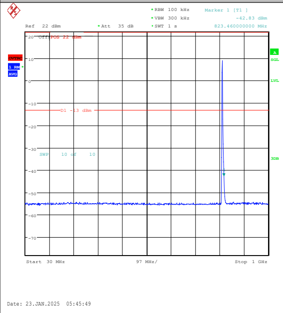
Band26(814-824)-3MHz-16QAM-26705-15RB#0-3 0~1000-PASS
