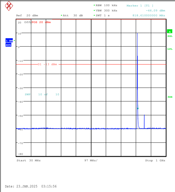
Band26(814-824)-1.4MHz-QPSK-26697-6RB#0-0.0~1000-PASS
