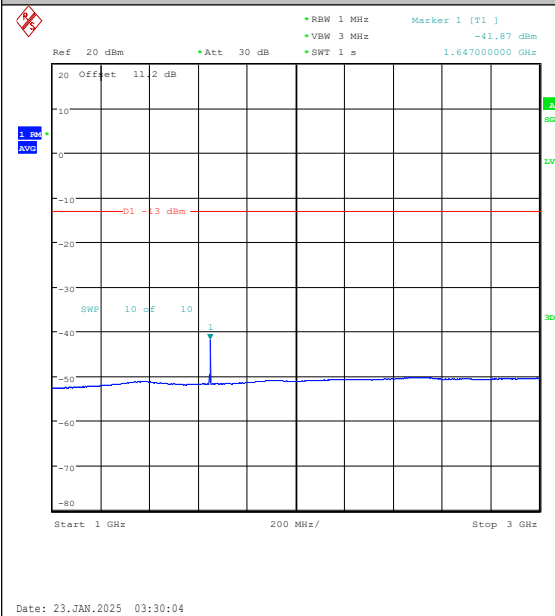
Band26(814-824)-1.4MHz-QPSK-26783-1RB#5-1 000~3000-PASS
