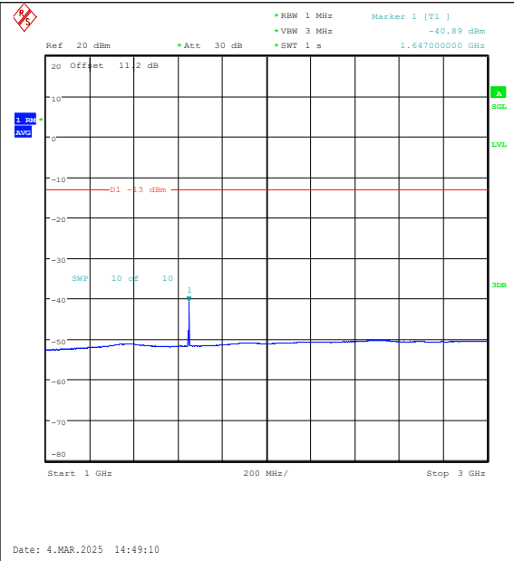
Band26(814-824)-5MHz-16QAM-26765-1RB#24-1 000~3000-PASS
