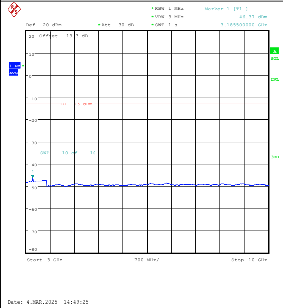
Band26(814-824)-5MHz-16QAM-26765-1RB#24-3 000~10000-PASS
