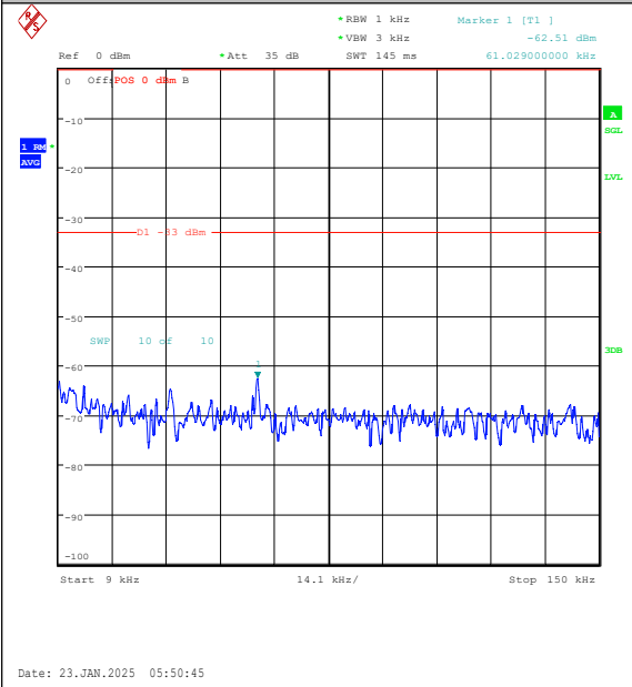
Band26(814-824)-3MHz-16QAM-26740-1RB#14-0 .009~0.15-PASS
