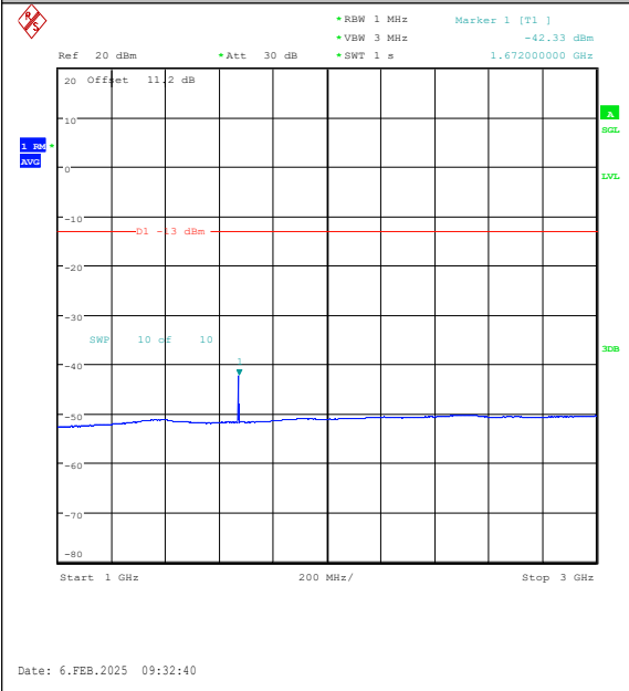
Band26(824-849)-1.4MHz-16QAM-26915-1RB#0-1000~3000-PASS
