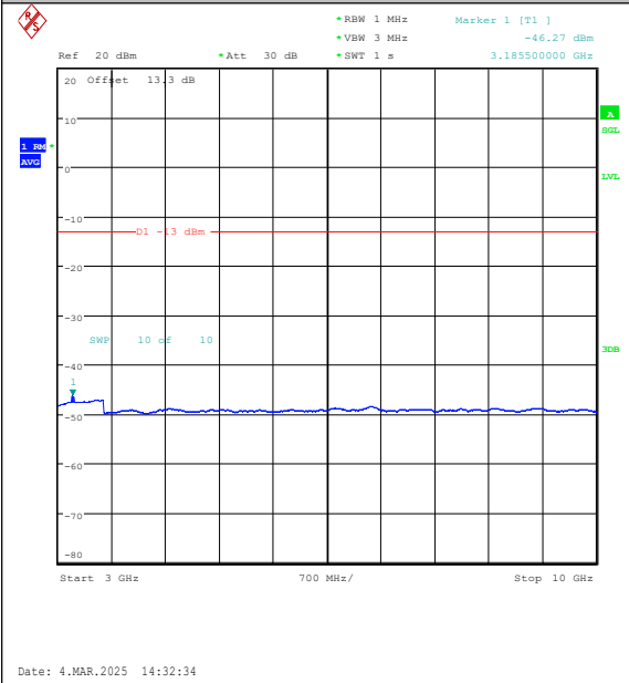
Band26(814-824)-5MHz-16QAM-26715-1RB#24-3 000~10000-PASS
