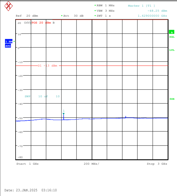
Band26(814-824)-1.4MHz-QPSK-26697-6RB#0-1.000~3000-PASS
