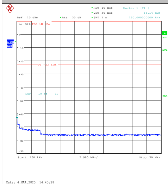
Band26(814-824)-5MHz-16QAM-26765-1RB#0-0. 15~30-PASS
