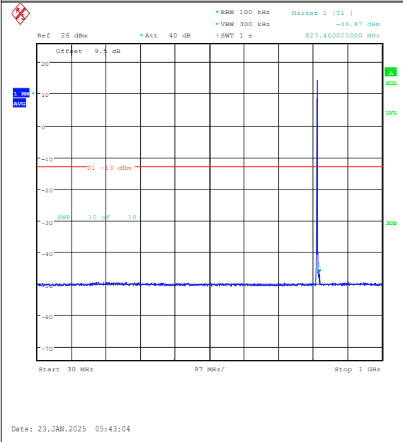
Band26(814-824)-3MHz-16QAM-26705-1RB#14-3 0~1000-PASS
