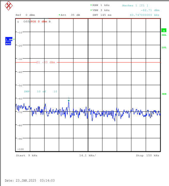
Band26(814-824)-1.4MHz-16QAM-26697-1RB#5-0.009~0.15-PASS
