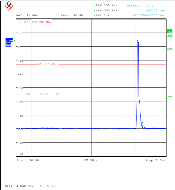
Band26(814-824)-10MHz-QPSK-26740-50RB#0-3 0~1000-PASS
