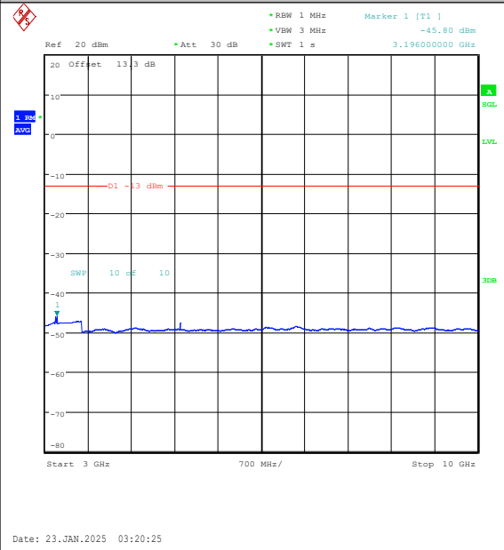
Band26(814-824)-1.4MHz-16QAM-26740-1RB#0-3000~10000-PASS
