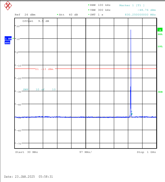
Band26(814-824)-3MHz-QPSK-26775-1RB#14-30 ~1000-PASS
