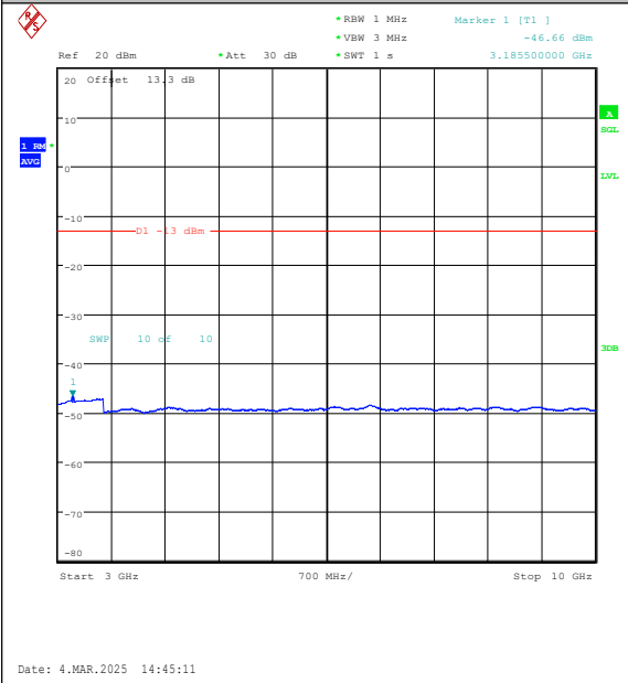
Band26(814-824)-5MHz-QPSK-26765-1RB#0-3000~10000-PASS
