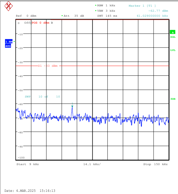
Band26(814-824)-10MHz-16QAM-26740-50RB#0-0.009~0.15-PASS
