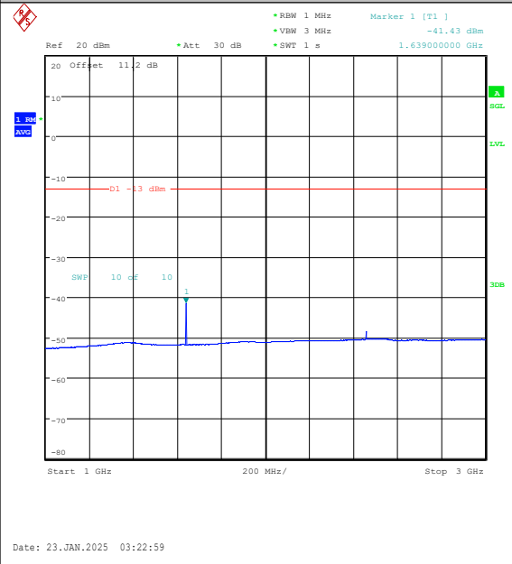
Band26(814-824)-1.4MHz-16QAM-26740-1RB#5-1000~3000-PASS
