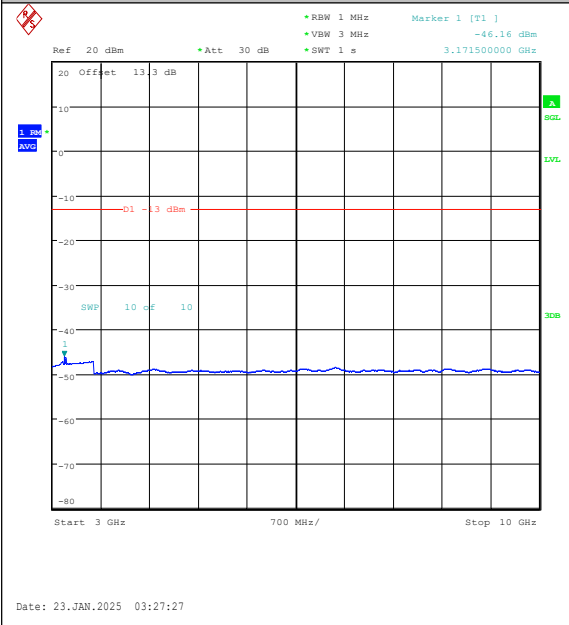
Band26(814-824)-1.4MHz-QPSK-26783-1RB#0-3 000~10000-PASS
