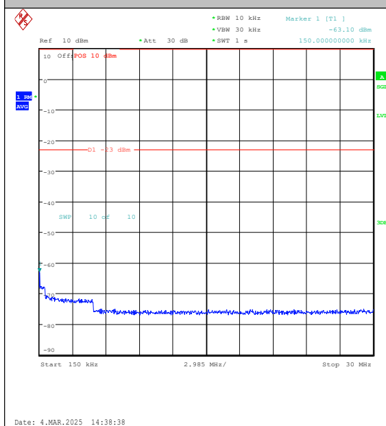
Band26(814-824)-5MHz-QPSK-26740-1RB#24-0. 15~30-PASS
