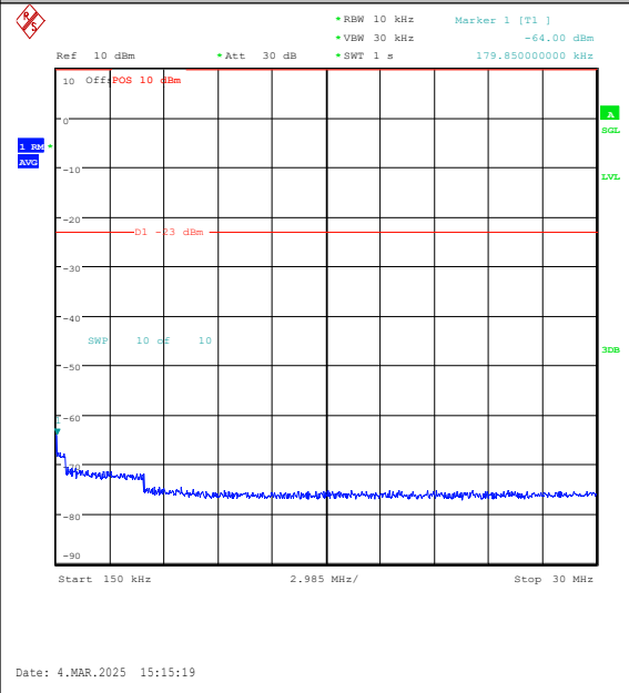
Band26(814-824)-10MHz-QPSK-26740-50RB#0-0 .15~30-PASS
