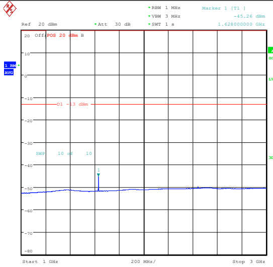
Band26(814-824)-3MHz-QPSK-26705-1RB#0-0.1 5~30-PASS
