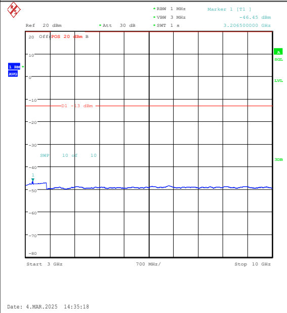
Band26(814-824)-5MHz-16QAM-26715-25RB#0-3 000~10000-PASS
