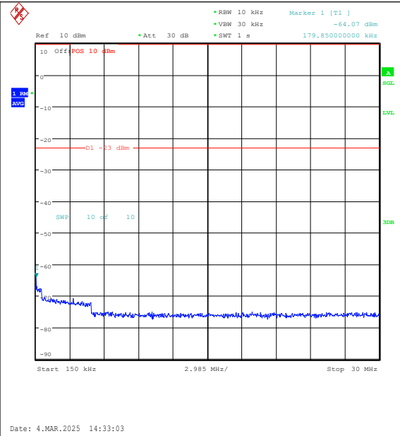
Band26(814-824)-5MHz-QPSK-26715-25RB#0-0.15~30-PASS
