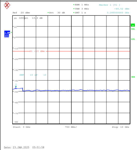
Band26(814-824)-3MHz-16QAM-26740-1RB#14-3 000~10000-PASS
