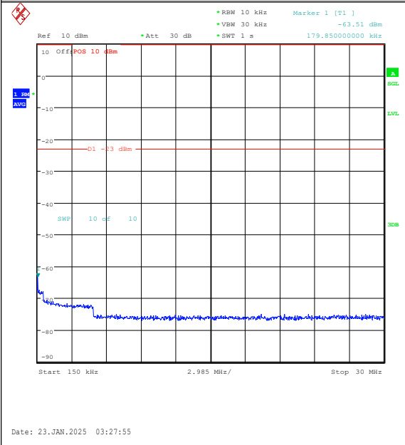
Band26(814-824)-1.4MHz-16QAM-26783-1RB#0- 0.15~30-PASS
