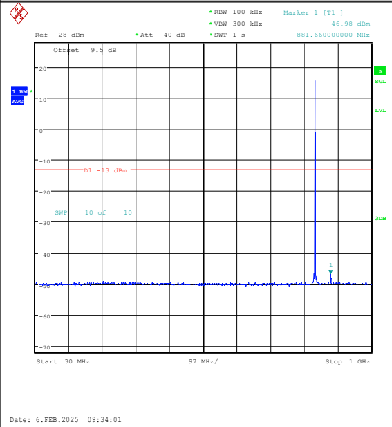
Band26(824-849)-1.4MHz-QPSK-26915-1RB#5-3 0~1000-PASS
