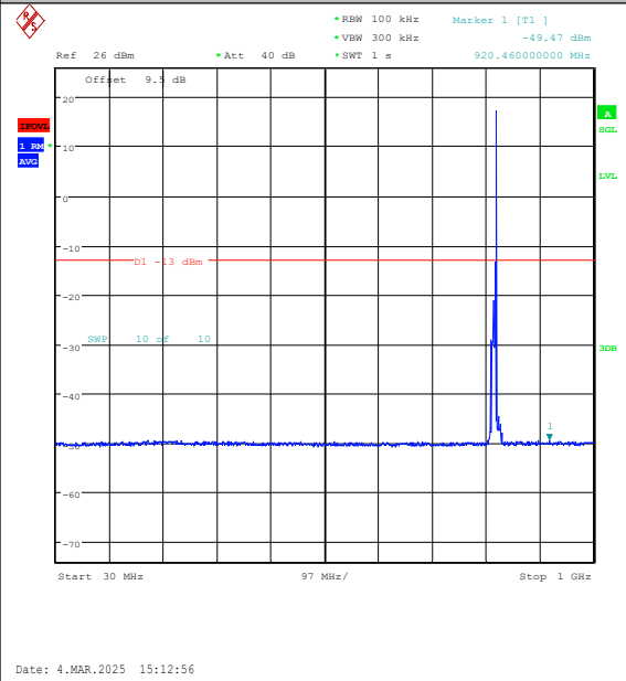
Band26(814-824)-10MHz-QPSK-26740-1RB#49-3 0~1000-PASS
