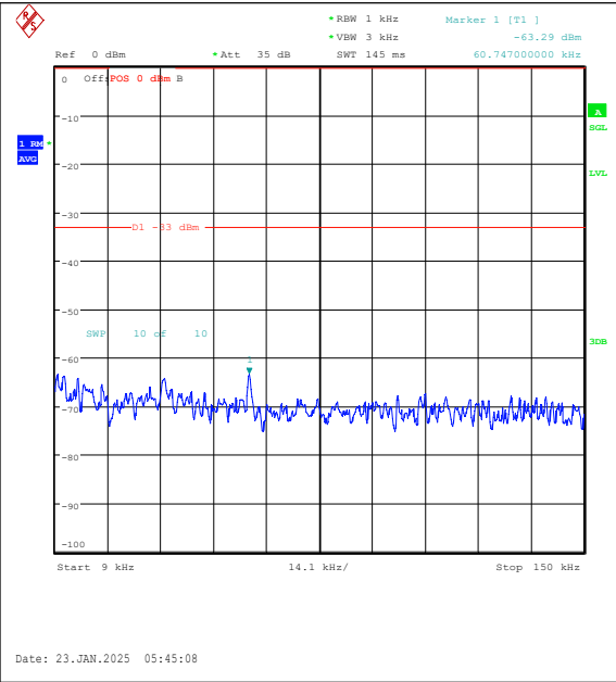
Band26(814-824)-3MHz-16QAM-26705-15RB#0-0 .009~0.15-PASS
