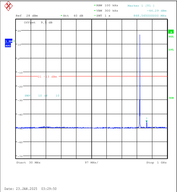
Band26(814-824)-1.4MHz-QPSK-26783-1RB#5-3 0~1000-PASS
