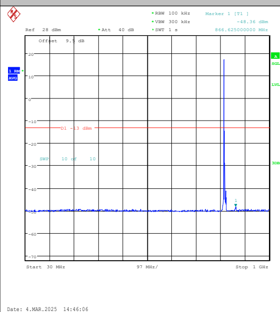
Band26(814-824)-5MHz-16QAM-26765-1RB#0-30 ~1000-PASS
