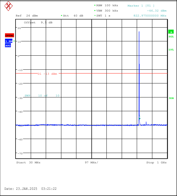
Band26(814-824)-1.4MHz-QPSK-26740-1RB#5-3 0~1000-PASS
