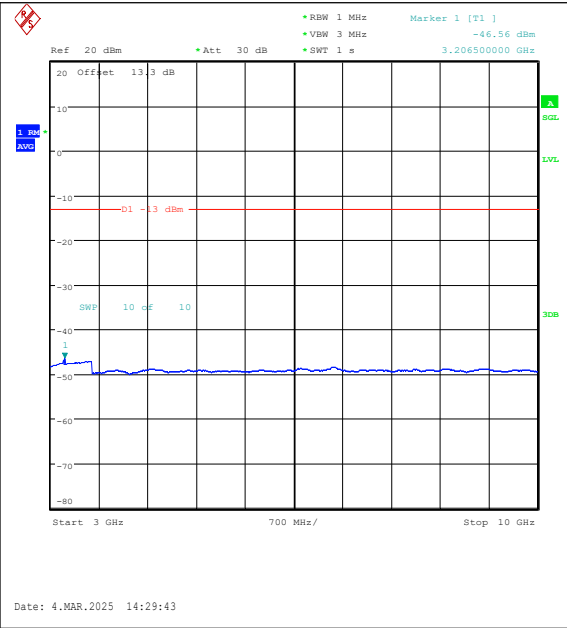
Band26(814-824)-5MHz-16QAM-26715-1RB#0-30 00~10000-PASS
