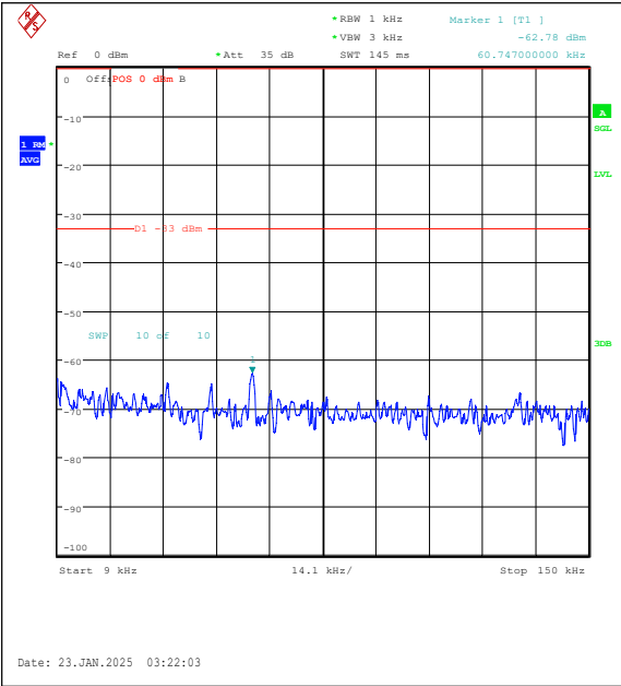
Band26(814-824)-1.4MHz-16QAM-26740-1RB#5-0.009~0.15-PASS
