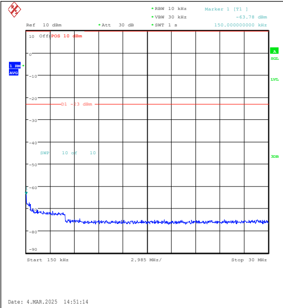
Band26(814-824)-5MHz-16QAM-26765-25RB#0-0 .15~30-PASS
