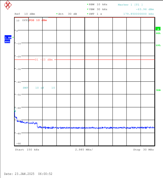
Band26(814-824)-3MHz-QPSK-26775-15RB#0-0. 15~30-PASS
