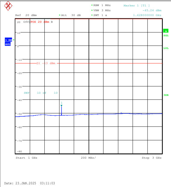
Band26(814-824)-1.4MHz-QPSK-26697-1RB#0-1 000~3000-PASS
