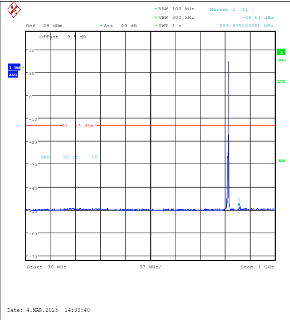
Band26(814-824)-5MHz-QPSK-26715-1RB#24-30 ~1000-PASS
