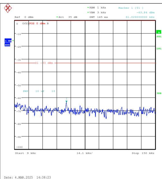
Band26(814-824)-5MHz-QPSK-26740-1RB#24-0. 009~0.15-PASS
