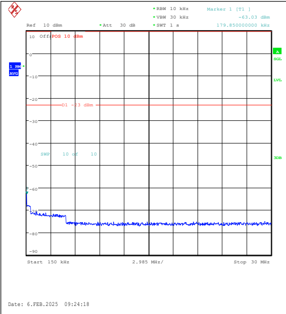
Band26(824-849)-1.4MHz-QPSK-26797-1RB#5-0. 15~30-PASS
