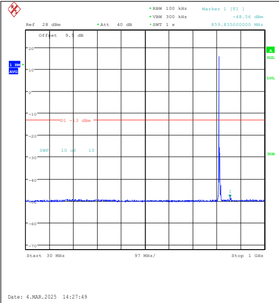
Band26(814-824)-5MHz-QPSK-26715-1RB#0-30~1000-PASS
