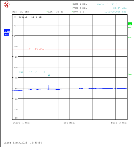
Band26(814-824)-5MHz-QPSK-26715-1RB#24-10 00~3000-PASS
