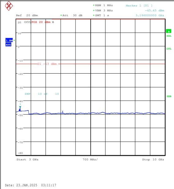
Band26(814-824)-1.4MHz-QPSK-26697-1RB#0-3 000~10000-PASS
