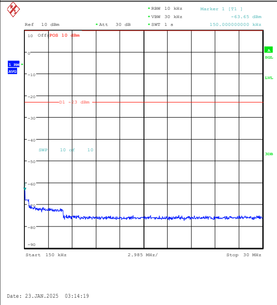
Band26(814-824)-1.4MHz-16QAM-26697-1RB#5-0.15~30-PASS
