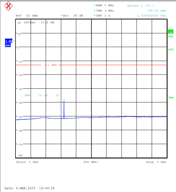
Band26(814-824)-5MHz-QPSK-26765-1RB#0-1000~3000-PASS
