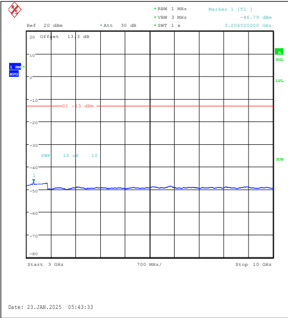
Band26(814-824)-3MHz-16QAM-26705-1RB#14-3 000~10000-PASS
