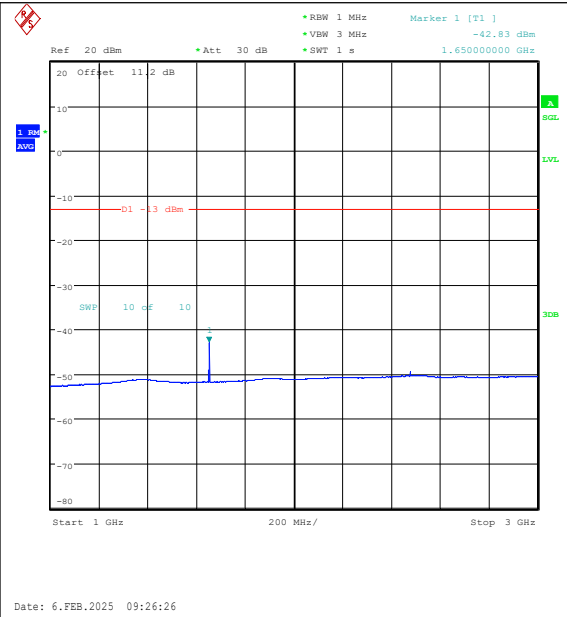
Band26(824-849)-1.4MHz-16QAM-26797-1RB#5-1000~3000-PASS
