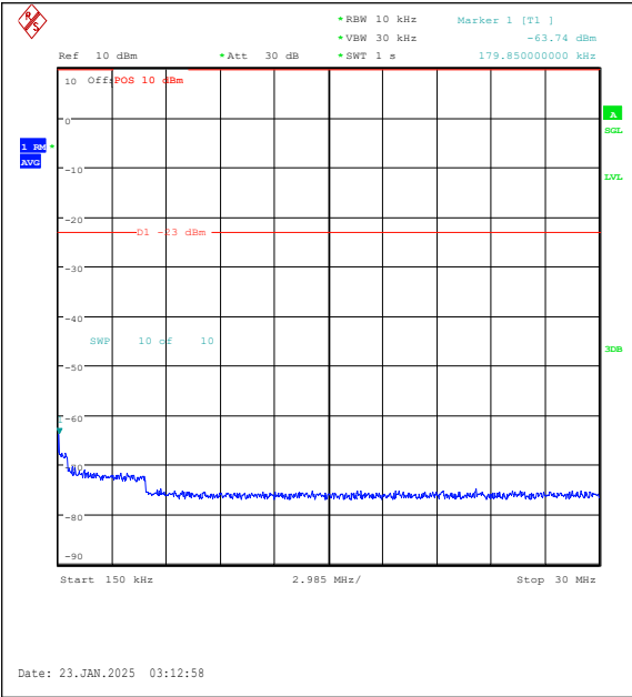
Band26(814-824)-1.4MHz-QPSK-26697-1RB#5-0. 15~30-PASS
