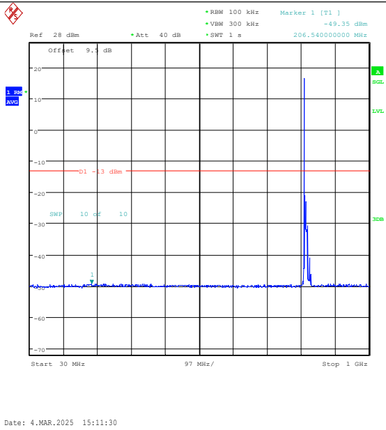
Band26(814-824)-10MHz-16QAM-26740-1RB#0-3 0~1000-PASS
