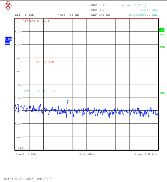
Band26(824-849)-1.4MHz-16QAM-26797-6RB#0-0.009~0.15-PASS
