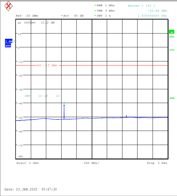
Band26(814-824)-3MHz-QPSK-26740-1RB#0-1000~3000-PASS
