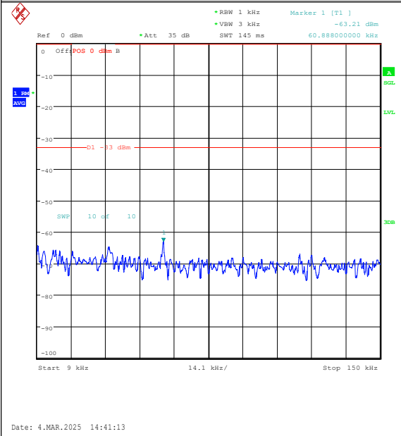
Band26(814-824)-5MHz-QPSK-26740-25RB#0-0. 009~0.15-PASS
