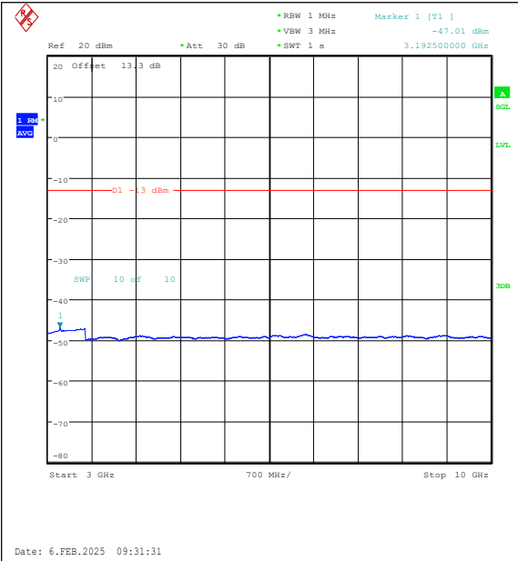
Band26(824-849)-1.4MHz-QPSK-26915-1RB#0-3 000~10000-PASS
