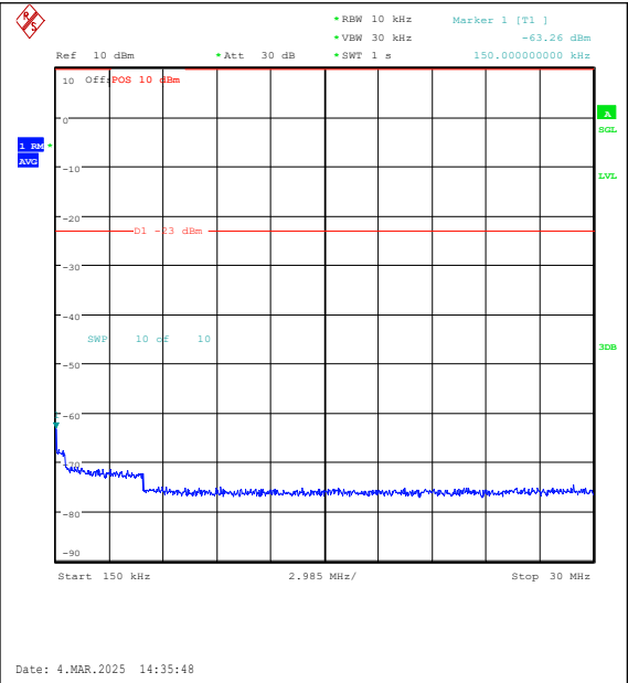
Band26(814-824)-5MHz-QPSK-26740-1RB#0-0.1 5~30-PASS
