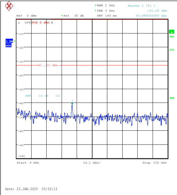
Band26(814-824)-3MHz-QPSK-26740-15RB#0-0. 009~0.15-PASS
