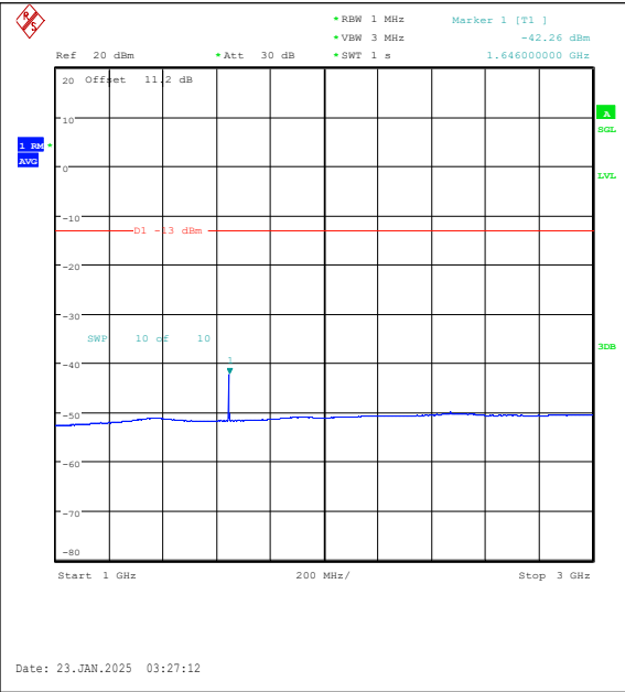
Band26(814-824)-1.4MHz-QPSK-26783-1RB#0-1 000~3000-PASS
