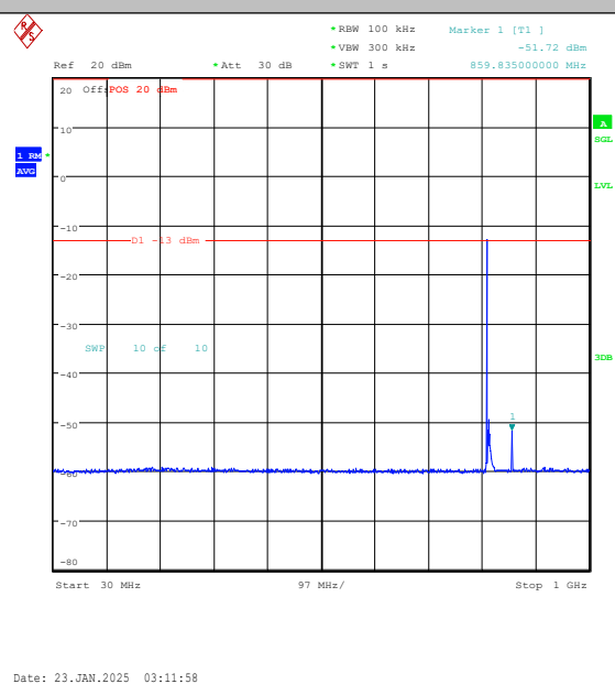
Band26(814-824)-1.4MHz-16QAM-26697-1RB#0- 30~1000-PASS
