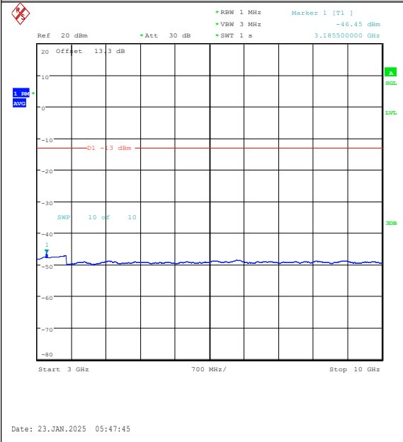
Band26(814-824)-3MHz-QPSK-26740-1RB#0-3000~10000-PASS
