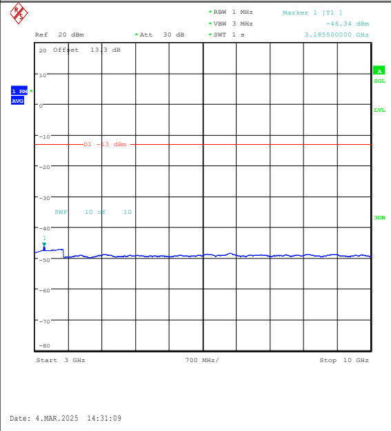
Band26(814-824)-5MHz-QPSK-26715-1RB#24-30 00~10000-PASS
