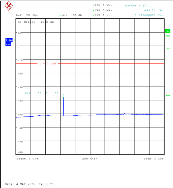
Band26(814-824)-5MHz-QPSK-26740-1RB#24-10 00~3000-PASS
