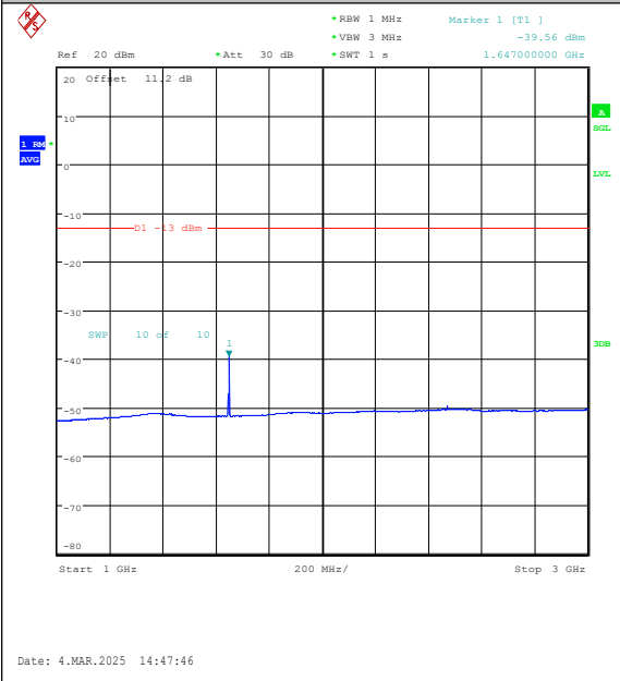
Band26(814-824)-5MHz-QPSK-26765-1RB#24-10 00~3000-PASS
