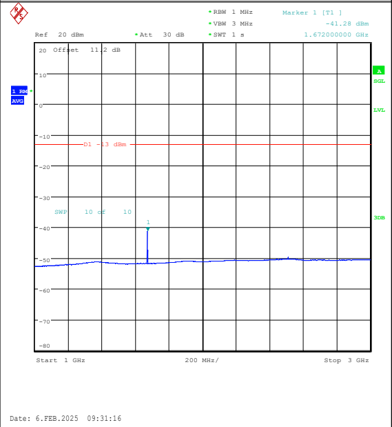
Band26(824-849)-1.4MHz-QPSK-26915-1RB#0-1000~3000-PASS
