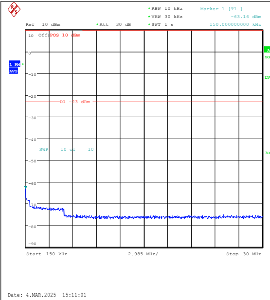
Band26(814-824)-10MHz-16QAM-26740-1RB#0-0 .15~30-PASS
