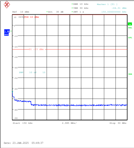
Band26(814-824)-3MHz-QPSK-26740-1RB#14-0. 15~30-PASS
