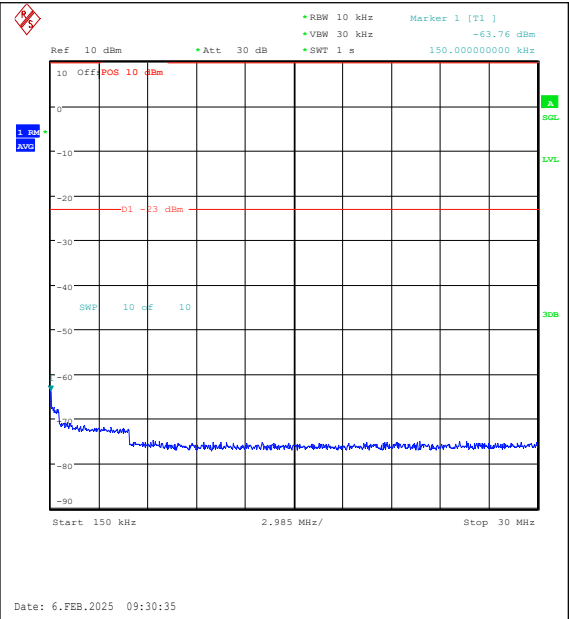
Band26(824-849)-1.4MHz-QPSK-26915-1RB#0-0.15~30-PASS
