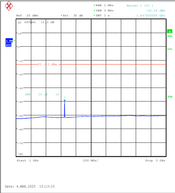
Band26(814-824)-10MHz-QPSK-26740-1RB#49-1 000~3000-PASS
