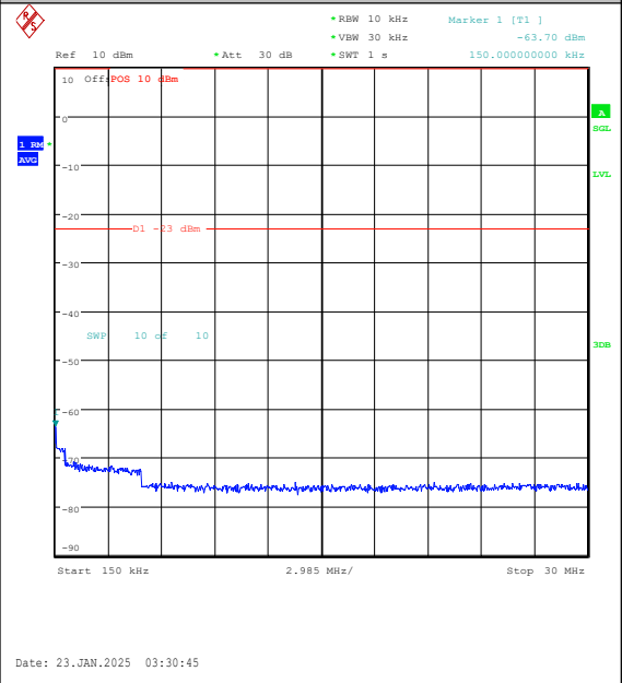
Band26(814-824)-1.4MHz-16QAM-26783-1RB#5-0.15~30-PASS
