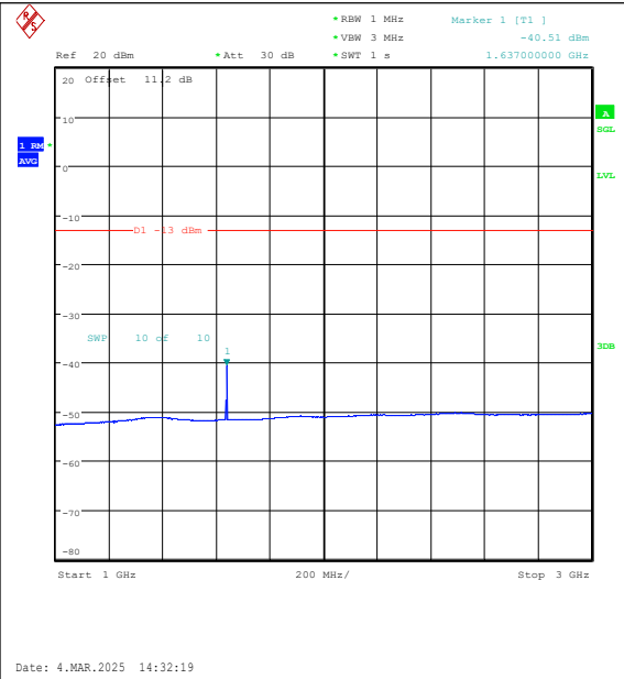
Band26(814-824)-5MHz-16QAM-26715-1RB#24-1 000~3000-PASS
