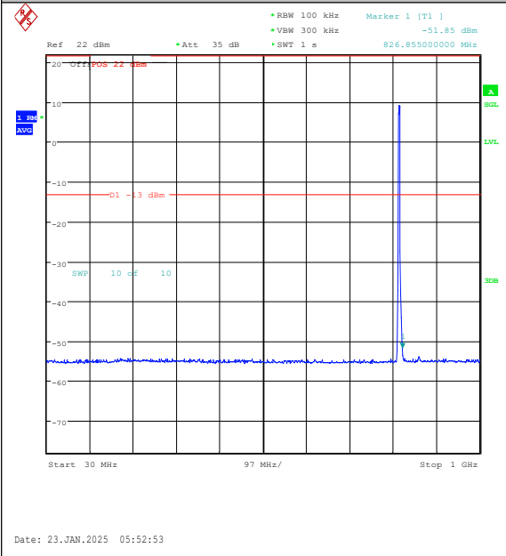
Band26(814-824)-3MHz-QPSK-26740-15RB#0-30 ~1000-PASS
