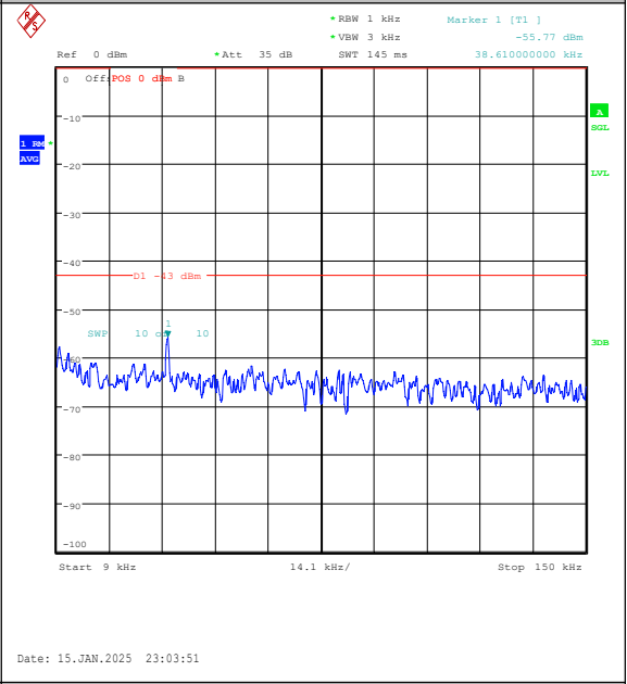
Band2-3MHz-16QAM-19185-15RB#0-0.009~0.15- PASS
