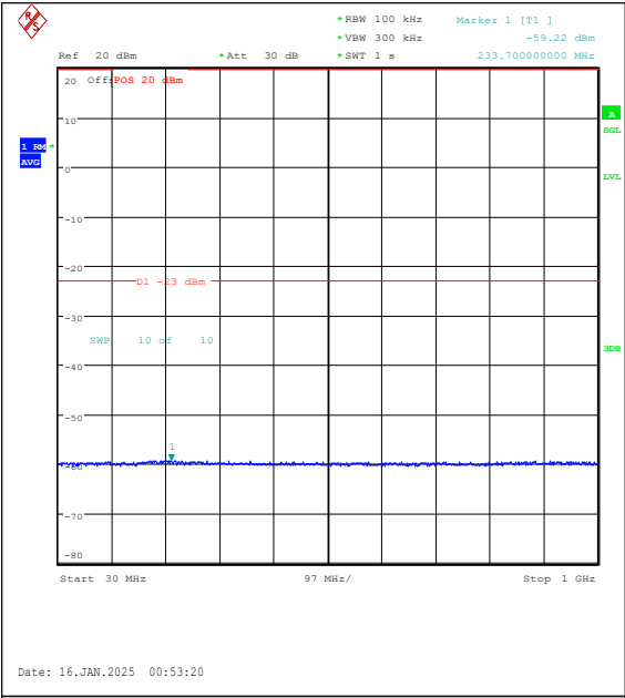
Band2-10MHz-QPSK-18900-50RB#0-30~1000-P ASS
