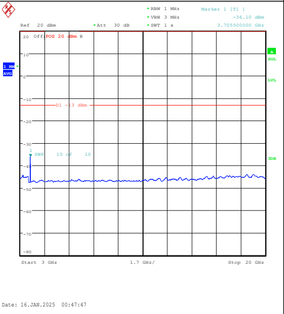
Band2-10MHz-16QAM-18650-50RB#0-3000~2000 0-PASS
