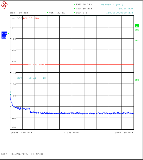
Band2-15MHz-QPSK-18675-1RB#0-0.15~30-PAS
