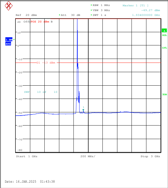
Band2-15MHz-16QAM-18675-1RB#0-1000~3000 -PASS
