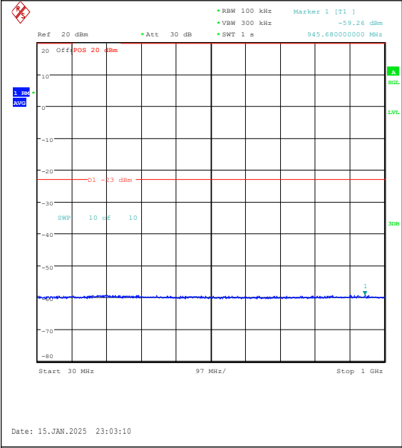
Band2-3MHz-QPSK-19185-15RB#0-30~1000-PA
