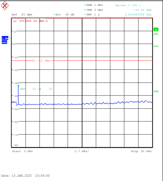
Band2-3MHz-16QAM-19185-15RB#0-3000~20000 -PASS
