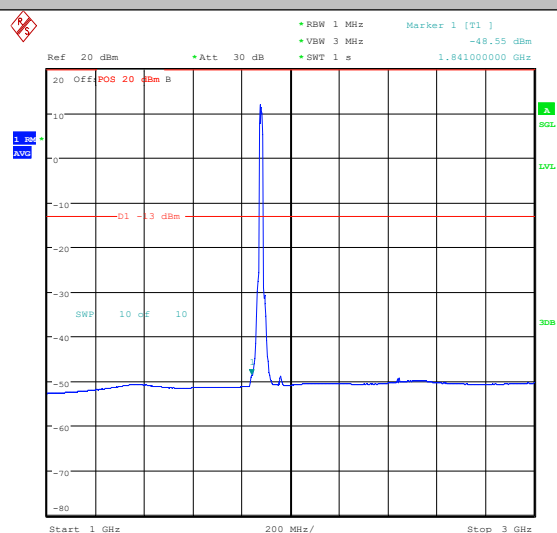
Band2-15MHz-QPSK-18900-75RB#0-0.15~30-PA SS
