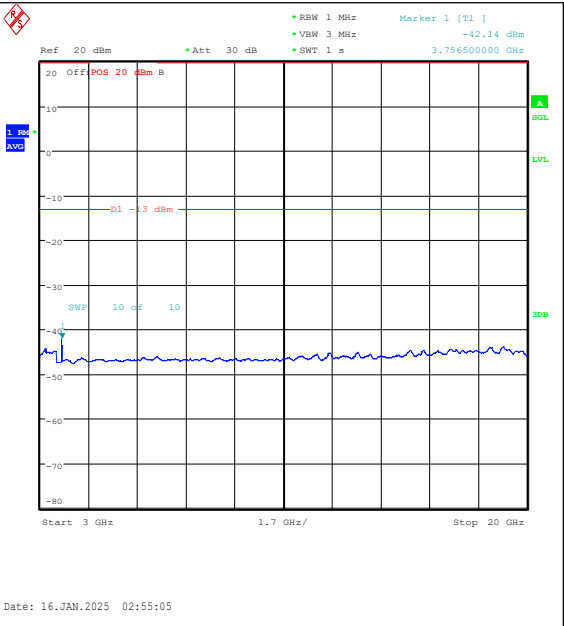
Band2-20MHz-16QAM-18900-100RB#0-3000~200 00-PASS
