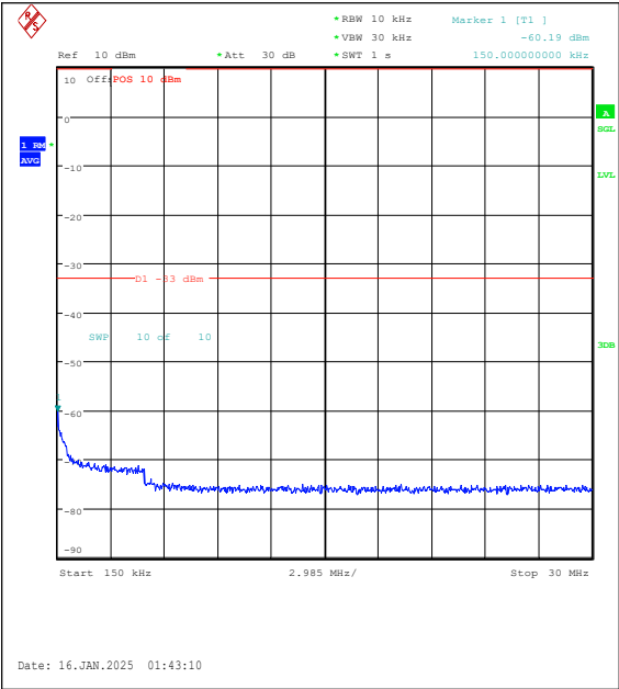
Band2-15MHz-16QAM-18675-1RB#0-0.15~30-PA SS
