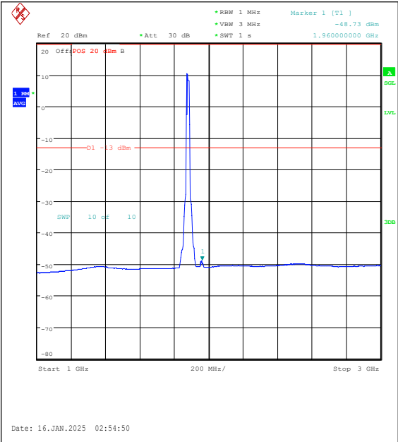
Band2-20MHz-16QAM-18900-100RB#0-1000~30 00-PASS
