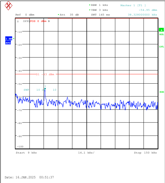
Band2-10MHz-16QAM-18900-1RB#49-0.009~0.1 5-PASS
