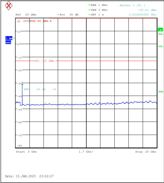
Band2-3MHz-16QAM-19185-1RB#14-3000~2000 0-PASS
