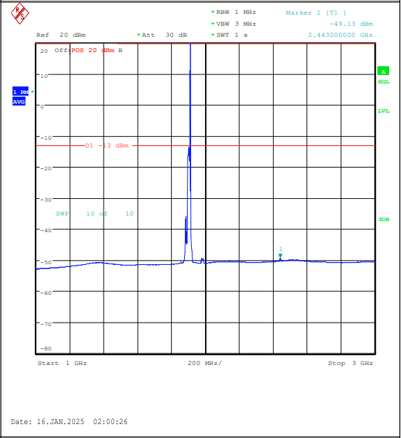
Band2-15MHz-16QAM-19125-1RB#74-1000~3000 -PASS
