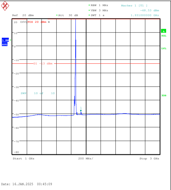
Band2-10MHz-16QAM-18650-1RB#49-1000~3000-PASS
