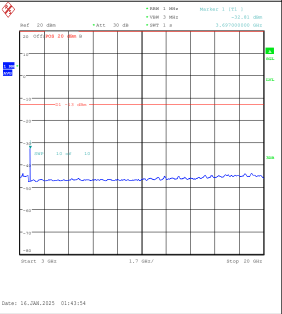
Band2-15MHz-16QAM-18675-1RB#0-3000~20000 -PASS
