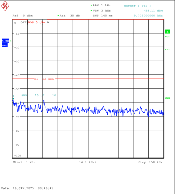
Band2-10MHz-16QAM-18650-50RB#0-0.009~0.15-PASS
