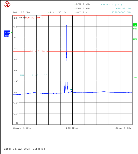
Band2-15MHz-16QAM-19125-1RB#0-1000~3000 -PASS
