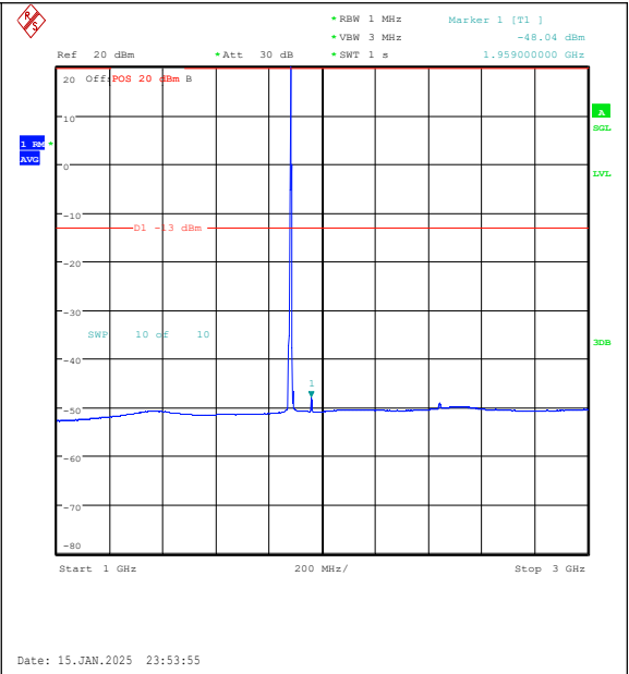
Band2-5MHz-16QAM-18900-1RB#24-1000~3000- PASS
