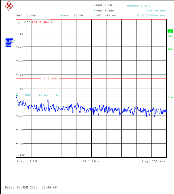
Band2-20MHz-16QAM-18700-1RB#99-0.009~0.1 5-PASS
