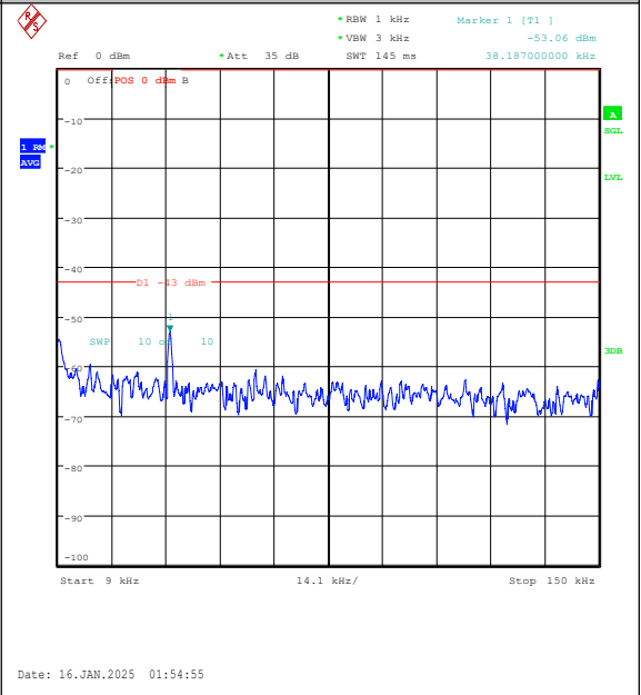
Band2-15MHz-16QAM-18900-75RB#0-0.009~0.15-PASS
