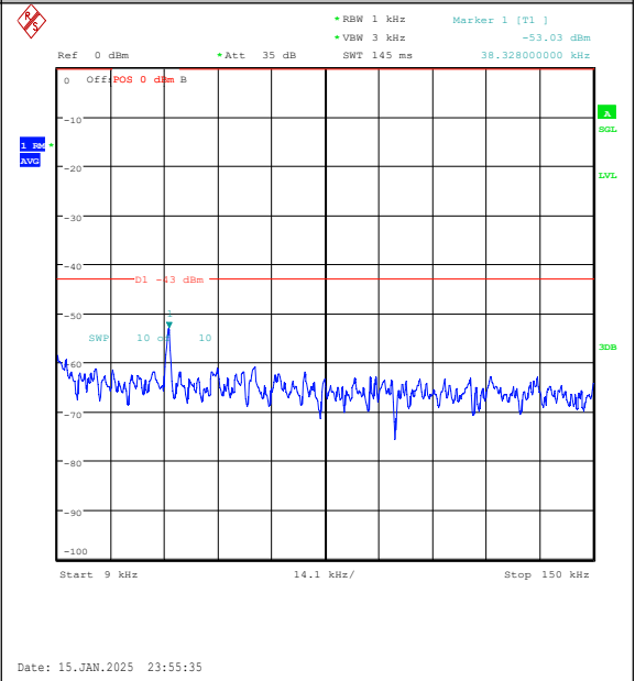
Band2-5MHz-16QAM-18900-25RB#0-0.009~0.15- PASS
