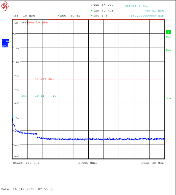
Band2-20MHz-QPSK-19100-1RB#0-0.15~30-PAS S
