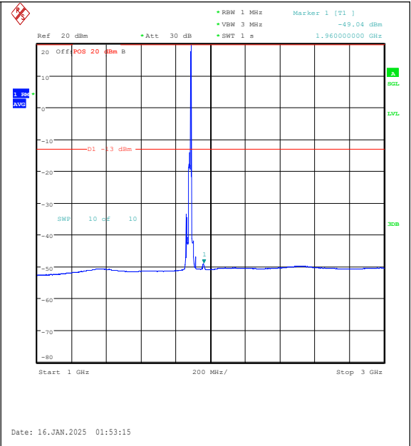
Band2-15MHz-16QAM-18900-1RB#74-1000~3000-PASS
