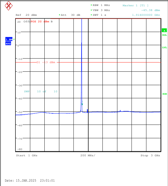
Band2-3MHz-QPSK-19185-1RB#14-1000~3000- PASS
