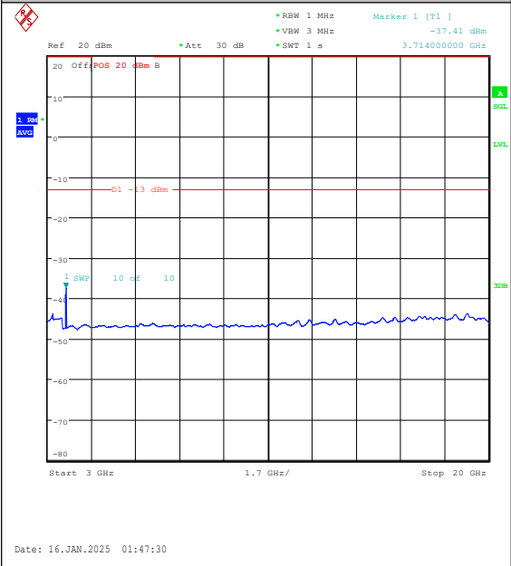
Band2-15MHz-QPSK-18675-75RB#0-3000~2000 0-PASS
