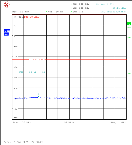
Band2-3MHz-QPSK-19185-1RB#0-30~1000-PAS S
