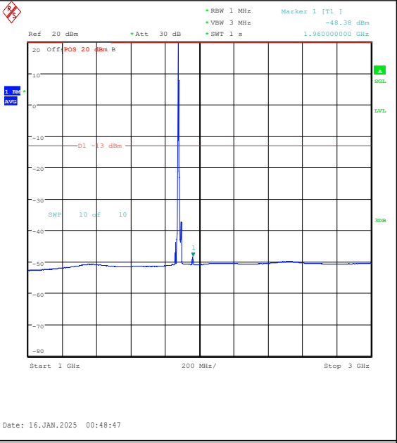
Band2-10MHz-QPSK-18900-1RB#0-1000~3000-P
