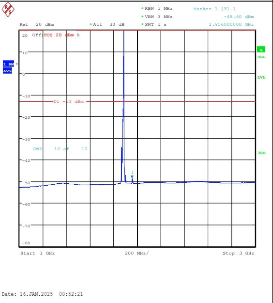
Band2-10MHz-16QAM-18900-1RB#49-1000~3000 -PASS
