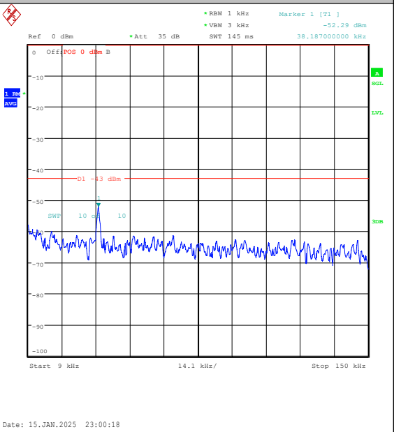
Band2-3MHz-QPSK-19185-1RB#14-0.009~0.15-P ASS
