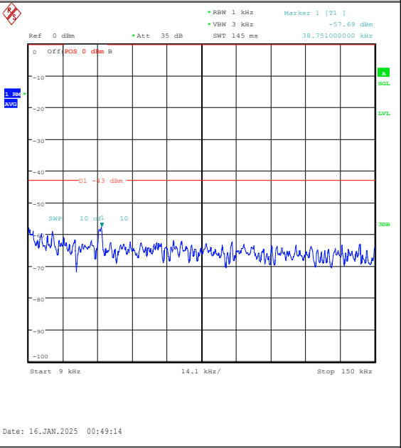
Band2-10MHz-16QAM-18900-1RB#0-0.009~0.15- PASS
