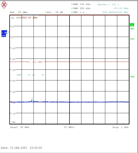
Band2-3MHz-16QAM-19185-15RB#0-30~1000-PA SS
