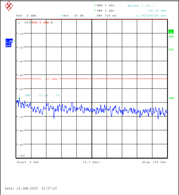
Band2-15MHz-16QAM-19125-1RB#0-0.009~0.15- PASS
