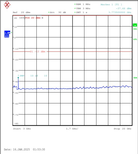
Band2-15MHz-16QAM-18900-1RB#74-3000~20000-PASS
