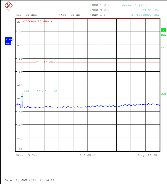
Band2-5MHz-16QAM-18900-1RB#24-3000~2000 0-PASS
