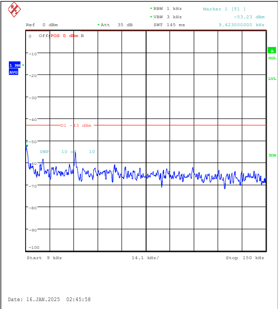
Band2-20MHz-QPSK-18700-100RB#0-0.009~0.1 5-PASS
