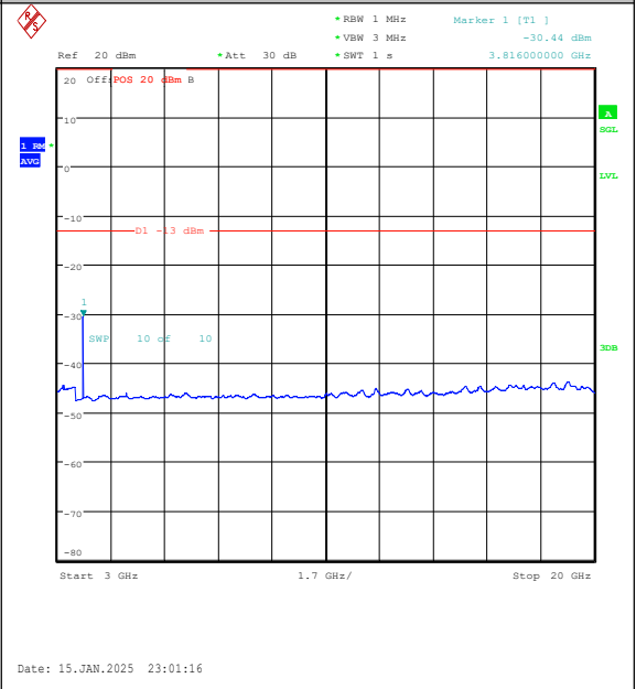
Band2-3MHz-QPSK-19185-1RB#14-3000~20000- PASS
