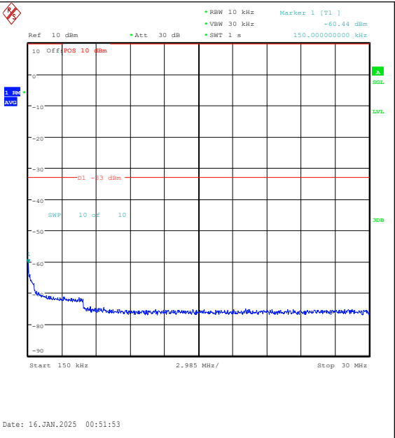
Band2-10MHz-16QAM-18900-1RB#49-0.15~30-P ASS
