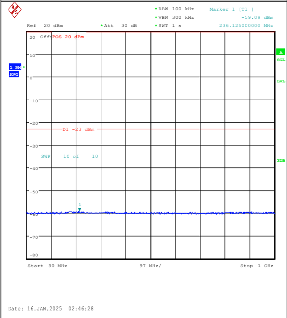
Band2-20MHz-QPSK-18700-100RB#0-30~1000- PASS
