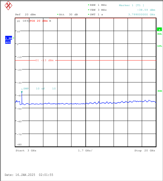
Band2-15MHz-QPSK-19125-75RB#0-3000~2000 0-PASS
