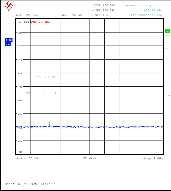
Band2-15MHz-QPSK-18675-1RB#0-30~1000-PA
