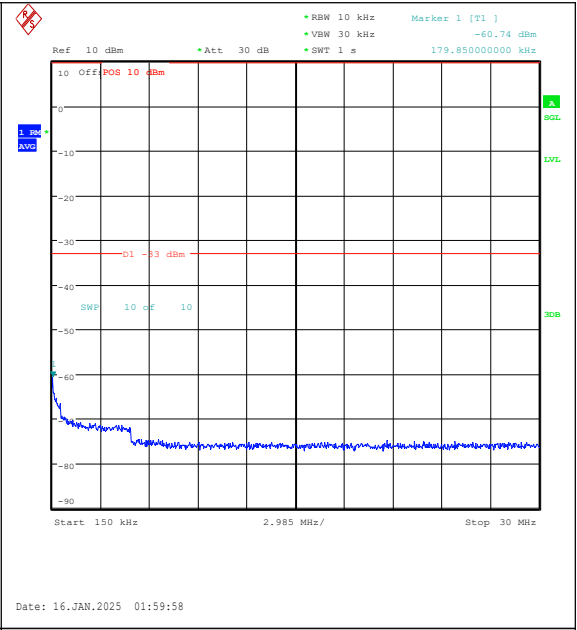
Band2-15MHz-16QAM-19125-1RB#74-0.15~30-P ASS
