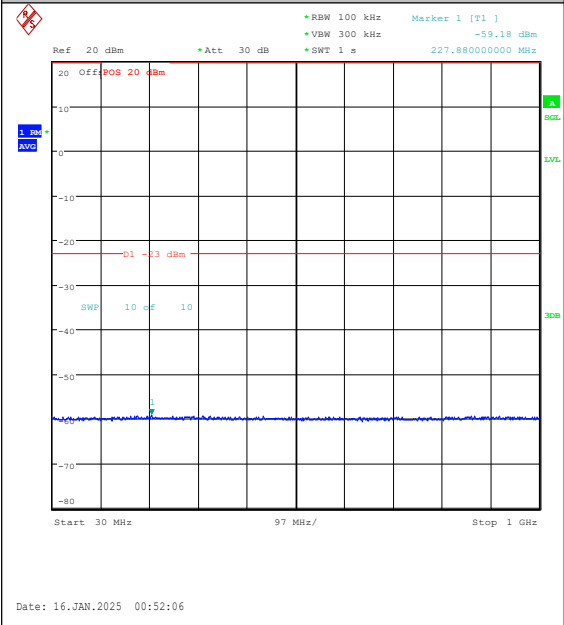
Band2-10MHz-16QAM-18900-1RB#49-30~1000- PASS
