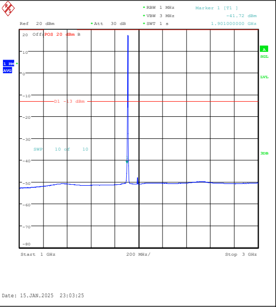
Band2-3MHz-QPSK-19185-15RB#0-1000~3000-P
