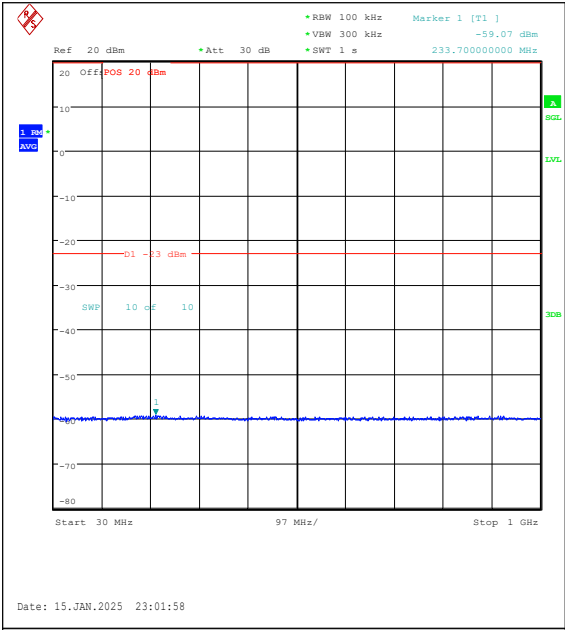
Band2-3MHz-16QAM-19185-1RB#14-30~1000-P ASS
