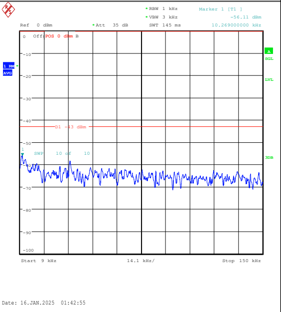
Band2-15MHz-16QAM-18675-1RB#0-0.009~0.15- PASS
