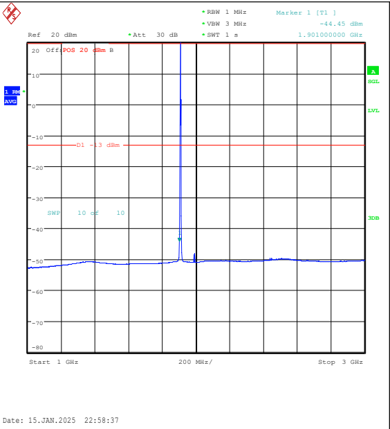
Band2-3MHz-QPSK-19185-1RB#0-1000~3000-PA SS
