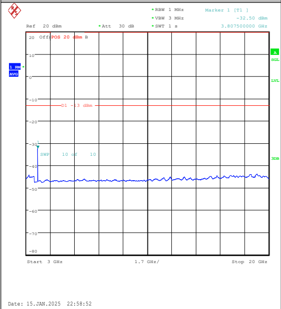
Band2-3MHz-QPSK-19185-1RB#0-3000~20000- PASS
