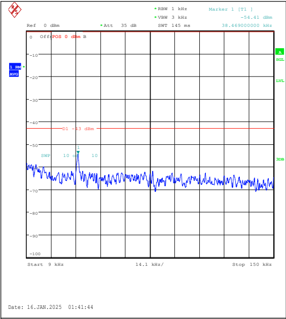
Band2-15MHz-QPSK-18675-1RB#0-0.009~0.15-PASS
