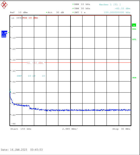
Band2-10MHz-QPSK-18650-50RB#0-0.15~30-PA SS
