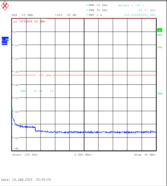
Band2-20MHz-16QAM-18700-1RB#99-0.15~30-P ASS
