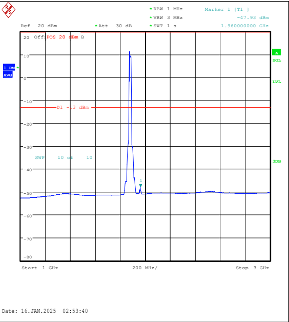
Band2-20MHz-QPSK-18900-100RB#0-1000~3000-PASS
