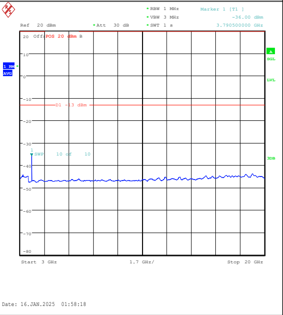
Band2-15MHz-16QAM-19125-1RB#0-3000~20000 -PASS
