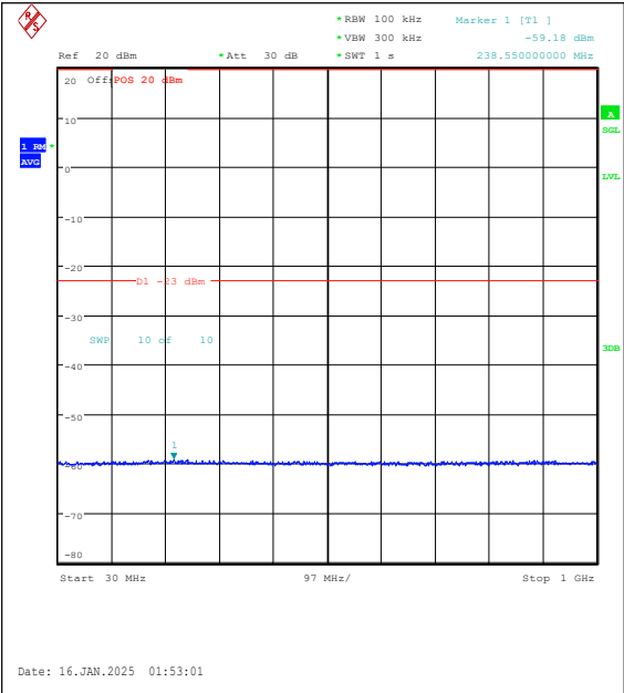
Band2-15MHz-16QAM-18900-1RB#74-30~1000-PASS
