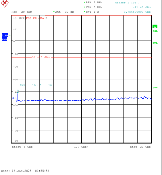
Band2-15MHz-16QAM-18900-75RB#0-3000~2000 0-PASS
