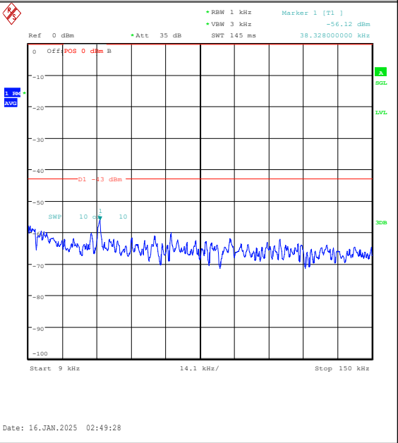
Band2-20MHz-16QAM-18900-1RB#0-0.009~0.15-PASS
