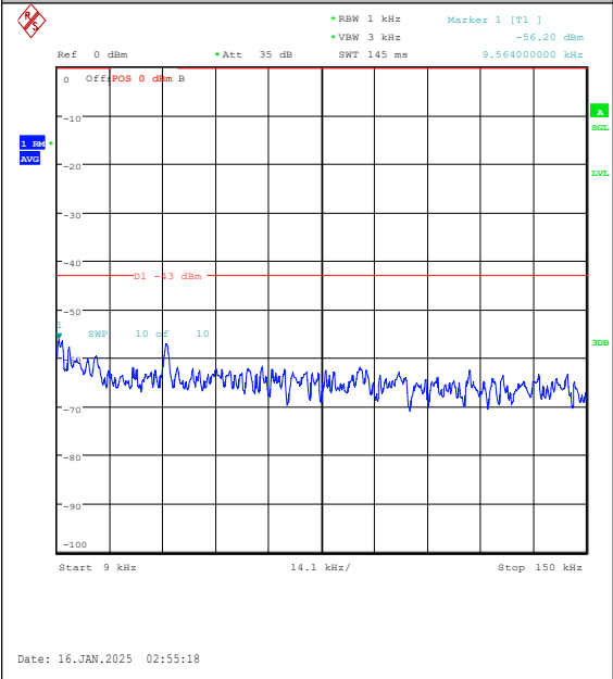
Band2-20MHz-QPSK-19100-1RB#0-0.009~0.15- PASS
