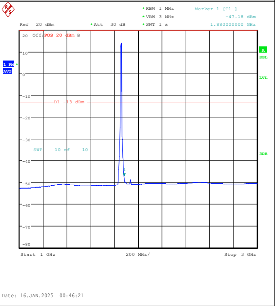
Band2-10MHz-QPSK-18650-50RB#0-1000~3000- PASS
