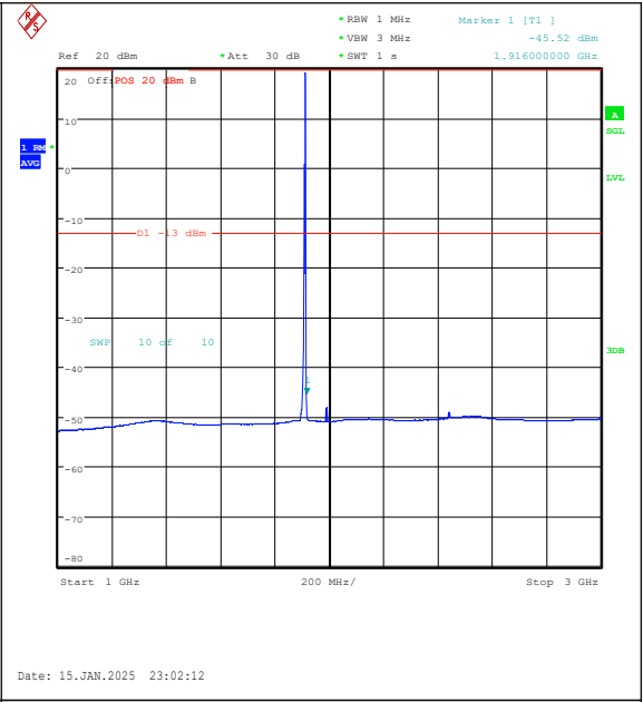
Band2-3MHz-16QAM-19185-1RB#14-1000~3000- PASS
