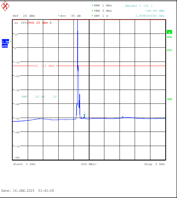
Band2-15MHz-QPSK-18675-1RB#0-1000~3000-P
