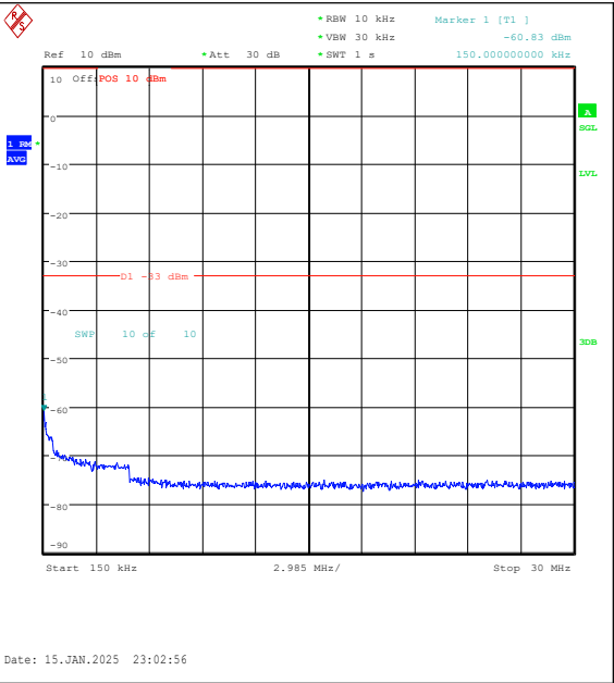
Band2-3MHz-QPSK-19185-15RB#0-0.15~30-PAS
