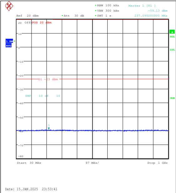
Band2-5MHz-16QAM-18900-1RB#24-30~1000-P ASS
