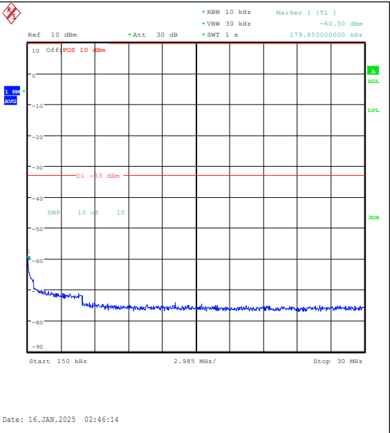
Band2-20MHz-QPSK-18700-100RB#0-0.15~30-PA SS
