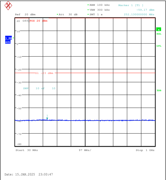
Band2-3MHz-QPSK-19185-1RB#14-30~1000-PAS S
