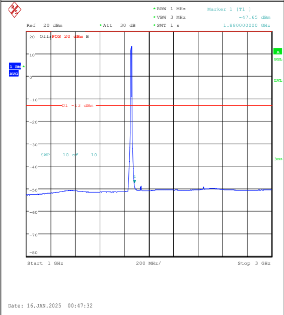
Band2-10MHz-16QAM-18650-50RB#0-1000~300 0-PASS
