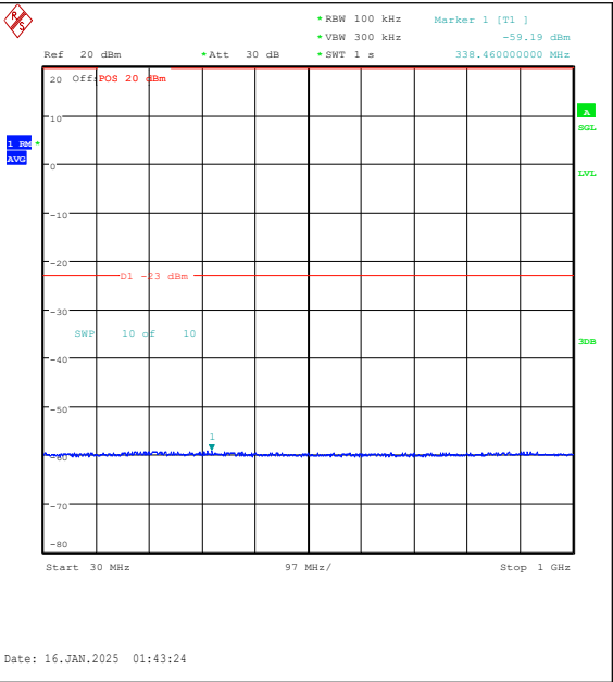
Band2-15MHz-16QAM-18675-1RB#0-30~1000-PA SS
