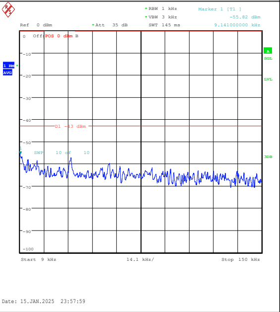
Band2-5MHz-16QAM-19175-1RB#0-0.009~0.15-P ASS
