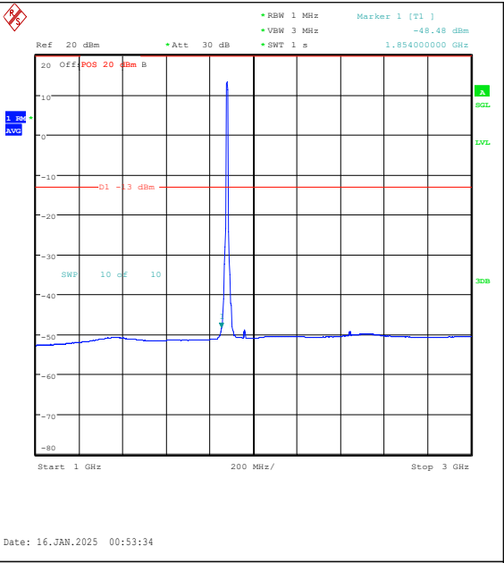
Band2-10MHz-QPSK-18900-50RB#0-1000~3000- PASS
