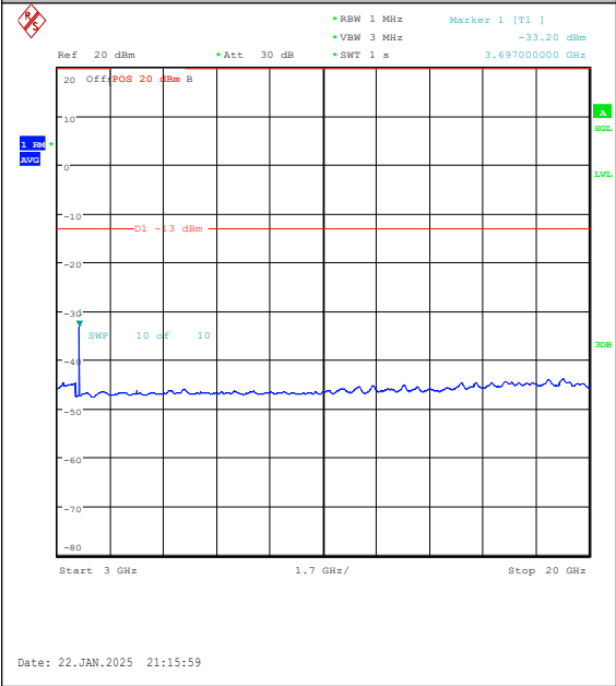
Band25-1.4MHz-QPSK-26047-6RB#0-3000~2000 0-PASS
