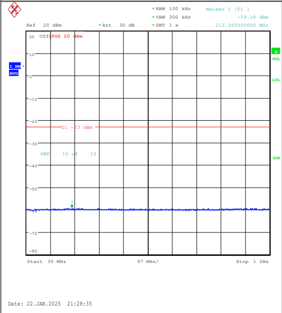
Band25-1.4MHz-16QAM-26683-1RB#5-30~1000- PASS
