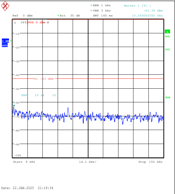
Band25-1.4MHz-16QAM-26365-1RB#0-0.009~0.1 5-PASS
