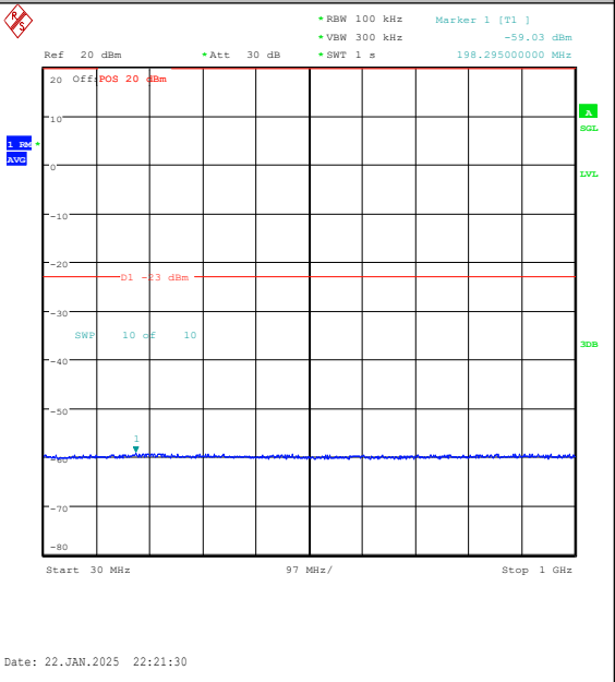
Band25-3MHz-16QAM-26365-15RB#0-30~1000-P ASS
