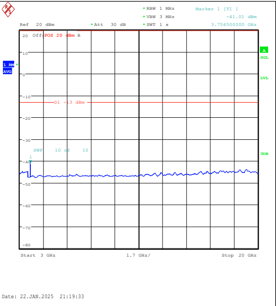
Band25-1.4MHz-16QAM-26365-1RB#0-3000~200 00-PASS
