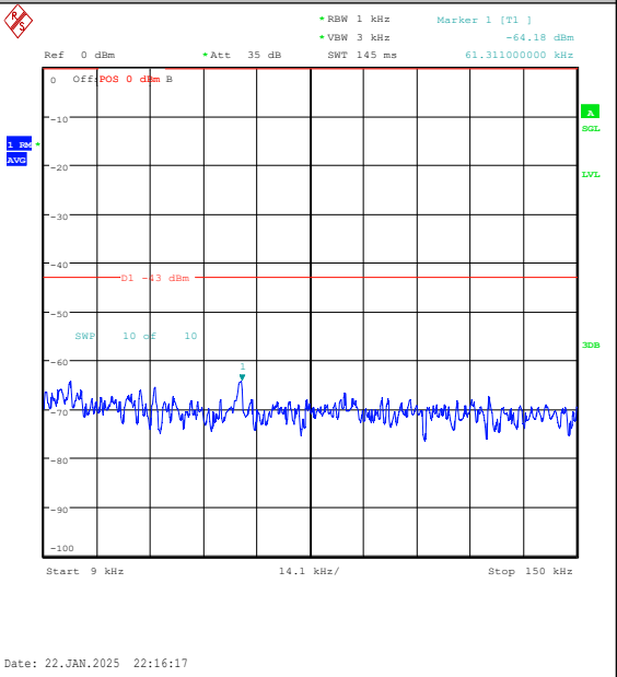
Band25-3MHz-16QAM-26365-1RB#0-0.009~0.15- PASS
