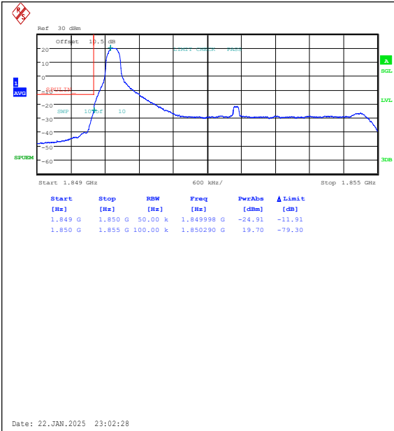
Band25-5MHz-QPSK-26065-1RB#0-PASS
