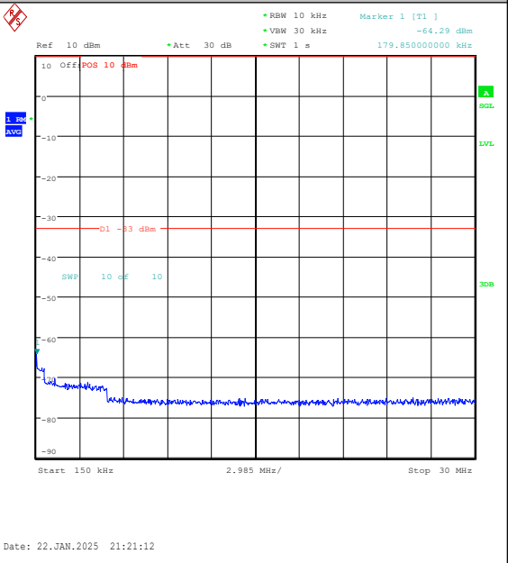
Band25-1.4MHz-16QAM-26365-1RB#5-0.15~30-P ASS
