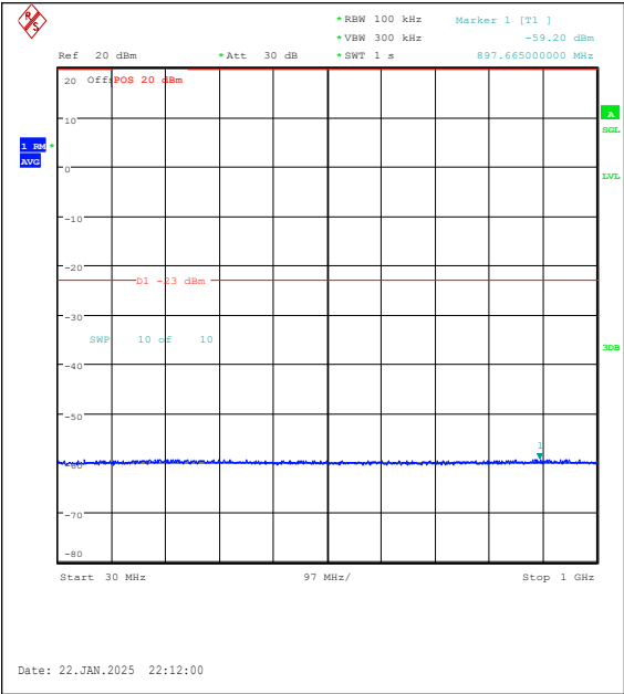
Band25-3MHz-16QAM-26055-1RB#14-30~1000-PASS
