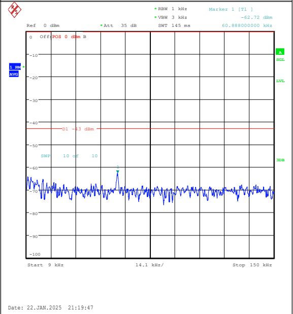
Band25-1.4MHz-QPSK-26365-1RB#5-0.009~0.15- PASS
