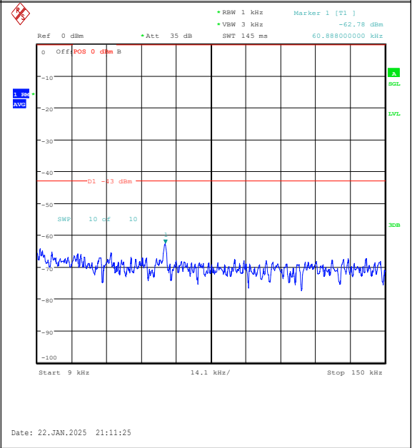
Band25-1.4MHz-16QAM-26047-1RB#0-0.009~0.1 5-PASS
