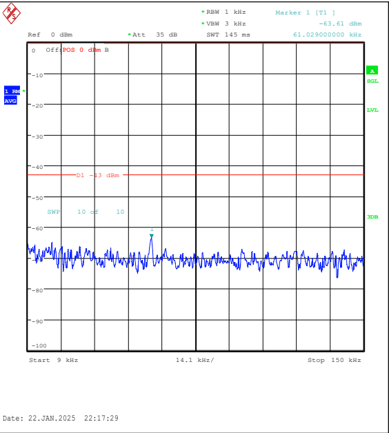
Band25-3MHz-QPSK-26365-1RB#14-0.009~0.15- PASS
