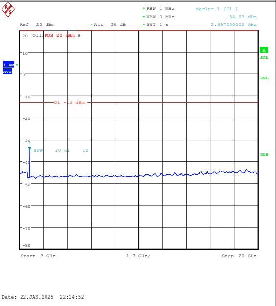
Band25-3MHz-16QAM-26055-15RB#0-3000~2000 0-PASS
