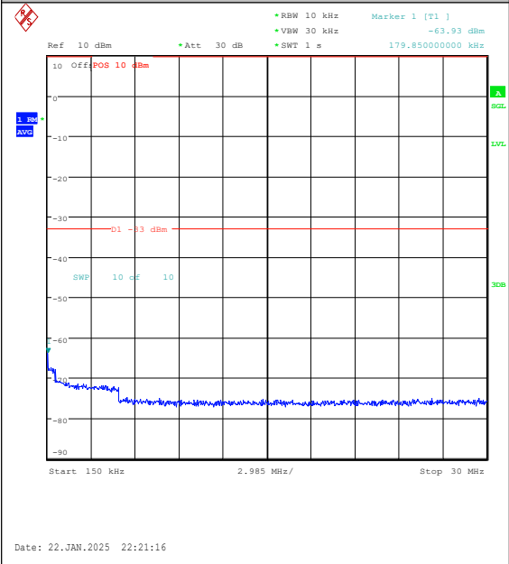
Band25-3MHz-16QAM-26365-15RB#0-0.15~30-P ASS
