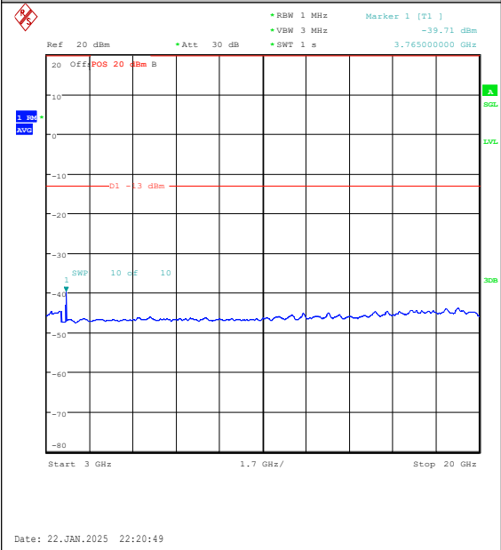
Band25-3MHz-QPSK-26365-15RB#0-3000~2000 0-PASS
