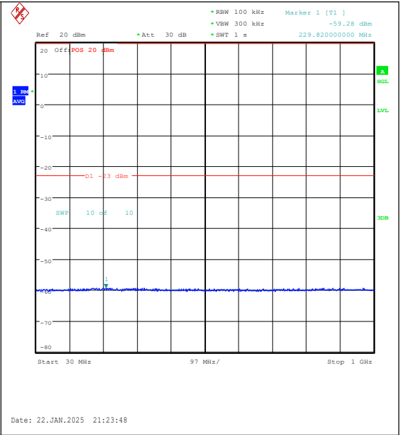
Band25-1.4MHz-16QAM-26365-6RB#0-30~1000-P ASS
