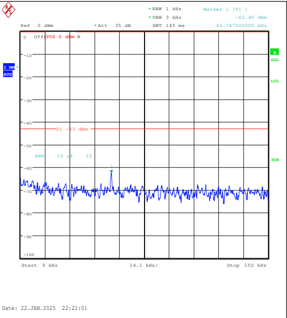
Band25-3MHz-16QAM-26365-15RB#0-0.009~0.15 -PASS
