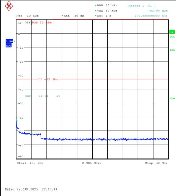
Band25-3MHz-QPSK-26365-1RB#14-0.15~30-PA SS
