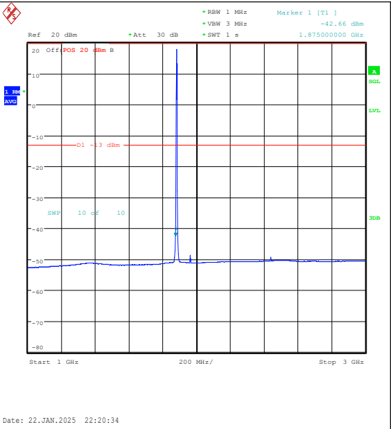
Band25-3MHz-QPSK-26365-15RB#0-1000~3000- PASS
