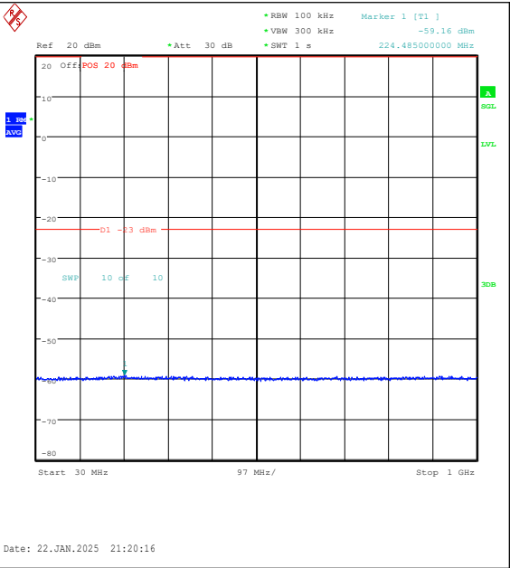
Band25-1.4MHz-QPSK-26365-1RB#5-30~1000-PA SS
