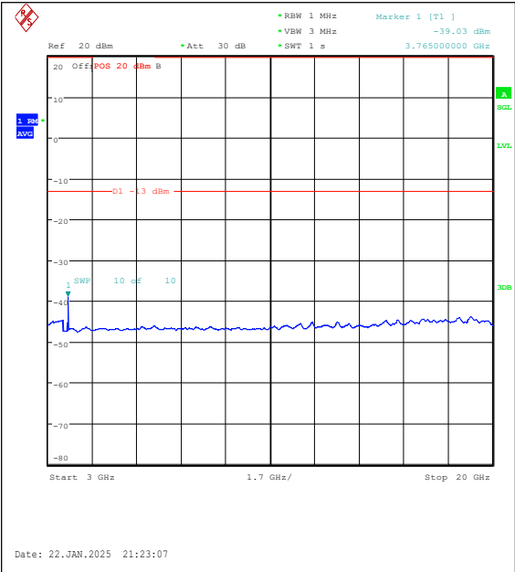
Band25-1.4MHz-QPSK-26365-6RB#0-3000~2000 0-PASS
