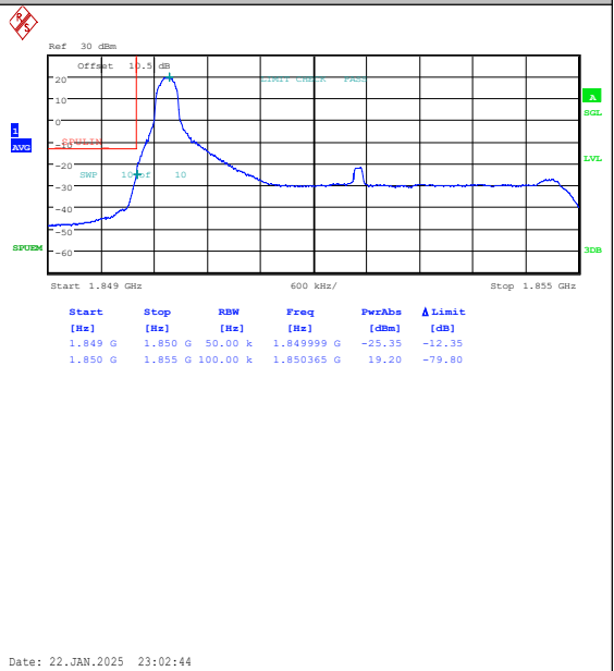
Band25-5MHz-16QAM-26065-1RB#0-PASS
