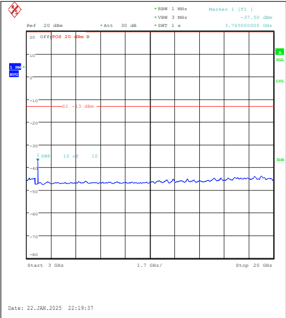
Band25-3MHz-16QAM-26365-1RB#14-3000~200 00-PASS
