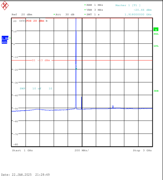
Band25-1.4MHz-16QAM-26683-1RB#5-1000~300 0-PASS
