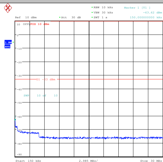
Band25-3MHz-QPSK-26055-15RB#0-3000~2000 0-PASS
