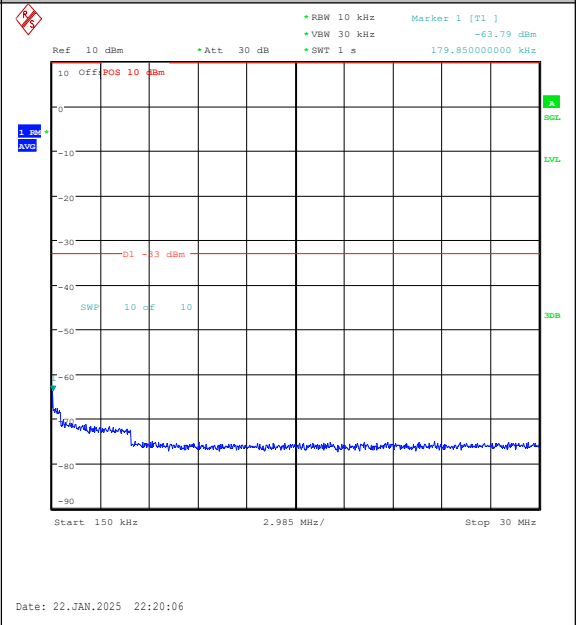
Band25-3MHz-QPSK-26365-15RB#0-0.15~30-PA SS
