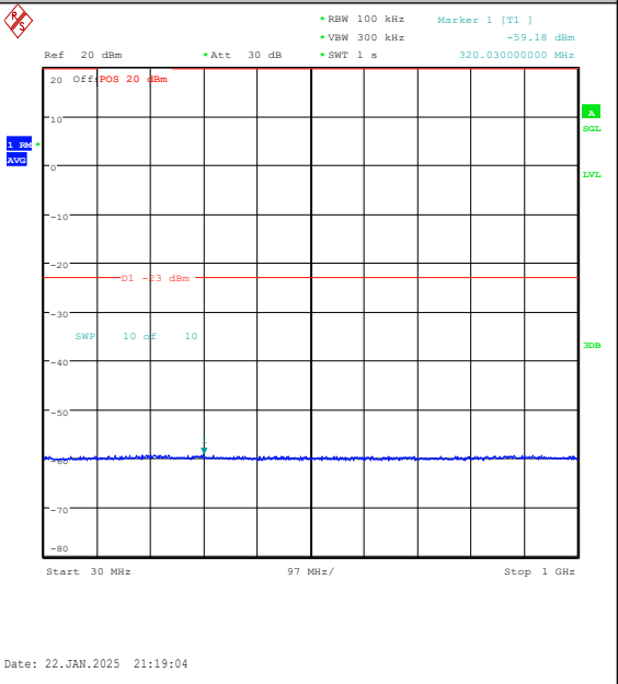
Band25-1.4MHz-16QAM-26365-1RB#0-30~1000-PASS
