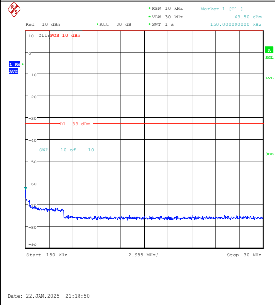
Band25-1.4MHz-16QAM-26365-1RB#0-0.15~30-PASS
