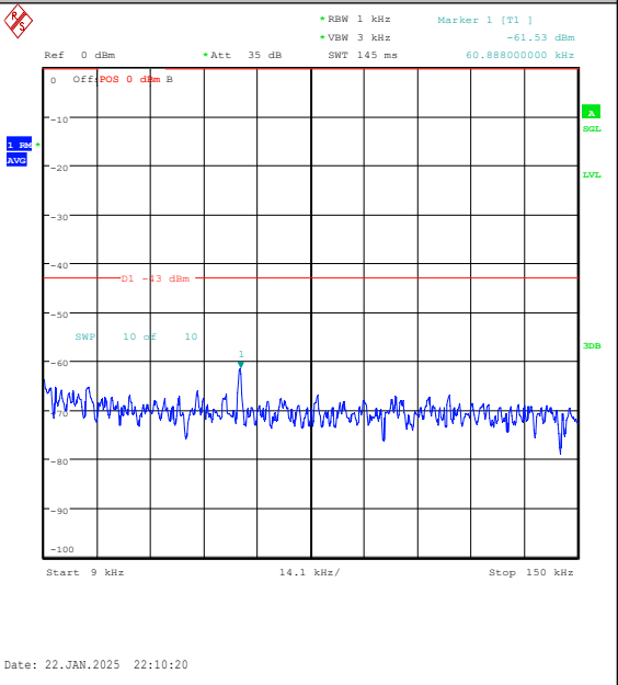
Band25-3MHz-QPSK-26055-1RB#14-0.009~0.15- PASS
