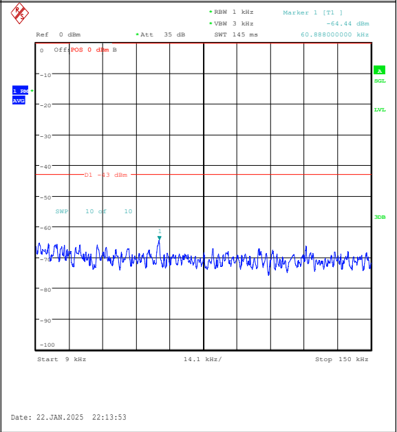
Band25-3MHz-16QAM-26055-15RB#0-0.009~0.15-PASS
