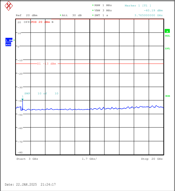
Band25-1.4MHz-16QAM-26365-6RB#0-3000~20000-PASS
