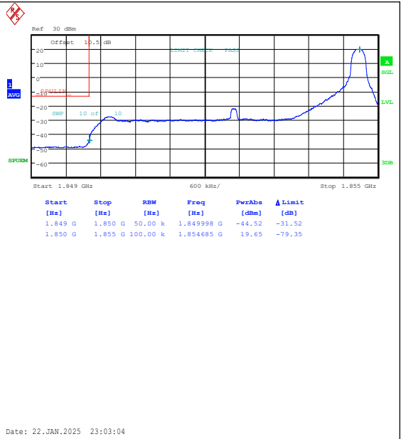
Band25-5MHz-QPSK-26065-1RB#24-PASS
