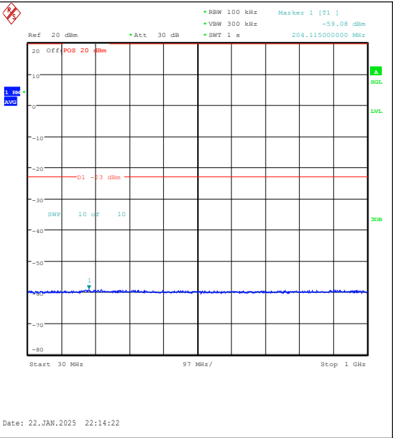
Band25-3MHz-16QAM-26055-15RB#0-30~1000-P ASS
