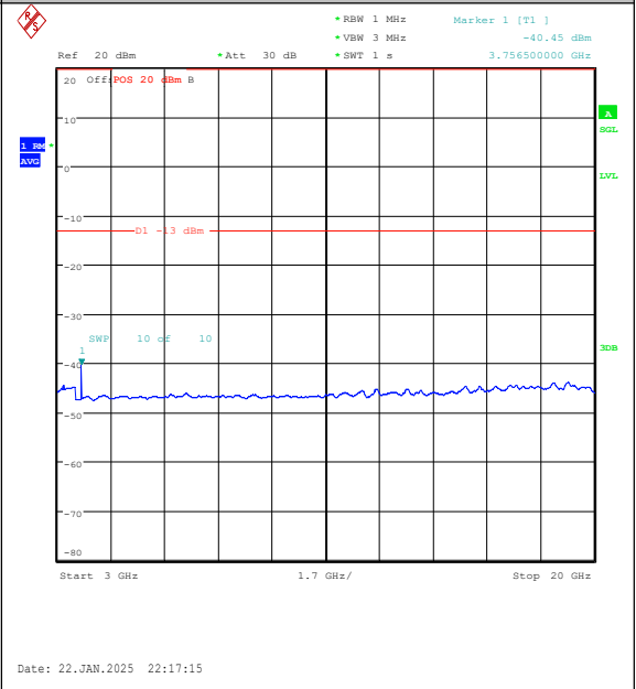
Band25-3MHz-16QAM-26365-1RB#0-3000~20000 -PASS
