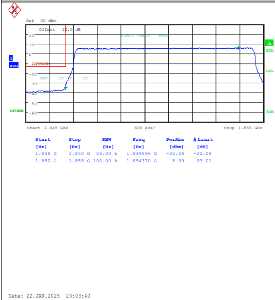
Band25-5MHz-QPSK-26065-25RB#0-PASS
