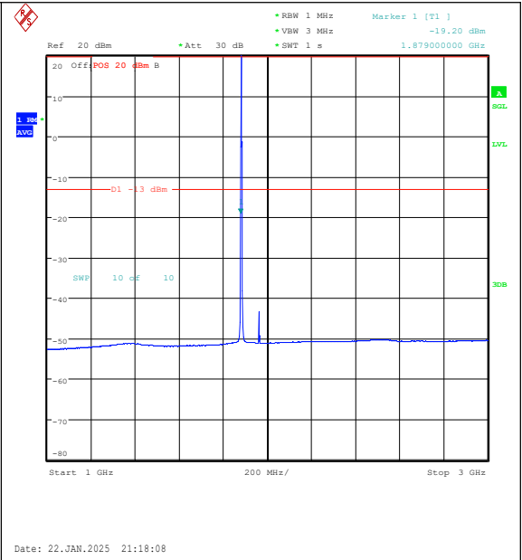
Band25-1.4MHz-QPSK-26365-1RB#0-1000~3000- PASS
