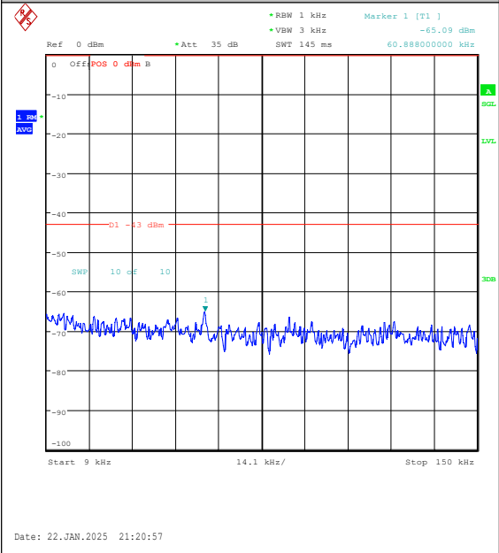
Band25-1.4MHz-16QAM-26365-1RB#5-0.009~0. 15-PASS
