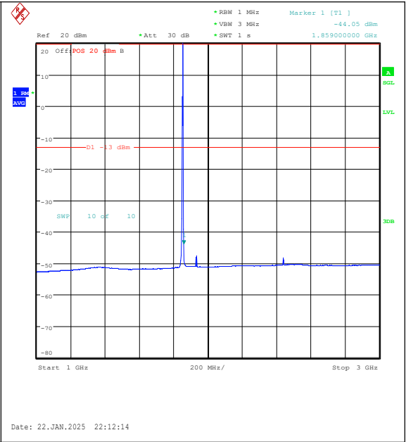
Band25-3MHz-16QAM-26055-1RB#14-1000~3000-PASS
