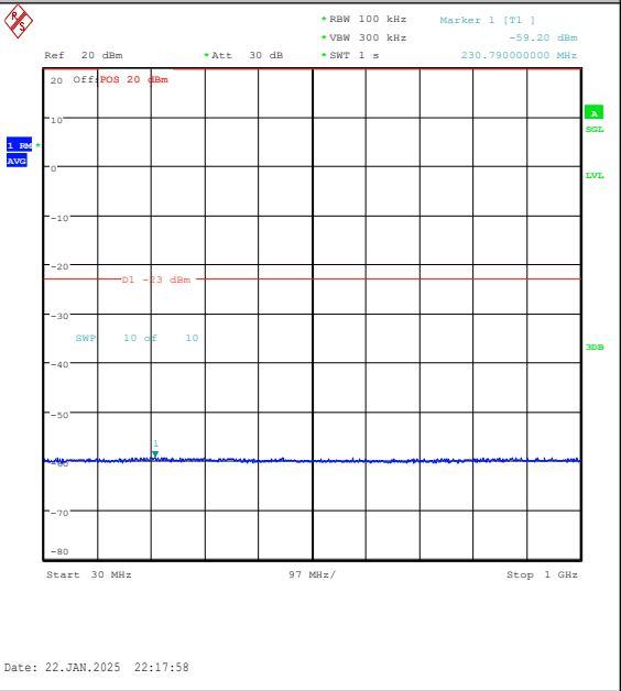
Band25-3MHz-QPSK-26365-1RB#14-30~1000-PA SS
