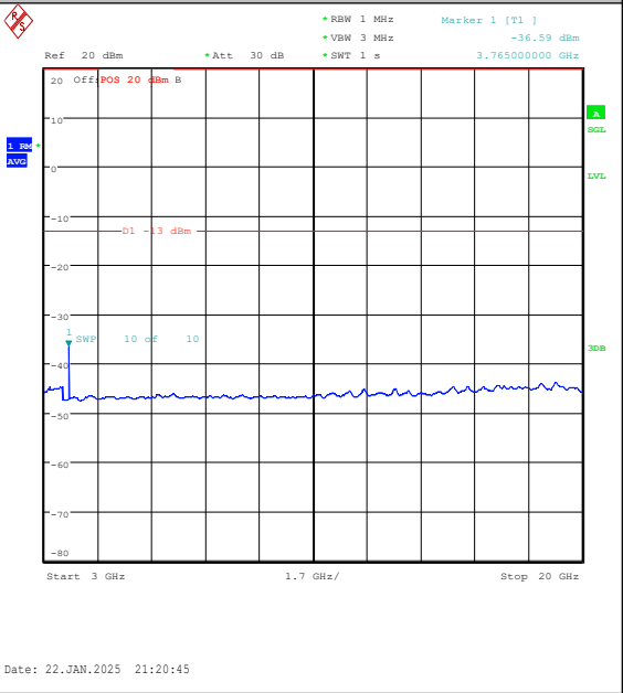
Band25-1.4MHz-QPSK-26365-1RB#5-3000~2000 0-PASS
