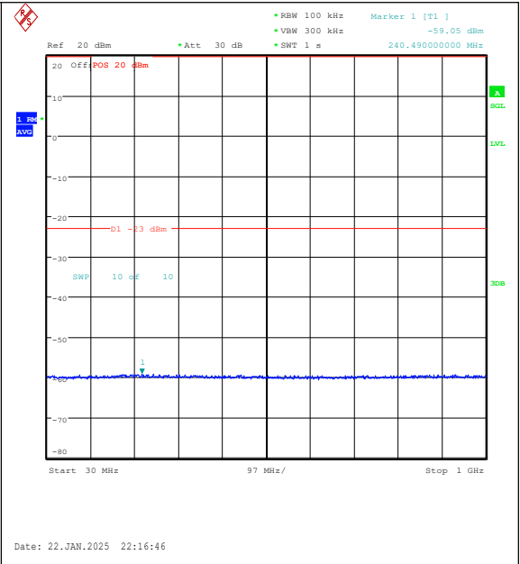
Band25-3MHz-16QAM-26365-1RB#0-30~1000-PA SS
