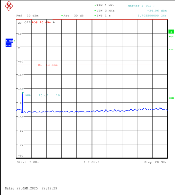
Band25-3MHz-16QAM-26055-1RB#14-3000~20000-PASS
