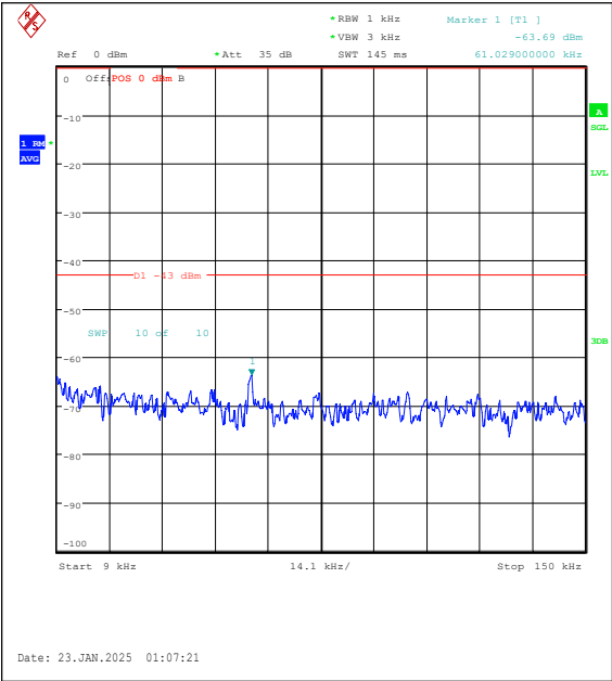
Band25-15MHz-16QAM-26115-1RB#74-0.009~0.15-PASS
