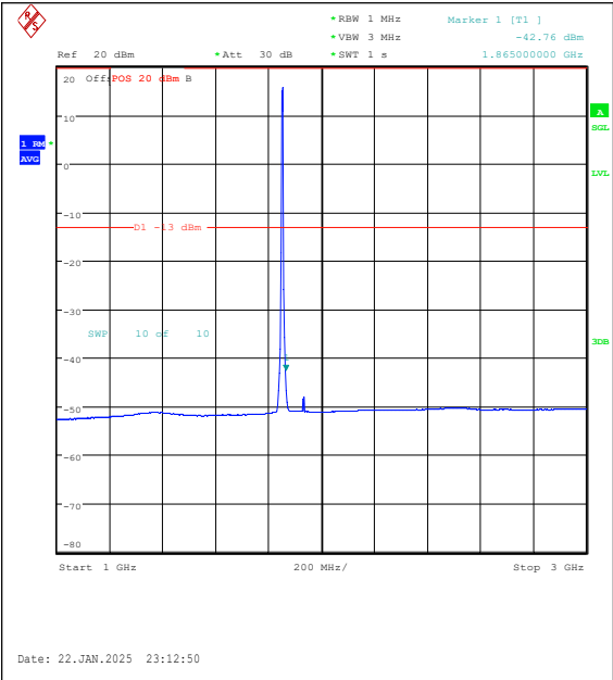
Band25-5MHz-16QAM-26065-25RB#0-1000~300 0-PASS
