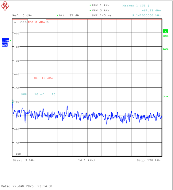
Band25-5MHz-16QAM-26365-1RB#0-0.009~0.15- PASS
