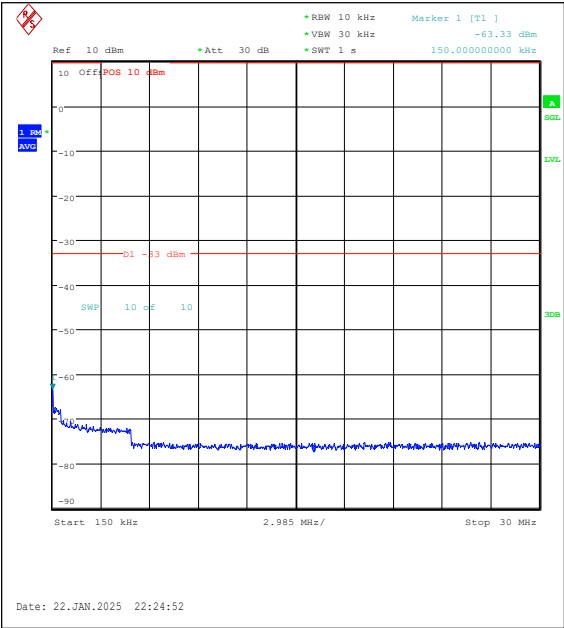
Band25-3MHz-QPSK-26675-1RB#14-0.15~30-PA SS
