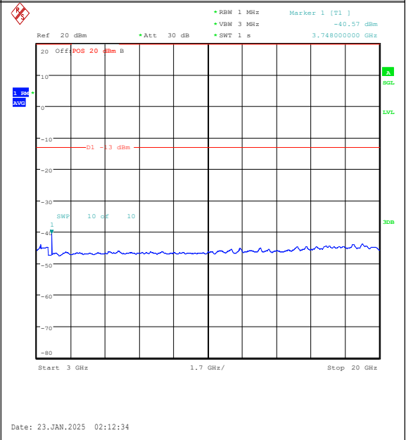
Band25-20MHz-16QAM-26365-1RB#0-3000~2000 0-PASS
