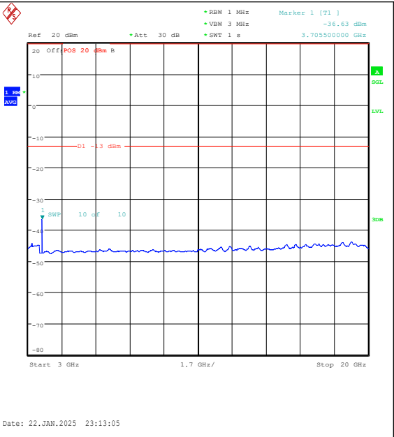
Band25-5MHz-16QAM-26065-25RB#0-3000~2000 0-PASS
