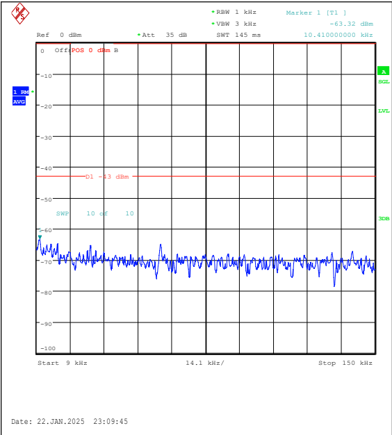
Band25-5MHz-16QAM-26065-1RB#24-0.009~0.1 5-PASS
