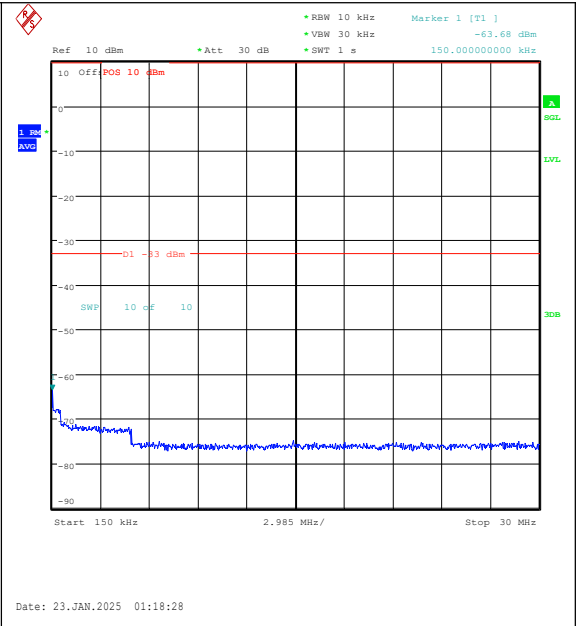
Band25-15MHz-QPSK-26615-1RB#0-0.15~30-PA SS
