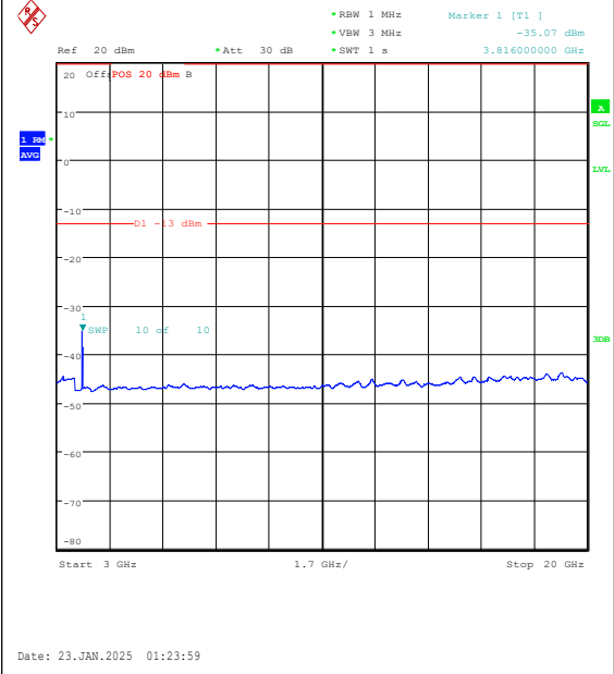
Band25-15MHz-QPSK-26615-75RB#0-3000~20000-PASS
