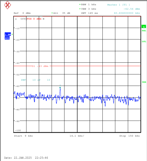
Band25-3MHz-16QAM-26675-1RB#14-0.009~0.1 5-PASS
