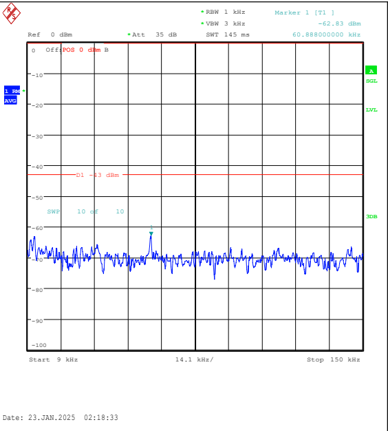
Band25-20MHz-16QAM-26590-1RB#0-0.009~0.15-PASS
