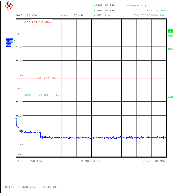
Band25-10MHz-QPSK-26090-1RB#49-0.15~30-P ASS
