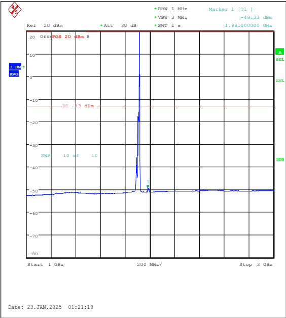
Band25-15MHz-QPSK-26615-1RB#74-1000~300 0-PASS
