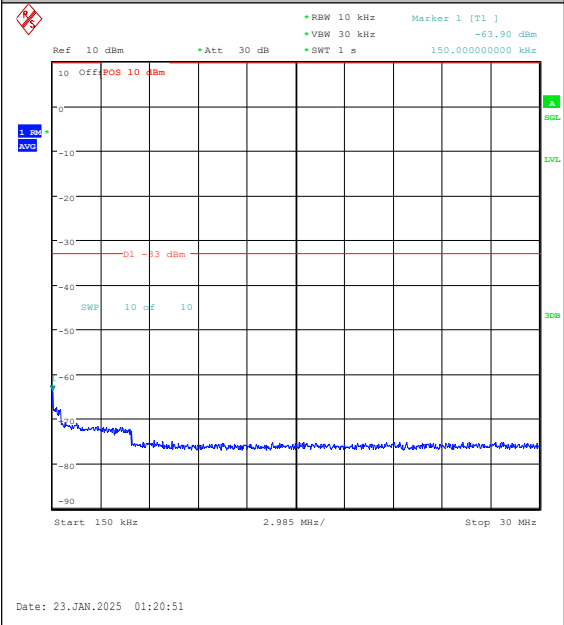
Band25-15MHz-QPSK-26615-1RB#74-0.15~30-P ASS
