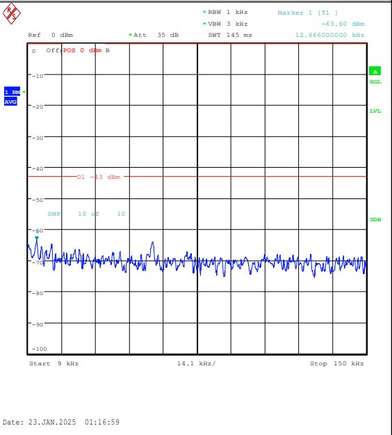
Band25-15MHz-16QAM-26365-75RB#0-0.009~0.1 5-PASS
