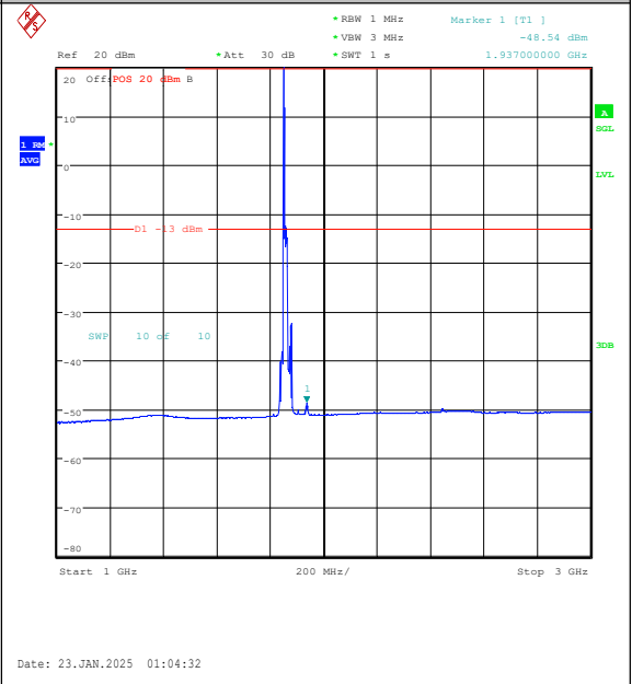
Band25-15MHz-QPSK-26115-1RB#0-1000~3000-PASS
