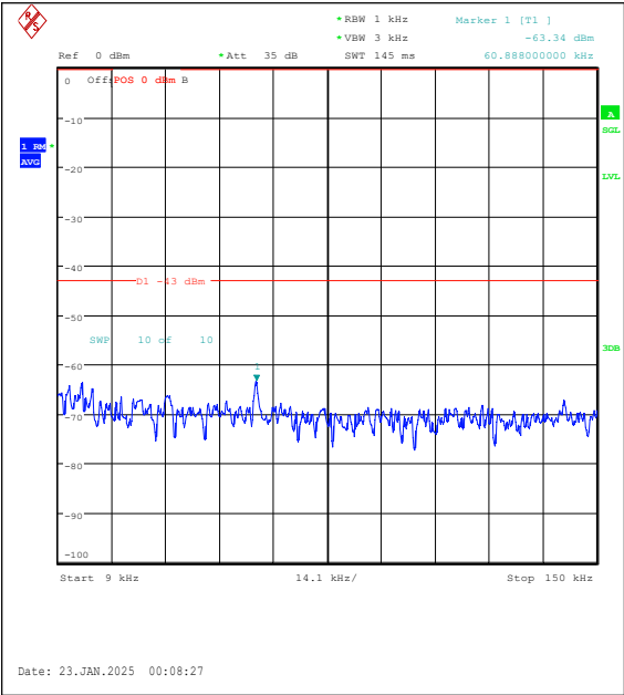
Band25-10MHz-QPSK-26090-50RB#0-0.009~0.1 5-PASS
