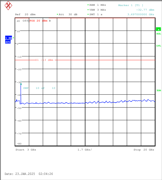
Band25-20MHz-QPSK-26140-1RB#0-3000~2000 0-PASS
