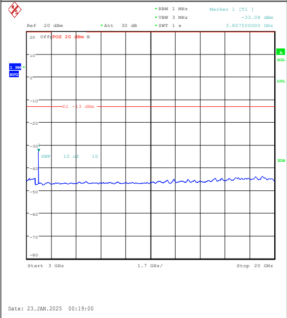
Band25-10MHz-QPSK-26640-1RB#0-3000~2000 0-PASS
