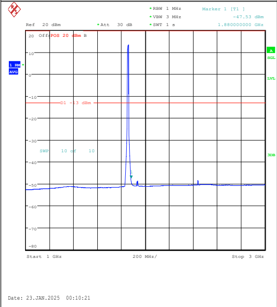
Band25-10MHz-16QAM-26090-50RB#0-1000~3000-PASS
