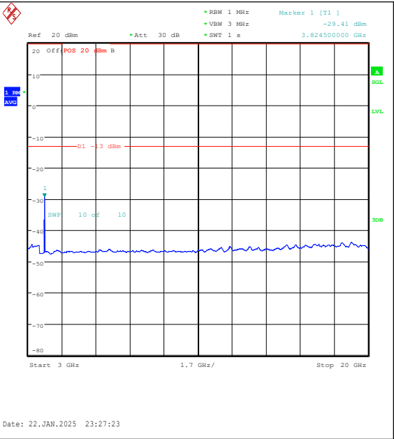
Band25-5MHz-16QAM-26665-25RB#0-3000~2000 0-PASS
