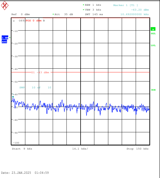
Band25-15MHz-16QAM-26115-1RB#0-0.009~0.15 -PASS
