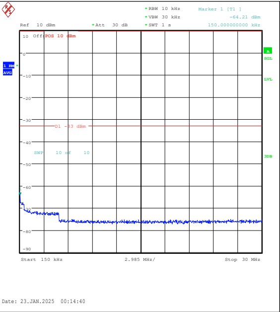
Band25-10MHz-16QAM-26365-1RB#49-0.15~30-P ASS
