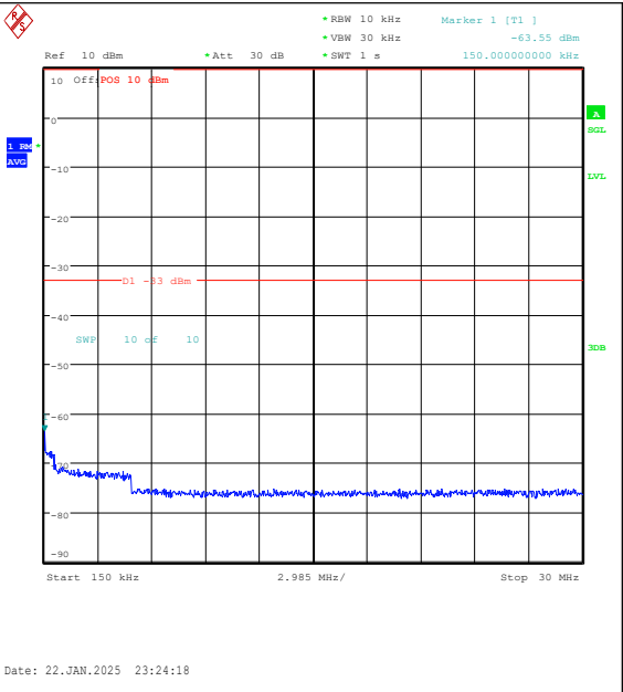
Band25-5MHz-16QAM-26665-1RB#24-0.15~30-P ASS
