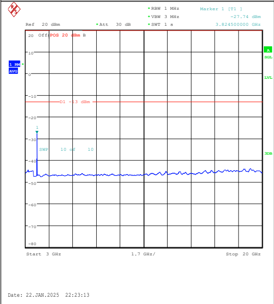
Band25-3MHz-QPSK-26675-1RB#0-3000~20000 -PASS
