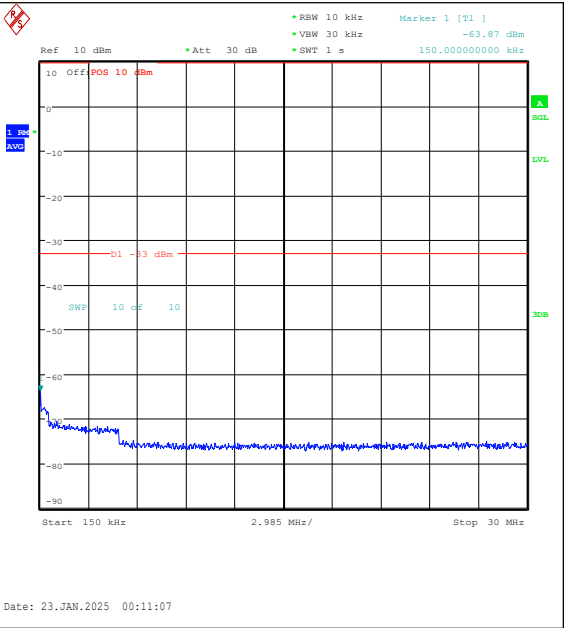
Band25-10MHz-QPSK-26365-1RB#0-0.15~30-PA SS
