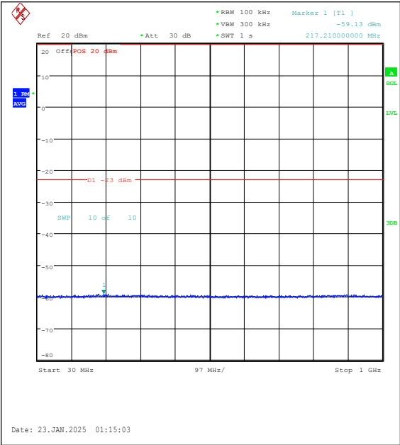
Band25-15MHz-16QAM-26365-1RB#74-30~1000 -PASS
