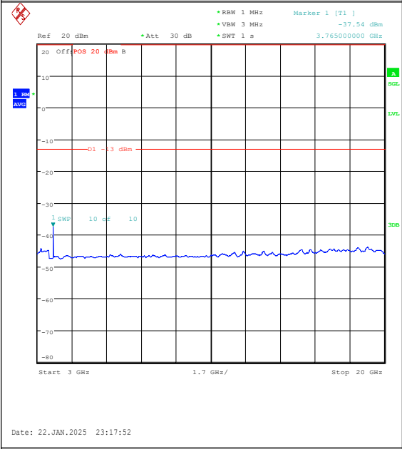
Band25-5MHz-16QAM-26365-1RB#24-3000~20000-PASS
