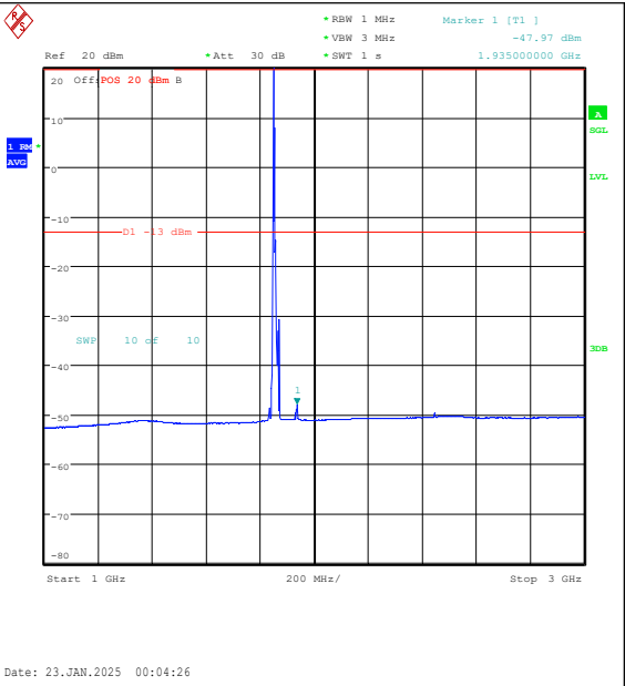
Band25-10MHz-QPSK-26090-1RB#0-1000~3000- PASS
