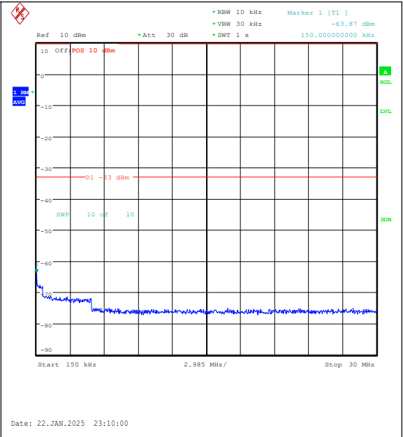
Band25-5MHz-16QAM-26065-1RB#24-0.15~30-P ASS
