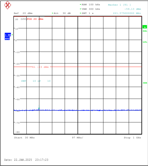
Band25-5MHz-16QAM-26365-1RB#24-30~1000-PASS
