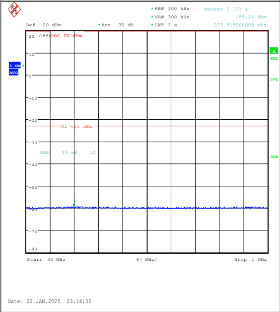
Band25-5MHz-QPSK-26365-25RB#0-30~1000-P ASS
