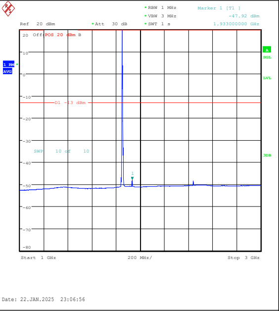
Band25-5MHz-QPSK-26065-1RB#0-1000~3000-P
