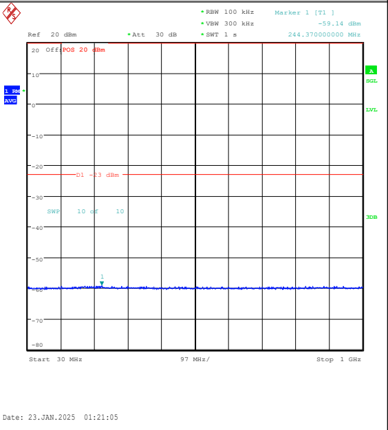
Band25-15MHz-QPSK-26615-1RB#74-30~1000-P ASS
