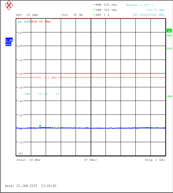
Band25-5MHz-QPSK-26065-1RB#0-30~1000-PA
