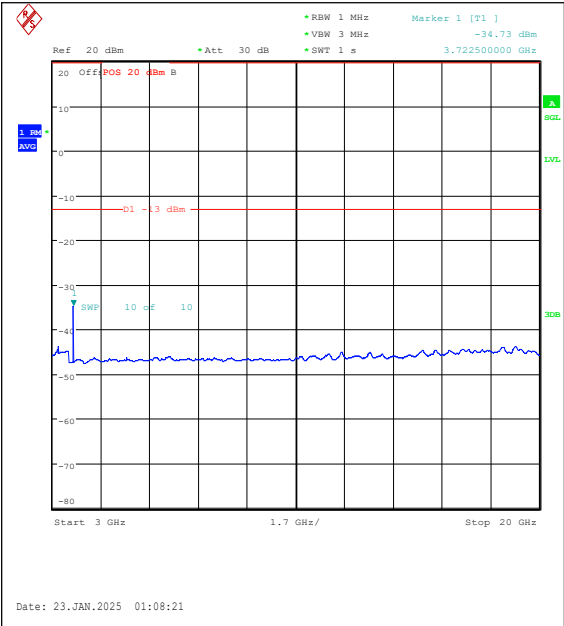
Band25-15MHz-16QAM-26115-1RB#74-3000~20000-PASS
