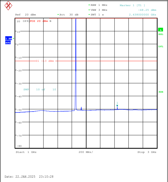
Band25-5MHz-16QAM-26065-1RB#24-1000~3000 -PASS
