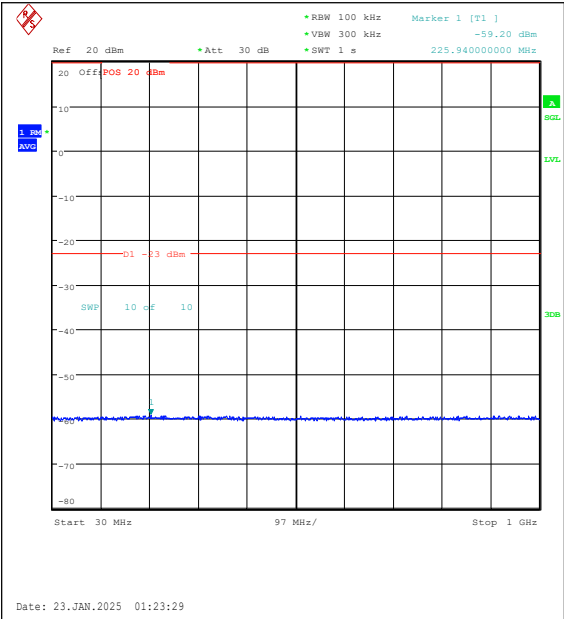
Band25-15MHz-QPSK-26615-75RB#0-30~1000-PASS
