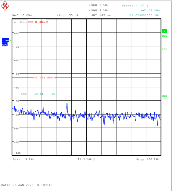
Band25-15MHz-16QAM-26115-75RB#0-0.009~0.15-PASS
