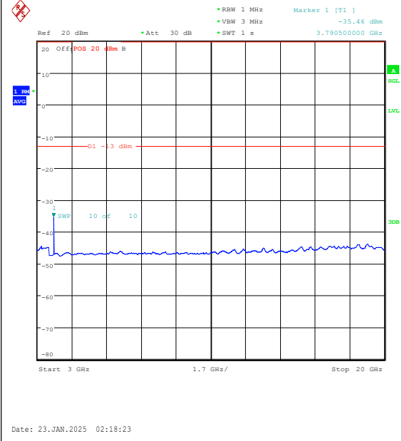
Band25-20MHz-QPSK-26590-1RB#0-3000~2000 0-PASS
