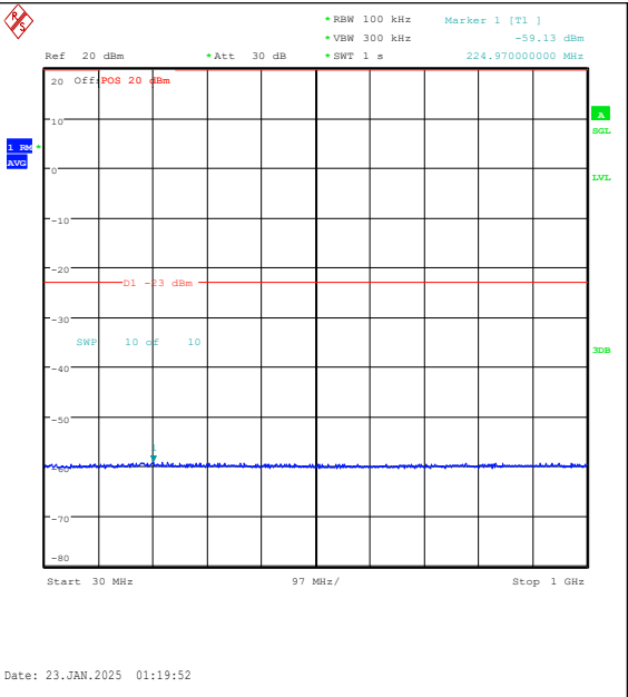
Band25-15MHz-16QAM-26615-1RB#0-30~1000-P ASS
