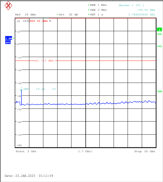
Band25-15MHz-QPSK-26365-1RB#0-3000~2000 0-PASS
