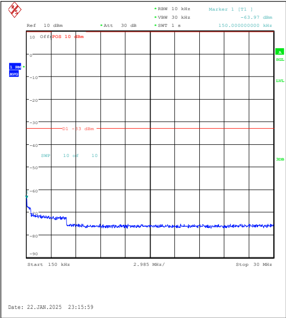
Band25-5MHz-QPSK-26365-1RB#24-0.15~30-PA SS
