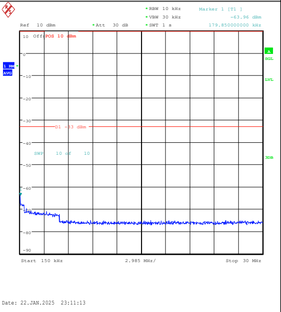
Band25-5MHz-QPSK-26065-25RB#0-0.15~30-PA SS
