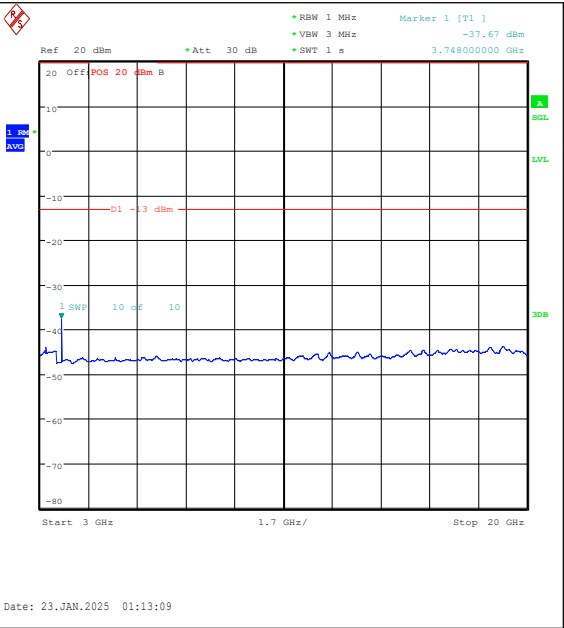
Band25-15MHz-16QAM-26365-1RB#0-3000~2000 0-PASS
