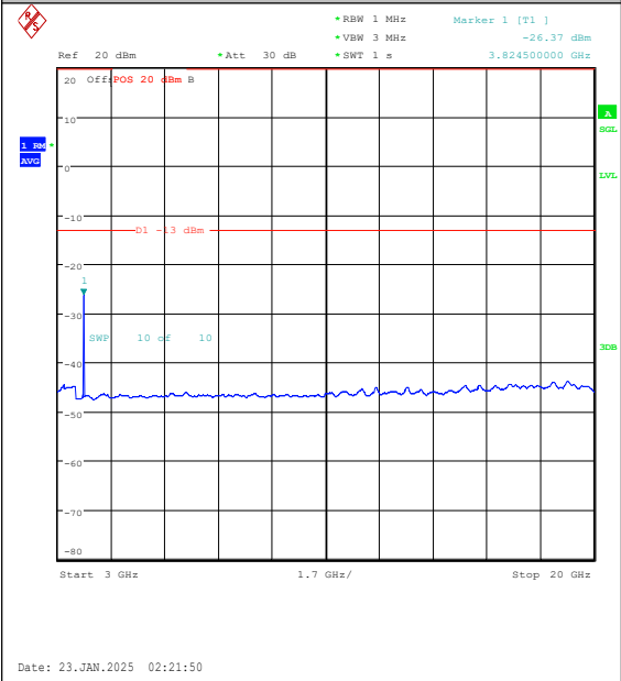
Band25-20MHz-16QAM-26590-1RB#99-3000~20 000-PASS
