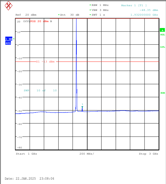
Band25-5MHz-16QAM-26065-1RB#0-1000~3000 -PASS
