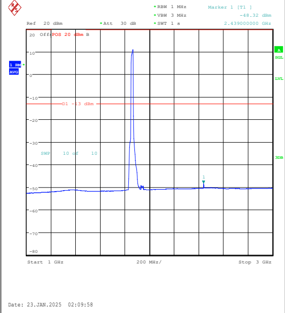
Band25-20MHz-16QAM-26140-100RB#0-1000~3 000-PASS
