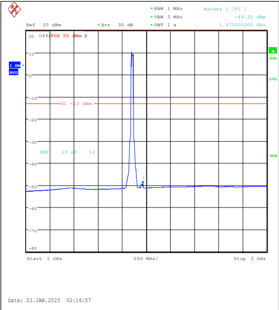
Band25-20MHz-16QAM-26365-100RB#0-1000~3 000-PASS
