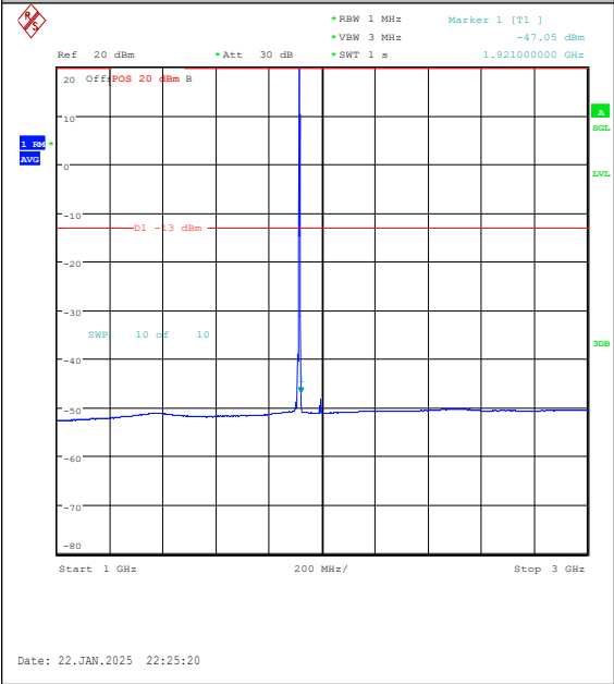
Band25-3MHz-QPSK-26675-1RB#14-1000~3000 -PASS
