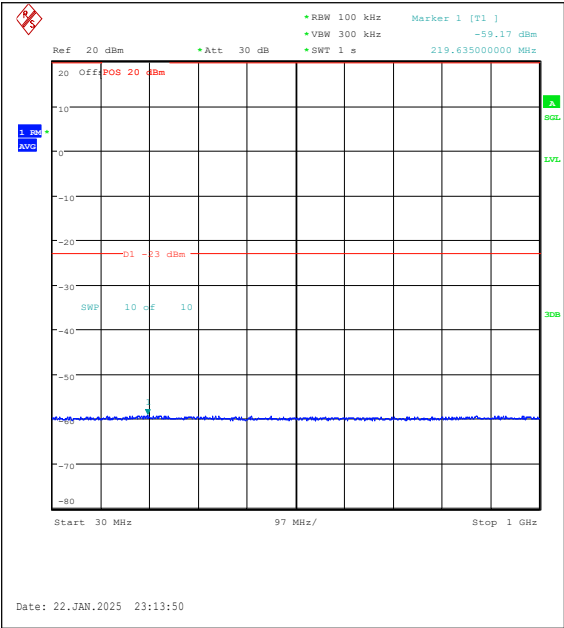
Band25-5MHz-QPSK-26365-1RB#0-30~1000-PA SS
