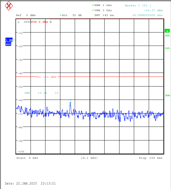
Band25-5MHz-QPSK-26365-1RB#0-0.009~0.15- PASS
