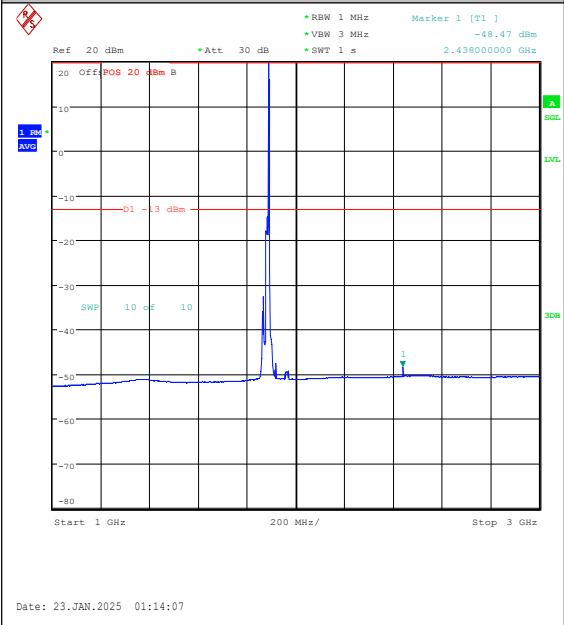
Band25-15MHz-QPSK-26365-1RB#74-1000~300 0-PASS
