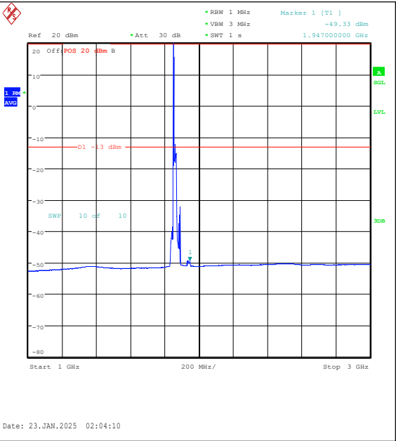
Band25-20MHz-QPSK-26140-1RB#0-1000~3000- PASS
