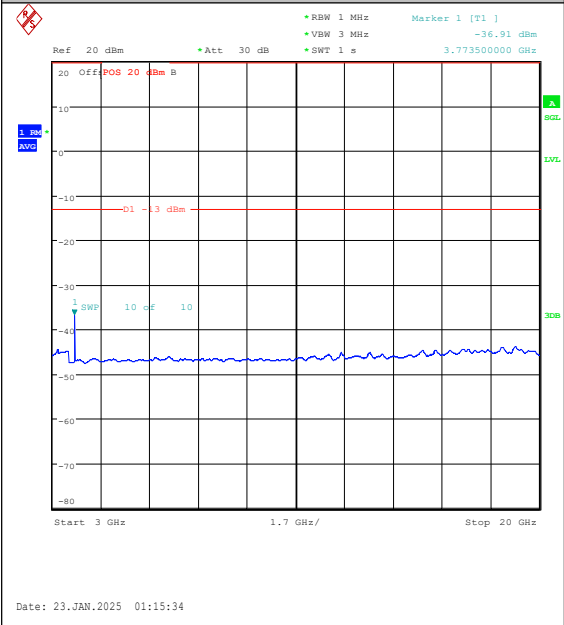
Band25-15MHz-16QAM-26365-1RB#74-3000~20 000-PASS
