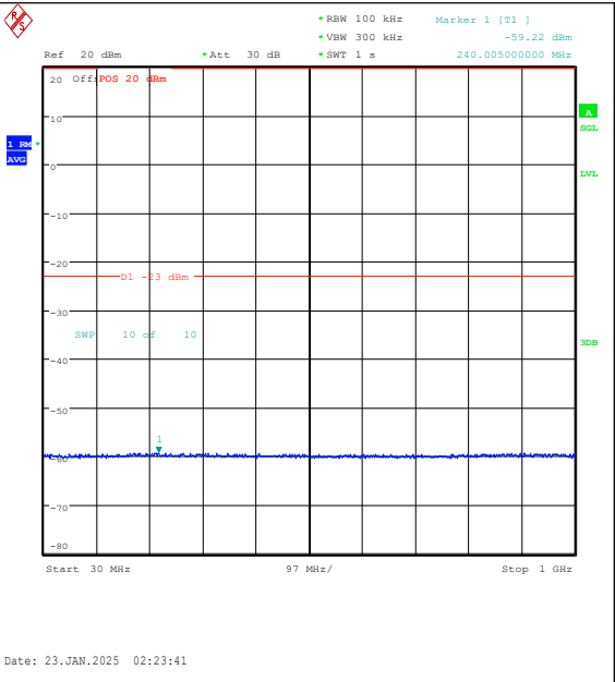
Band25-20MHz-16QAM-26590-100RB#0-30~1000 -PASS
