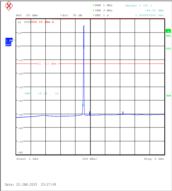
Band25-5MHz-16QAM-26665-25RB#0-1000~300 0-PASS
