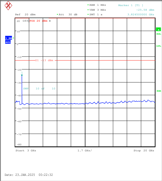
Band25-10MHz-16QAM-26640-1RB#49-3000~20 000-PASS
