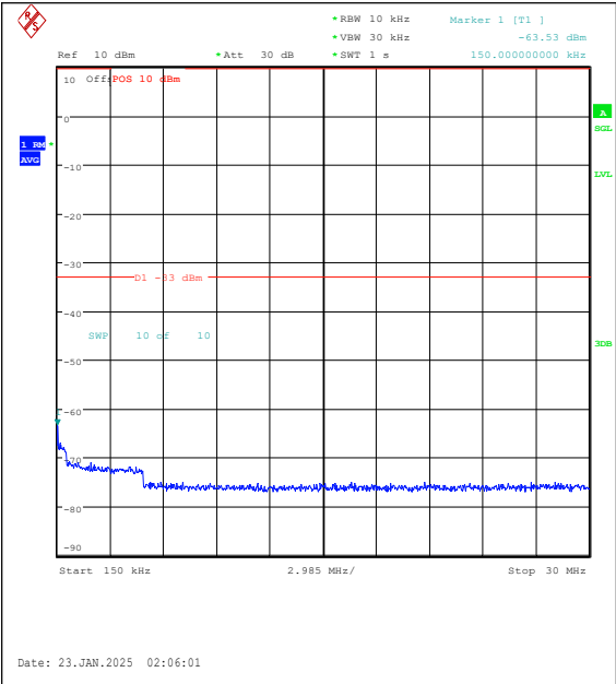
Band25-20MHz-QPSK-26140-1RB#99-0.15~30-P ASS
