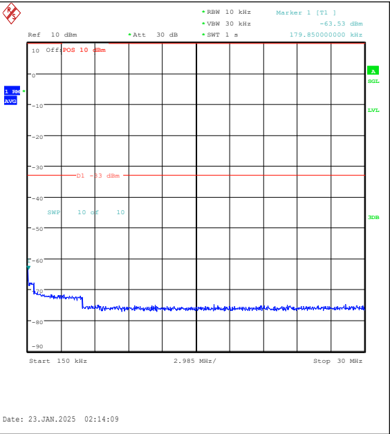
Band25-20MHz-16QAM-26365-1RB#99-0.15~30-P ASS
