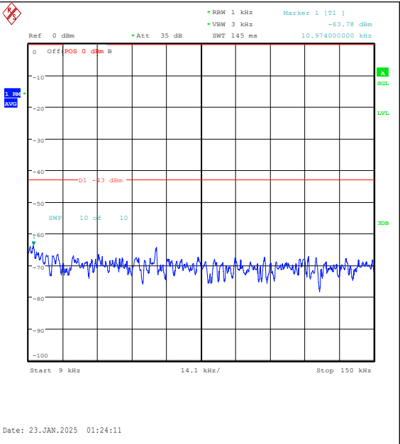
Band25-15MHz-16QAM-26615-75RB#0-0.009~0.15-PASS
