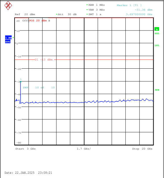
Band25-5MHz-16QAM-26065-1RB#0-3000~20000 -PASS
