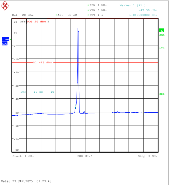
Band25-15MHz-QPSK-26615-75RB#0-1000~3000-PASS
