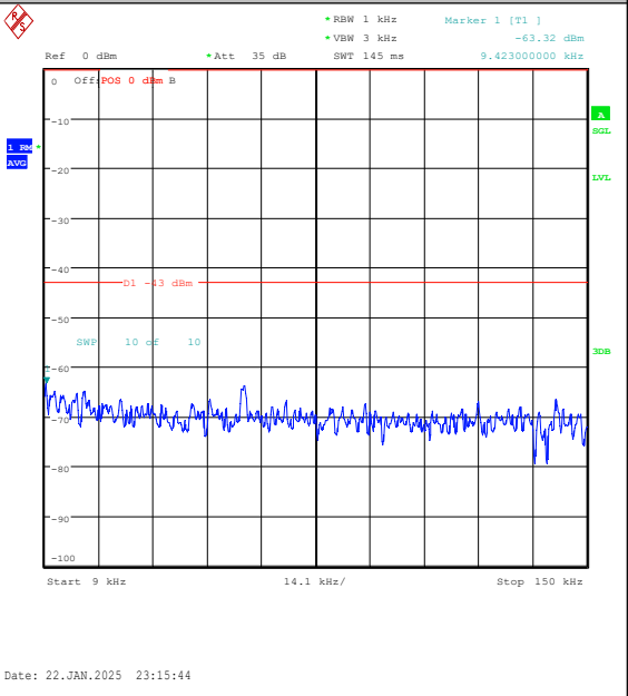
Band25-5MHz-QPSK-26365-1RB#24-0.009~0.15- PASS
