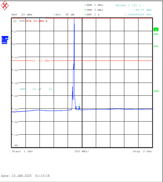
Band25-15MHz-16QAM-26365-1RB#74-1000~300 0-PASS
