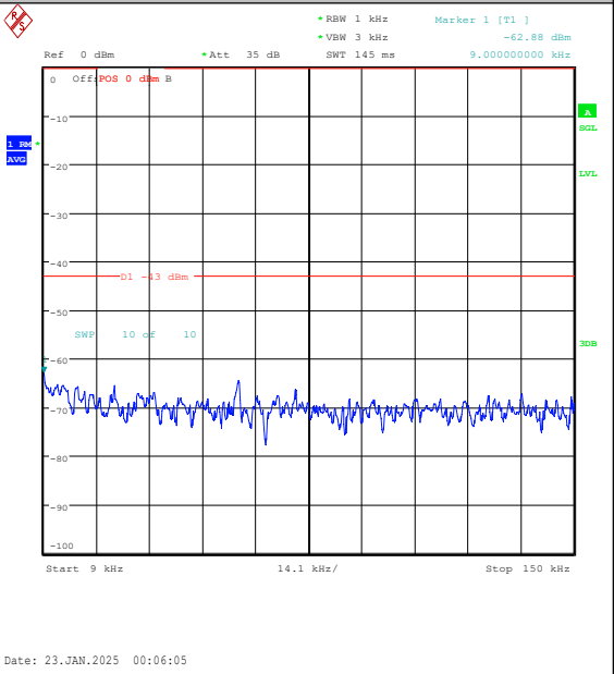
Band25-10MHz-QPSK-26090-1RB#49-0.009~0.15 -PASS
