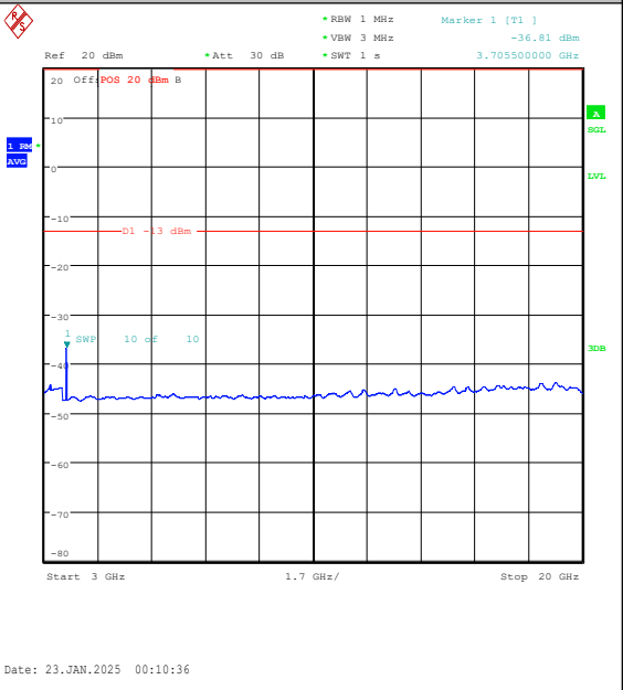
Band25-10MHz-16QAM-26090-50RB#0-3000~20000-PASS
