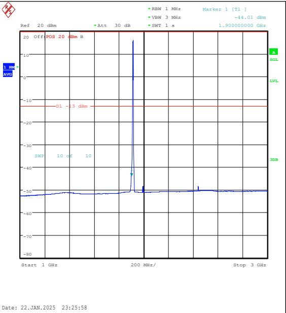
Band25-5MHz-QPSK-26665-25RB#0-1000~3000- PASS
