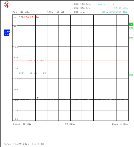
Band25-15MHz-QPSK-26365-75RB#0-30~1000- PASS
