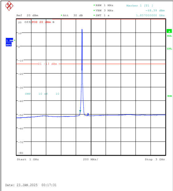
Band25-10MHz-16QAM-26365-50RB#0-1000~30 00-PASS
