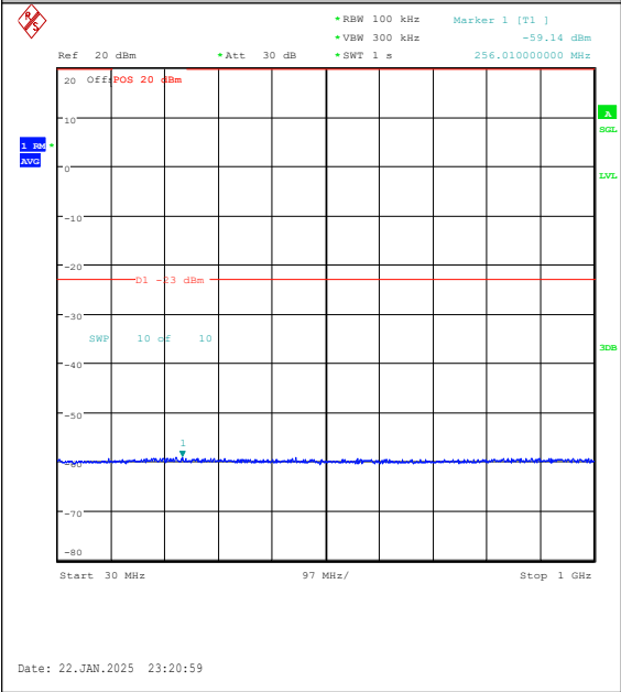
Band25-5MHz-QPSK-26665-1RB#0-30~1000-PA
