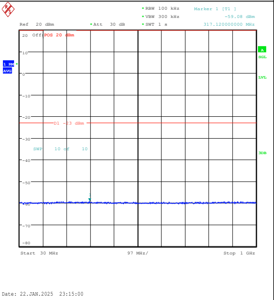
Band25-5MHz-16QAM-26365-1RB#0-30~1000-PA SS
