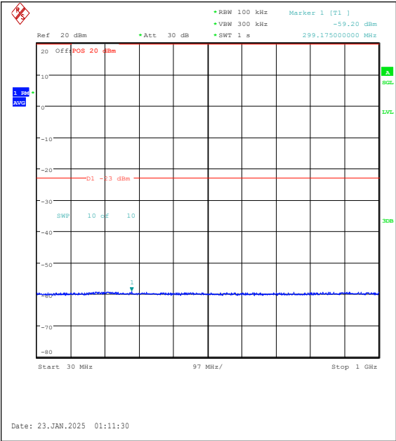
Band25-15MHz-QPSK-26365-1RB#0-30~1000-P ASS
