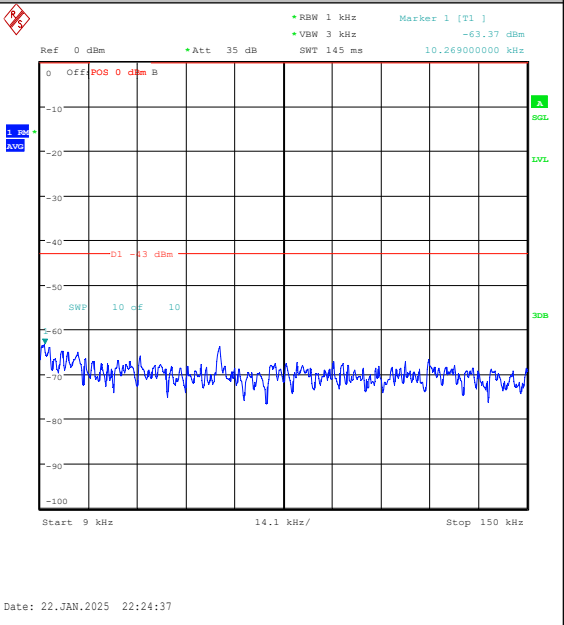
Band25-3MHz-QPSK-26675-1RB#14-0.009~0.15- PASS
