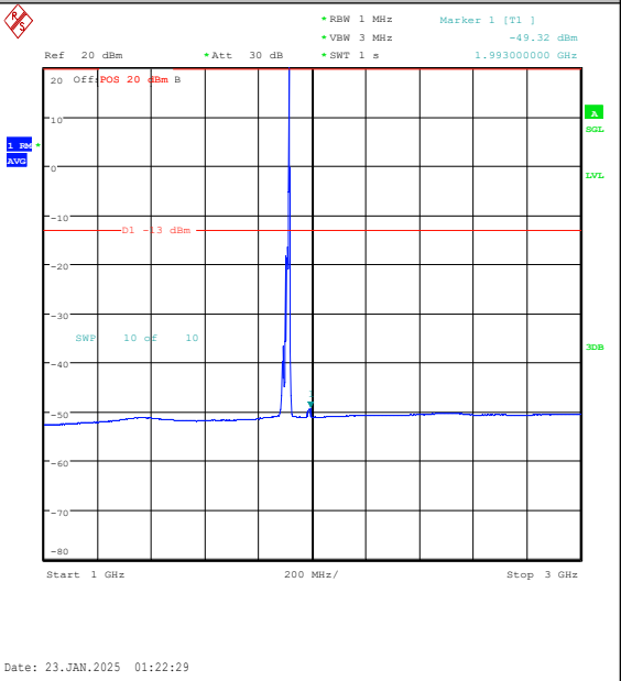
Band25-15MHz-16QAM-26615-1RB#74-1000~3000 0-PASS
