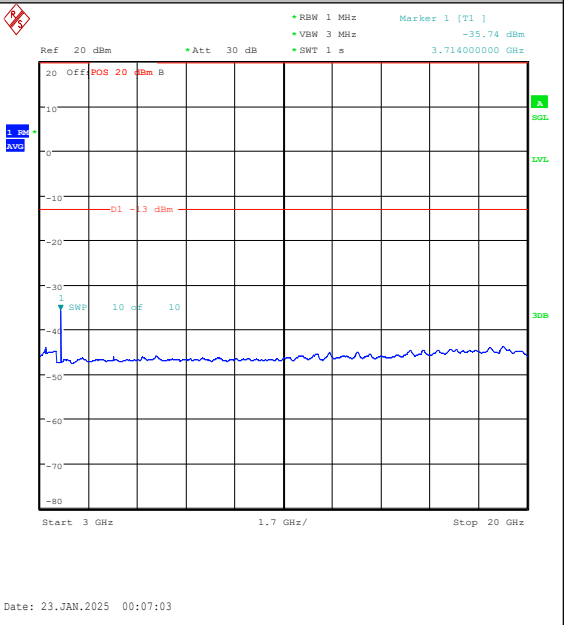
Band25-10MHz-QPSK-26090-1RB#49-3000~2000 0-PASS
