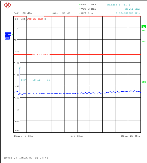
Band25-15MHz-16QAM-26615-1RB#74-3000~20000-PASS
