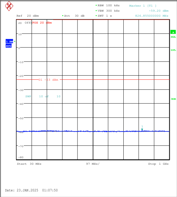
Band25-15MHz-16QAM-26115-1RB#74-30~1000-PASS
