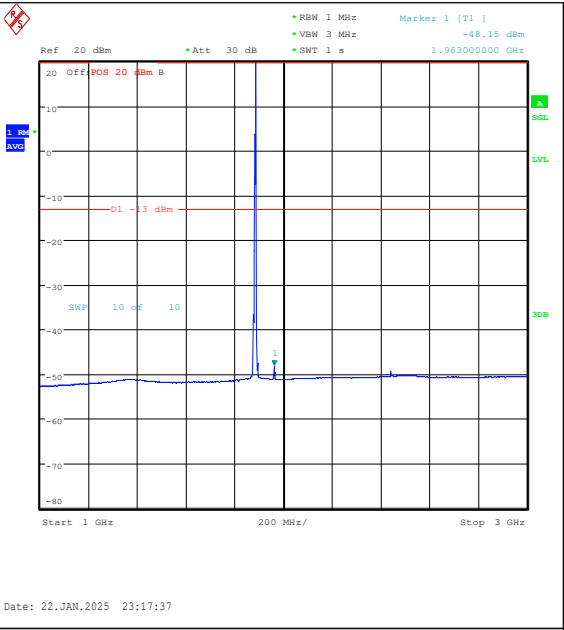
Band25-5MHz-16QAM-26365-1RB#24-1000~3000-PASS
