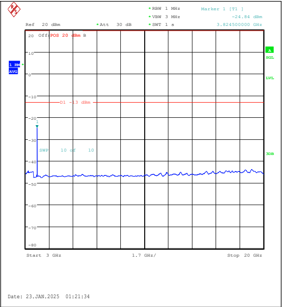
Band25-15MHz-QPSK-26615-1RB#74-3000~2000 0-PASS
