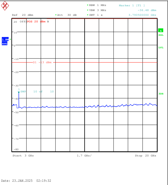
Band25-20MHz-16QAM-26590-1RB#0-3000~2000 0-PASS
