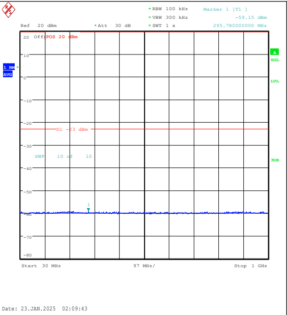
Band25-20MHz-16QAM-26140-100RB#0-30~1000 -PASS
