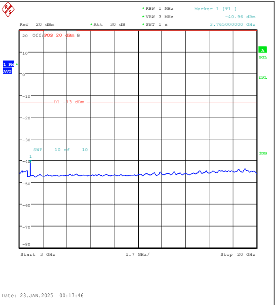
Band25-10MHz-16QAM-26365-50RB#0-3000~200 00-PASS
