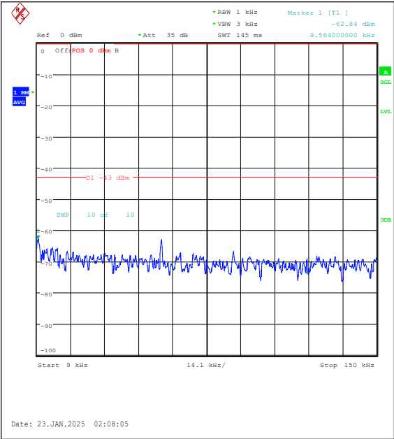
Band25-20MHz-QPSK-26140-100RB#0-0.009~0.15-PASS
