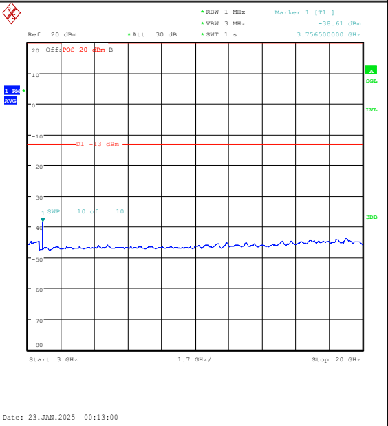
Band25-10MHz-16QAM-26365-1RB#0-3000~2000 0-PASS
