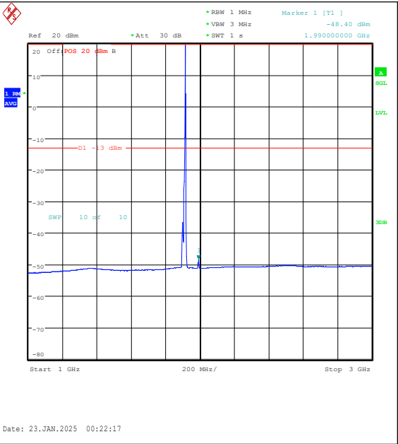
Band25-10MHz-16QAM-26640-1RB#49-1000~300 0-PASS
