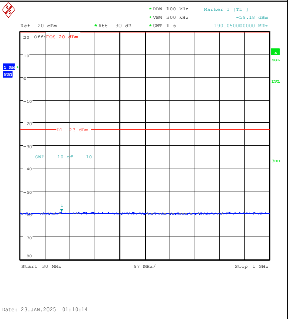
Band25-15MHz-16QAM-26115-75RB#0-30~1000-PASS
