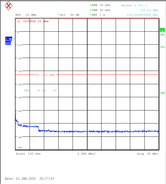
Band25-10MHz-16QAM-26365-50RB#0-0.15~30000-PASS
