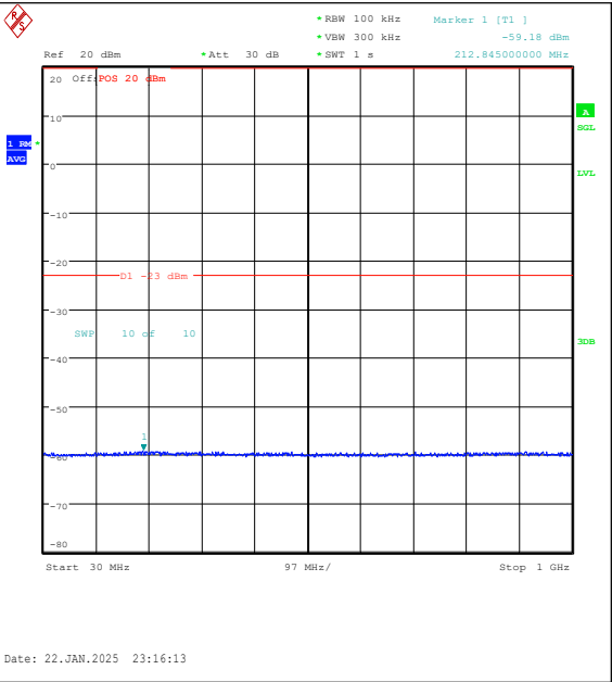
Band25-5MHz-QPSK-26365-1RB#24-30~1000-PA SS
