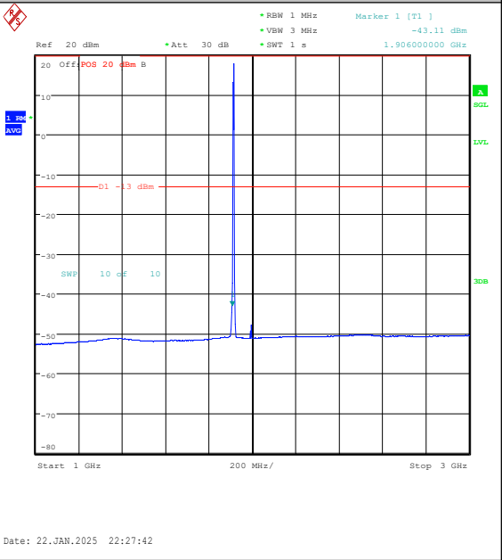
Band25-3MHz-QPSK-26675-15RB#0-1000~3000- PASS
