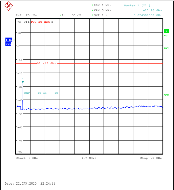
Band25-3MHz-16QAM-26675-1RB#0-3000~20000 -PASS
