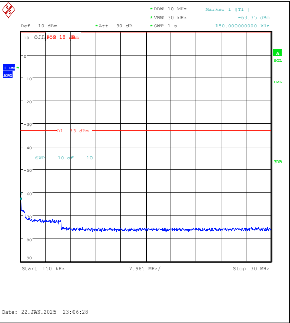
Band25-5MHz-QPSK-26065-1RB#0-0.15~30-PAS
