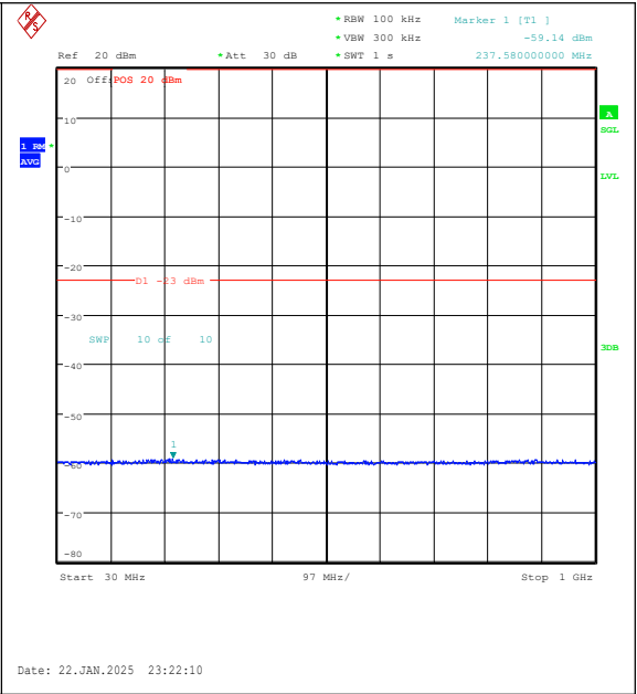
Band25-5MHz-16QAM-26665-1RB#0-30~1000-PA SS
