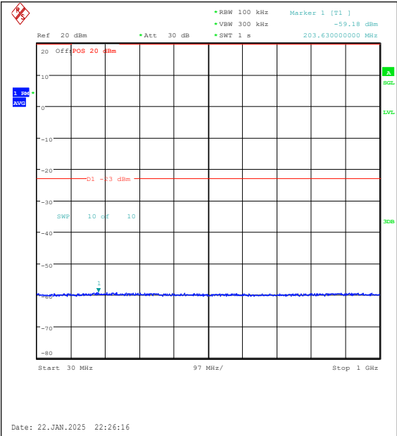
Band25-3MHz-16QAM-26675-1RB#14-30~1000-PASS
