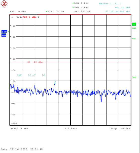
Band25-5MHz-16QAM-26665-1RB#0-0.009~0.15- PASS
