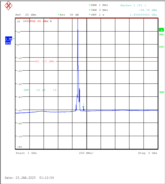
Band25-15MHz-16QAM-26365-1RB#0-1000~300 0-PASS
