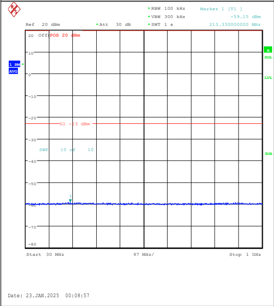
Band25-10MHz-QPSK-26090-50RB#0-30~1000- PASS
