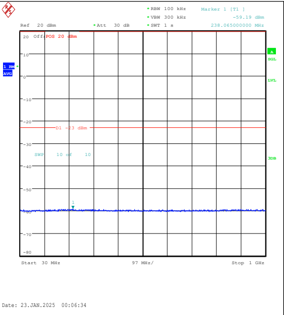
Band25-10MHz-QPSK-26090-1RB#49-30~1000-P ASS
