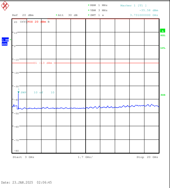
Band25-20MHz-QPSK-26140-1RB#99-3000~2000 0-PASS
