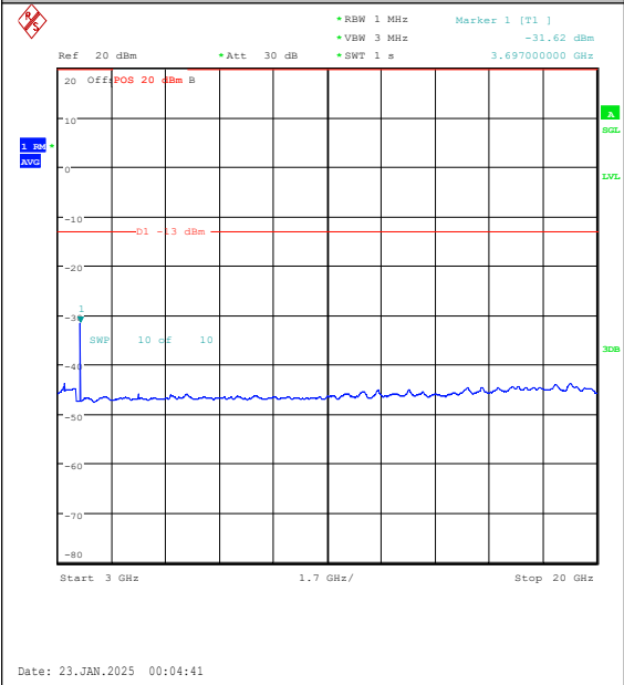
Band25-10MHz-QPSK-26090-1RB#0-3000~2000 0-PASS
