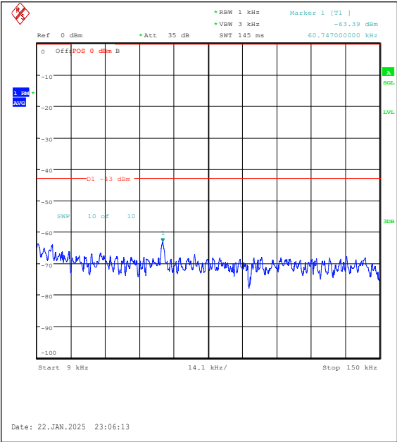
Band25-5MHz-QPSK-26065-1RB#0-0.009~0.15-PASS
