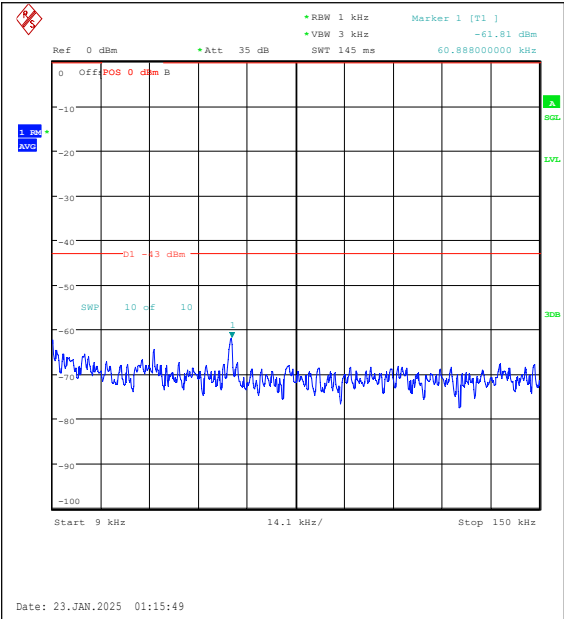
Band25-15MHz-QPSK-26365-75RB#0-0.009~0.1 5-PASS
