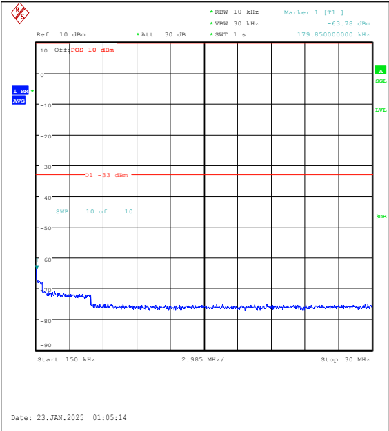
Band25-15MHz-16QAM-26115-1RB#0-0.15~30-P ASS
