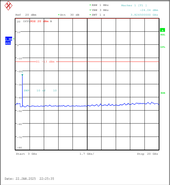
Band25-3MHz-QPSK-26675-1RB#14-3000~20000 -PASS
