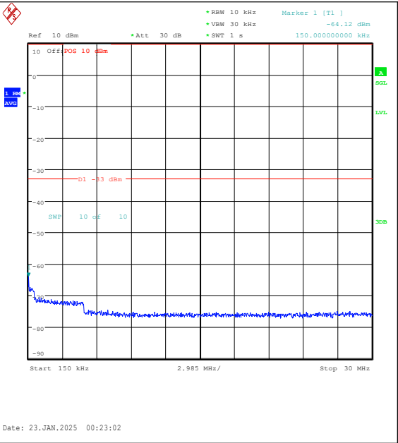
Band25-10MHz-QPSK-26640-50RB#0-0.15~30-PA SS
