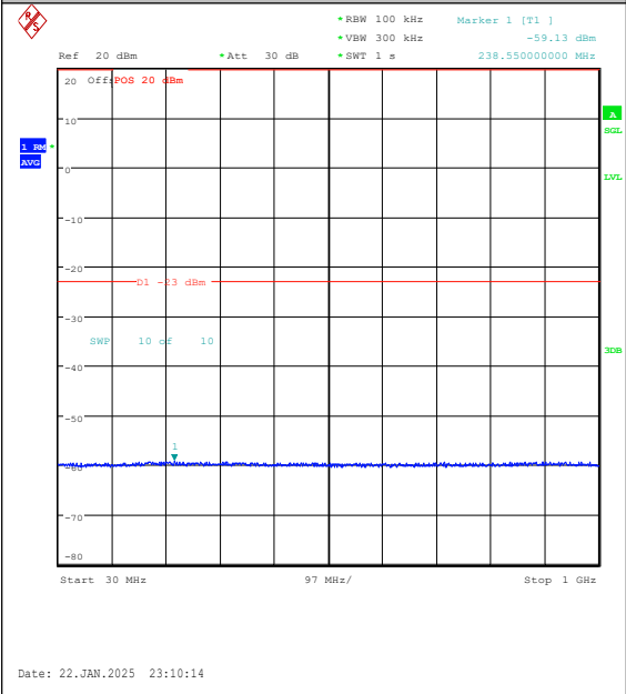
Band25-5MHz-16QAM-26065-1RB#24-30~1000- PASS
