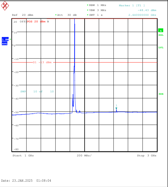
Band25-15MHz-16QAM-26115-1RB#74-1000~3000-PASS
