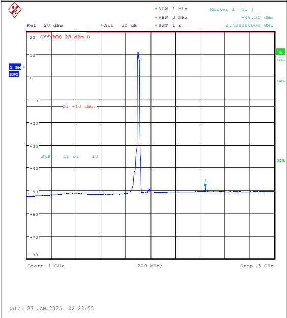
Band25-20MHz-16QAM-26590-100RB#0-1000~3 000-PASS
