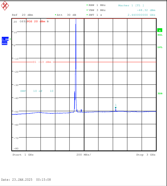
Band25-10MHz-16QAM-26365-1RB#49-1000~300 0-PASS
