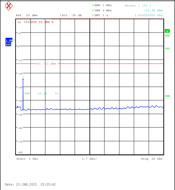
Band25-20MHz-QPSK-26590-1RB#99-3000~2000 0-PASS
