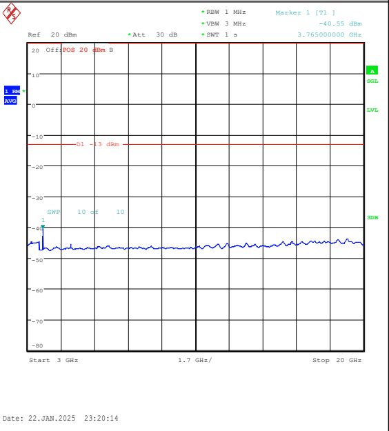
Band25-5MHz-16QAM-26365-25RB#0-3000~2000 0-PASS
