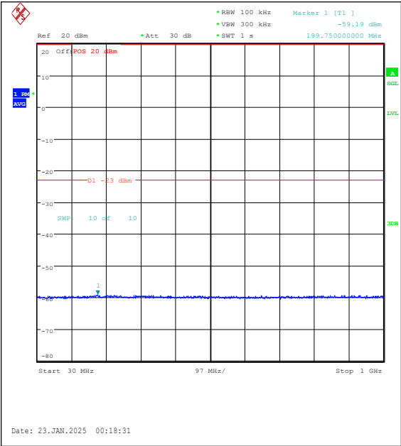
Band25-10MHz-QPSK-26640-1RB#0-30~1000-P ASS
