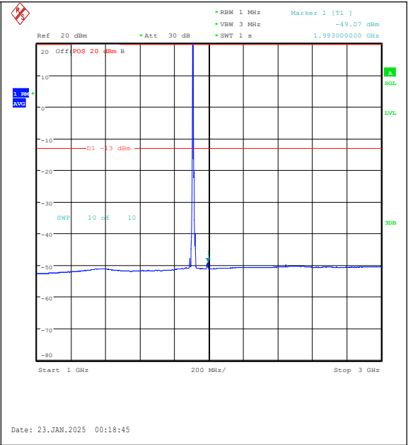
Band25-10MHz-QPSK-26640-1RB#0-1000~3000- PASS
