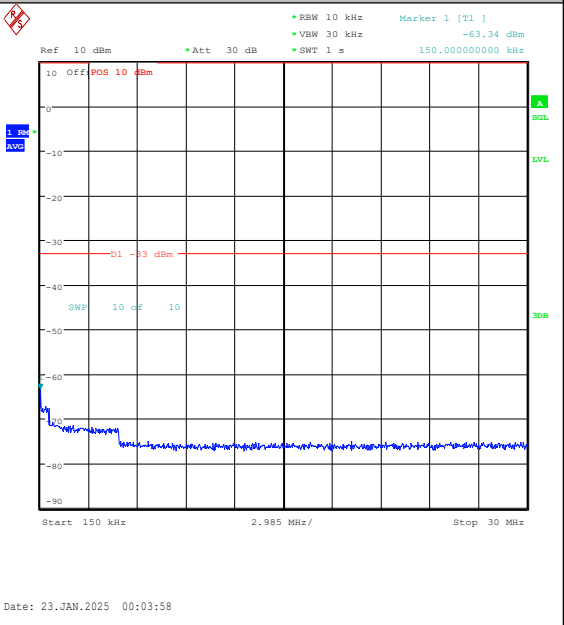
Band25-10MHz-QPSK-26090-1RB#0-0.15~30-PA SS
