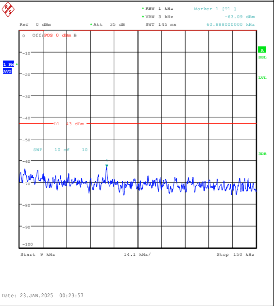
Band25-10MHz-16QAM-26640-50RB#0-0.009~0.1 5-PASS
