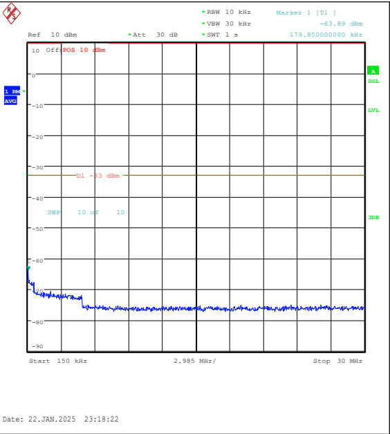
Band25-5MHz-QPSK-26365-25RB#0-0.15~30-PA SS
