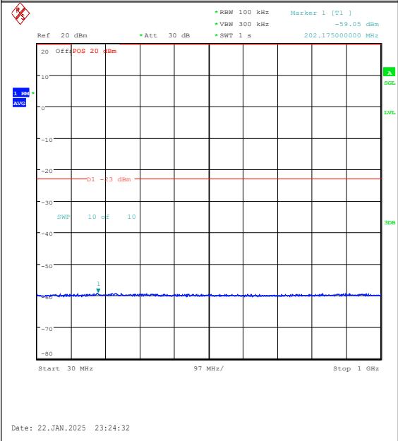
Band25-5MHz-16QAM-26665-1RB#24-30~1000- PASS
