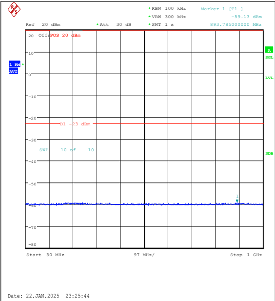
Band25-5MHz-QPSK-26665-25RB#0-30~1000-P ASS
