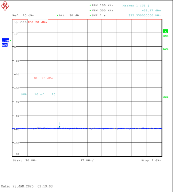
Band25-20MHz-16QAM-26590-1RB#0-30~1000-PASS
