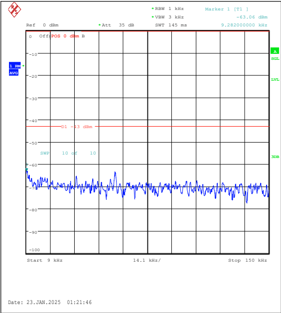
Band25-15MHz-16QAM-26615-1RB#74-0.009~0.15-PASS
