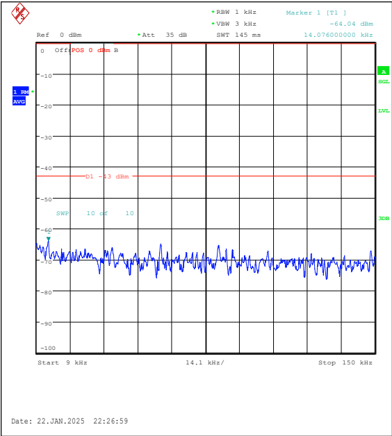
Band25-3MHz-QPSK-26675-15RB#0-0.009~0.15 -PASS
