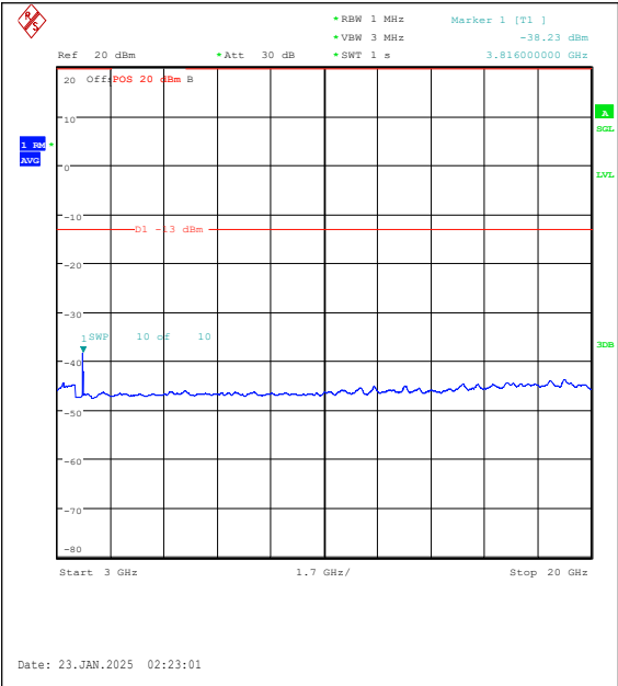
Band25-20MHz-QPSK-26590-100RB#0-3000~20000-PASS
