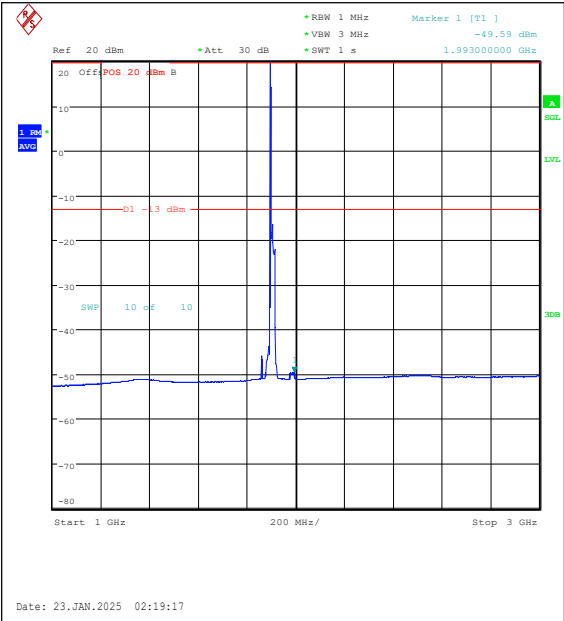
Band25-20MHz-16QAM-26590-1RB#0-1000~300 0-PASS
