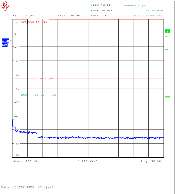
Band25-20MHz-QPSK-26140-100RB#0-0.15~30-P ASS
