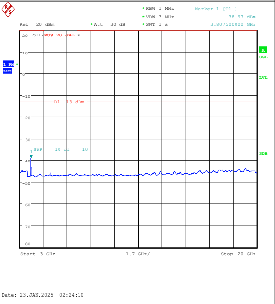
Band25-20MHz-16QAM-26590-100RB#0-3000~20 000-PASS
