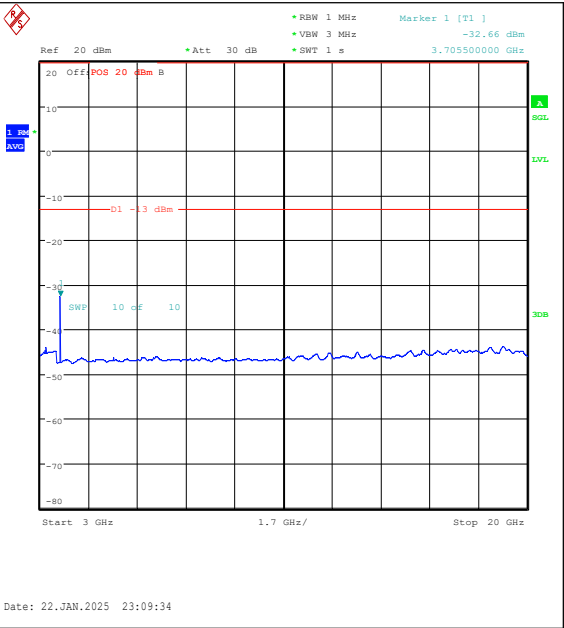
Band25-5MHz-QPSK-26065-1RB#24-3000~20000 -PASS
