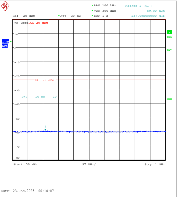
Band25-10MHz-16QAM-26090-50RB#0-30~1000-PASS
