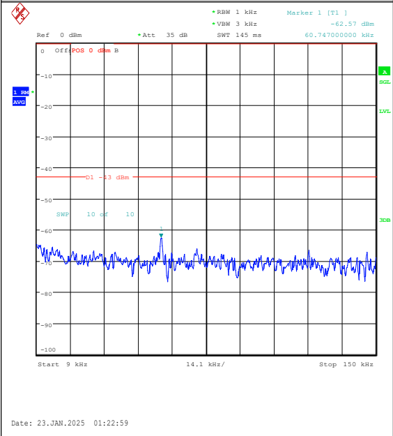
Band25-15MHz-QPSK-26615-75RB#0-0.009~0.1 5-PASS
