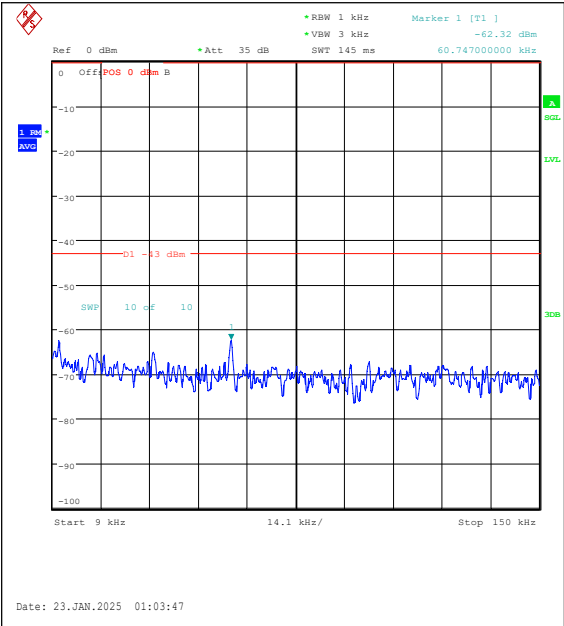
Band25-15MHz-QPSK-26115-1RB#0-0.009~0.15-PASS
