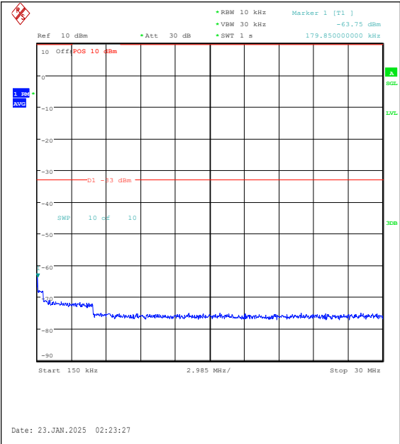
Band25-20MHz-16QAM-26590-100RB#0-0.15~3 0-PASS
