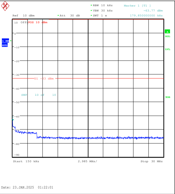
Band25-15MHz-16QAM-26615-1RB#74-0.15~30-P ASS
