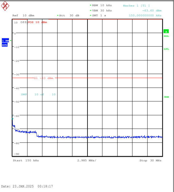
Band25-10MHz-QPSK-26640-1RB#0-0.15~30-PA SS
