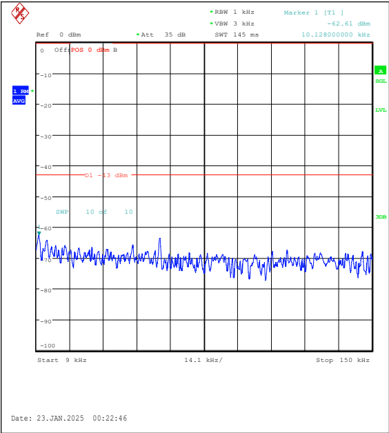
Band25-10MHz-QPSK-26640-50RB#0-0.009~0.1 5-PASS
