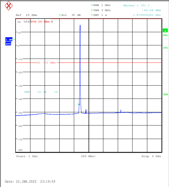
Band25-5MHz-16QAM-26365-25RB#0-1000~300 0-PASS
