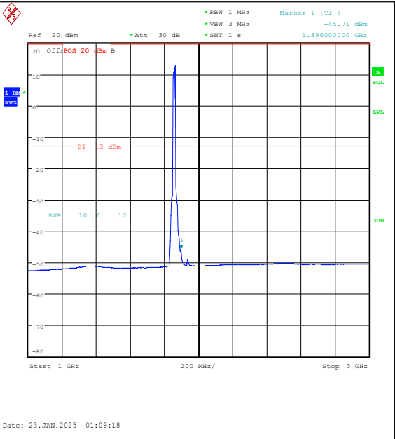
Band25-15MHz-QPSK-26115-75RB#0-1000~3000 -PASS
