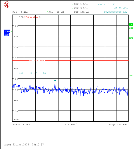
Band25-5MHz-QPSK-26065-25RB#0-0.009~0.15 -PASS
