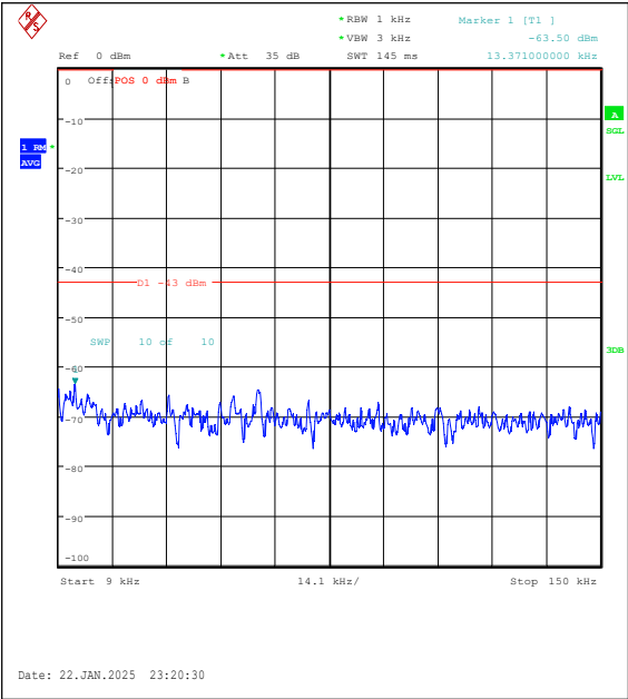
Band25-5MHz-QPSK-26665-1RB#0-0.009~0.15-PASS
