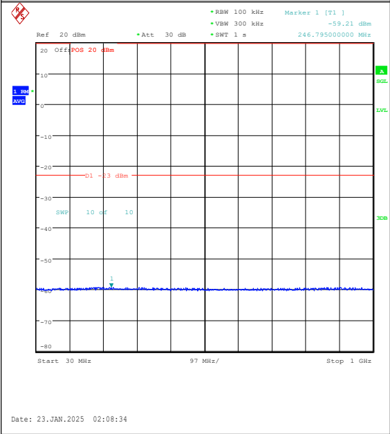
Band25-20MHz-QPSK-26140-100RB#0-30~1000-PASS
