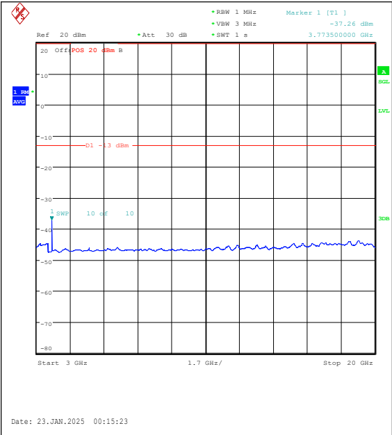
Band25-10MHz-16QAM-26365-1RB#49-3000~20000-PASS
