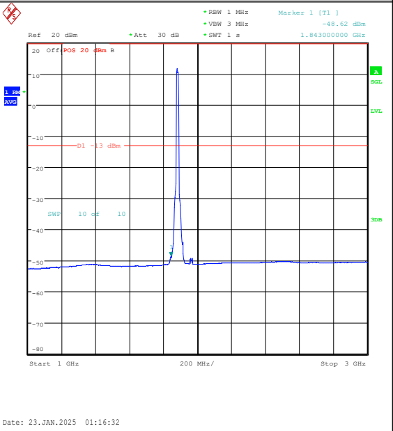
Band25-15MHz-QPSK-26365-75RB#0-1000~3000 -PASS
