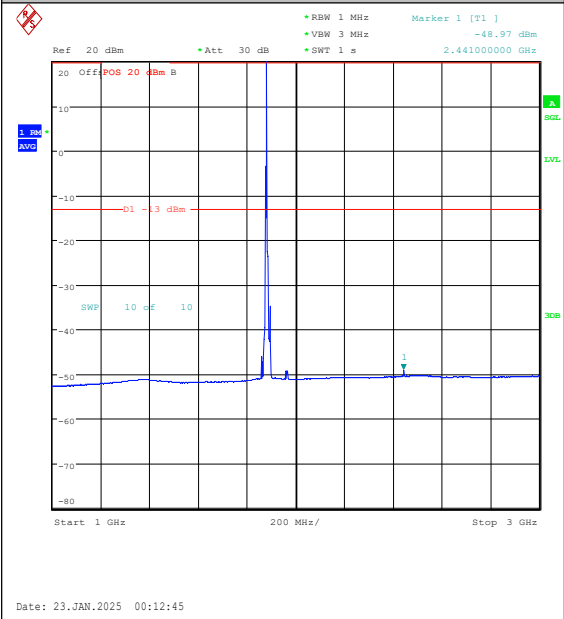
Band25-10MHz-16QAM-26365-1RB#0-1000~300 0-PASS
