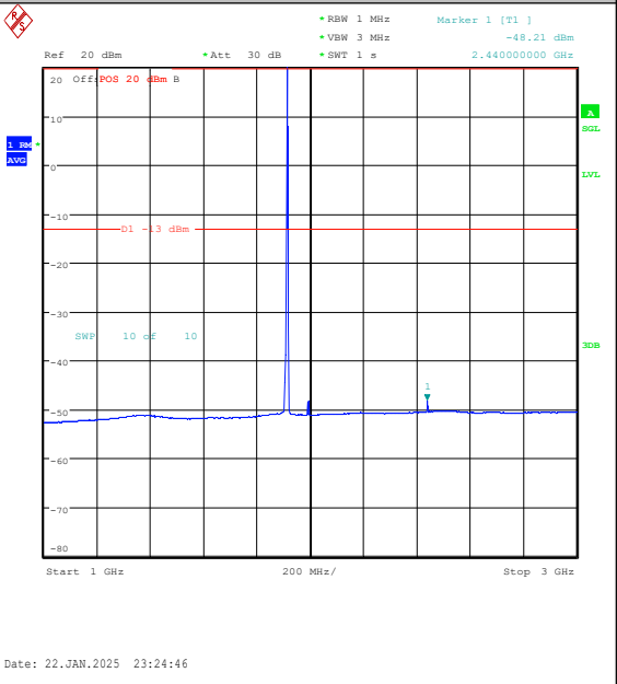
Band25-5MHz-16QAM-26665-1RB#24-1000~3000 -PASS
