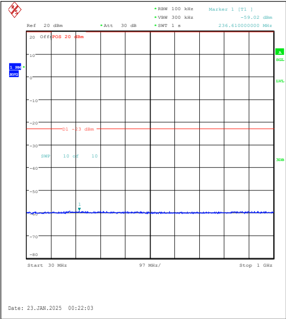
Band25-10MHz-16QAM-26640-1RB#49-30~1000 -PASS
