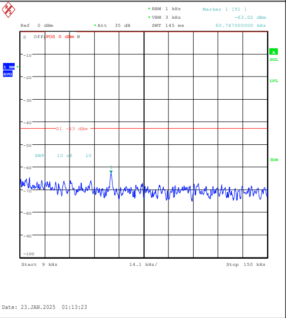
Band25-15MHz-QPSK-26365-1RB#74-0.009~0.15 -PASS
