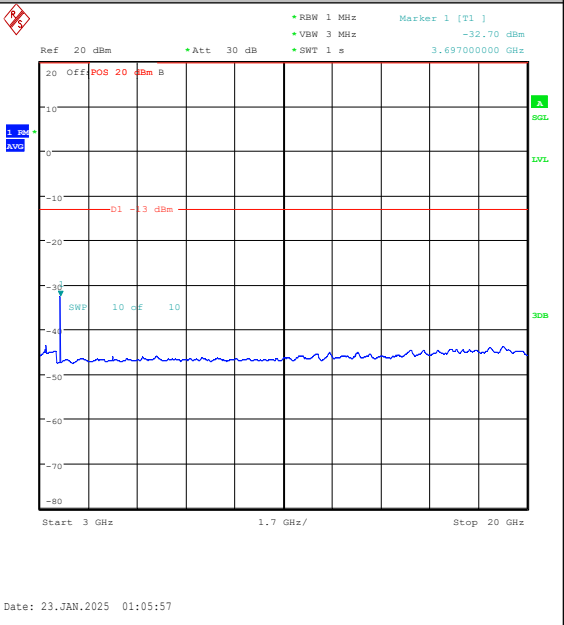
Band25-15MHz-16QAM-26115-1RB#0-3000~2000 0-PASS
