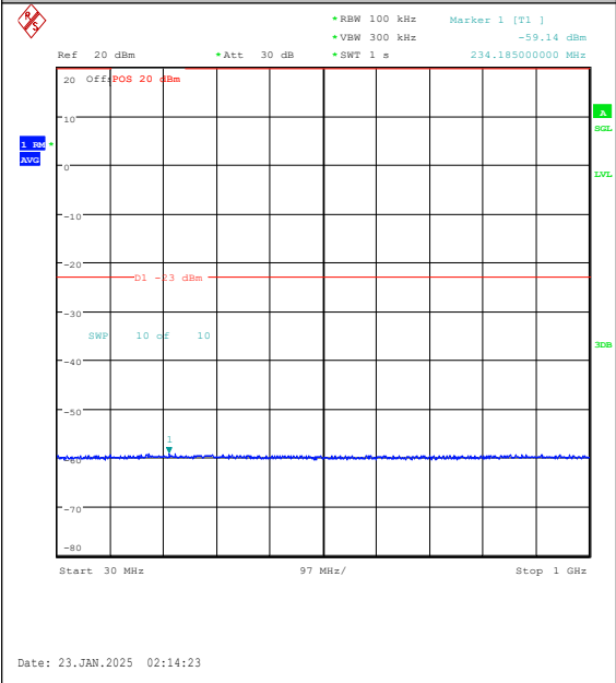
Band25-20MHz-16QAM-26365-1RB#99-30~1000-PASS
