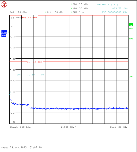
Band25-20MHz-16QAM-26140-1RB#99-0.15~30-P ASS
