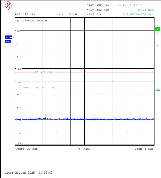
Band25-15MHz-QPSK-26615-1RB#0-30~1000-P ASS
