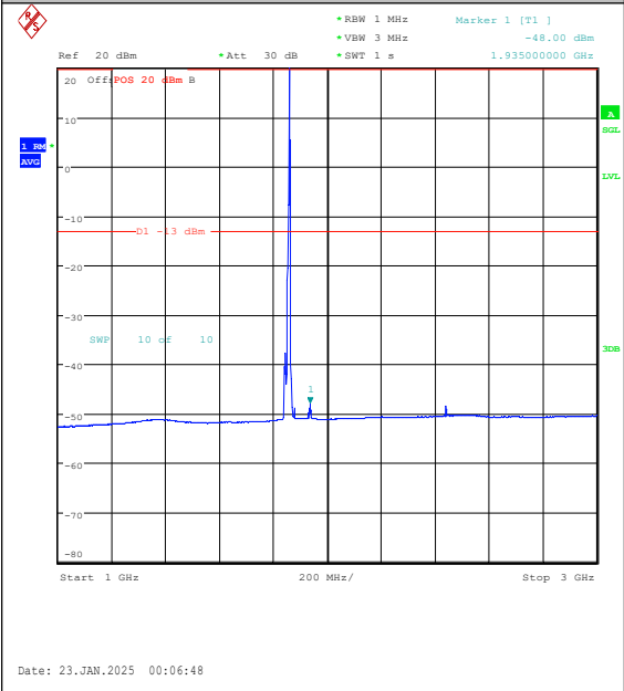
Band25-10MHz-QPSK-26090-1RB#49-1000~300 0-PASS
