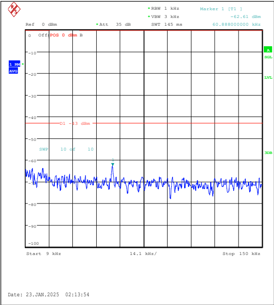
Band25-20MHz-16QAM-26365-1RB#99-0.009~0.15-PASS
