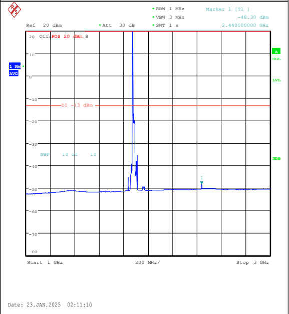
Band25-20MHz-QPSK-26365-1RB#0-1000~3000- PASS
