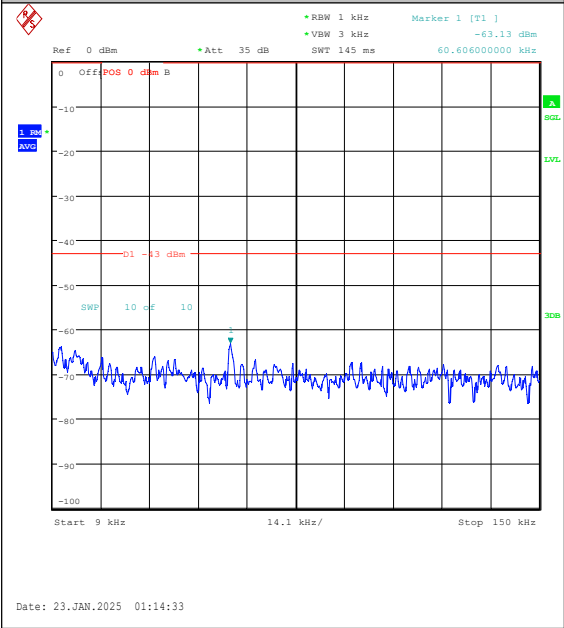
Band25-15MHz-16QAM-26365-1RB#74-0.009~0. 15-PASS
