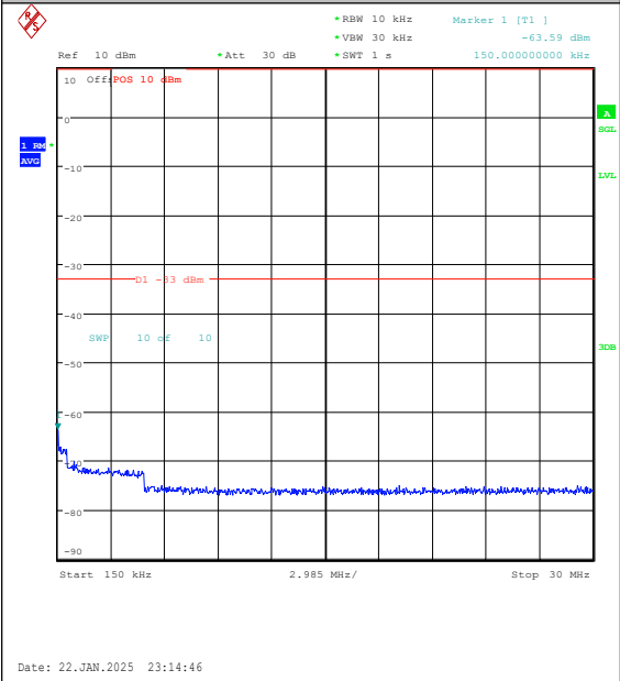
Band25-5MHz-16QAM-26365-1RB#0-0.15~30-PA SS
