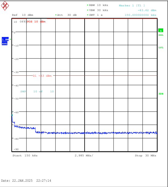
Band25-3MHz-QPSK-26675-15RB#0-0.15~30-PA SS
