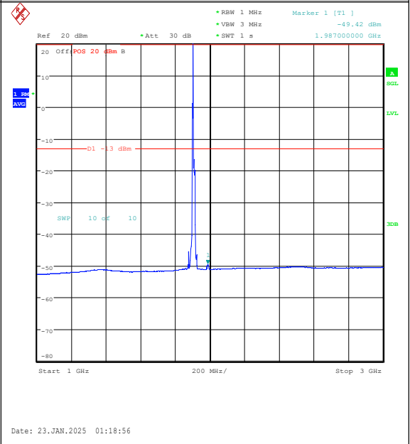
Band25-15MHz-QPSK-26615-1RB#0-1000~3000- PASS
