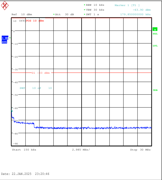
Band25-5MHz-QPSK-26665-1RB#0-0.15~30-PAS
