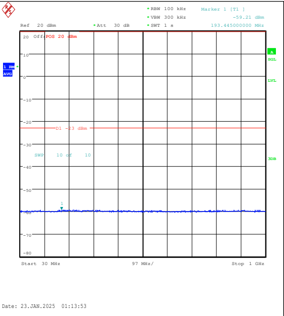
Band25-15MHz-QPSK-26365-1RB#74-30~1000-P ASS
