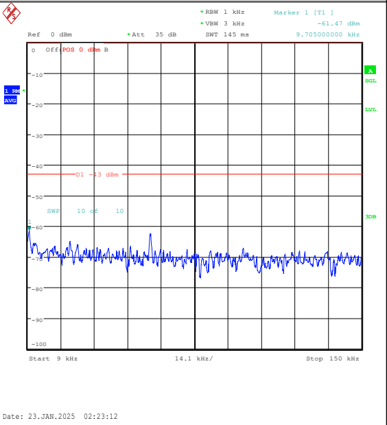
Band25-20MHz-16QAM-26590-100RB#0-0.009~0. 15-PASS
