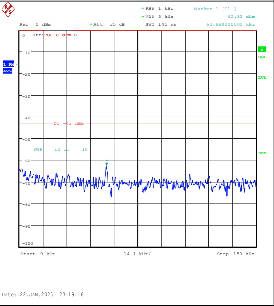
Band25-5MHz-16QAM-26365-25RB#0-0.009~0.15-PASS
