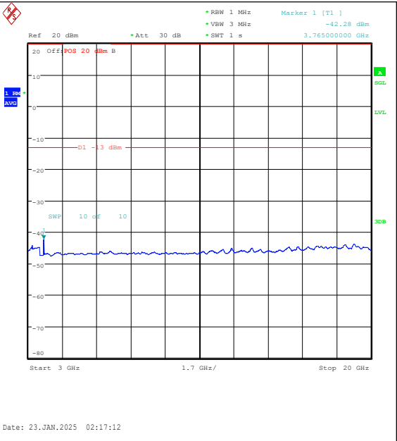
Band25-20MHz-16QAM-26365-100RB#0-3000~20 000-PASS
