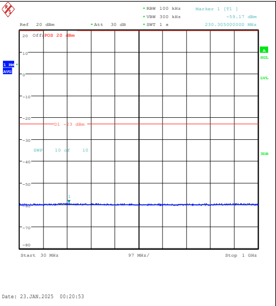
Band25-10MHz-QPSK-26640-1RB#49-30~1000-P ASS
