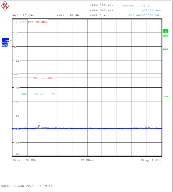
Band25-5MHz-16QAM-26365-25RB#0-30~1000-P ASS
