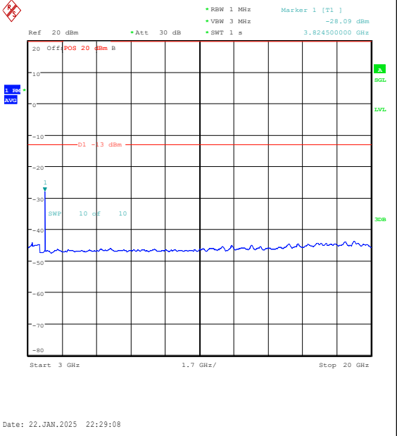
Band25-3MHz-16QAM-26675-15RB#0-3000~2000 0-PASS
