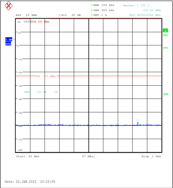
Band25-3MHz-QPSK-26675-1RB#14-30~1000-PA SS
