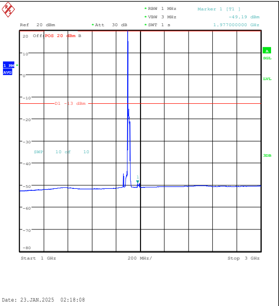
Band25-20MHz-QPSK-26590-1RB#0-1000~3000- PASS
