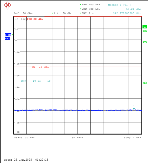
Band25-15MHz-16QAM-26615-1RB#74-30~1000 -PASS
