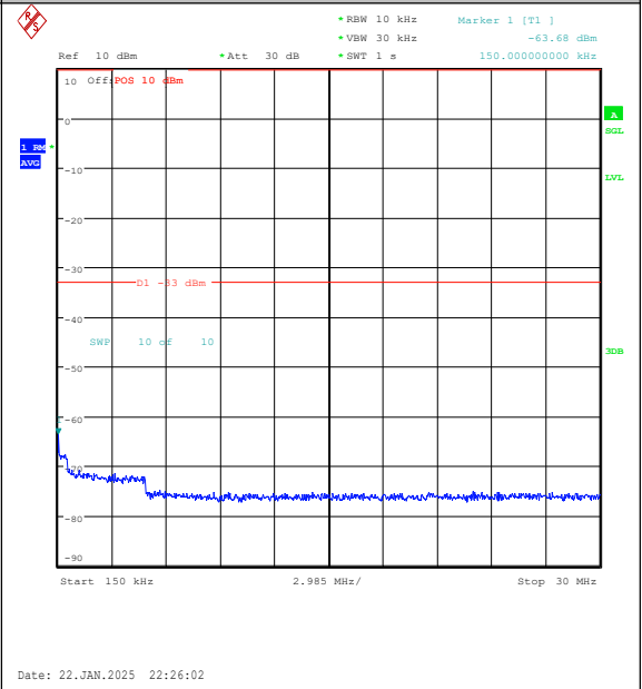
Band25-3MHz-16QAM-26675-1RB#14-0.15~30-P ASS
