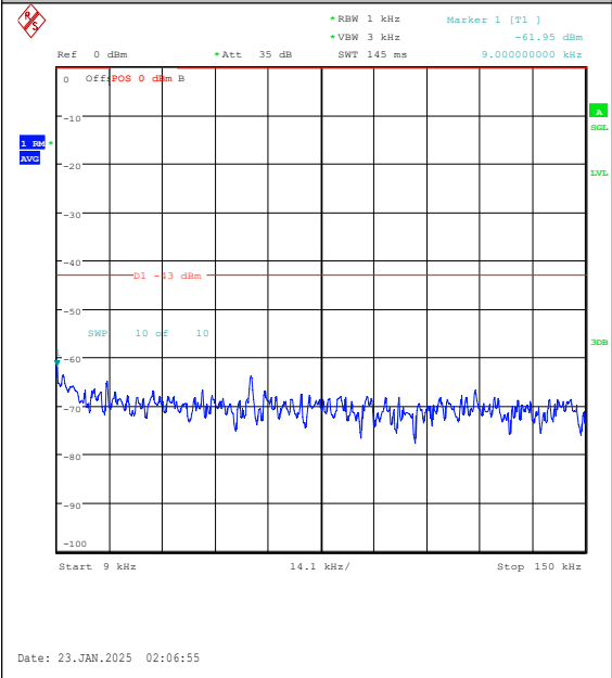
Band25-20MHz-16QAM-26140-1RB#99-0.009~0. 15-PASS
