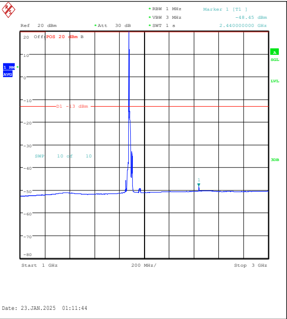
Band25-15MHz-QPSK-26365-1RB#0-1000~3000- PASS
