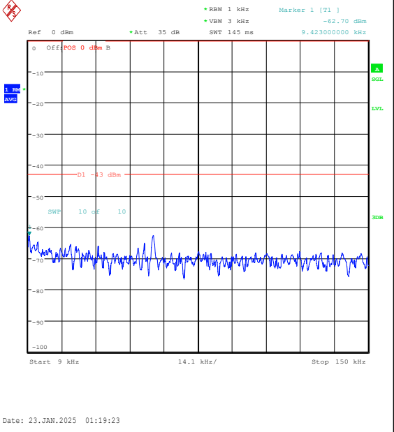
Band25-15MHz-16QAM-26615-1RB#0-0.009~0.15-PASS
