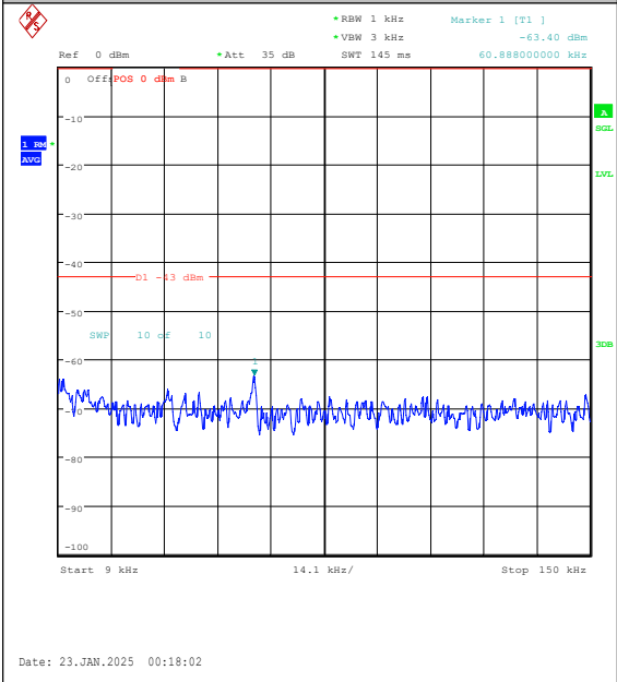
Band25-10MHz-QPSK-26640-1RB#0-0.009~0.15 -PASS
