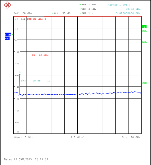
Band25-5MHz-16QAM-26665-1RB#0-3000~20000 -PASS
