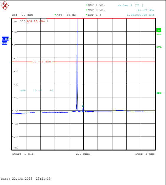
Band25-5MHz-QPSK-26665-1RB#0-1000~3000-P
