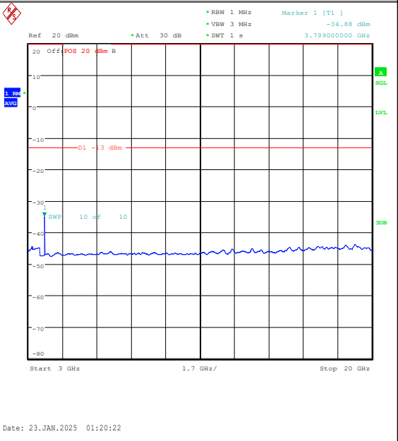
Band25-15MHz-16QAM-26615-1RB#0-3000~2000 0-PASS
