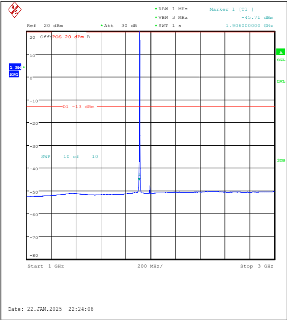
Band25-3MHz-16QAM-26675-1RB#0-1000~3000 -PASS
