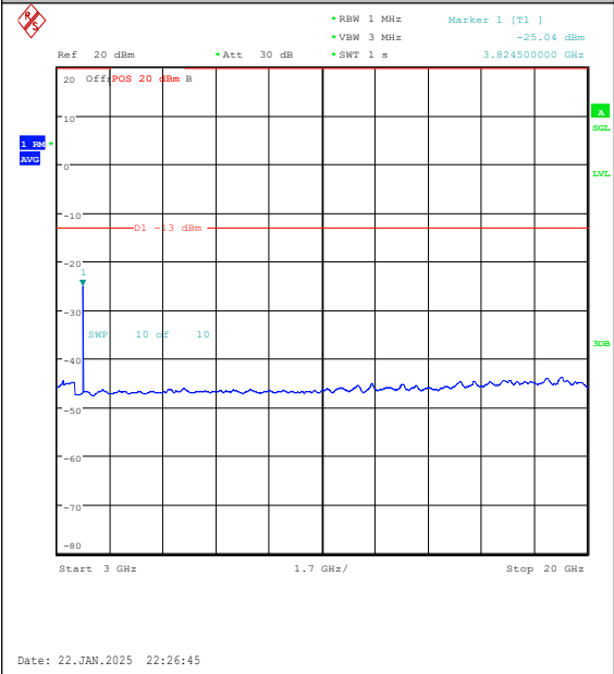
Band25-3MHz-16QAM-26675-1RB#14-3000~20000-PASS
