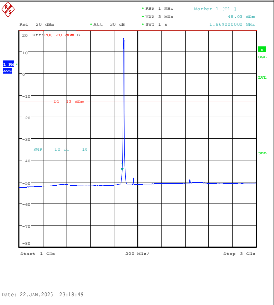
Band25-5MHz-QPSK-26365-25RB#0-1000~3000- PASS
