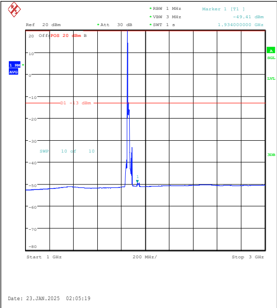
Band25-20MHz-16QAM-26140-1RB#0-1000~300 0-PASS
