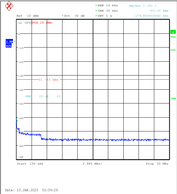
Band25-20MHz-16QAM-26140-100RB#0-0.15~3 0-PASS
