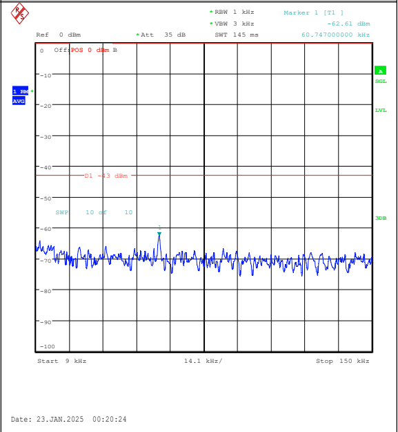
Band25-10MHz-QPSK-26640-1RB#49-0.009~0.15 -PASS
