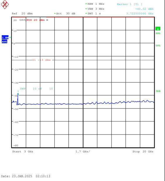
Band25-20MHz-16QAM-26140-100RB#0-3000~20 000-PASS
