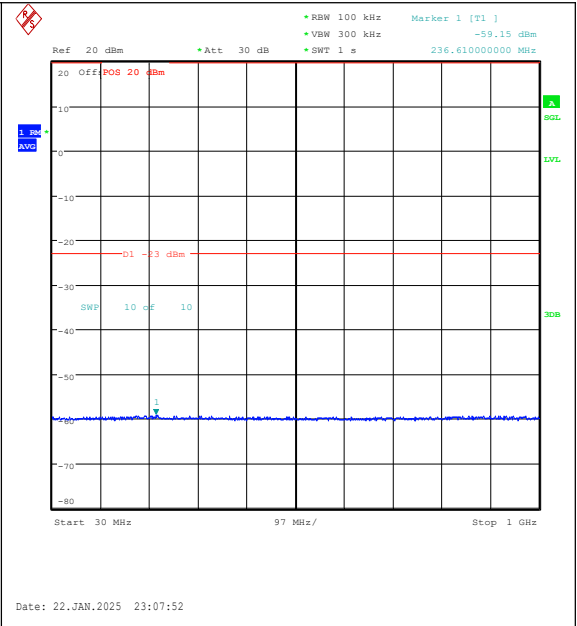
Band25-5MHz-16QAM-26065-1RB#0-30~1000-PA SS
