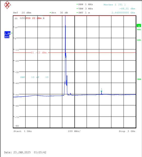
Band25-15MHz-16QAM-26115-1RB#0-1000~300 0-PASS
