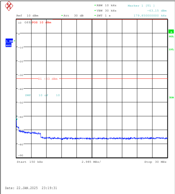
Band25-5MHz-16QAM-26365-25RB#0-0.15~30-P ASS
