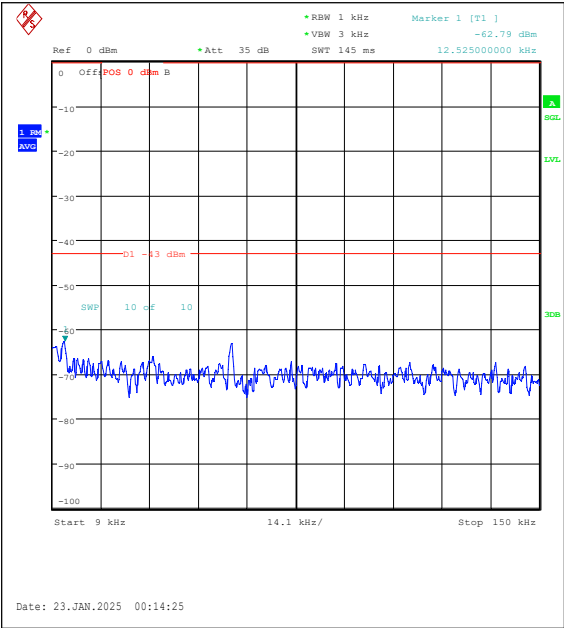
Band25-10MHz-16QAM-26365-1RB#49-0.009~0. 15-PASS
