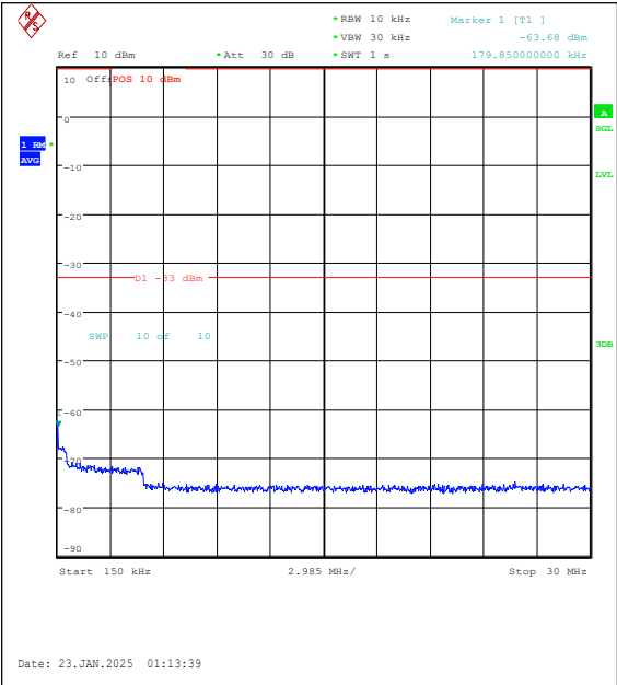
Band25-15MHz-QPSK-26365-1RB#74-0.15~30-P ASS
