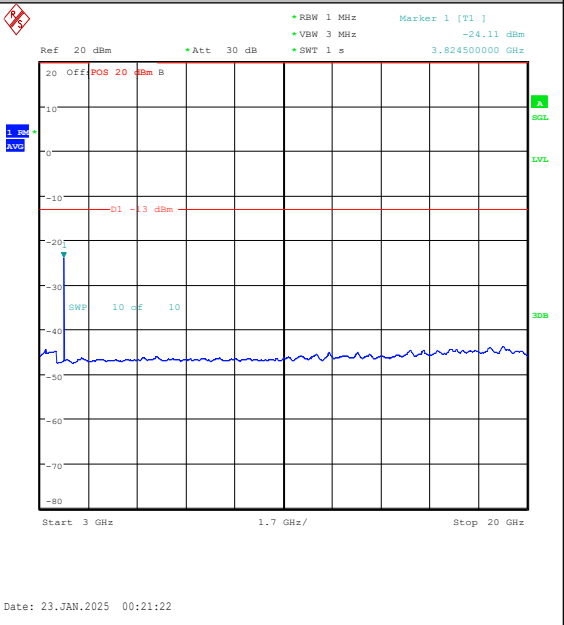
Band25-10MHz-QPSK-26640-1RB#49-3000~2000 0-PASS
