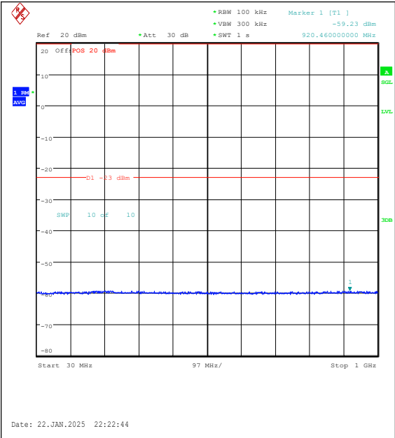
Band25-3MHz-QPSK-26675-1RB#0-30~1000-PA SS
