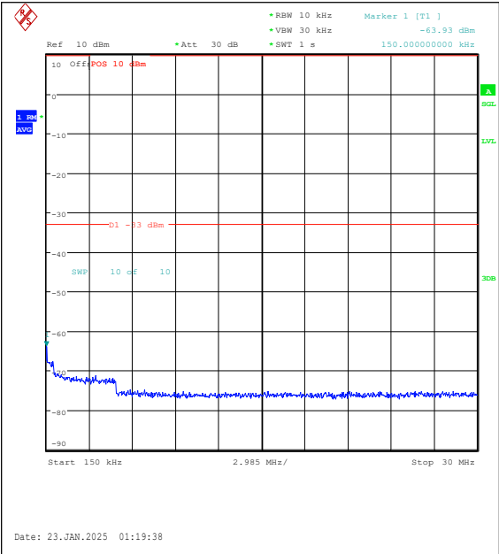
Band25-15MHz-16QAM-26615-1RB#0-0.15~30-P ASS
