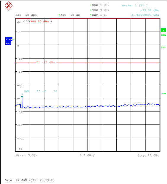
Band25-5MHz-QPSK-26365-25RB#0-3000~2000 0-PASS
