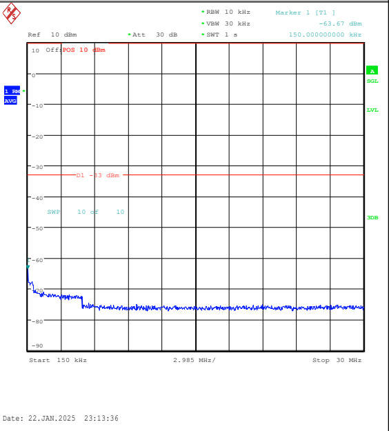
Band25-5MHz-QPSK-26365-1RB#0-0.15~30-PAS S
