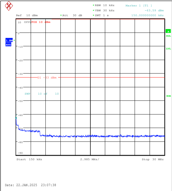
Band25-5MHz-16QAM-26065-1RB#0-0.15~30-PA SS
