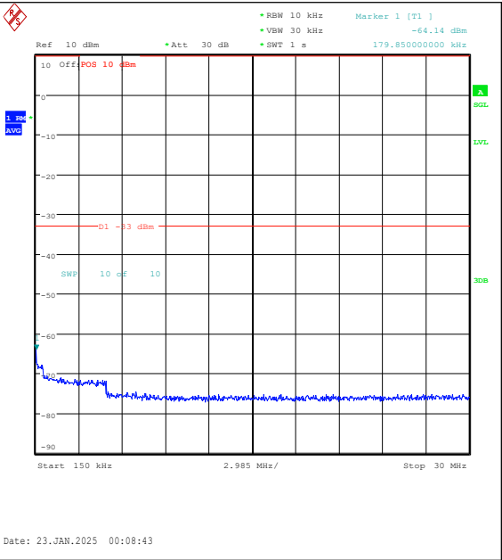
Band25-10MHz-QPSK-26090-50RB#0-0.15~30-PA SS
