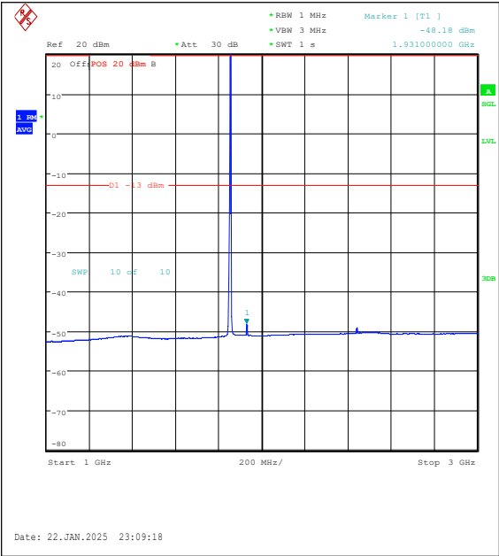
Band25-5MHz-QPSK-26065-1RB#24-1000~3000 -PASS
