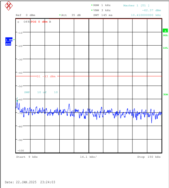
Band25-5MHz-16QAM-26665-1RB#24-0.009~0.1 5-PASS
