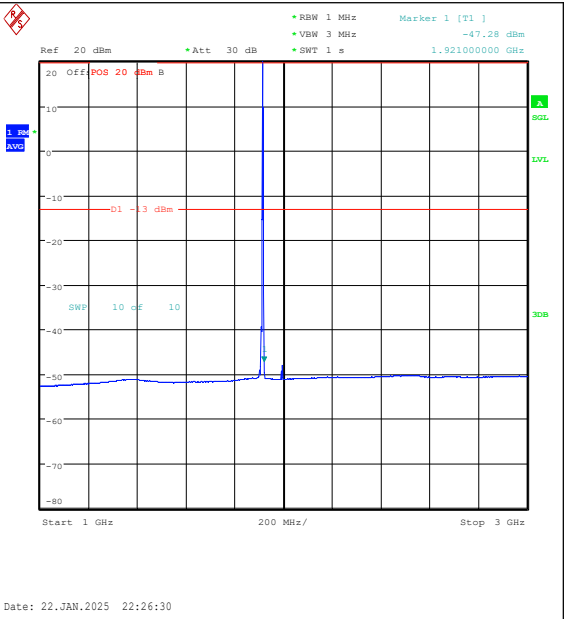
Band25-3MHz-16QAM-26675-1RB#14-1000~3000-PASS
