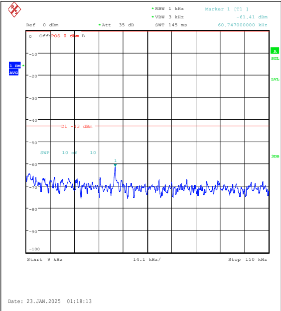
Band25-15MHz-QPSK-26615-1RB#0-0.009~0.15 -PASS
