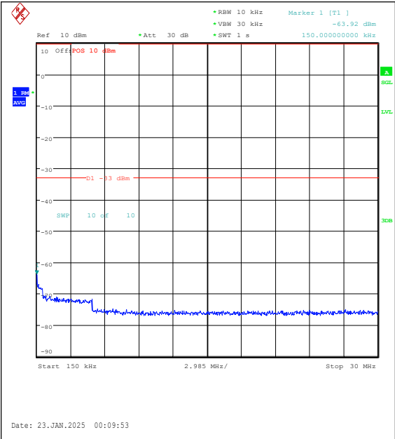
Band25-10MHz-16QAM-26090-50RB#0-0.15~30-PASS
