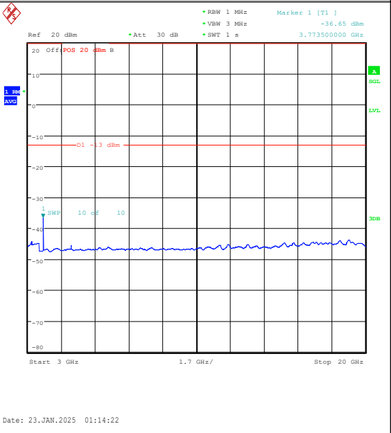
Band25-15MHz-QPSK-26365-1RB#74-3000~2000 0-PASS
