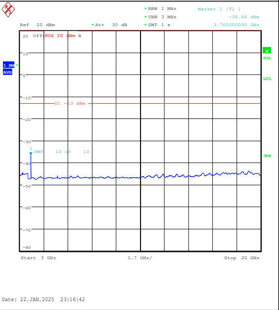
Band25-5MHz-QPSK-26365-1RB#24-3000~20000 -PASS
