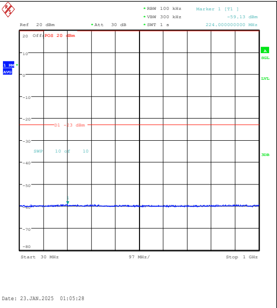
Band25-15MHz-16QAM-26115-1RB#0-30~1000-P ASS
