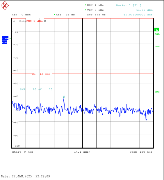
Band25-3MHz-16QAM-26675-15RB#0-0.009~0.15-PASS
