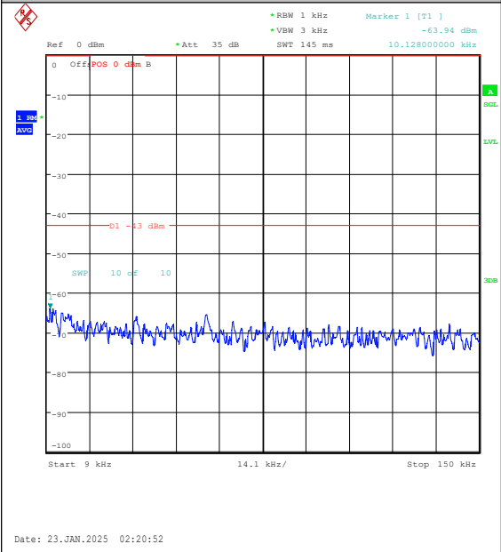
Band25-20MHz-16QAM-26590-1RB#99-0.009~0. 15-PASS
