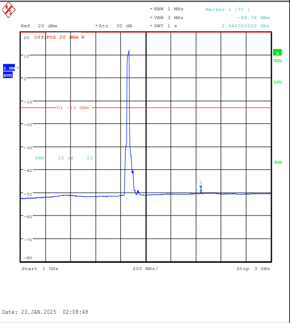
Band25-20MHz-QPSK-26140-100RB#0-1000~3000-PASS
