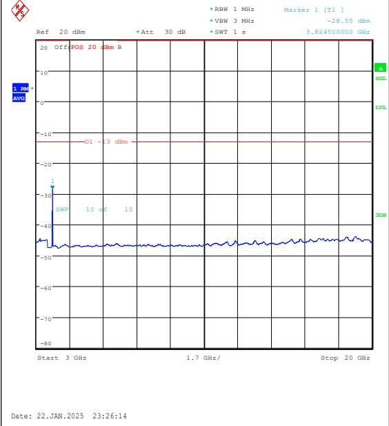
Band25-5MHz-QPSK-26665-25RB#0-3000~2000 0-PASS
