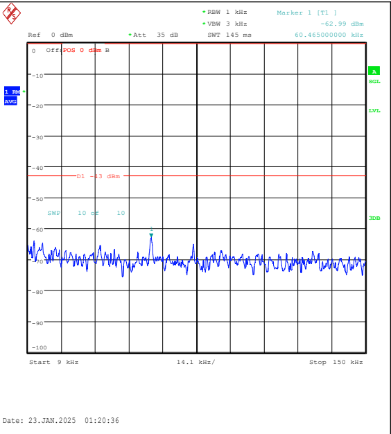
Band25-15MHz-QPSK-26615-1RB#74-0.009~0.15 -PASS
