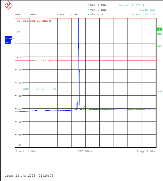
Band25-15MHz-16QAM-26615-1RB#0-1000~300 0-PASS
