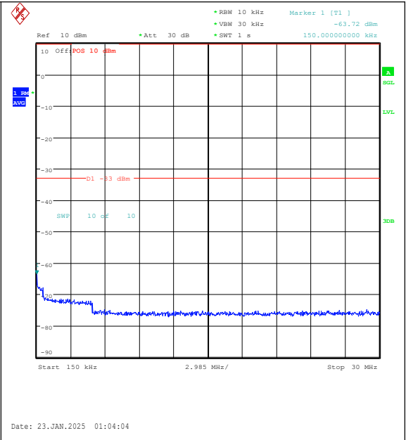
Band25-15MHz-QPSK-26115-1RB#0-0.15~30-PA SS
