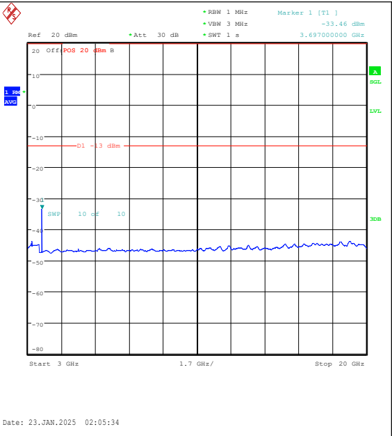
Band25-20MHz-16QAM-26140-1RB#0-3000~2000 0-PASS
