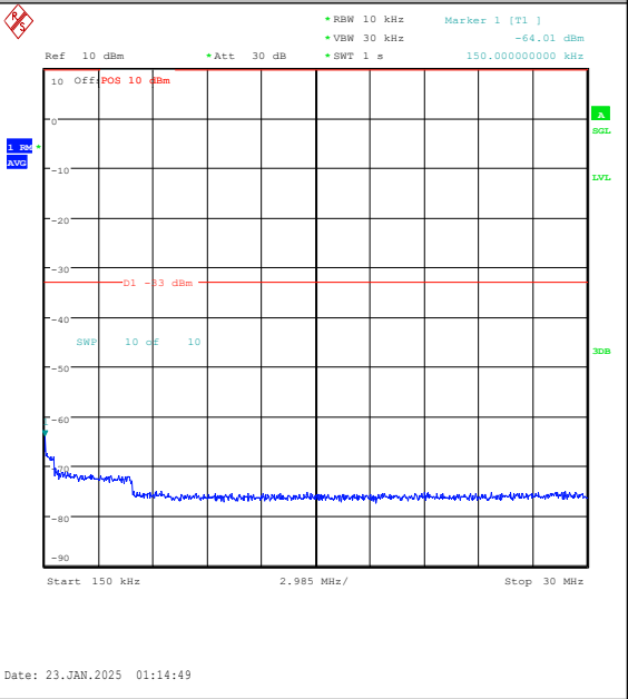
Band25-15MHz-16QAM-26365-1RB#74-0.15~30-P ASS
