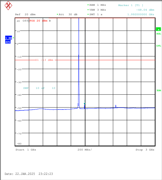
Band25-5MHz-16QAM-26665-1RB#0-1000~3000 -PASS
