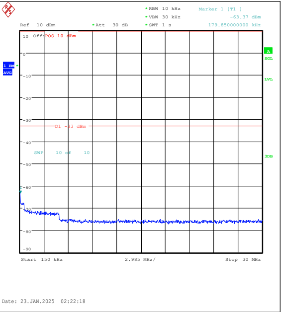
Band25-20MHz-QPSK-26590-100RB#0-0.15~30-P ASS
