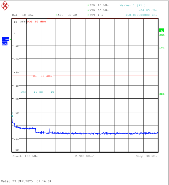
Band25-15MHz-QPSK-26365-75RB#0-0.15~30-PA SS
