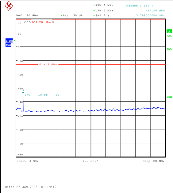
Band25-15MHz-QPSK-26615-1RB#0-3000~2000 0-PASS
