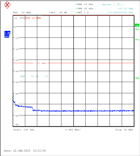
Band25-5MHz-16QAM-26665-1RB#0-0.15~30-PA SS
