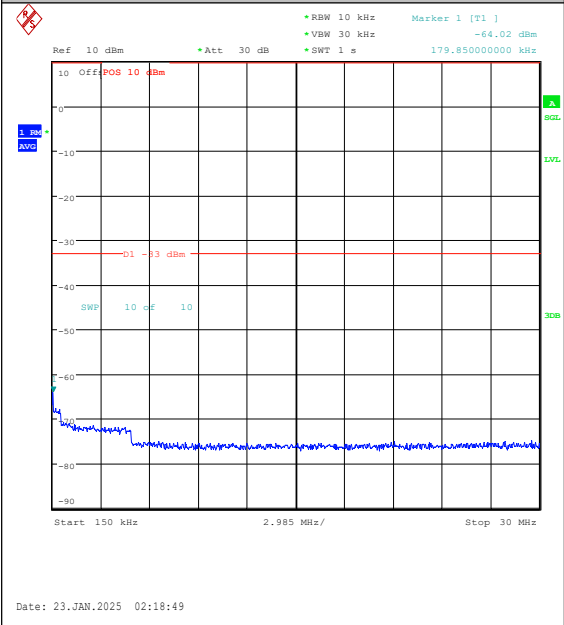
Band25-20MHz-16QAM-26590-1RB#0-0.15~30-PASS
