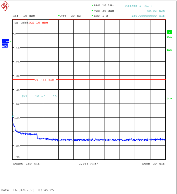
Band4-1.4MHz-16QAM-19957-1RB#5-0.15~30-PA SS
