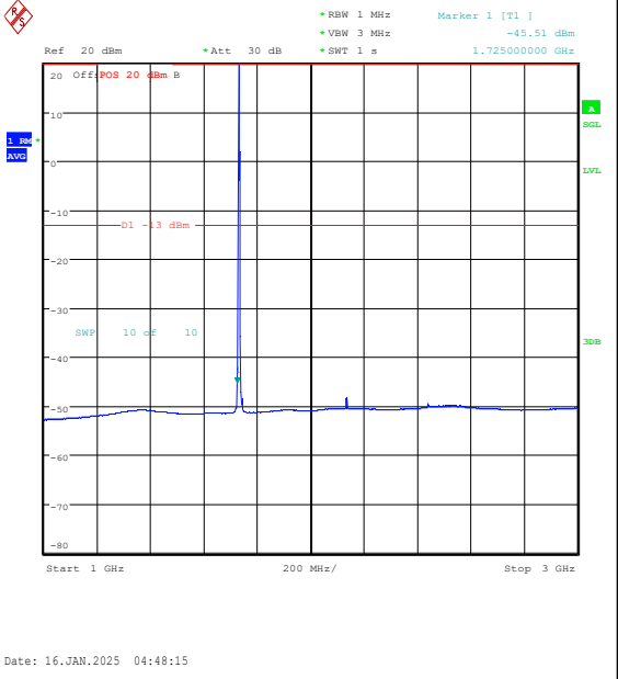
Band4-3MHz-QPSK-20175-1RB#0-1000~3000-PA SS
