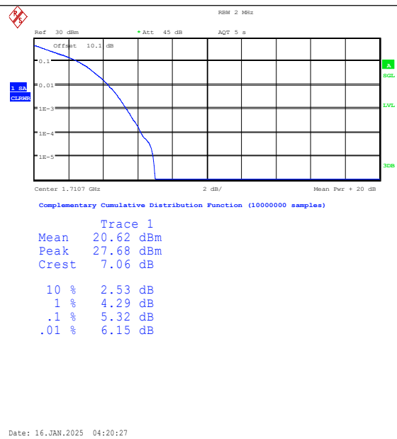
Band4-1.4MHz-QPSK-19957-6RB#0-PASS
