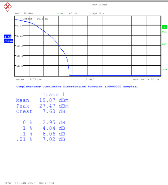
Band4-1.4MHz-16QAM-19957-6RB#0-PASS
