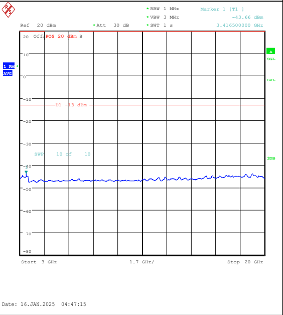
Band4-3MHz-16QAM-19965-15RB#0-3000~20000 -PASS
