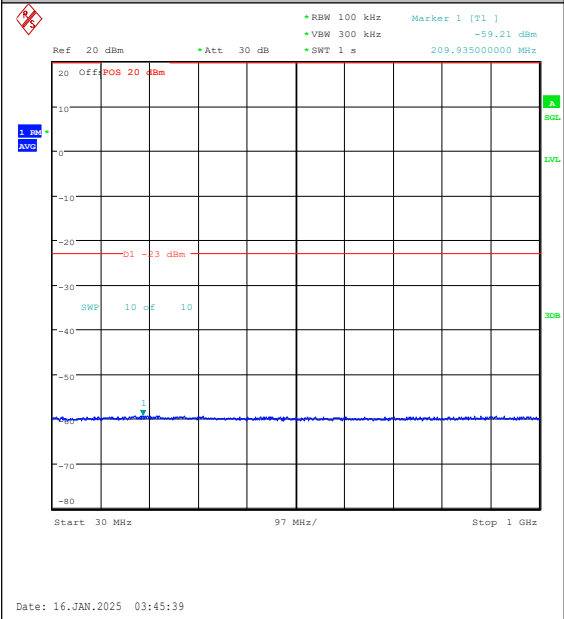
Band4-1.4MHz-16QAM-19957-1RB#5-30~1000-P ASS
