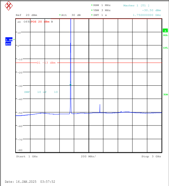
Band4-1.4MHz-16QAM-20393-1RB#0-1000~300 0-PASS
