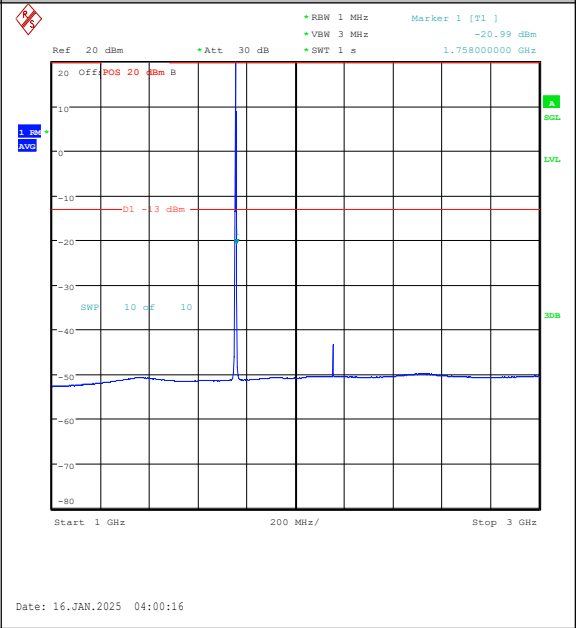
Band4-1.4MHz-16QAM-20393-1RB#5-1000~3000-P PASS
