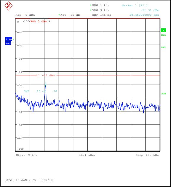
Band4-1.4MHz-16QAM-20393-1RB#0-0.009~0.15- PASS
