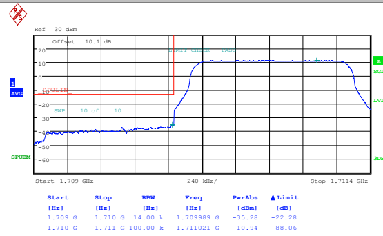
Band4-1.4MHz-QPSK-19957-1RB#0-PASS
