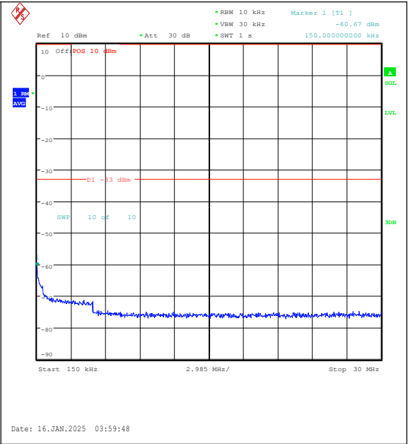
Band4-1.4MHz-16QAM-20393-1RB#5-0.15~30-PA SS
