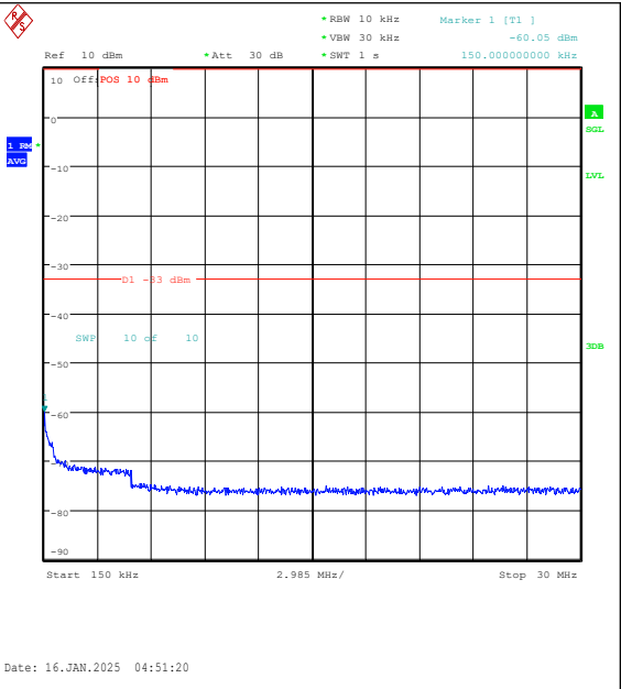
Band4-3MHz-16QAM-20175-1RB#14-0.15~30-PA SS
