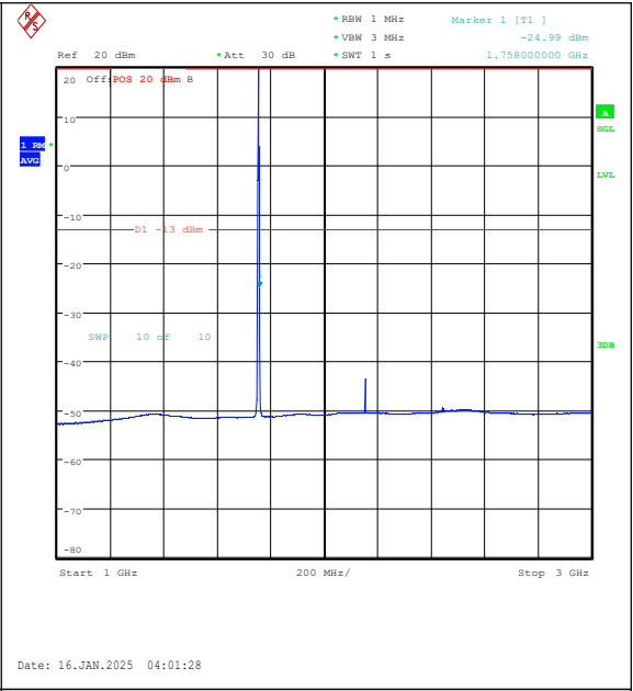
Band4-1.4MHz-QPSK-20393-6RB#0-1000~3000-P ASS
