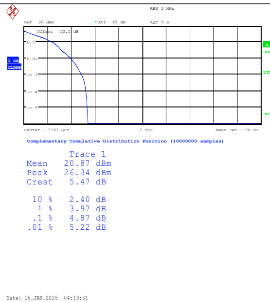
Band4-1.4MHz-QPSK-19957-1RB#0-PASS
