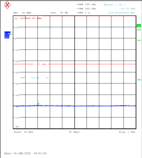
Band4-3MHz-16QAM-20175-1RB#14-30~1000-P ASS
