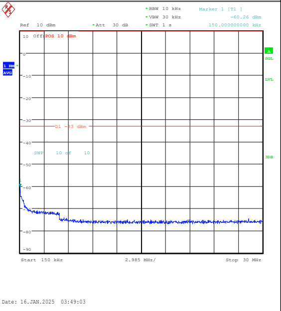
Band4-1.4MHz-QPSK-20175-1RB#0-0.15~30-PAS S
