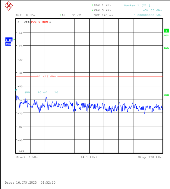
Band4-3MHz-QPSK-20175-15RB#0-0.009~0.15-PASS
