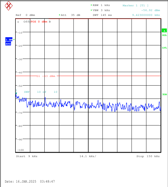
Band4-1.4MHz-QPSK-20175-1RB#0-0.009~0.15- PASS
