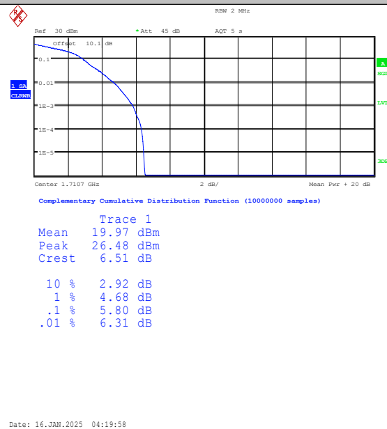
Band4-1.4MHz-16QAM-19957-1RB#0-PASS
