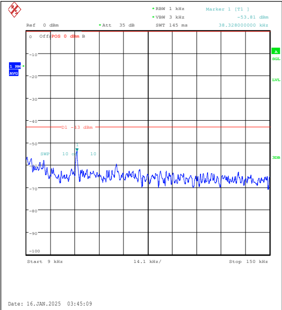
Band4-1.4MHz-16QAM-19957-1RB#5-0.009~0.1 5-PASS
