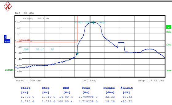
Band4-1.4MHz-QPSK-19957-1RB#5-PASS
