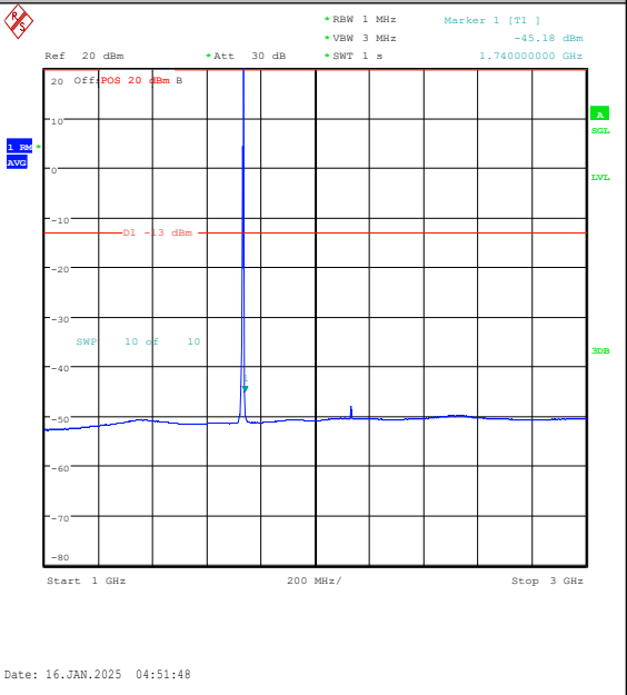
Band4-3MHz-16QAM-20175-1RB#14-1000~3000- PASS
