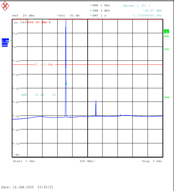
Band4-1.4MHz-16QAM-19957-1RB#5-1000~3000-P PASS
