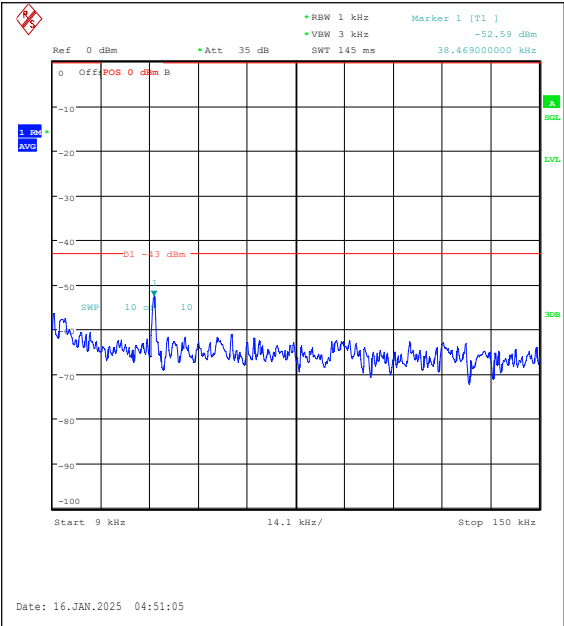
Band4-3MHz-16QAM-20175-1RB#14-0.009~0.15 -PASS
