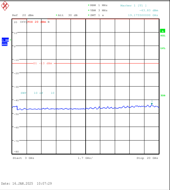
Band4-15MHz-16QAM-20325-1RB#0-3000~20000 -PASS
