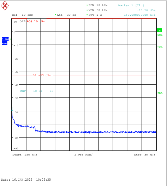
Band4-15MHz-QPSK-20325-1RB#0-0.15~30-PAS S
