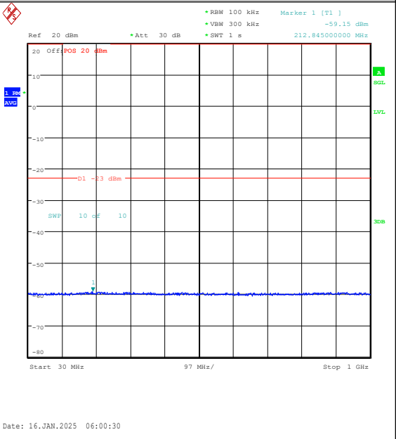
Band4-5MHz-16QAM-20375-25RB#0-30~1000-PA SS
