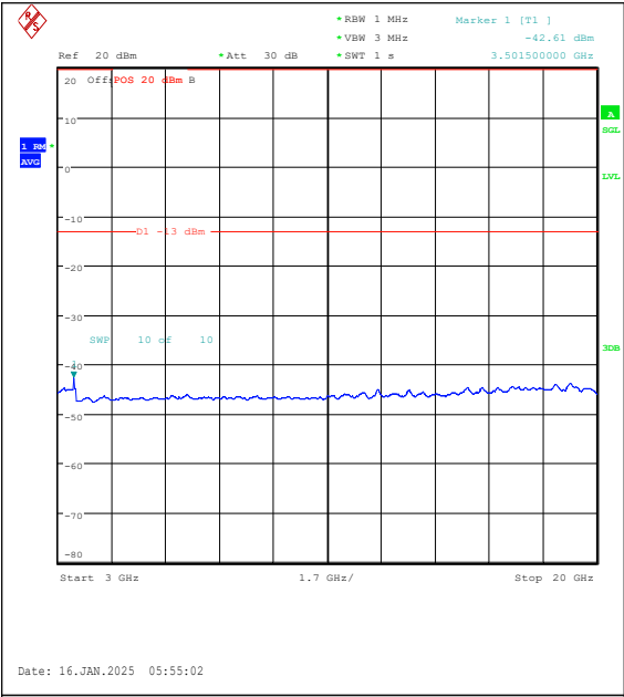
Band4-5MHz-QPSK-20375-1RB#0-3000~20000-PASS
