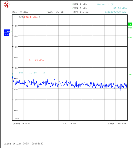
Band4-10MHz-QPSK-20350-1RB#0-0.009~0.15- PASS
