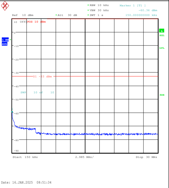
Band4-10MHz-QPSK-20000-1RB#0-0.15~30-PAS S
