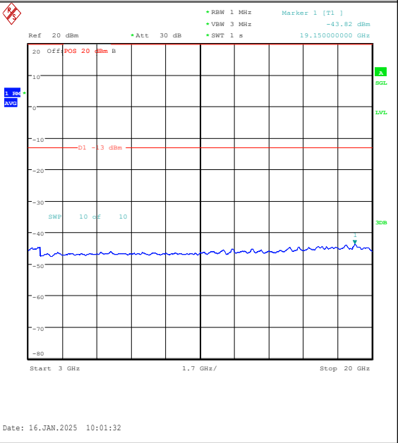
Band4-15MHz-QPSK-20175-1RB#74-3000~20000 -PASS
