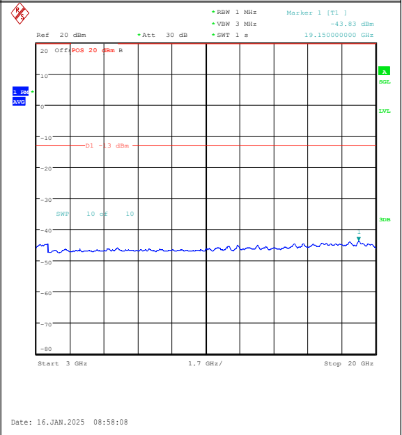
Band4-10MHz-16QAM-20000-50RB#0-3000~2000 0-PASS
