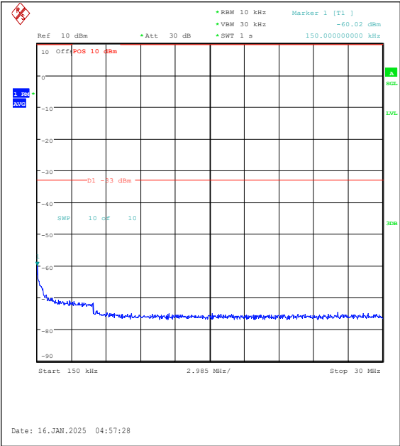
Band4-3MHz-QPSK-20385-1RB#14-0.15~30-PA SS
