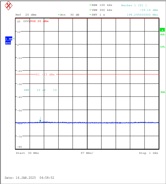
Band4-3MHz-16QAM-20385-1RB#14-30~1000-P ASS
