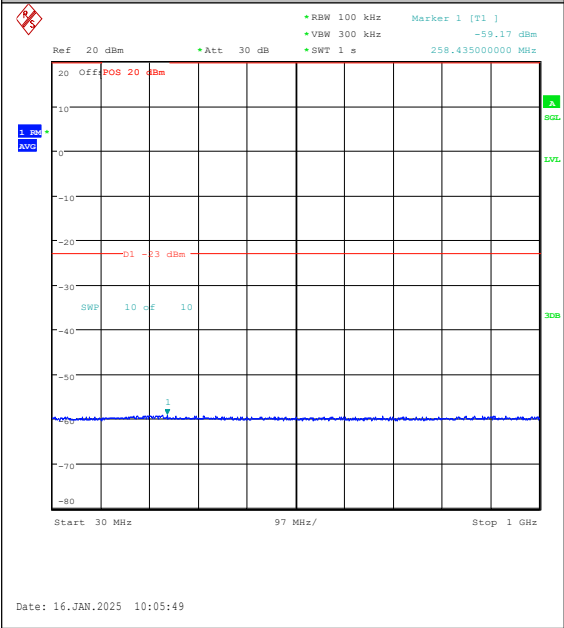
Band4-15MHz-QPSK-20325-1RB#0-30~1000-PA SS
