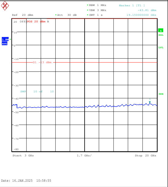
Band4-20MHz-16QAM-20175-1RB#0-3000~20000 -PASS
