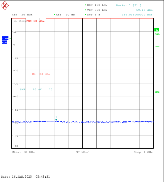
Band4-5MHz-16QAM-20175-1RB#0-30~1000-PAS S
