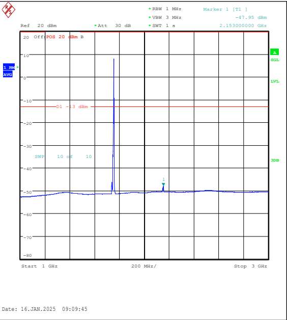
Band4-10MHz-16QAM-20350-1RB#49-1000~3000-PASS
