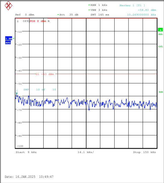
Band4-20MHz-QPSK-20050-1RB#0-0.009~0.15- PASS
