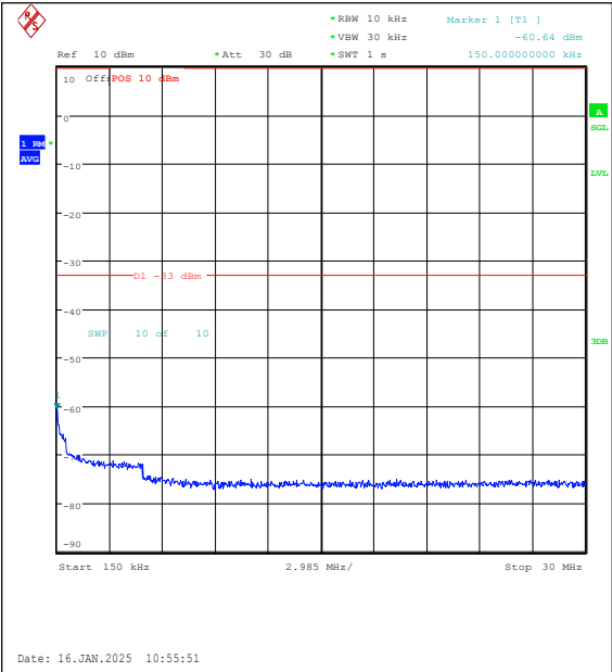
Band4-20MHz-16QAM-20050-100RB#0-0.15~30-PASS
