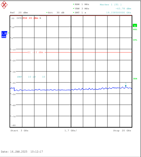
Band4-15MHz-16QAM-20325-75RB#0-3000~2000 0-PASS
