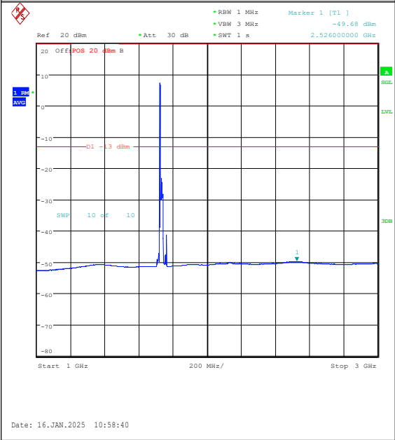
Band4-20MHz-16QAM-20175-1RB#0-1000~3000 -PASS
