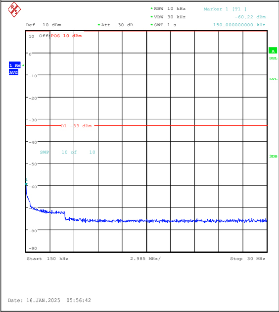
Band4-5MHz-QPSK-20375-1RB#24-0.15~30-PASS
