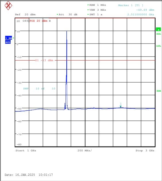
Band4-15MHz-QPSK-20175-1RB#74-1000~3000 -PASS
