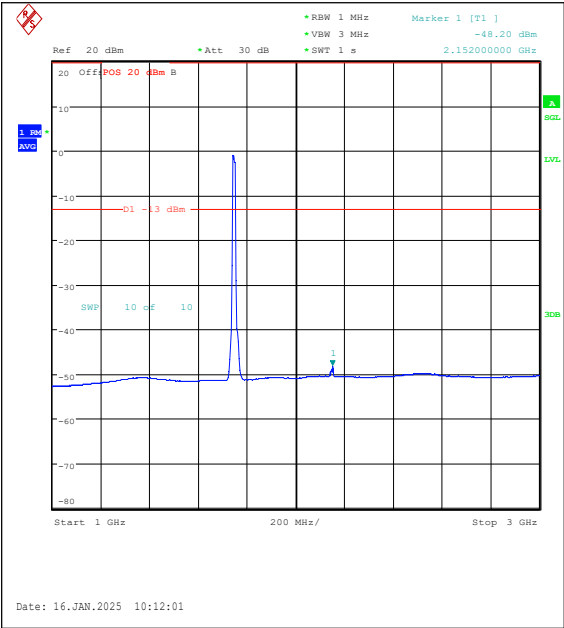
Band4-15MHz-16QAM-20325-75RB#0-1000~300 0-PASS
