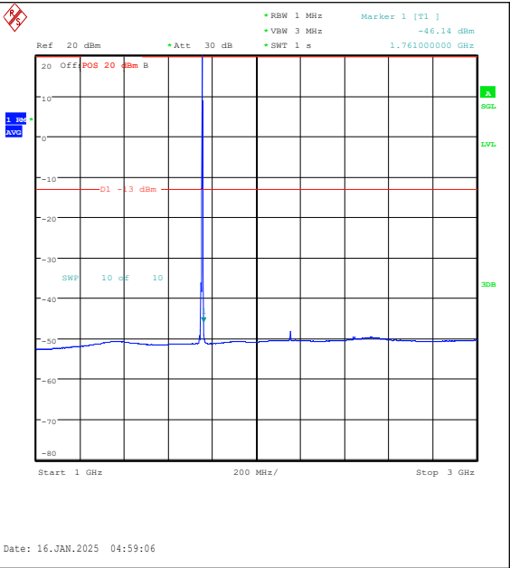
Band4-3MHz-16QAM-20385-1RB#14-1000~3000- PASS
