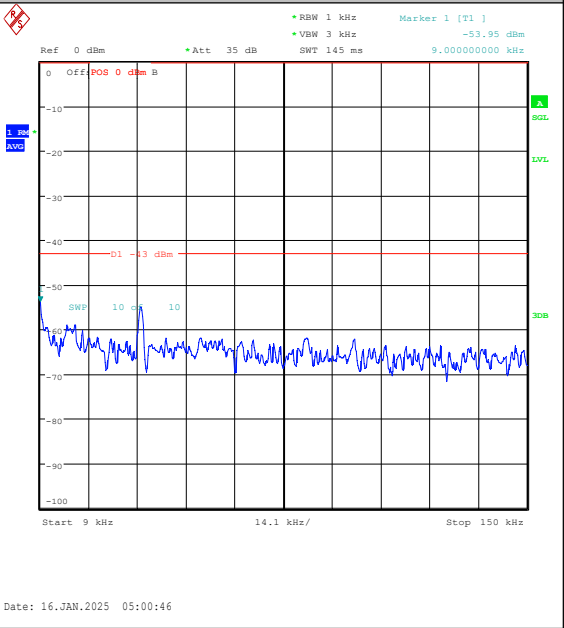
Band4-3MHz-16QAM-20385-15RB#0-0.009~0.15- PASS
