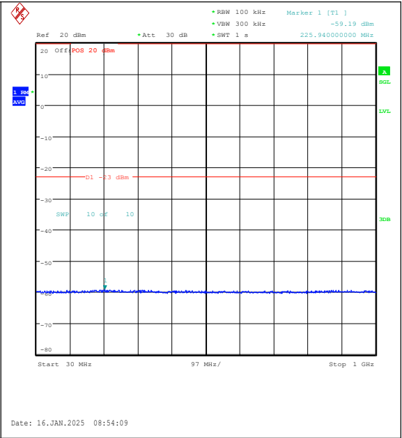
Band4-10MHz-QPSK-20000-1RB#49-30~1000-PA SS
