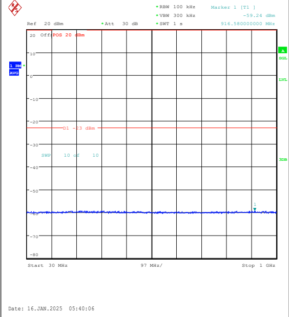
Band4-5MHz-QPSK-19975-1RB#0-30~1000-PAS S
