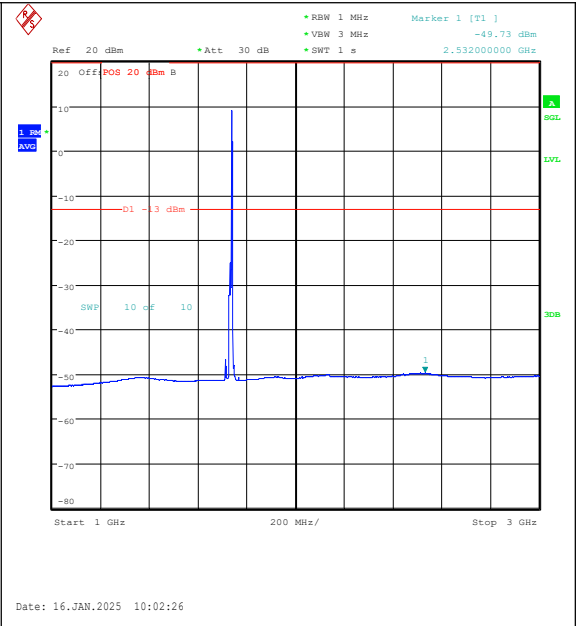
Band4-15MHz-16QAM-20175-1RB#74-1000~3000-PASS
