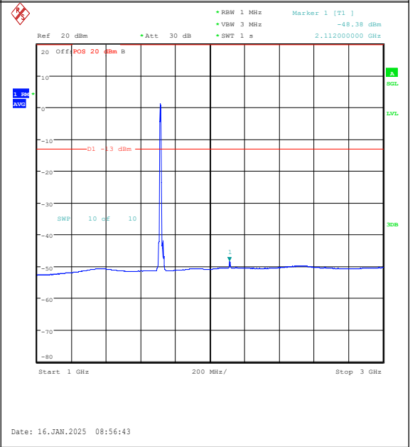
Band4-10MHz-QPSK-20000-50RB#0-1000~3000- PASS
