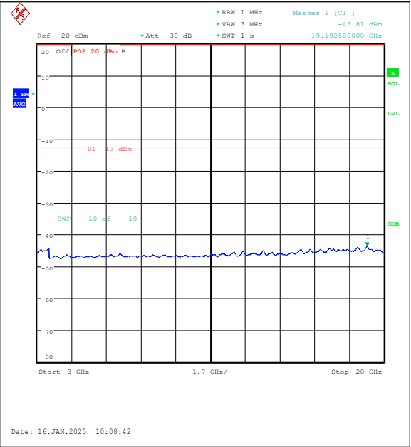
Band4-15MHz-QPSK-20325-1RB#74-3000~20000 -PASS
