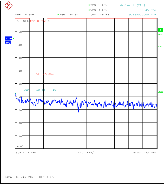
Band4-10MHz-QPSK-20175-1RB#0-0.009~0.15-PASS
