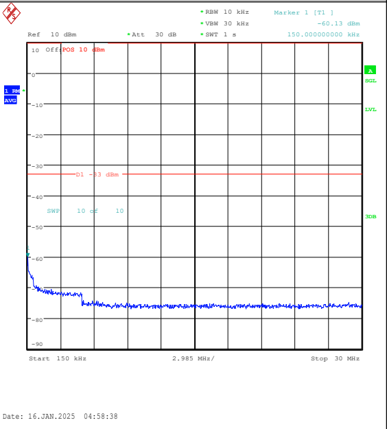
Band4-3MHz-16QAM-20385-1RB#14-0.15~30-PA-SS
