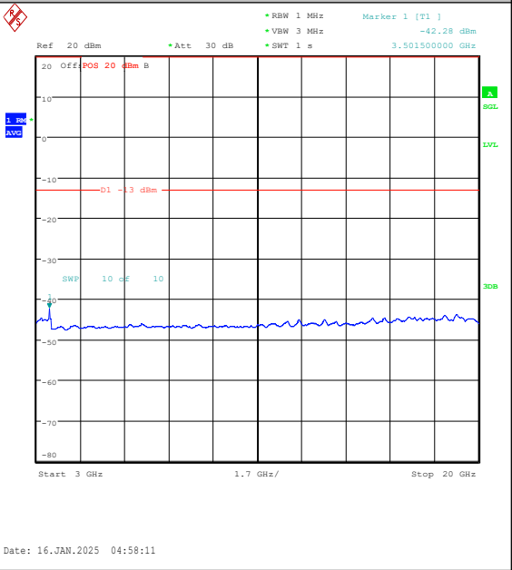
Band4-3MHz-QPSK-20385-1RB#14-3000~20000- PASS
