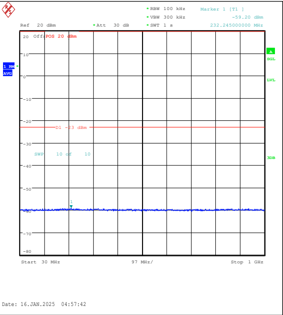
Band4-3MHz-QPSK-20385-1RB#14-30~1000-PAS S
