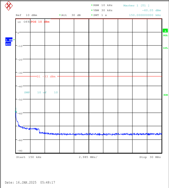
Band4-5MHz-16QAM-20175-1RB#0-0.15~30-PA SS
