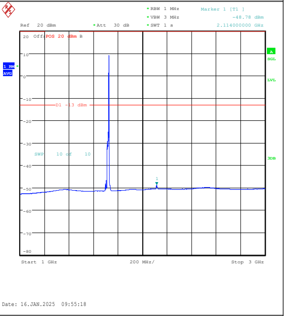
Band4-15MHz-16QAM-20025-1RB#74-1000~3000 -PASS
