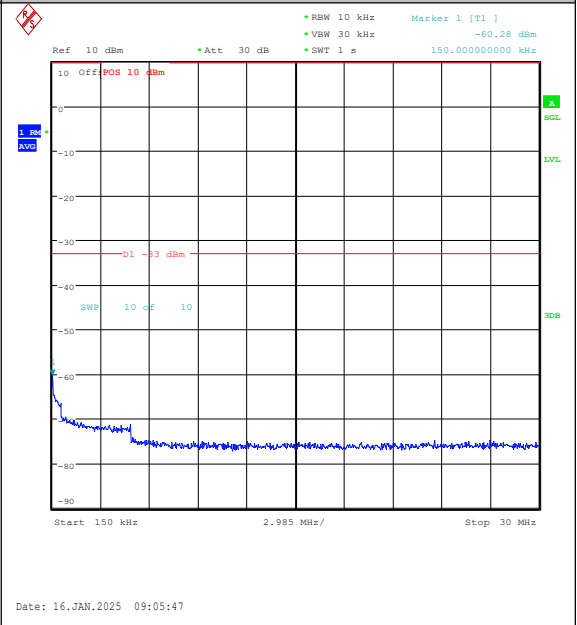
Band4-10MHz-QPSK-20350-1RB#0-0.15~30-PAS S
