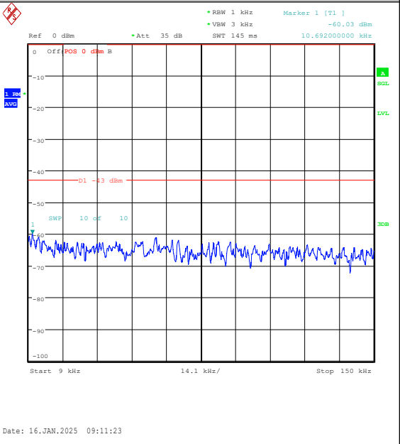
Band4-10MHz-16QAM-20350-50RB#0-0.009~0.15-PASS
