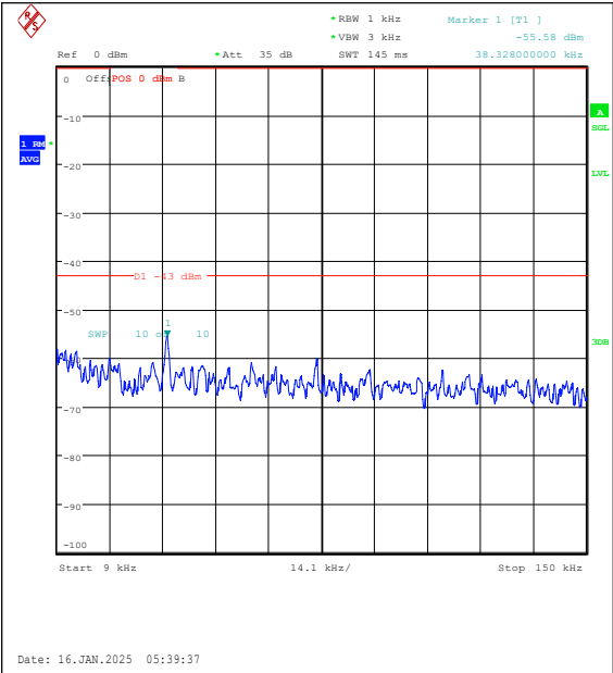
Band4-5MHz-QPSK-19975-1RB#0-0.009~0.15-P ASS
