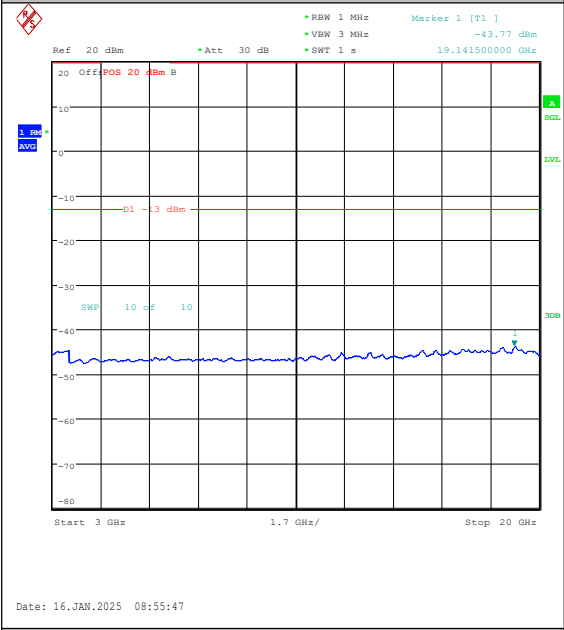
Band4-10MHz-16QAM-20000-1RB#49-3000~20000-PASS
