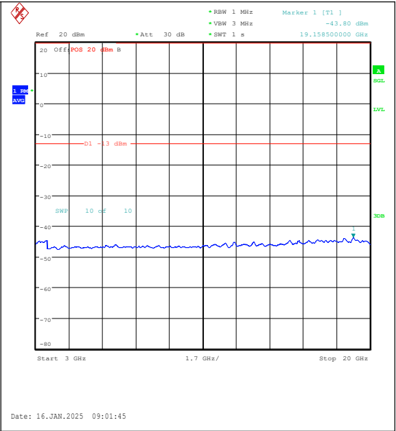
Band4-10MHz-QPSK-20175-1RB#49-3000~20000 -PASS
