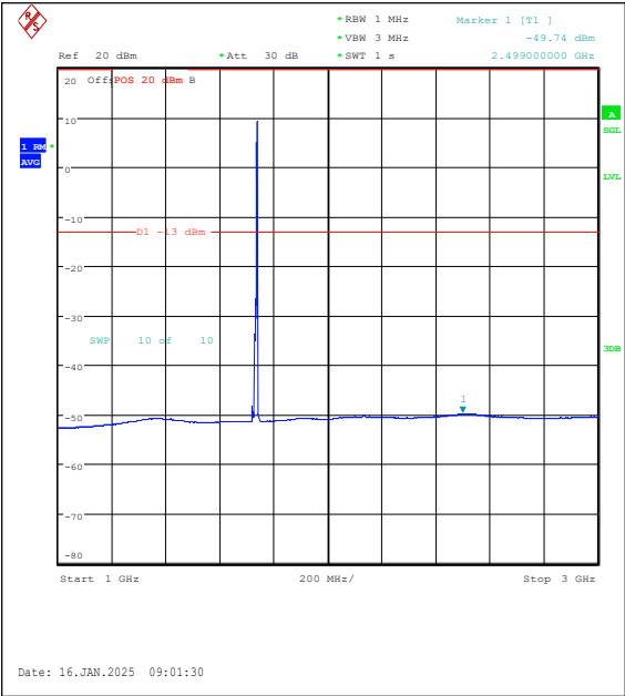
Band4-10MHz-QPSK-20175-1RB#49-1000~3000 -PASS
