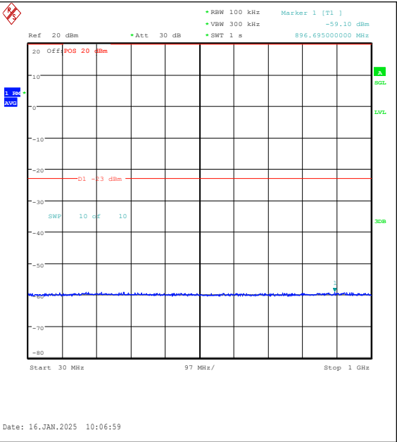
Band4-15MHz-16QAM-20325-1RB#0-30~1000-PA SS
