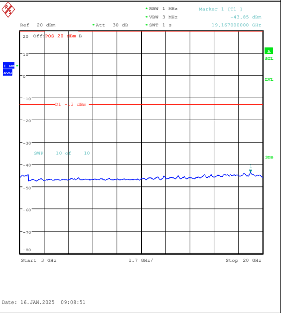
Band4-10MHz-QPSK-20350-1RB#49-3000~20000 -PASS
