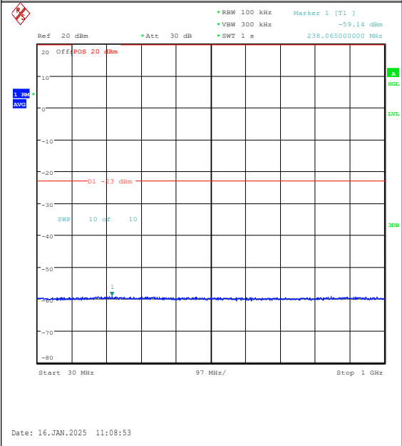
Band4-20MHz-QPSK-20300-100RB#0-30~1000- PASS
