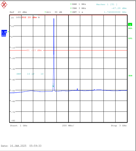
Band4-5MHz-QPSK-20375-25RB#0-1000~3000-P ASS
