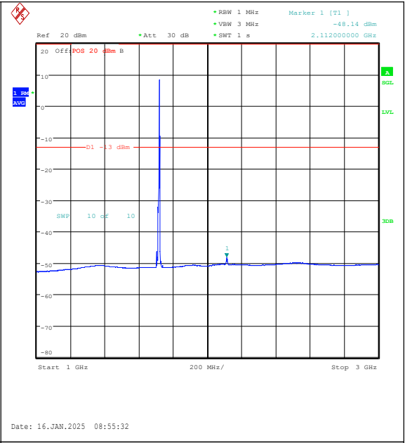
Band4-10MHz-16QAM-20000-1RB#49-1000~3000-PASS
