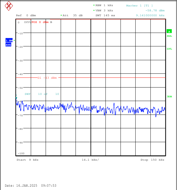
Band4-10MHz-QPSK-20350-1RB#49-0.009~0.15- PASS
