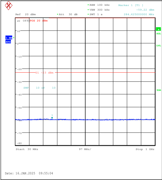
Band4-15MHz-16QAM-20025-1RB#74-30~1000- PASS
