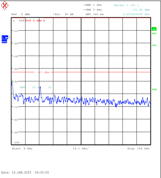
Band4-5MHz-16QAM-20375-25RB#0-0.009~0.15- PASS
