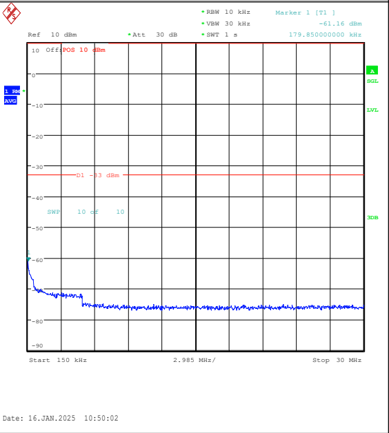
Band4-20MHz-QPSK-20050-1RB#0-0.15~30-PAS S
