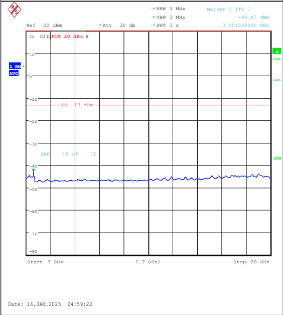
Band4-3MHz-16QAM-20385-1RB#14-3000~2000 0-PASS
