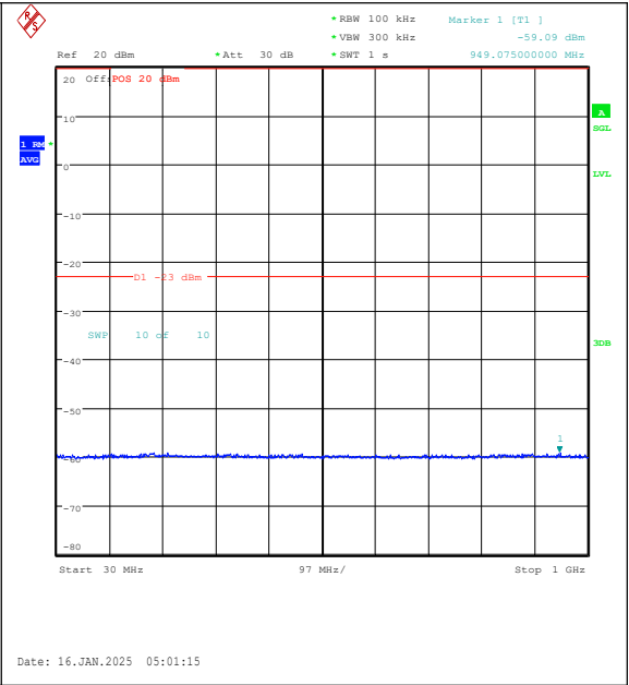
Band4-3MHz-16QAM-20385-15RB#0-30~1000-PA SS
