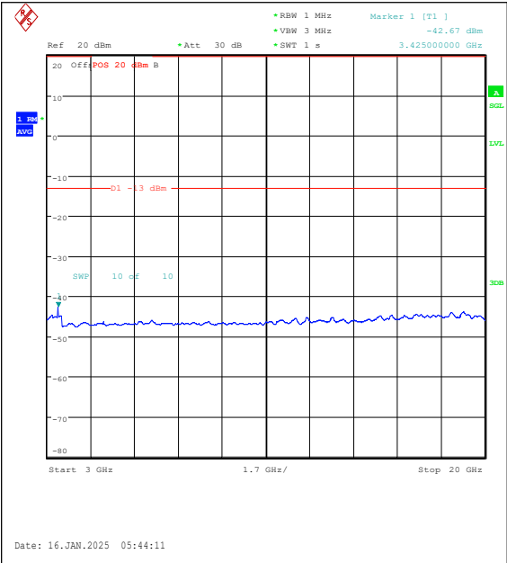
Band4-5MHz-16QAM-19975-1RB#24-3000~2000 0-PASS
