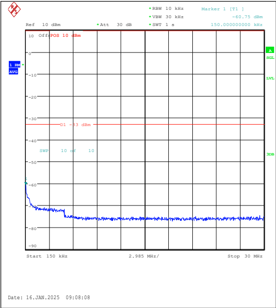
Band4-10MHz-QPSK-20350-1RB#49-0.15~30-PA SS
