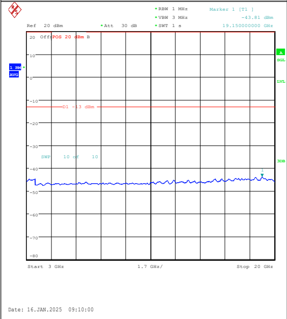
Band4-10MHz-16QAM-20350-1RB#49-3000~20000-PASS
