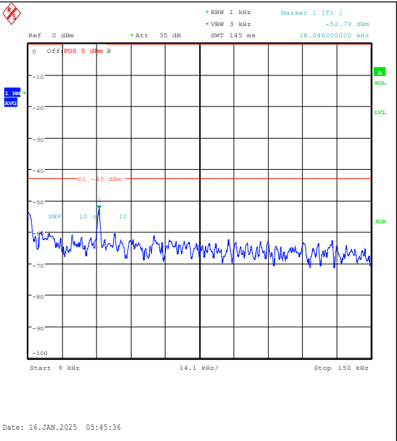
Band4-5MHz-16QAM-19975-25RB#0-0.009~0.15- PASS
