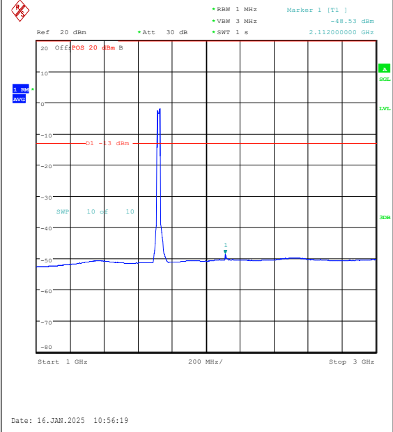
Band4-20MHz-16QAM-20050-100RB#0-1000~3000-PASS
