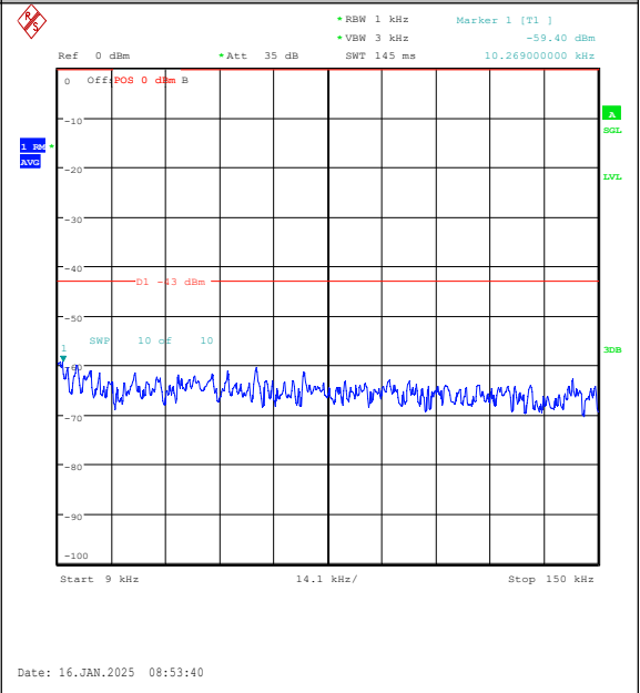
Band4-10MHz-QPSK-20000-1RB#49-0.009~0.15- PASS
