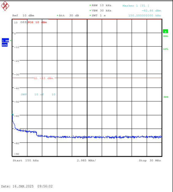
Band4-15MHz-QPSK-20025-75RB#0-0.15~30-PA SS
