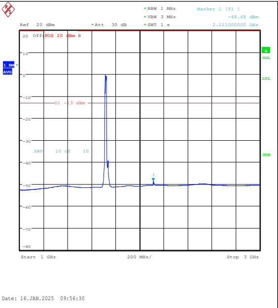
Band4-15MHz-QPSK-20025-75RB#0-1000~3000- PASS
