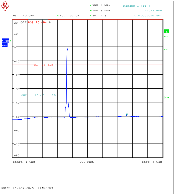
Band4-20MHz-QPSK-20175-100RB#0-1000~3000-PASS
