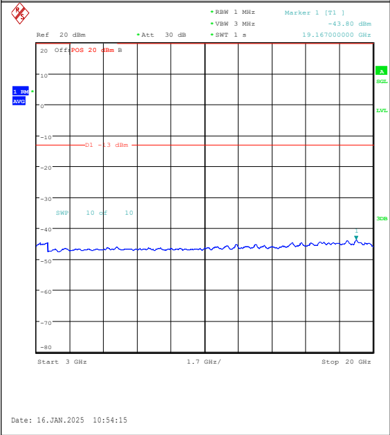
Band4-20MHz-16QAM-20050-1RB#99-3000~20000-PASS
