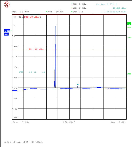
Band4-10MHz-QPSK-20350-1RB#49-1000~3000 -PASS
