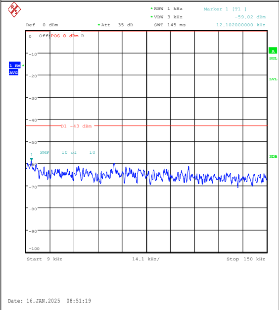
Band4-10MHz-QPSK-20000-1RB#0-0.009~0.15- PASS
