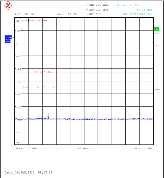
Band4-10MHz-16QAM-20000-50RB#0-30~1000-P ASS
