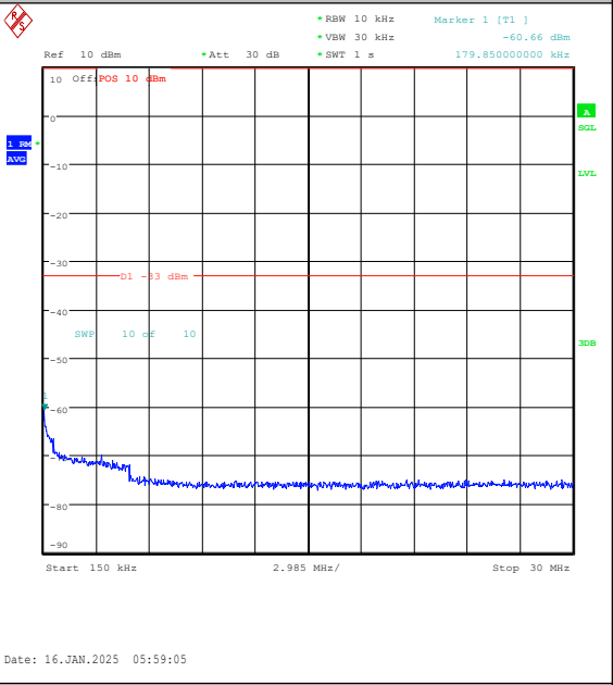
Band4-5MHz-QPSK-20375-25RB#0-0.15~30-PAS
