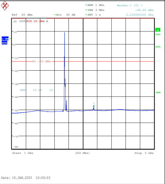
Band4-15MHz-QPSK-20325-1RB#0-1000~3000-P ASS
