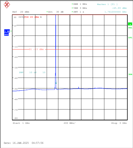
Band4-3MHz-QPSK-20385-1RB#14-1000~3000- PASS
