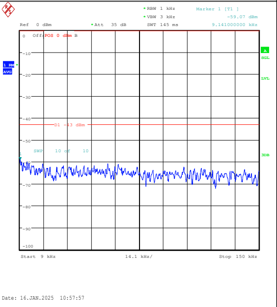
Band4-20MHz-16QAM-20175-1RB#0-0.009~0.15-PASS
