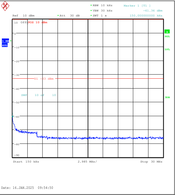
Band4-15MHz-16QAM-20025-1RB#74-0.15~30-P ASS
