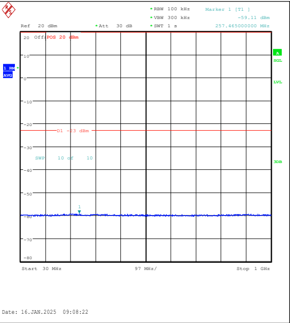
Band4-10MHz-QPSK-20350-1RB#49-30~1000-PA SS
