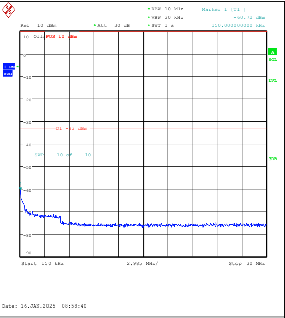
Band4-10MHz-QPSK-20175-1RB#0-0.15~30-PAS
