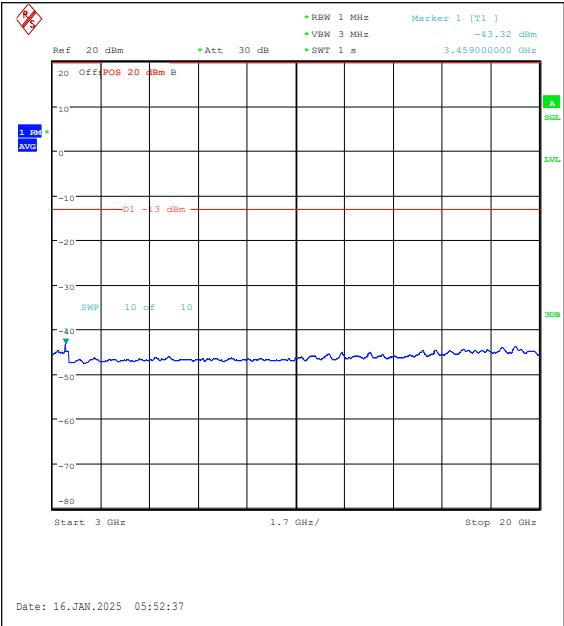
Band4-5MHz-QPSK-20175-25RB#0-3000~20000 -PASS
