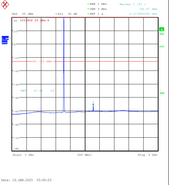
Band4-5MHz-QPSK-19975-1RB#0-1000~3000-PA SS
