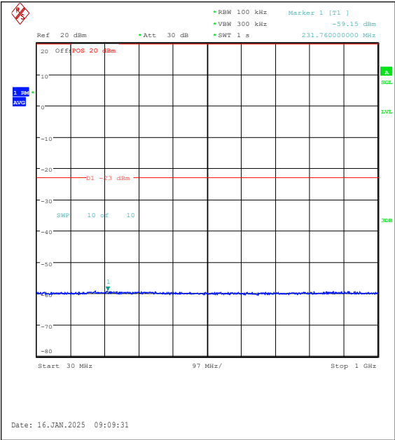
Band4-10MHz-16QAM-20350-1RB#49-30~1000-PASS
