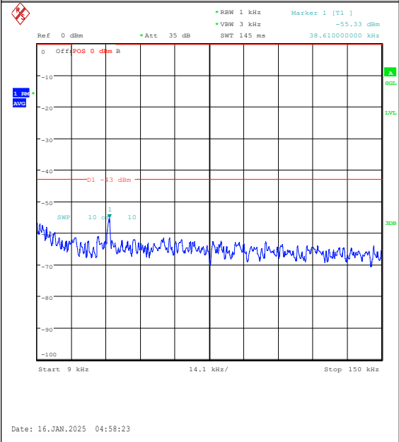
Band4-3MHz-16QAM-20385-1RB#14-0.009~0.15-PASS
