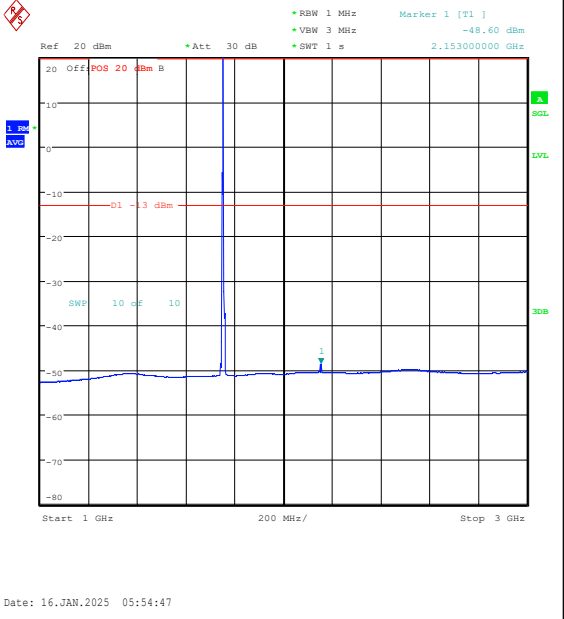
Band4-5MHz-QPSK-20375-1RB#0-1000~3000-PASS SS
