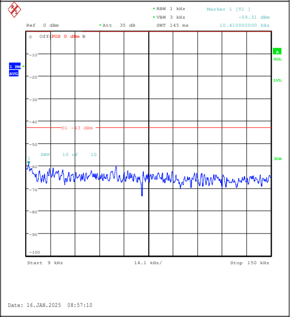
Band4-10MHz-16QAM-20000-50RB#0-0.009~0.15-PASS
