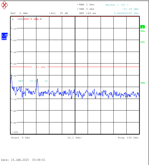
Band4-5MHz-16QAM-20175-1RB#0-0.009~0.15-P ASS
