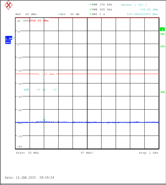
Band4-10MHz-QPSK-20175-1RB#0-30~1000-PA
