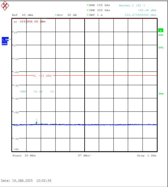
Band4-20MHz-QPSK-20050-1RB#99-30~1000-PA SS
