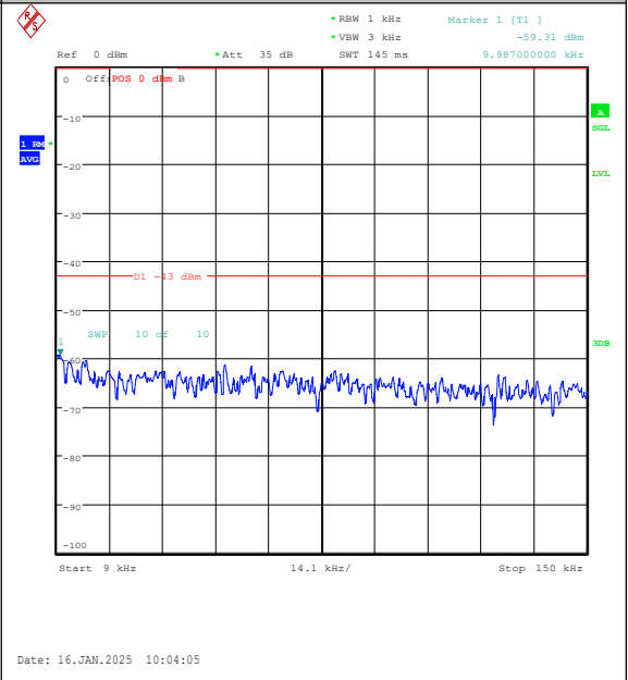
Band4-15MHz-16QAM-20175-75RB#0-0.009~0.15-PASS
