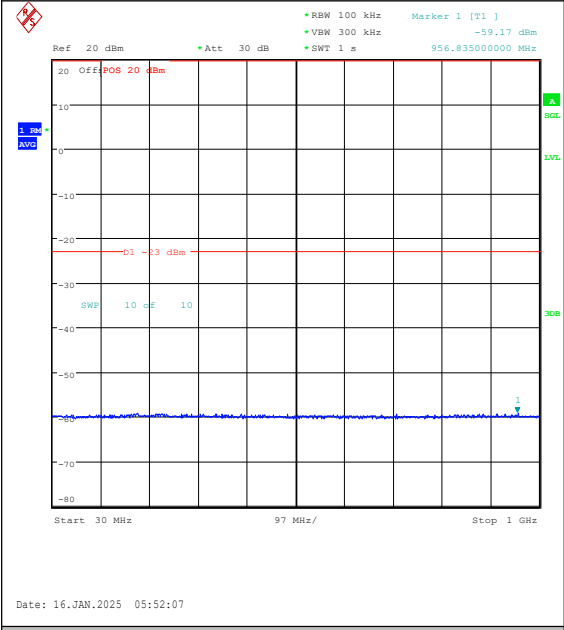
Band4-5MHz-QPSK-20175-25RB#0-30~1000-PA
