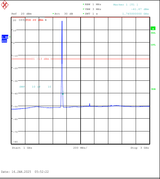
Band4-5MHz-QPSK-20175-25RB#0-1000~3000-P
