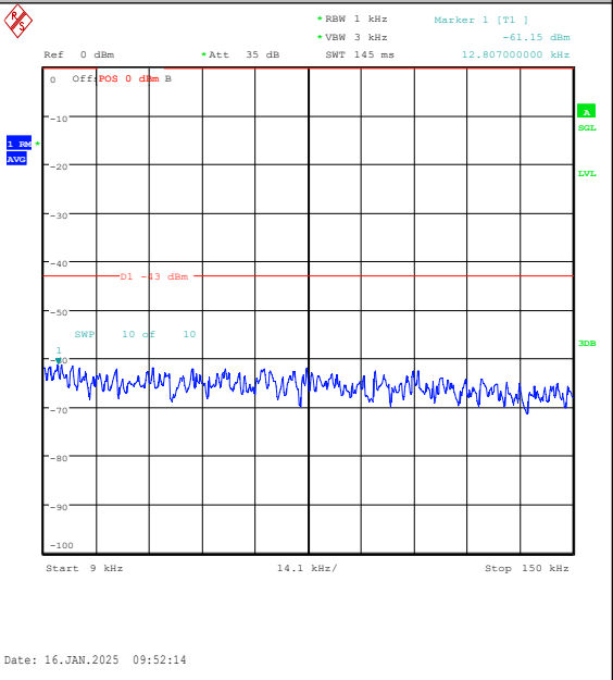
Band4-15MHz-16QAM-20025-1RB#0-0.009~0.15- PASS
