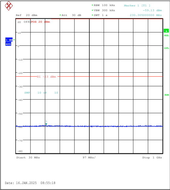
Band4-10MHz-16QAM-20000-1RB#49-30~1000-PASS
