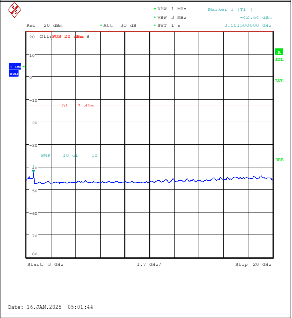
Band4-3MHz-16QAM-20385-15RB#0-3000~20000 -PASS
