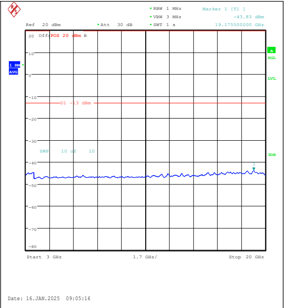
Band4-10MHz-16QAM-20175-50RB#0-3000~2000 0-PASS
