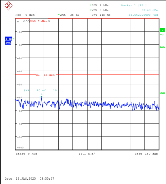
Band4-15MHz-QPSK-20025-75RB#0-0.009~0.15 -PASS
