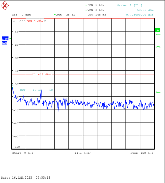
Band4-5MHz-16QAM-20375-1RB#0-0.009~0.15-P ASS
