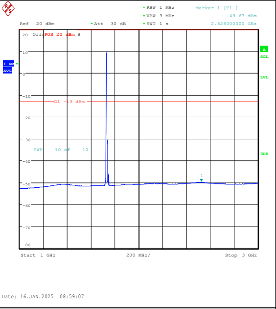
Band4-10MHz-QPSK-20175-1RB#0-1000~3000-P
