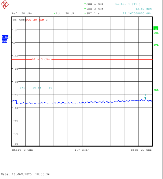
Band4-20MHz-16QAM-20050-100RB#0-3000~20000-PASS
