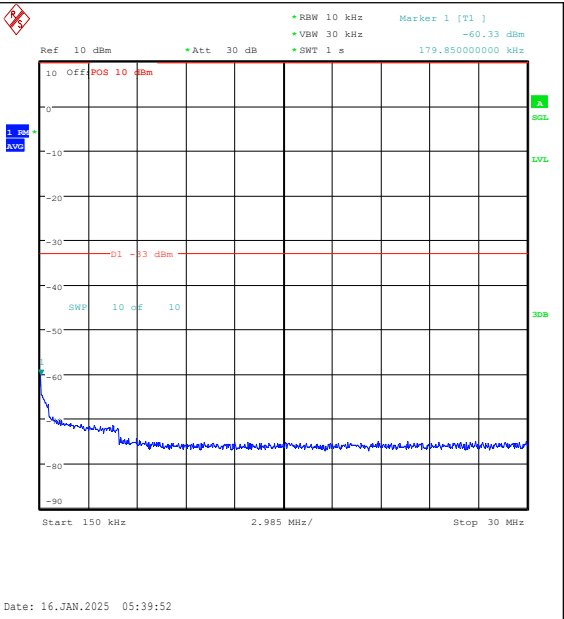
Band4-5MHz-QPSK-19975-1RB#0-0.15~30-PASS
