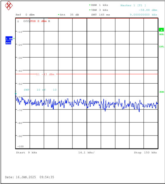
Band4-15MHz-16QAM-20025-1RB#74-0.009~0.1 5-PASS
