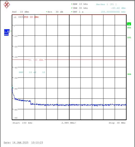
Band4-15MHz-QPSK-20325-75RB#0-0.15~30-PA SS
