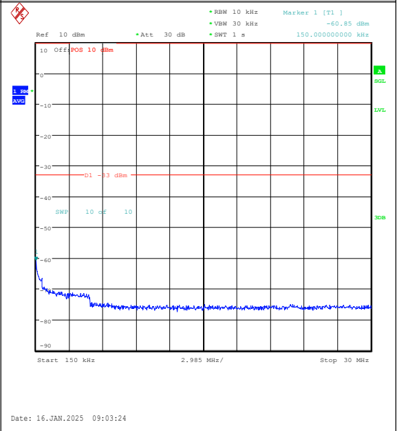
Band4-10MHz-QPSK-20175-50RB#0-0.15~30-PA SS
