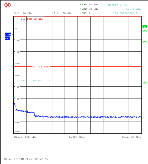
Band4-5MHz-16QAM-19975-25RB#0-0.15~30-PA SS
