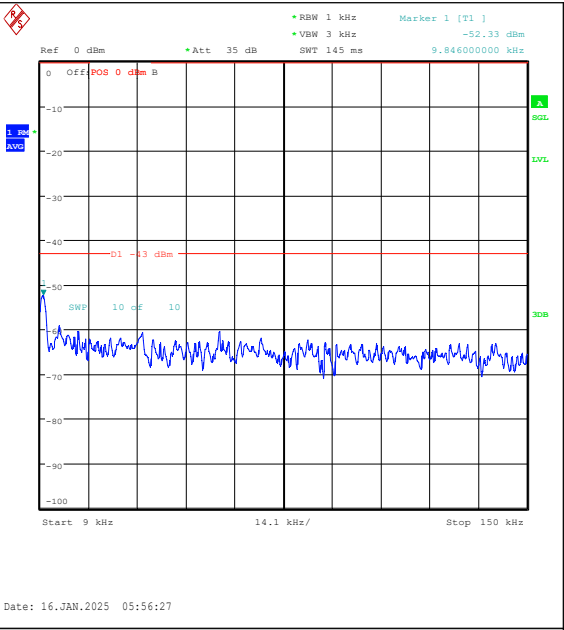
Band4-5MHz-QPSK-20375-1RB#24-0.009~0.15-PASS
