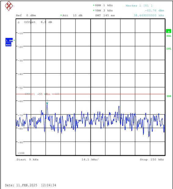
Band41(2535-2655)-15MHz-QPSK-41165-1RB#0-0.009~0.15-PASS
