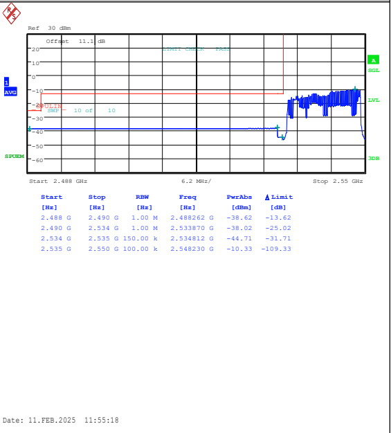
Band41(2535-2655)-15MHz-16QAM-40115-75RB# 0-PASS
