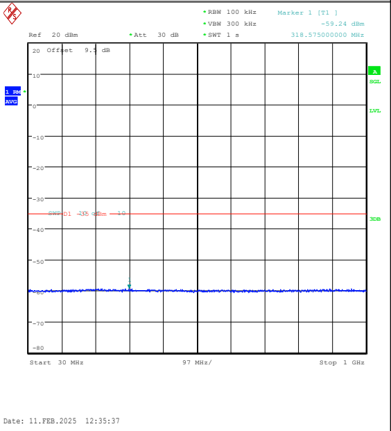
Band41(2535-2655)-20MHz-16QAM-40590-1RB#0 -30~1000-PASS
