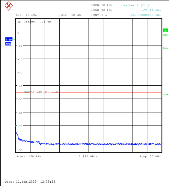
Band41(2535-2655)-20MHz-16QAM-40590-1RB#0 0-0.15~30-PASS
