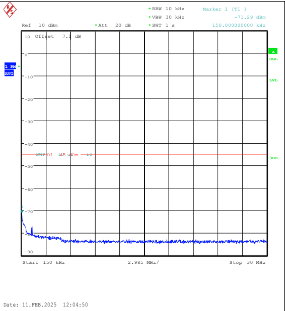
Band41(2535-2655)-15MHz-QPSK-41165-1RB#0-0.15~30-PASS
