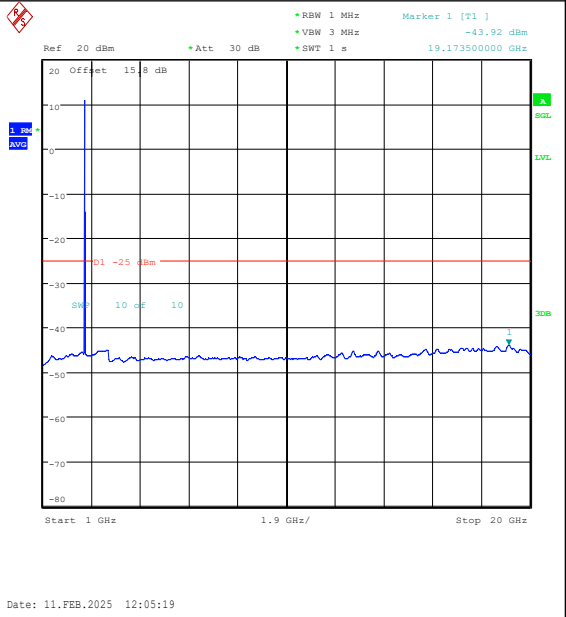
Band41(2535-2655)-15MHz-QPSK-41165-1RB#0-1000~20000-PASS
