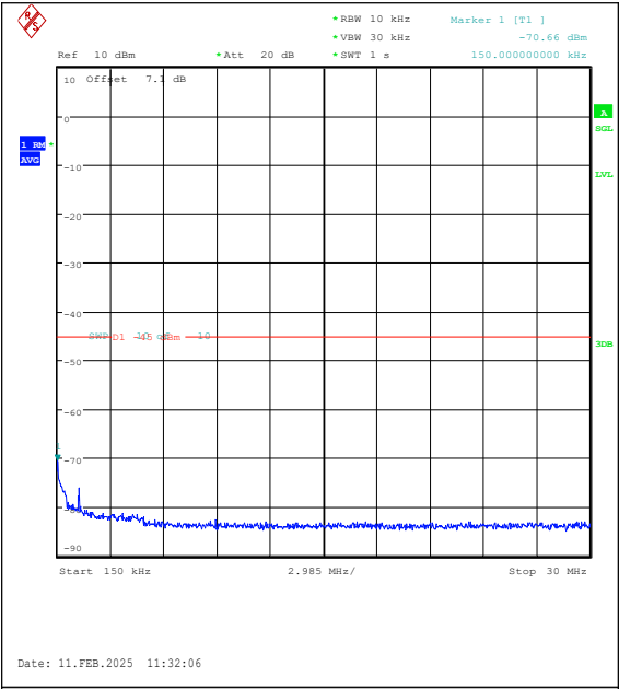
Band41(2535-2655)-10MHz-16QAM-41190-1RB# 0-0.15~30-PASS
