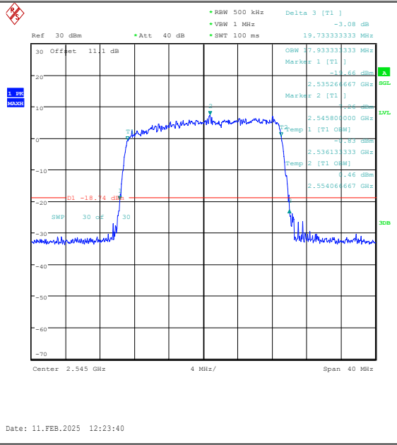
Band41(2535-2655)-20MHz-16QAM-40140-100RB #0-PASS
