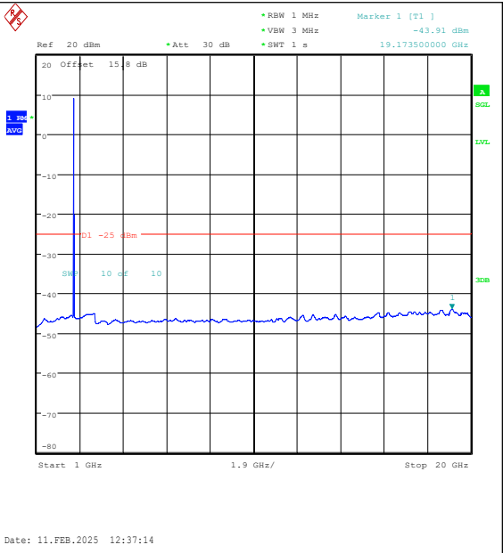
Band41(2535-2655)-20MHz-QPSK-41140-1RB#0-1000~20000-PASS
