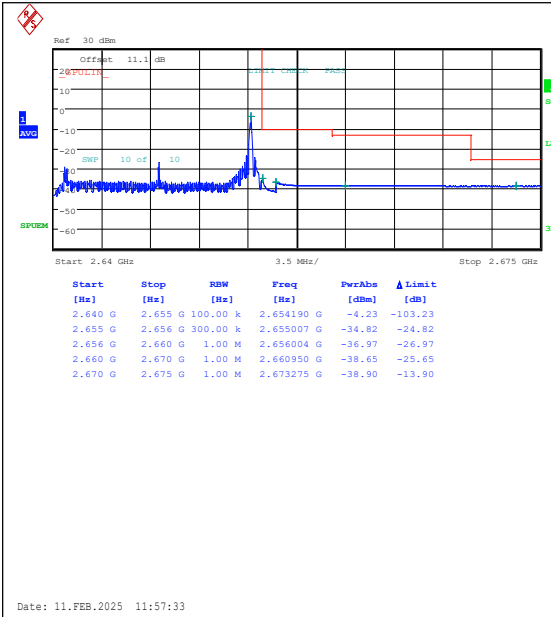
Band41(2535-2655)-15MHz-16QAM-41165-1RB# 74-PASS
