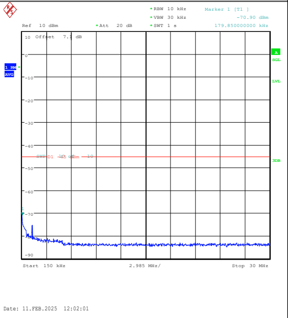
Band41(2535-2655)-15MHz-QPSK-40590-1RB#0- 0.15~30-PASS
