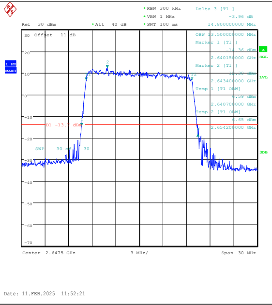
Band41(2535-2655)-15MHz-16QAM-41165-75RB# 0-PASS
