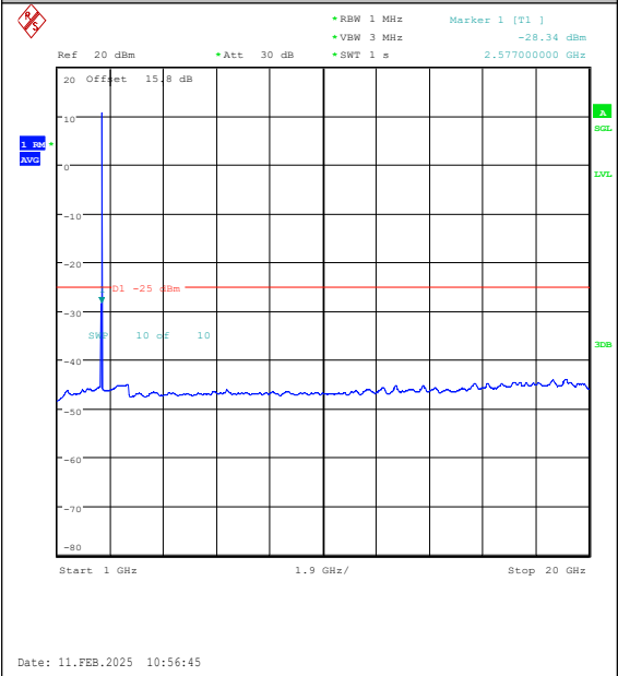
Band41(2535-2655)-5MHz-16QAM-40590-1RB#0 -1000~20000-PASS
