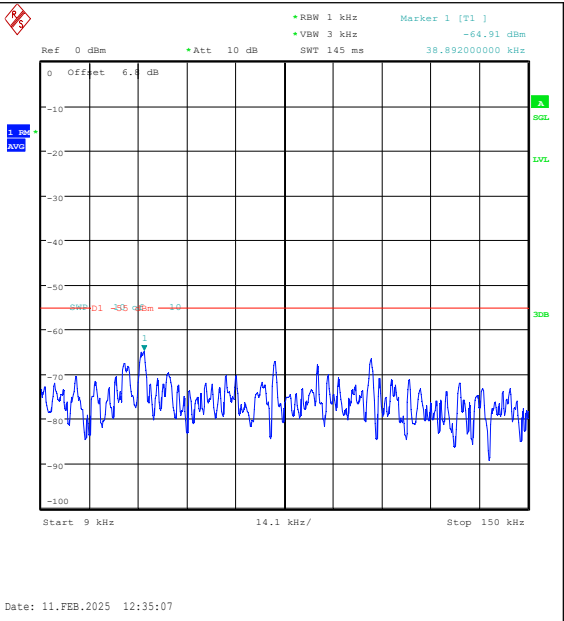
Band41(2535-2655)-20MHz-16QAM-40590-1RB#0 -0.009~0.15-PASS
