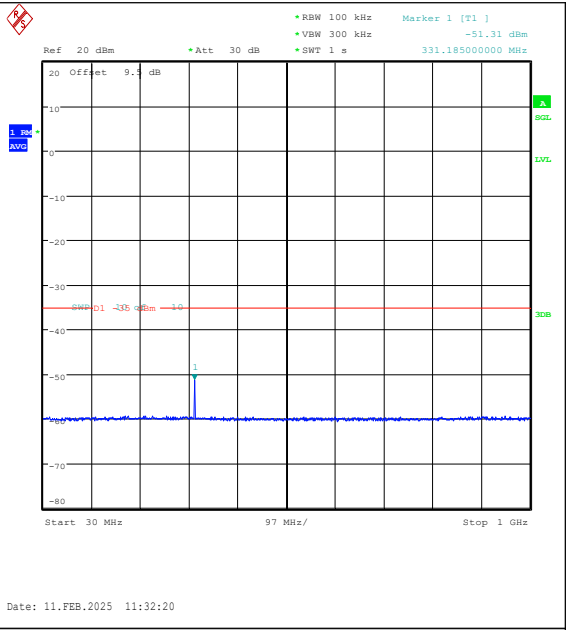
Band41(2535-2655)-10MHz-16QAM-41190-1RB#0 -30~1000-PASS
