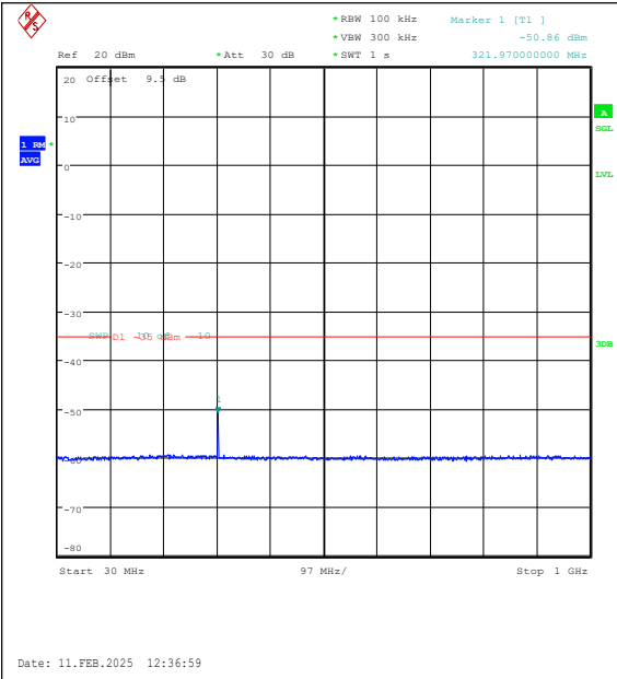
Band41(2535-2655)-20MHz-QPSK-41140-1RB#0-30~1000-PASS
