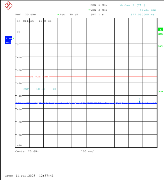
Band41(2535-2655)-20MHz-QPSK-41140-1RB#0-20000~27000-PASS
