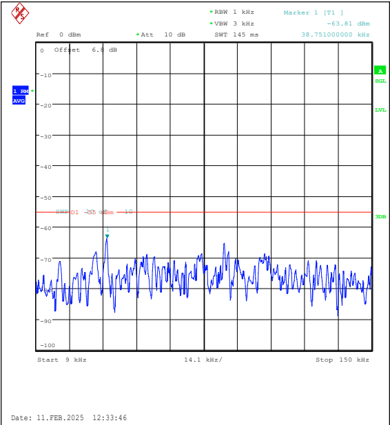
Band41(2535-2655)-20MHz-QPSK-40590-1RB#0 -0.009~0.15-PASS
