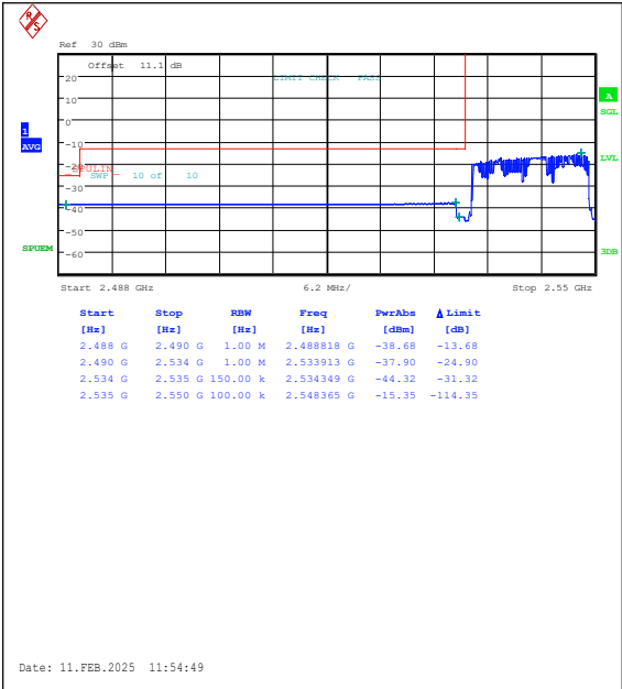
Band41(2535-2655)-15MHz-QPSK-40115-75RB# 0-PASS
