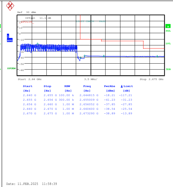
Band41(2535-2655)-15MHz-16QAM-41165-75RB# 0-PASS
