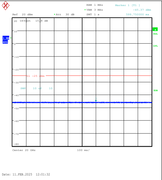
Band41(2535-2655)-15MHz-16QAM-40115-1RB#0 -20000~27000-PASS
