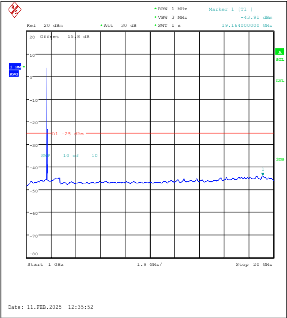
Band41(2535-2655)-20MHz-16QAM-40590-1RB# 0-1000~20000-PASS
