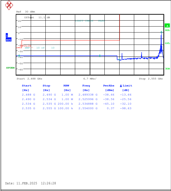
Band41(2535-2655)-20MHz-16QAM-40140-1RB# 99-PASS
