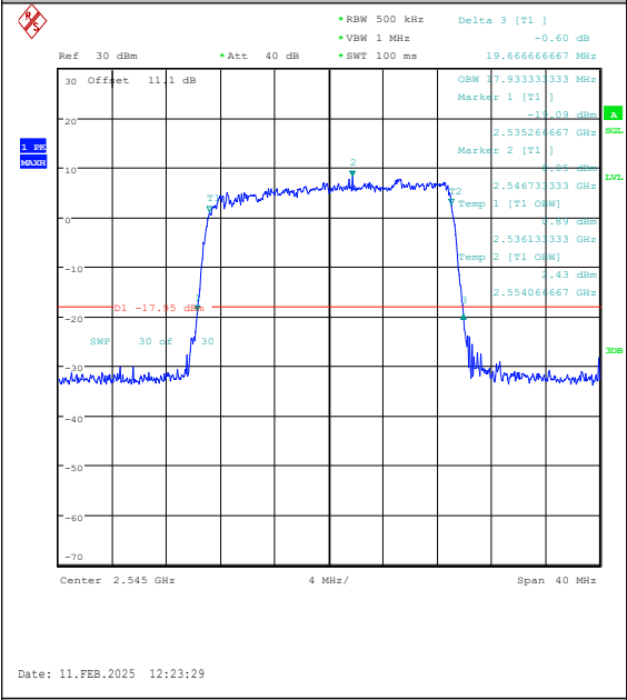
Band41(2535-2655)-20MHz-QPSK-40140-100RB #0-PASS
