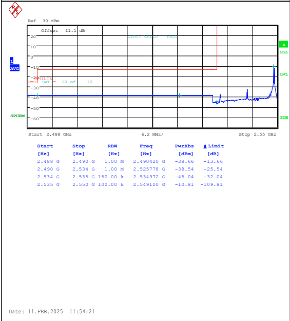
Band41(2535-2655)-15MHz-16QAM-40115-1RB# 74-PASS
