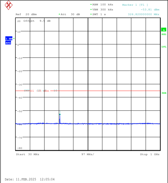
Band41(2535-2655)-15MHz-QPSK-41165-1RB#0-30~1000-PASS
