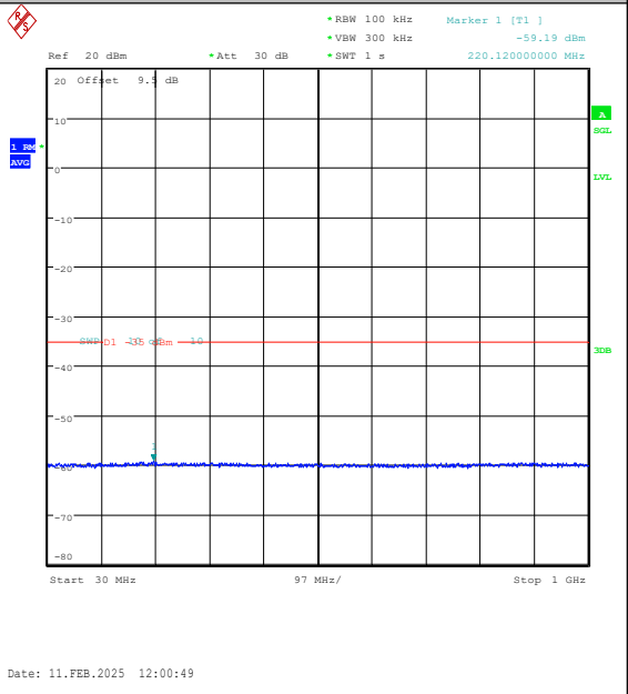
Band41(2535-2655)-15MHz-16QAM-40115-1RB#0-30~1000-PASS
