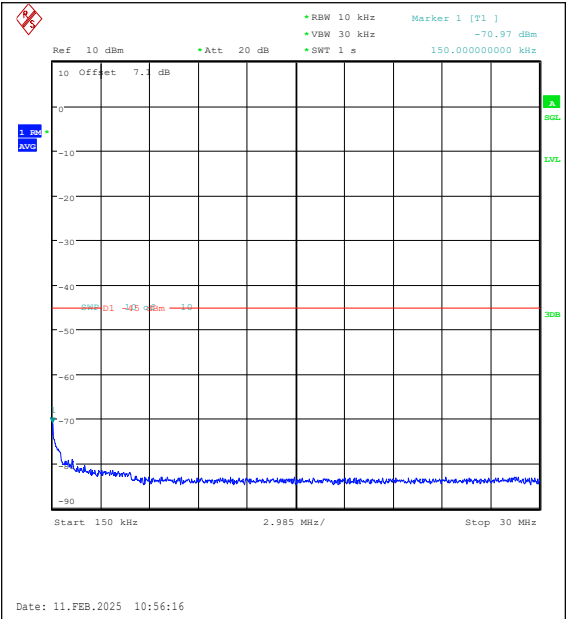
Band41(2535-2655)-5MHz-16QAM-40590-1RB#0 -0.15~30-PASS
