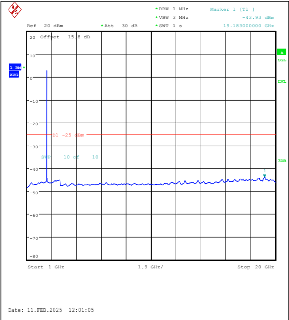
Band41(2535-2655)-15MHz-16QAM-40115-1RB# 0-1000~20000-PASS
