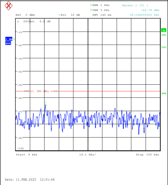
Band41(2535-2655)-15MHz-QPSK-40590-1RB#0 -0.009~0.15-PASS
