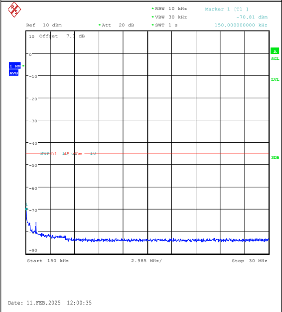
Band41(2535-2655)-15MHz-16QAM-40115-1RB#0-0.0.15~30-PASS
