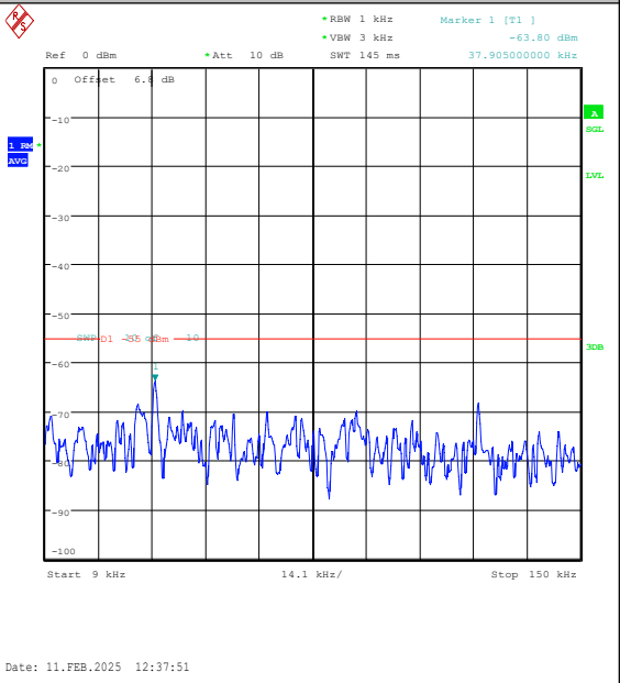
Band41(2535-2655)-20MHz-16QAM-41140-1RB#0-0.009~0.15-PASS
