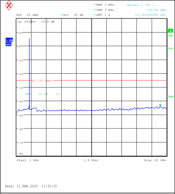
Band41(2535-2655)-10MHz-16QAM-41190-1RB# 0-1000~20000-PASS
