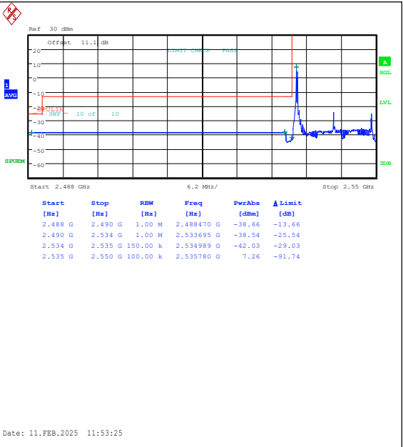
Band41(2535-2655)-15MHz-16QAM-40115-1RB#0 -PASS
