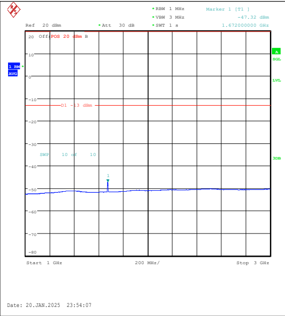
Band5-5MHz-QPSK-20525-25RB#0-1000~3000-P ASS
