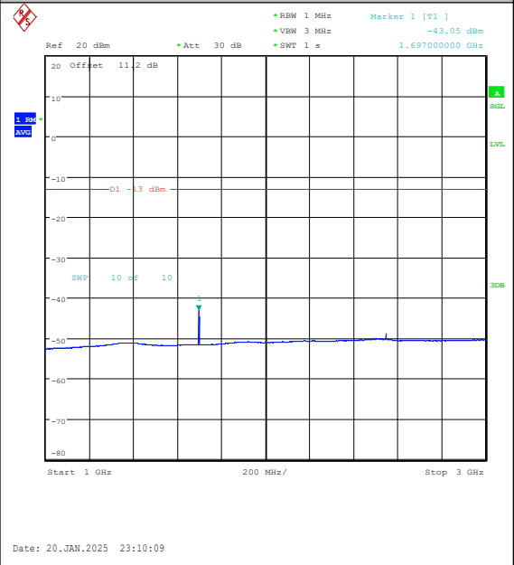
Band5-3MHz-16QAM-20635-1RB#14-1000~3000-PASS
