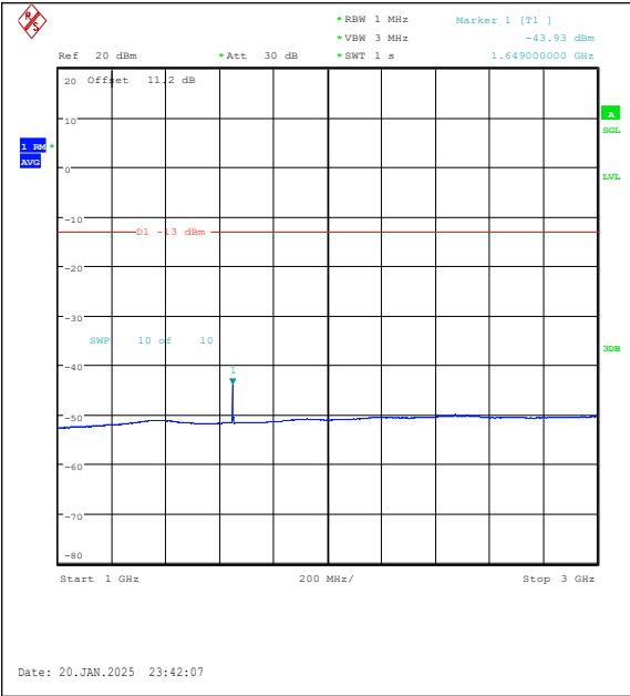
Band5-5MHz-16QAM-20425-1RB#0-1000~3000-P ASS
