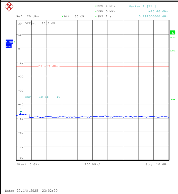
Band5-3MHz-16QAM-20525-1RB#14-3000~1000 0-PASS
