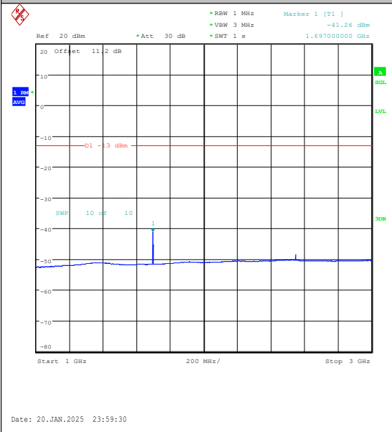
Band5-5MHz-QPSK-20625-1RB#24-1000~3000-P ASS
