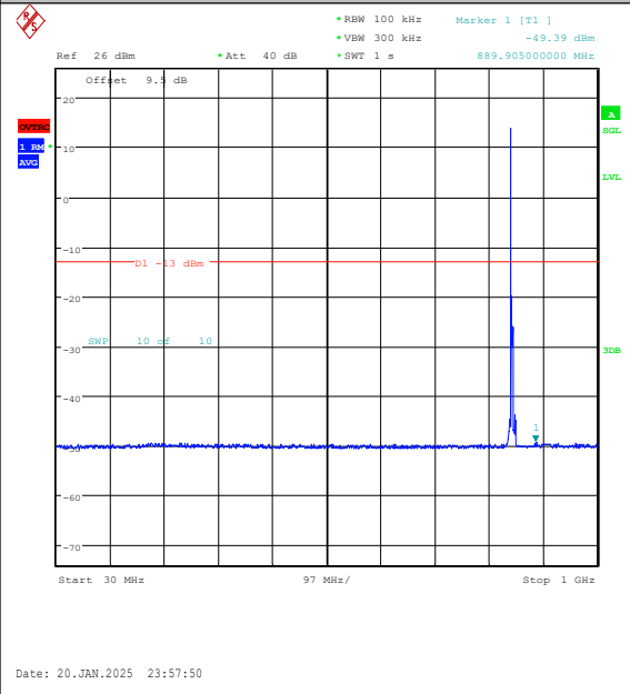
Band5-5MHz-16QAM-20625-1RB#0-30~1000-PA SS
