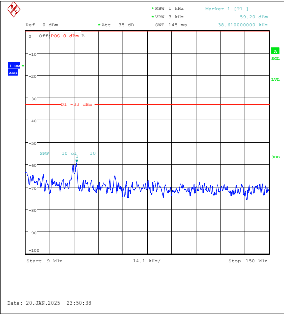
Band5-5MHz-QPSK-20525-1RB#24-0.009~0.15-P ASS
