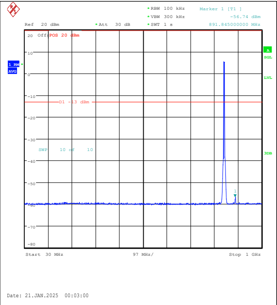
Band5-5MHz-16QAM-20625-25RB#0-30~1000-PA SS
