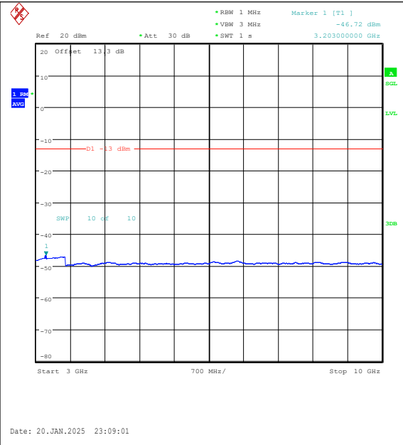
Band5-3MHz-QPSK-20635-1RB#14-3000~10000-P PASS
