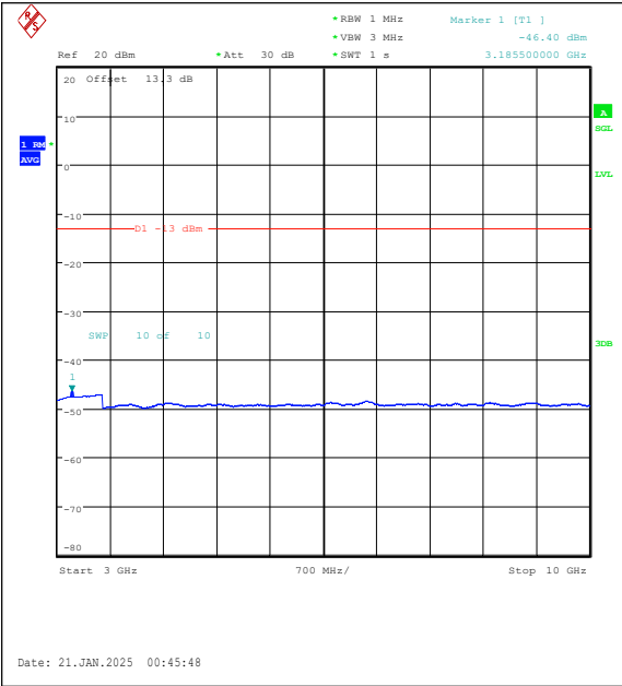
Band5-10MHz-QPSK-20600-1RB#0-3000~10000-PASS
