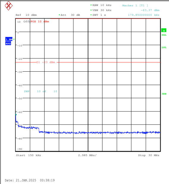
Band5-10MHz-16QAM-20525-1RB#0-0.15~30-PA SS
