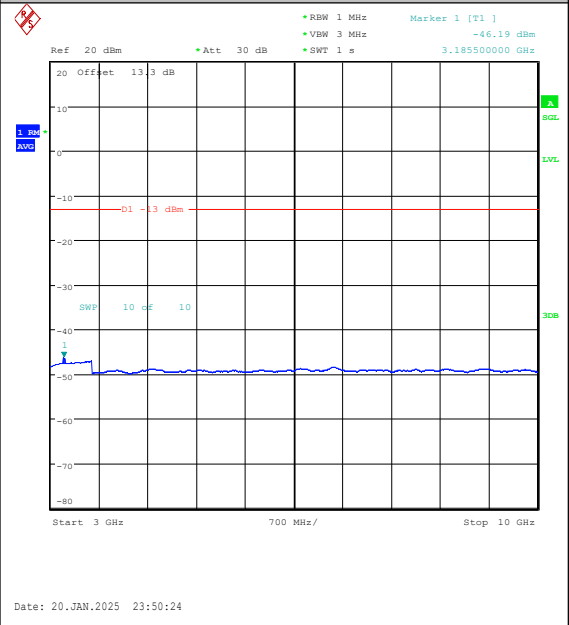
Band5-5MHz-16QAM-20525-1RB#0-3000~10000- PASS
