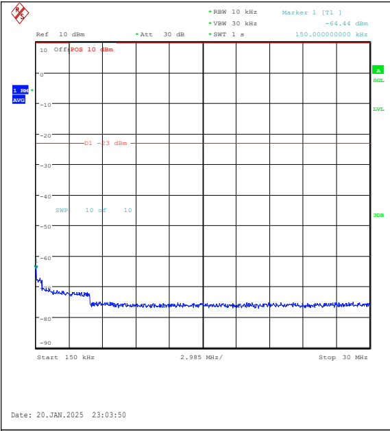
Band5-3MHz-16QAM-20525-15RB#0-0.15~30-PA SS
