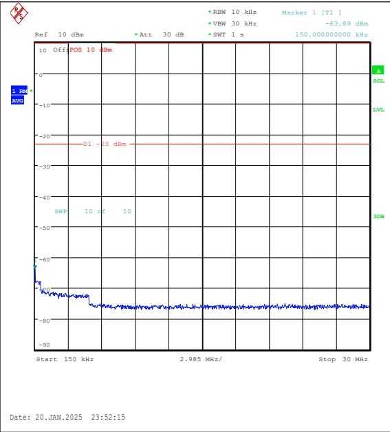
Band5-5MHz-16QAM-20525-1RB#24-0.15~30-PA-SS
