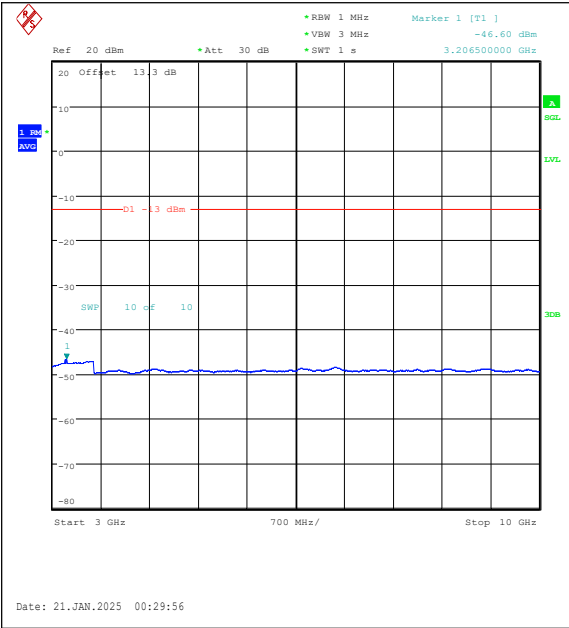
Band5-10MHz-QPSK-20450-1RB#0-3000~10000-PASS
