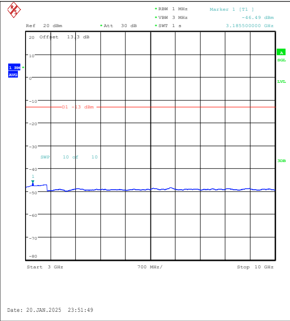
Band5-5MHz-QPSK-20525-1RB#24-3000~10000-P PASS
