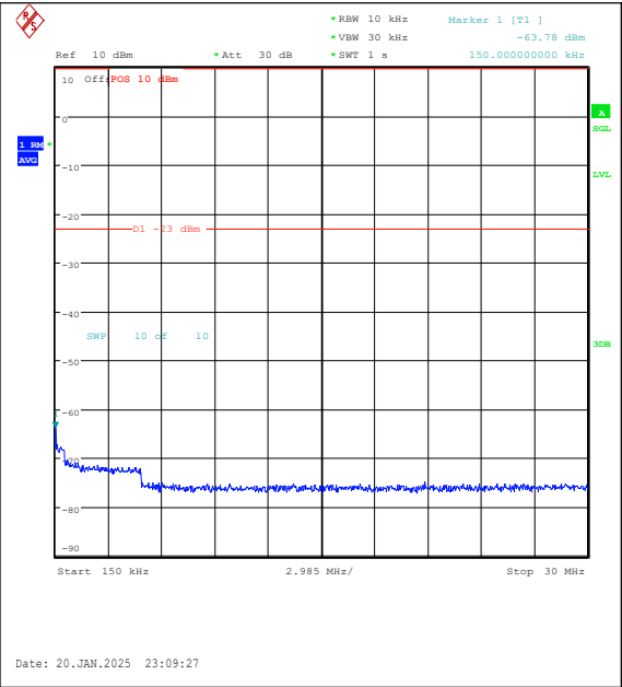
Band5-3MHz-16QAM-20635-1RB#14-0.15~30-PA-SS
