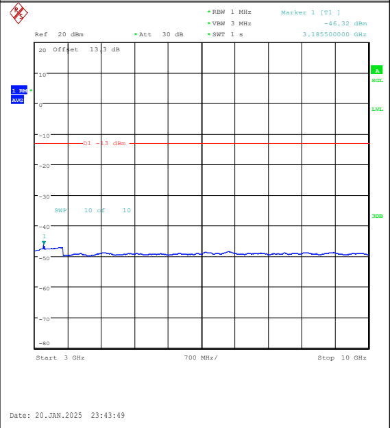
Band5-5MHz-QPSK-20425-1RB#24-3000~10000-PASS
