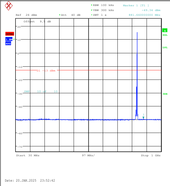
Band5-5MHz-16QAM-20525-1RB#24-30~1000-PA-SS
