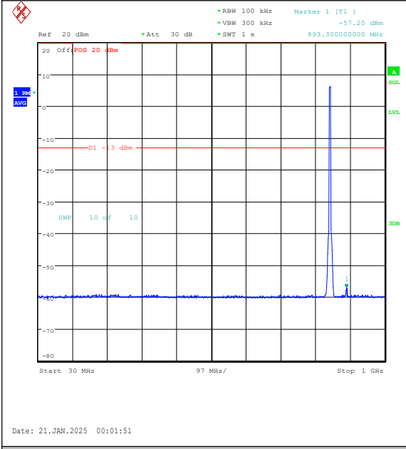
Band5-5MHz-QPSK-20625-25RB#0-30~1000-PA SS
