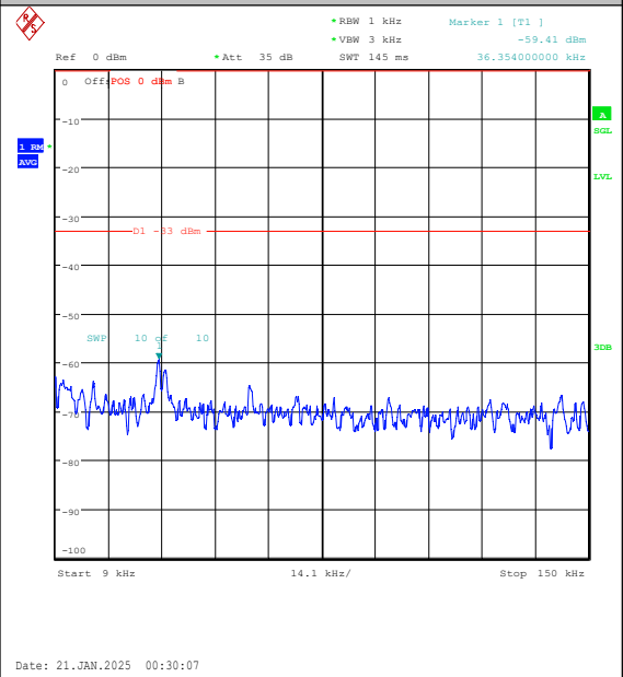
Band5-10MHz-16QAM-20450-1RB#0-0.009~0.15- PASS
