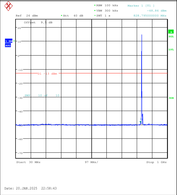
Band5-3MHz-16QAM-20525-1RB#0-30~1000-PASS
