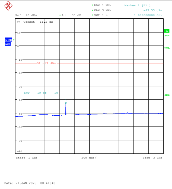
Band5-10MHz-16QAM-20525-1RB#49-1000~300 0-PASS
