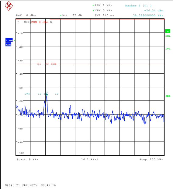
Band5-10MHz-QPSK-20525-50RB#0-0.009~0.15-PASS
