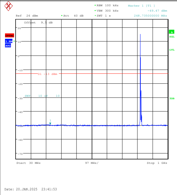
Band5-5MHz-16QAM-20425-1RB#0-30~1000-PA SS
