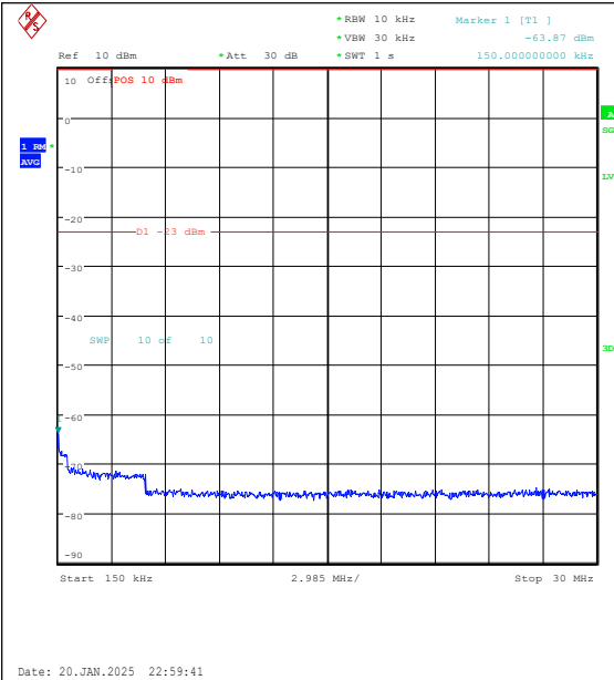
Band5-3MHz-QPSK-20525-1RB#14-0.15~30-PAS S
