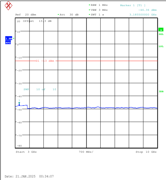
Band5-10MHz-16QAM-20450-1RB#49-3000~100 00-PASS
