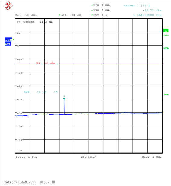
Band5-10MHz-QPSK-20525-1RB#0-1000~3000-P ASS
