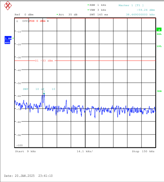
Band5-5MHz-16QAM-20425-1RB#0-0.009~0.15-P ASS
