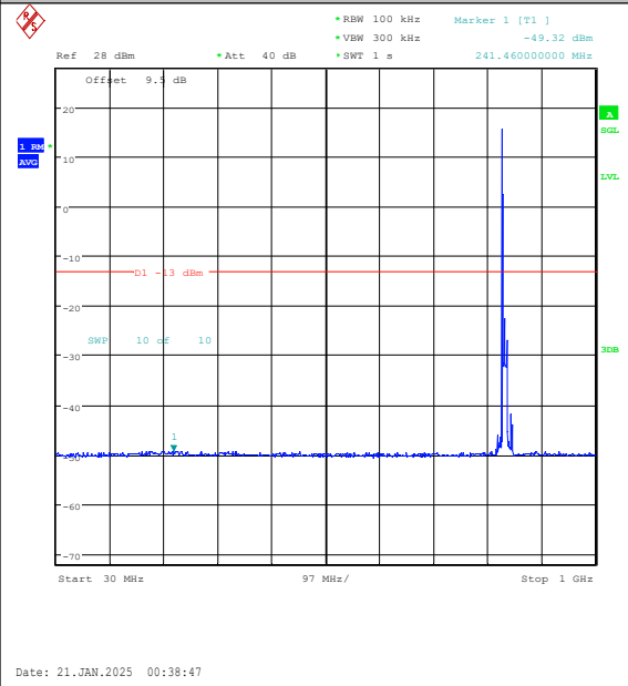
Band5-10MHz-16QAM-20525-1RB#0-30~1000-PA SS
