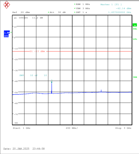
Band5-5MHz-16QAM-20425-1RB#24-1000~3000- PASS
