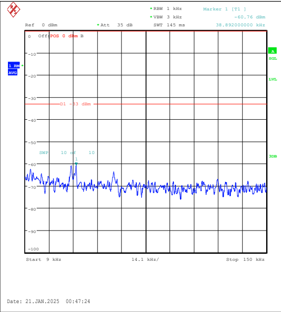
Band5-10MHz-QPSK-20600-1RB#49-0.009~0.15-PASS
