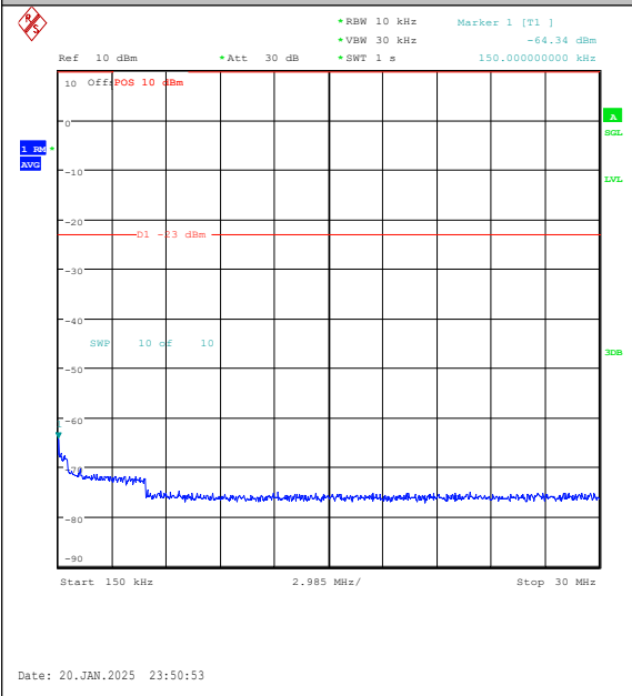
Band5-5MHz-QPSK-20525-1RB#24-0.15~30-PAS S
