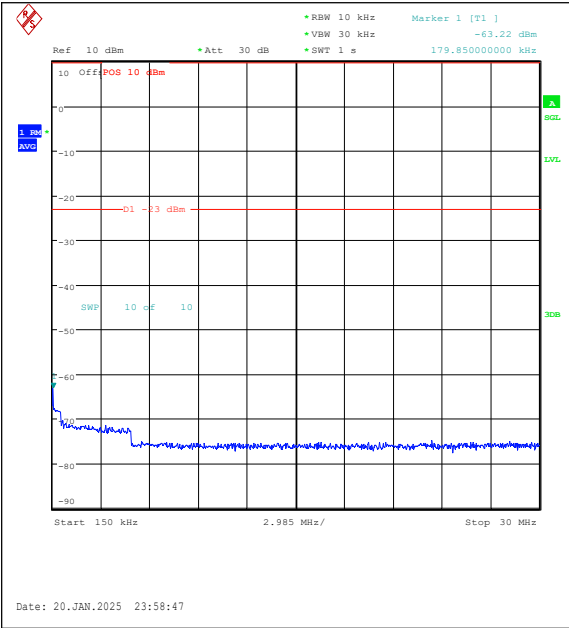
Band5-5MHz-QPSK-20625-1RB#24-0.15~30-PAS S
