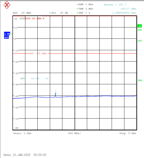
Band5-10MHz-QPSK-20600-50RB#0-1000~3000- PASS
