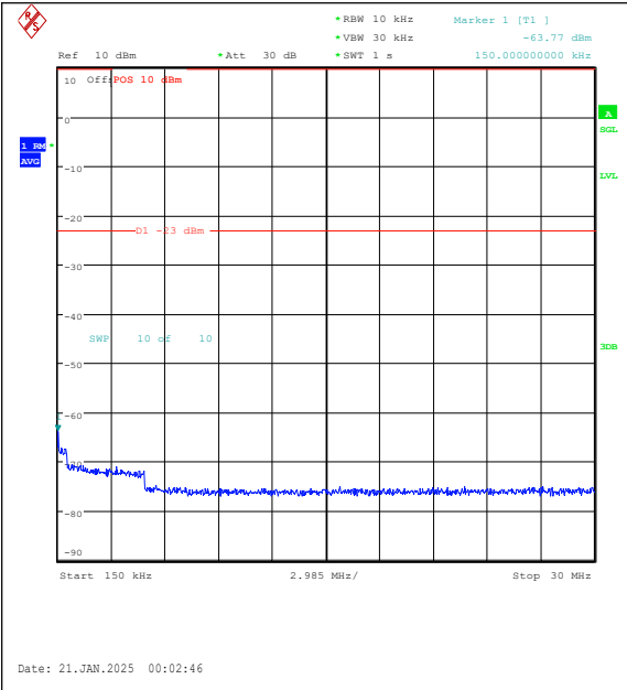
Band5-5MHz-16QAM-20625-25RB#0-0.15~30-PA SS
