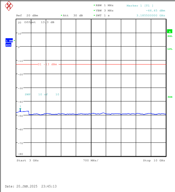
Band5-5MHz-16QAM-20425-1RB#24-3000~1000 0-PASS
