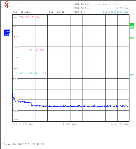
Band5-5MHz-16QAM-20525-1RB#0-0.15~30-PAS S
