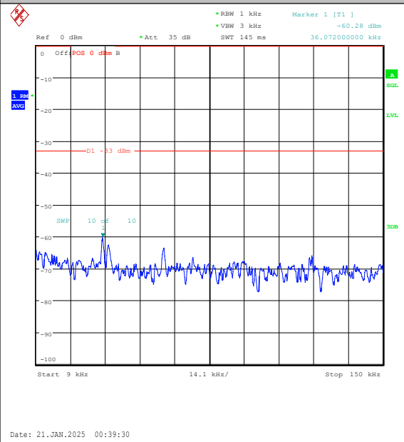
Band5-10MHz-QPSK-20525-1RB#49-0.009~0.15- PASS
