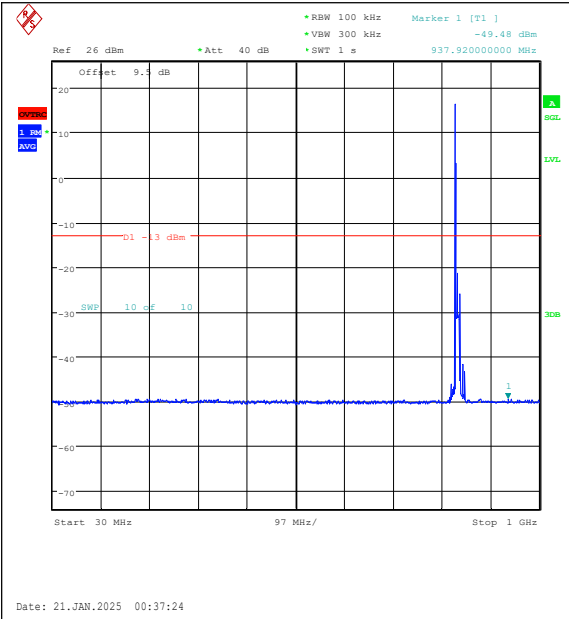
Band5-10MHz-QPSK-20525-1RB#0-30~1000-PA SS
