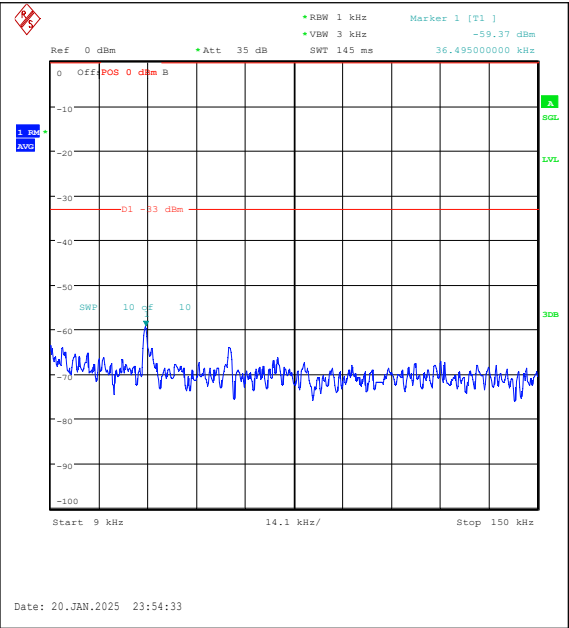
Band5-5MHz-16QAM-20525-25RB#0-0.009~0.15- PASS
