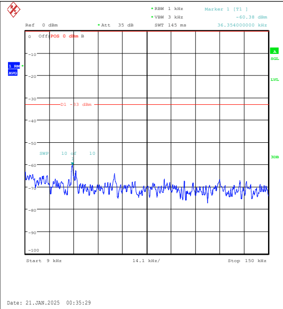
Band5-10MHz-16QAM-20450-50RB#0-0.009~0.1 5-PASS
