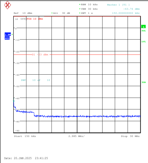
Band5-5MHz-16QAM-20425-1RB#0-0.15~30-PAS S
