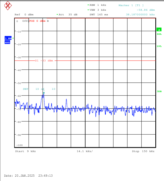
Band5-5MHz-16QAM-20525-1RB#0-0.009~0.15-P ASS
