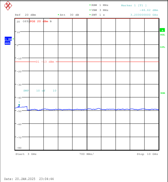
Band5-3MHz-16QAM-20525-15RB#0-3000~1000 0-PASS
