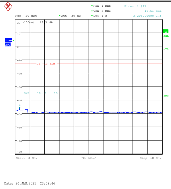
Band5-5MHz-QPSK-20625-1RB#24-3000~10000- PASS
