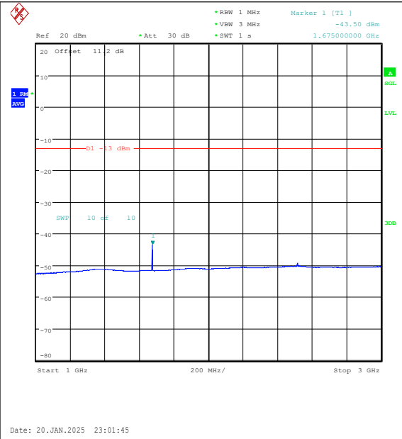
Band5-3MHz-16QAM-20525-1RB#14-1000~3000- PASS
