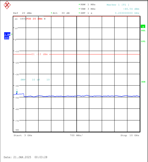
Band5-5MHz-16QAM-20625-25RB#0-3000~1000 0-PASS
