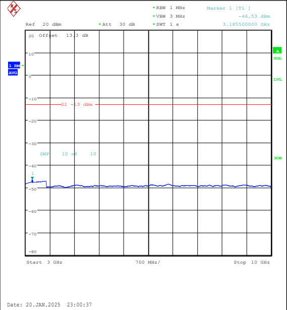
Band5-3MHz-QPSK-20525-1RB#14-3000~10000- PASS
