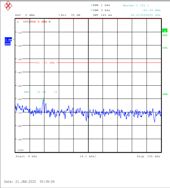
Band5-10MHz-16QAM-20525-1RB#0-0.009~0.15- PASS
