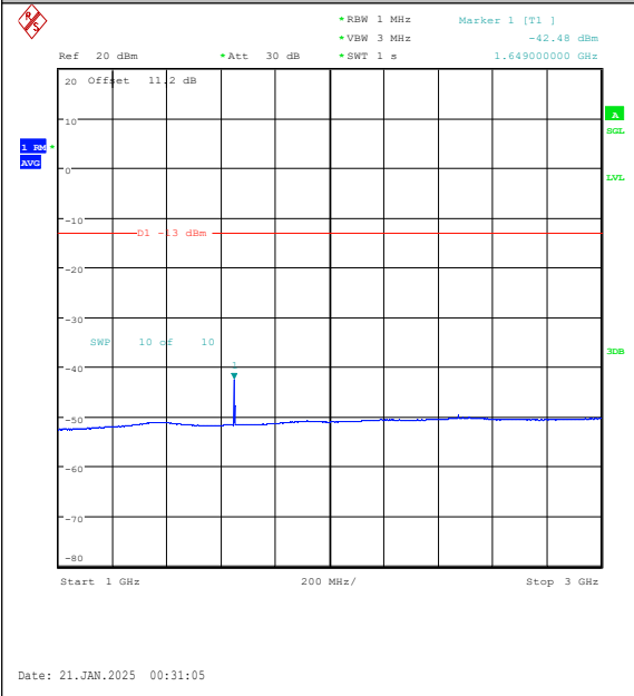
Band5-10MHz-16QAM-20450-1RB#0-1000~3000- PASS
