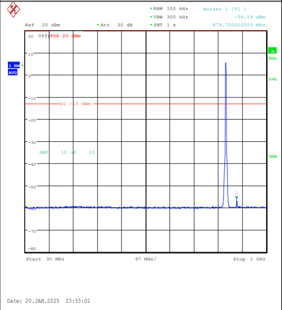
Band5-5MHz-16QAM-20525-25RB#0-30~1000-PA SS
