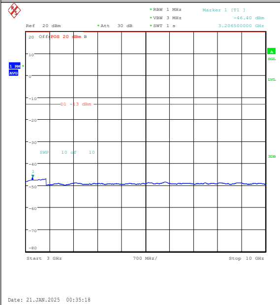
Band5-10MHz-QPSK-20450-50RB#0-3000~1000 0-PASS
