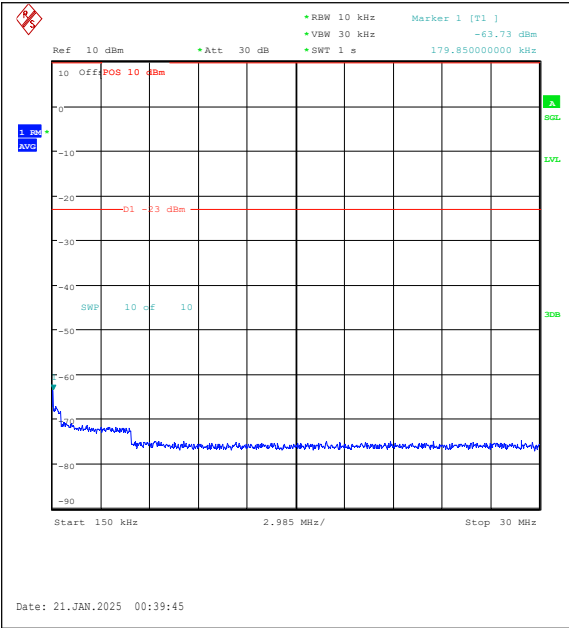
Band5-10MHz-QPSK-20525-1RB#49-0.15~30-PA SS
