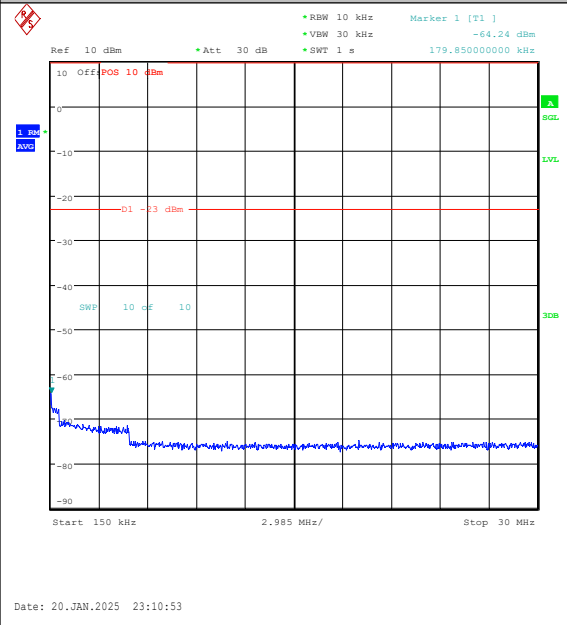
Band5-3MHz-QPSK-20635-15RB#0-0.15~30-PAS S
