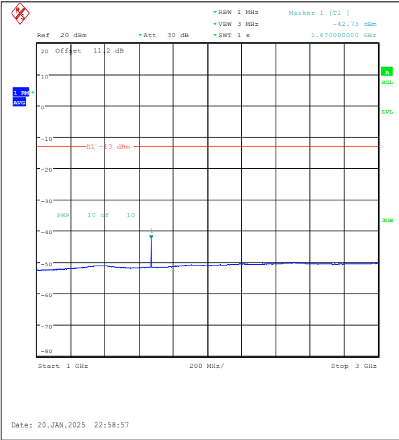
Band5-3MHz-16QAM-20525-1RB#0-1000~3000-P ASS
