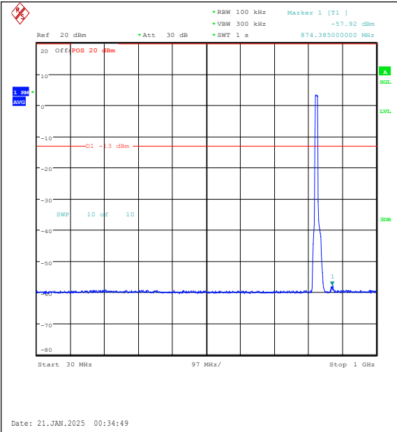
Band5-10MHz-QPSK-20450-50RB#0-30~1000-PA SS
