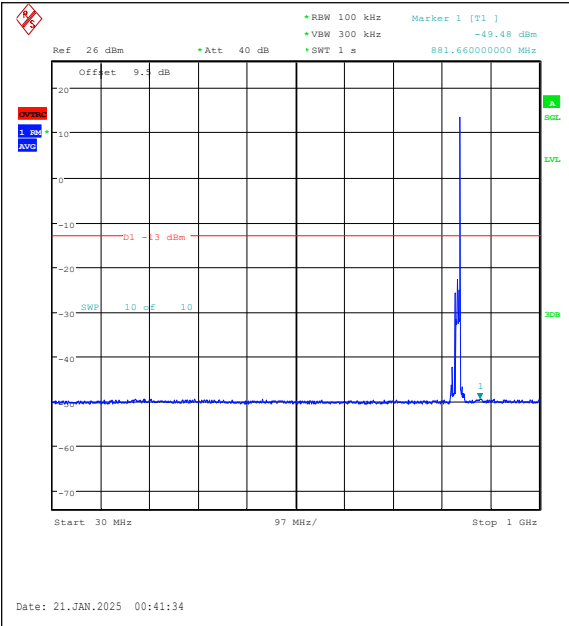
Band5-10MHz-16QAM-20525-1RB#49-30~1000-P ASS
