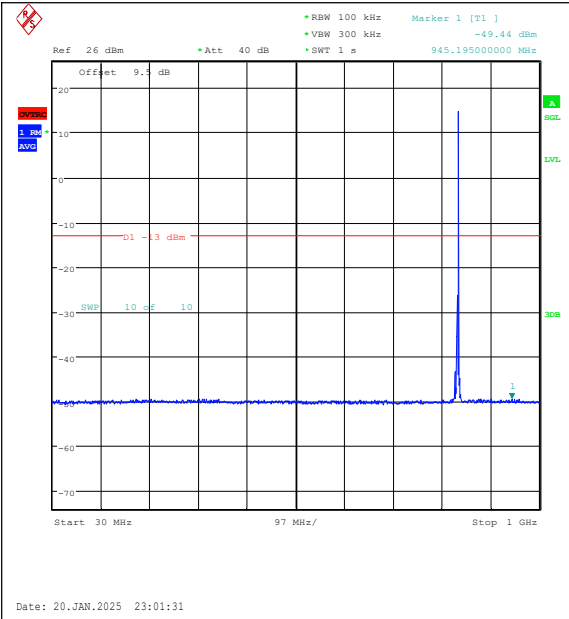
Band5-3MHz-16QAM-20525-1RB#14-30~1000-PA SS
