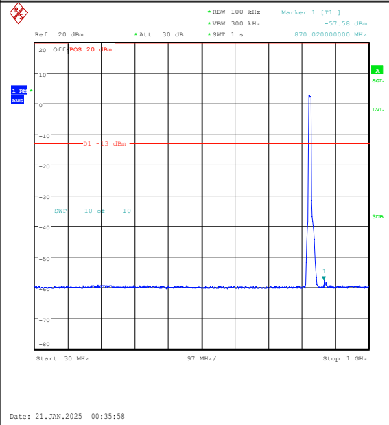
Band5-10MHz-16QAM-20450-50RB#0-30~1000-P ASS
