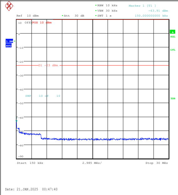
Band5-10MHz-QPSK-20600-1RB#49-0.15~30-PA-SS
