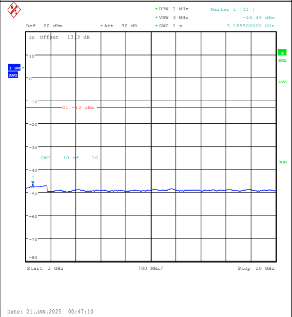
Band5-10MHz-16QAM-20600-1RB#0-3000~1000 0-PASS
