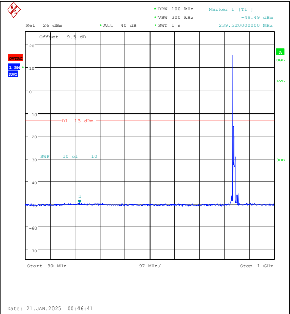
Band5-10MHz-16QAM-20600-1RB#0-30~1000-PA SS
