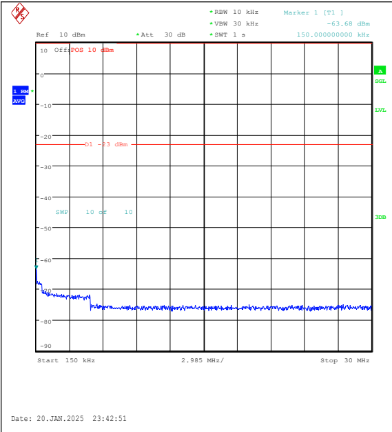
Band5-5MHz-QPSK-20425-1RB#24-0.15~30-PAS S
