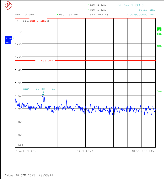
Band5-5MHz-QPSK-20525-25RB#0-0.009~0.15-P ASS
