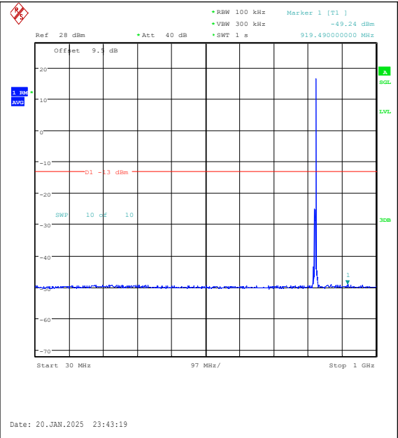
Band5-5MHz-QPSK-20425-1RB#24-30~1000-PA SS
