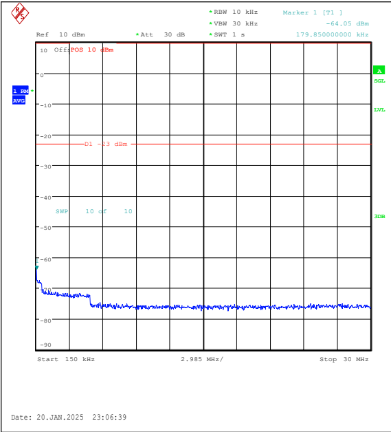
Band5-3MHz-16QAM-20635-1RB#0-0.15~30-PAS S
