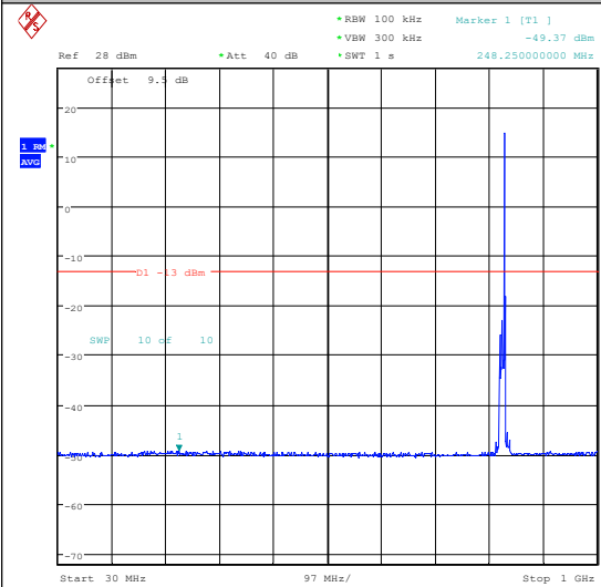
Band5-10MHz-16QAM-20450-1RB#49-0.009~0.1 5-PASS
