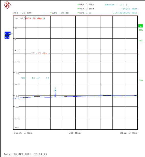
Band5-3MHz-16QAM-20525-15RB#0-1000~3000- PASS
