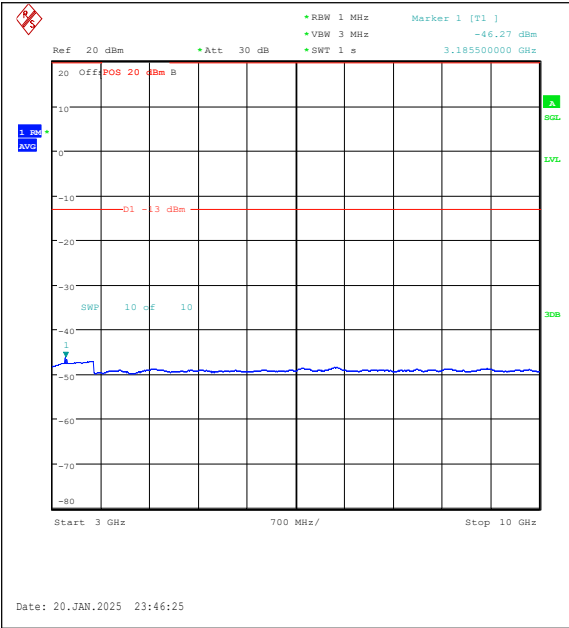
Band5-5MHz-QPSK-20425-25RB#0-3000~10000-PASS
