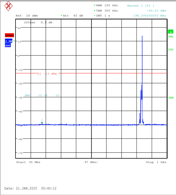
Band5-10MHz-QPSK-20525-1RB#49-30~1000-PA SS
