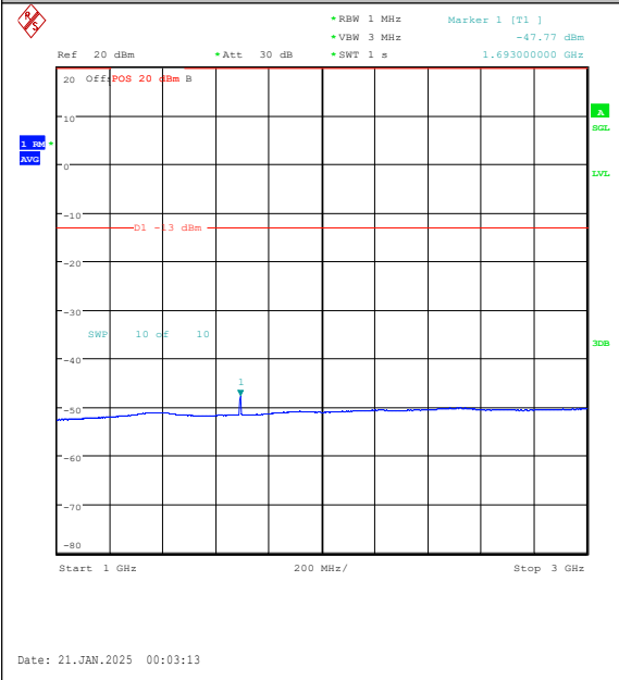
Band5-5MHz-16QAM-20625-25RB#0-1000~3000- PASS
