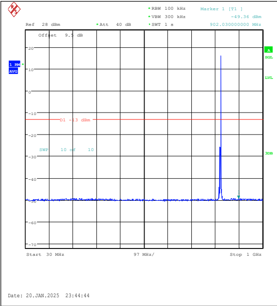
Band5-5MHz-16QAM-20425-1RB#24-30~1000-PA SS
