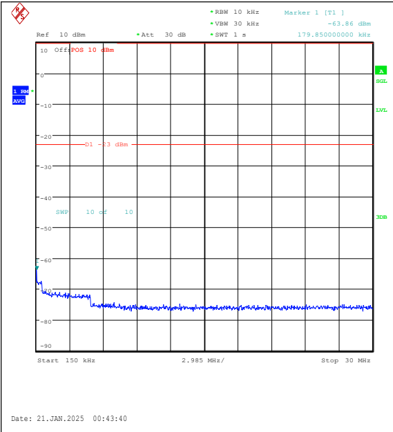
Band5-10MHz-16QAM-20525-50RB#0-0.15~30-P ASS
