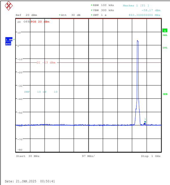
Band5-10MHz-QPSK-20600-50RB#0-30~1000-PA SS
