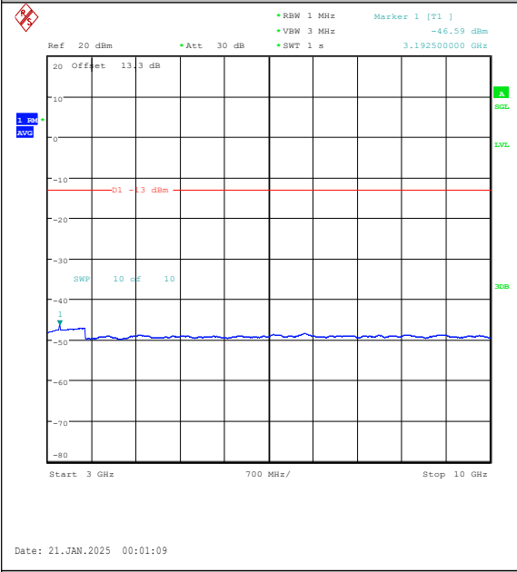
Band5-5MHz-16QAM-20625-1RB#24-3000~1000 0-PASS
