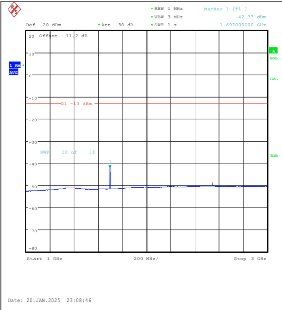
Band5-3MHz-QPSK-20635-1RB#14-1000~3000-P ASS
