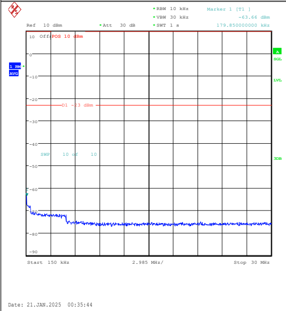
Band5-10MHz-16QAM-20450-50RB#0-0.15~30-P ASS
