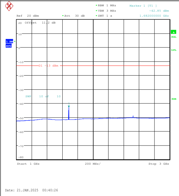
Band5-10MHz-QPSK-20525-1RB#49-1000~3000- PASS
