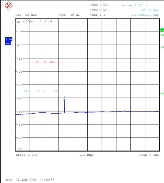
Band5-10MHz-16QAM-20600-1RB#0-1000~3000- PASS
