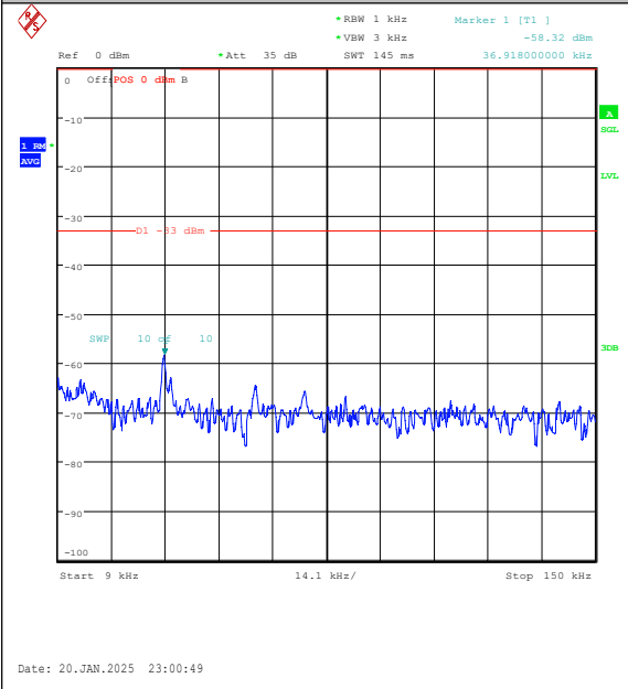
Band5-3MHz-16QAM-20525-1RB#14-0.009~0.15- PASS
