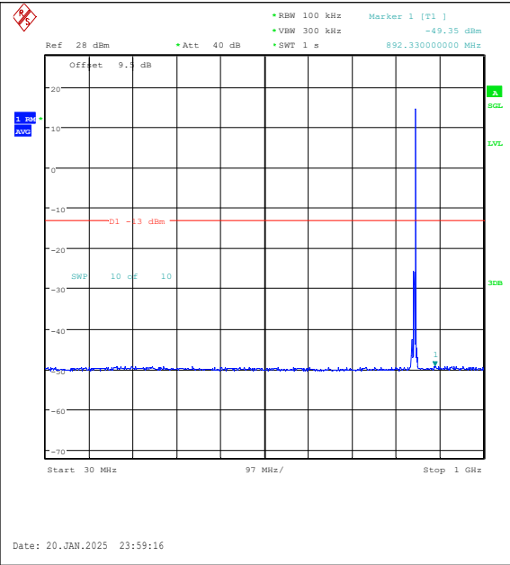
Band5-5MHz-QPSK-20625-1RB#24-30~1000-PA SS
