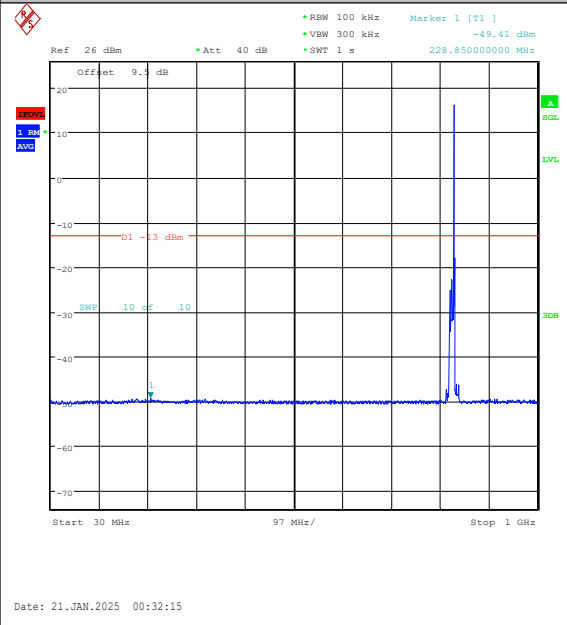
Band5-10MHz-QPSK-20450-1RB#49-30~1000-PA-SS
