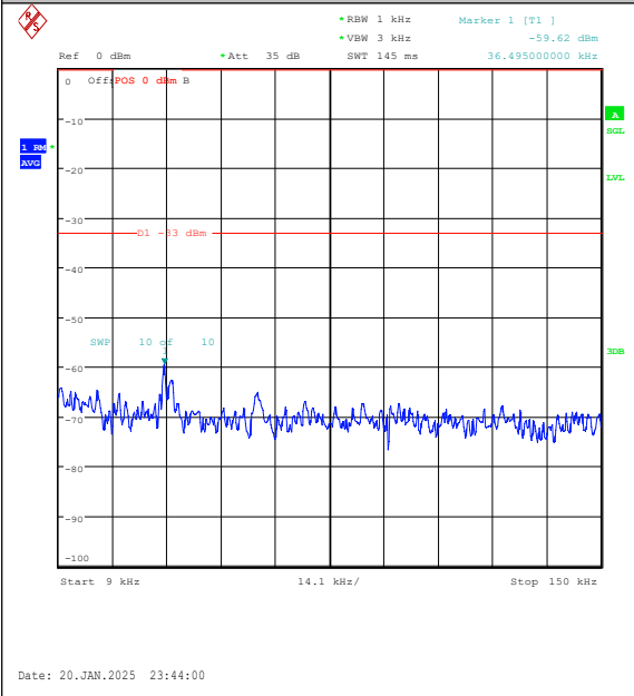
Band5-5MHz-16QAM-20425-1RB#24-0.009~0.15- PASS
