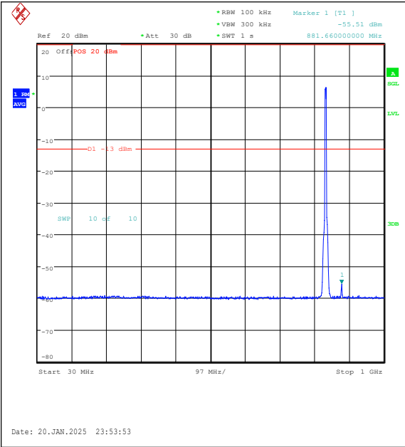
Band5-5MHz-QPSK-20525-25RB#0-30~1000-PA SS
