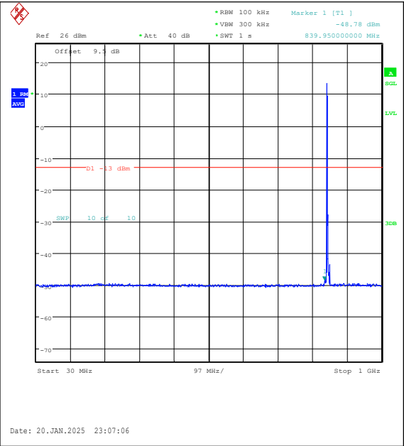
Band5-3MHz-16QAM-20635-1RB#0-30~1000-PA SS
