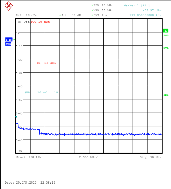
Band5-3MHz-16QAM-20525-1RB#0-0.15~30-PASS
