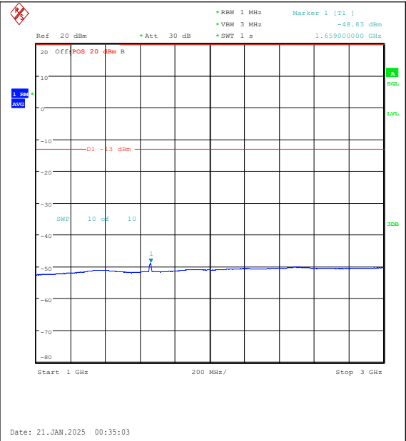
Band5-10MHz-QPSK-20450-50RB#0-1000~3000- PASS
