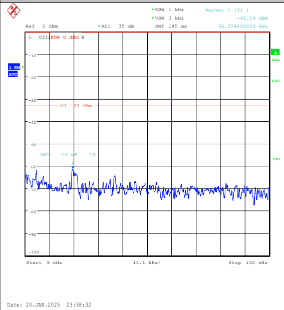
Band5-5MHz-QPSK-20625-1RB#24-0.009~0.15-P ASS
