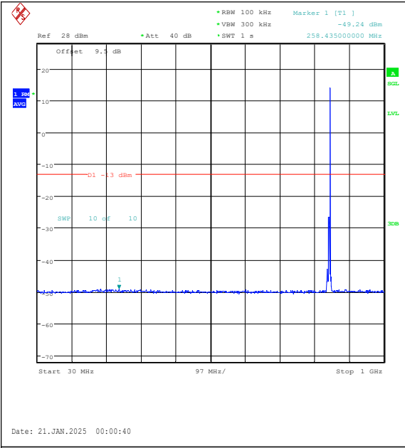
Band5-5MHz-16QAM-20625-1RB#24-30~1000-PA SS
