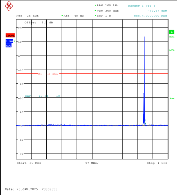
Band5-3MHz-16QAM-20635-1RB#14-30~1000-PA-SS
