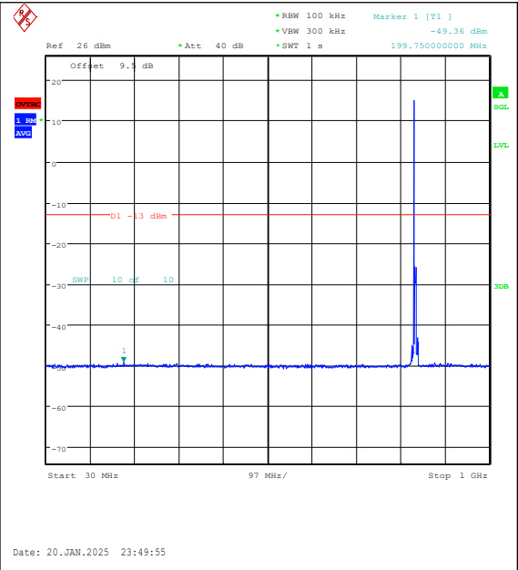
Band5-5MHz-16QAM-20525-1RB#0-30~1000-PA SS
