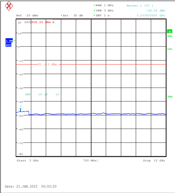
Band5-5MHz-QPSK-20625-25RB#0-3000~10000-PASS
