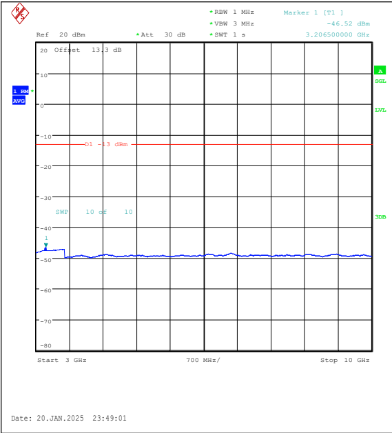
Band5-5MHz-QPSK-20525-1RB#0-3000~10000-P ASS
