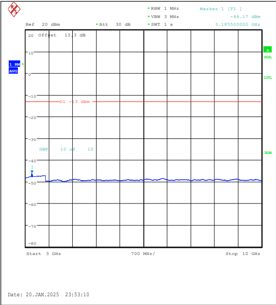
Band5-5MHz-16QAM-20525-1RB#24-3000~1000 0-PASS
