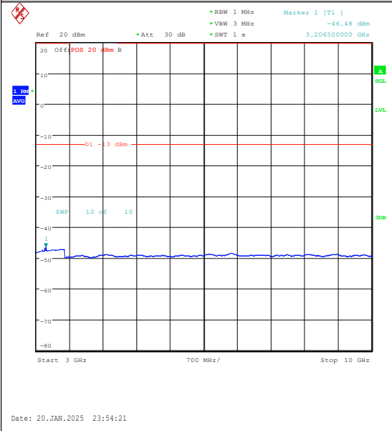
Band5-5MHz-QPSK-20525-25RB#0-3000~10000- PASS
