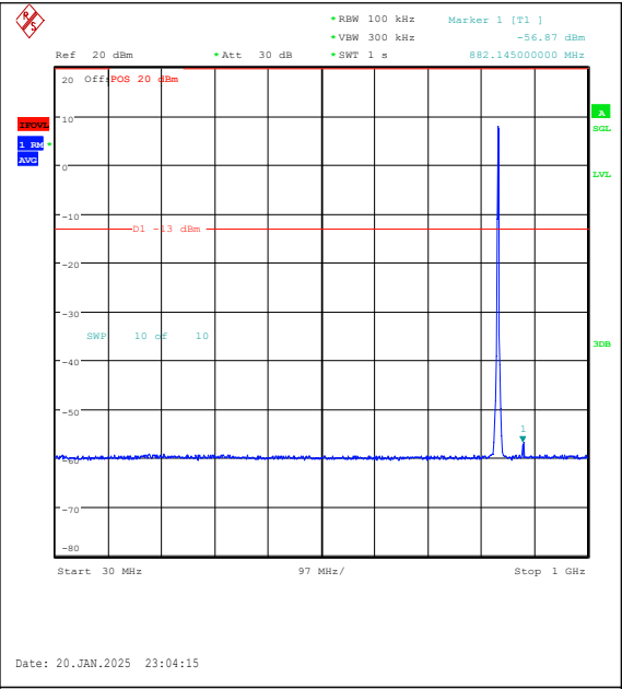
Band5-3MHz-16QAM-20525-15RB#0-30~1000-PA SS
