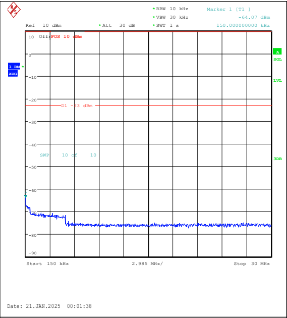
Band5-5MHz-QPSK-20625-25RB#0-0.15~30-PAS S
