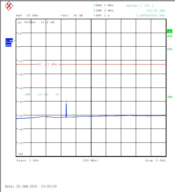
Band5-5MHz-16QAM-20525-1RB#0-1000~3000-P ASS
