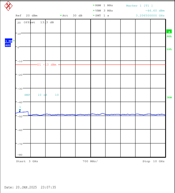
Band5-3MHz-16QAM-20635-1RB#0-3000~10000- PASS
