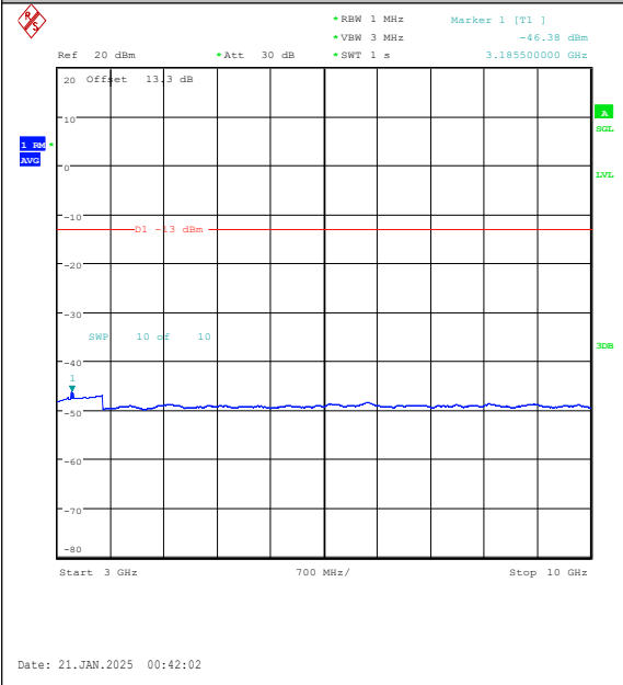
Band5-10MHz-16QAM-20525-1RB#49-3000~100 00-PASS
