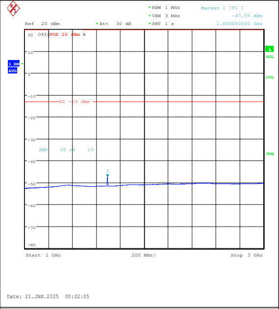
Band5-5MHz-QPSK-20625-25RB#0-1000~3000-P ASS
