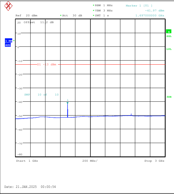
Band5-5MHz-16QAM-20625-1RB#24-1000~3000- PASS
