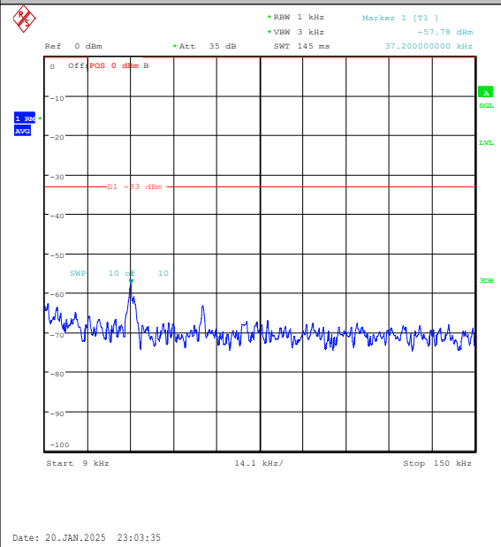
Band5-3MHz-16QAM-20525-15RB#0-0.009~0.15- PASS
