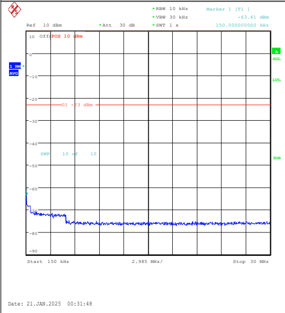
Band5-10MHz-QPSK-20450-1RB#49-0.15~30-PA-SS
