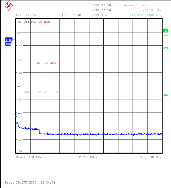
Band5-5MHz-16QAM-20525-25RB#0-0.15~30-PA SS
