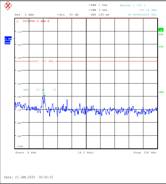
Band5-5MHz-16QAM-20625-25RB#0-0.009~0.15- PASS
