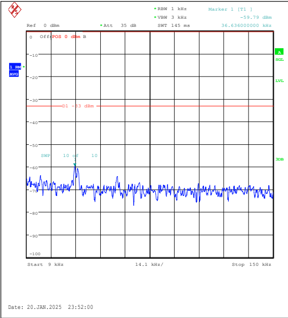
Band5-5MHz-16QAM-20525-1RB#24-0.009~0.15-PASS
