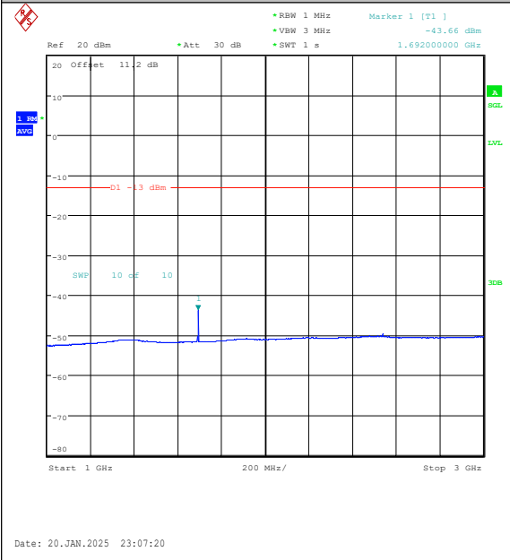
Band5-3MHz-16QAM-20635-1RB#0-1000~3000-P ASS
