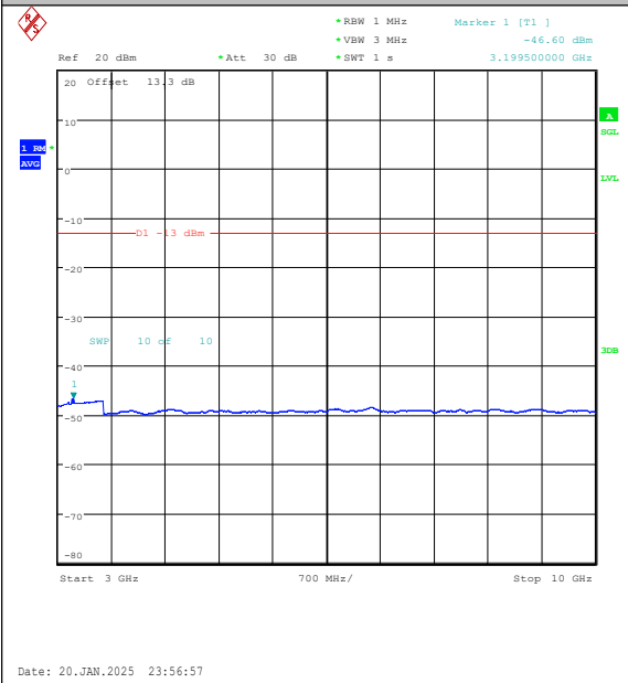
Band5-5MHz-QPSK-20625-1RB#0-3000~10000-P ASS
