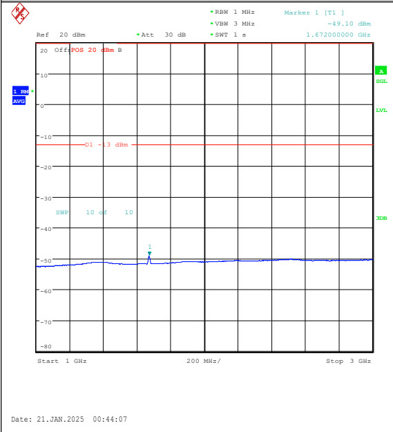
Band5-10MHz-16QAM-20525-50RB#0-1000~300 0-PASS
