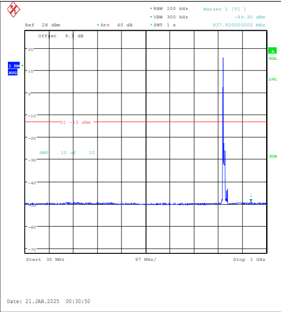
Band5-10MHz-16QAM-20450-1RB#0-30~1000-PA SS
