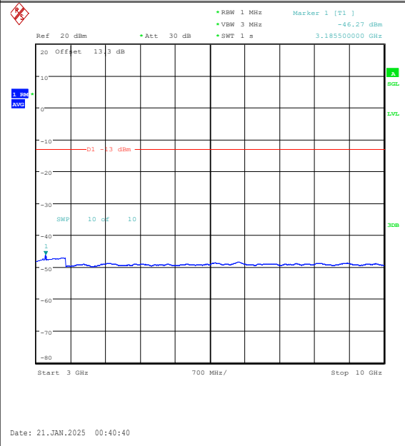
Band5-10MHz-QPSK-20525-1RB#49-3000~1000 0-PASS
