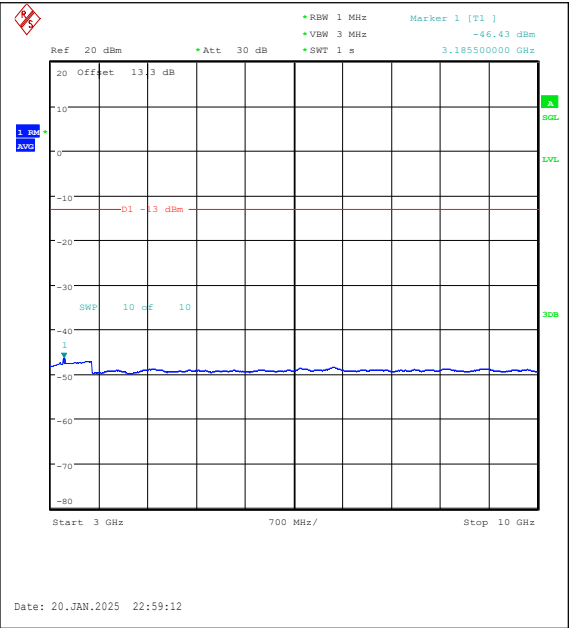
Band5-3MHz-16QAM-20525-1RB#0-3000~10000- PASS
