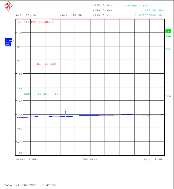
Band5-10MHz-QPSK-20525-50RB#0-1000~3000-PASS
