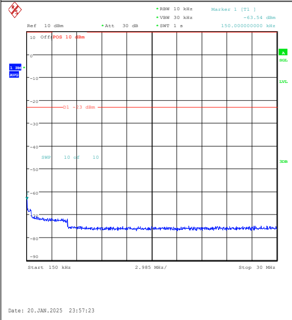
Band5-5MHz-16QAM-20625-1RB#0-0.15~30-PAS S
