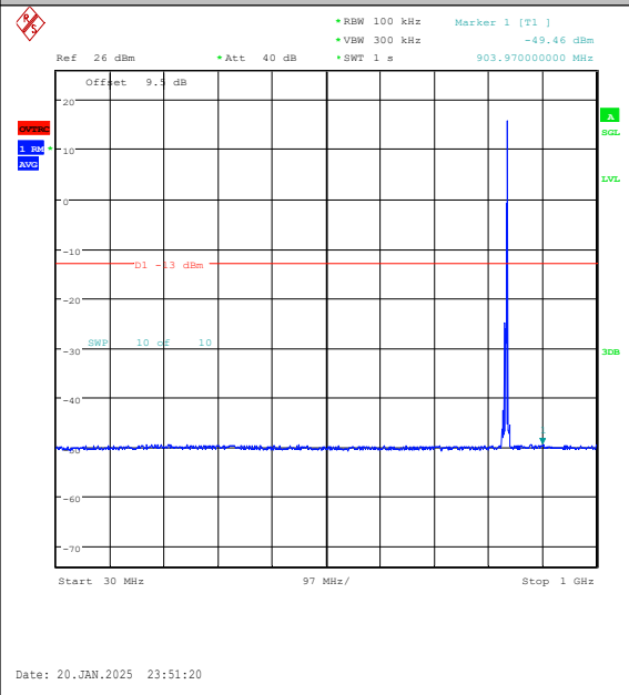
Band5-5MHz-QPSK-20525-1RB#24-30~1000-PA SS
