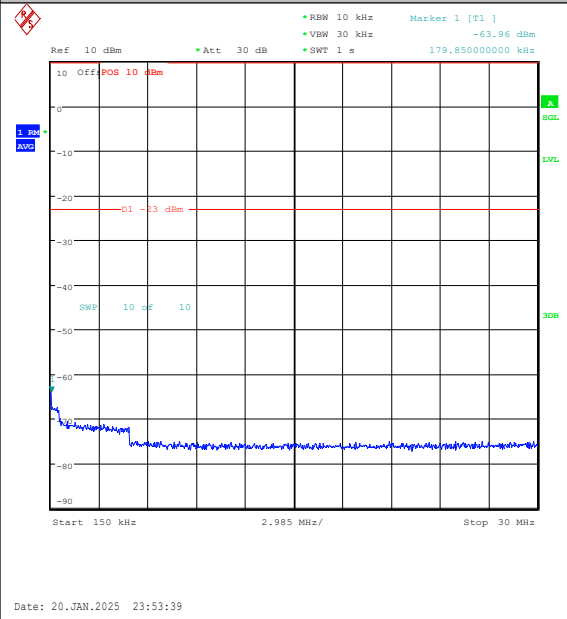
Band5-5MHz-QPSK-20525-25RB#0-0.15~30-PAS S
