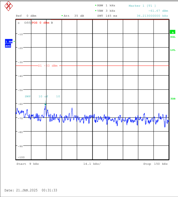
Band5-10MHz-QPSK-20450-1RB#49-0.009~0.15-PASS
