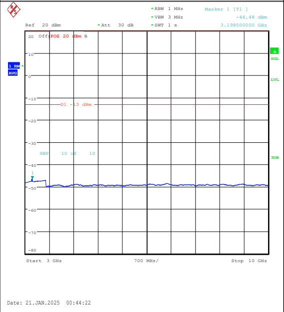
Band5-10MHz-16QAM-20525-50RB#0-3000~100 00-PASS
