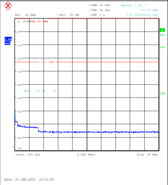
Band5-3MHz-16QAM-20525-1RB#14-0.15~30-PA SS
