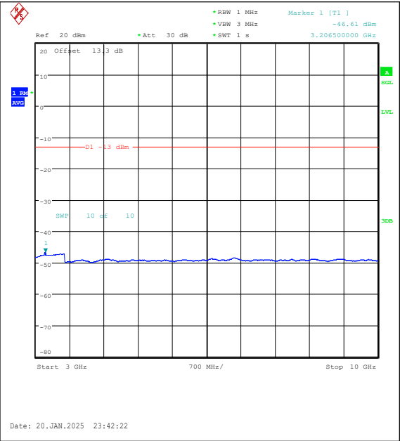
Band5-5MHz-16QAM-20425-1RB#0-3000~10000- PASS
