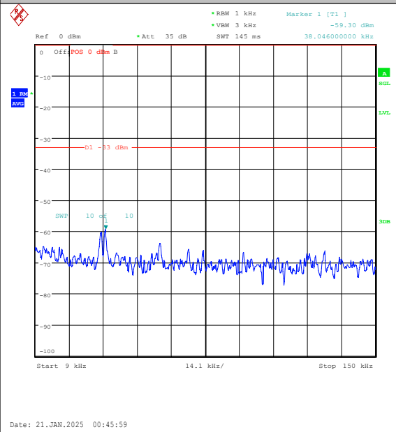
Band5-10MHz-16QAM-20600-1RB#0-0.009~0.15- PASS
