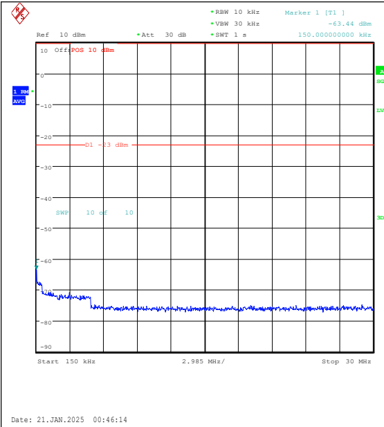
Band5-10MHz-16QAM-20600-1RB#0-0.15~30-PA SS
