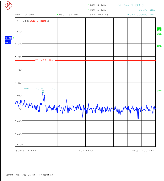
Band5-3MHz-16QAM-20635-1RB#14-0.009~0.15-PASS
