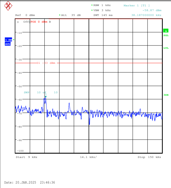
Band5-5MHz-16QAM-20425-25RB#0-0.009~0.15- PASS
