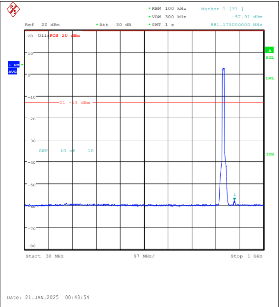
Band5-10MHz-16QAM-20525-50RB#0-30~1000-P ASS
