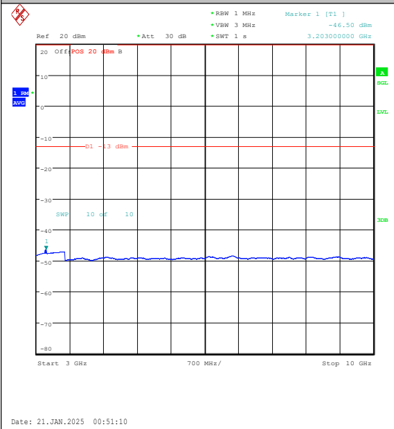
Band5-10MHz-QPSK-20600-50RB#0-3000~1000 0-PASS
