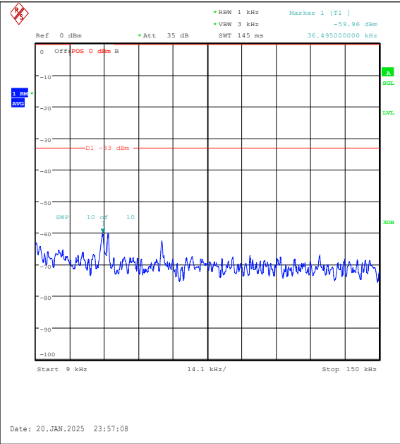
Band5-5MHz-16QAM-20625-1RB#0-0.009~0.15-P ASS
