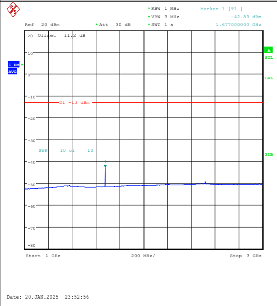
Band5-5MHz-16QAM-20525-1RB#24-1000~3000-PASS
