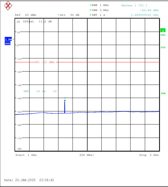
Band5-5MHz-QPSK-20625-1RB#0-1000~3000-PA SS
