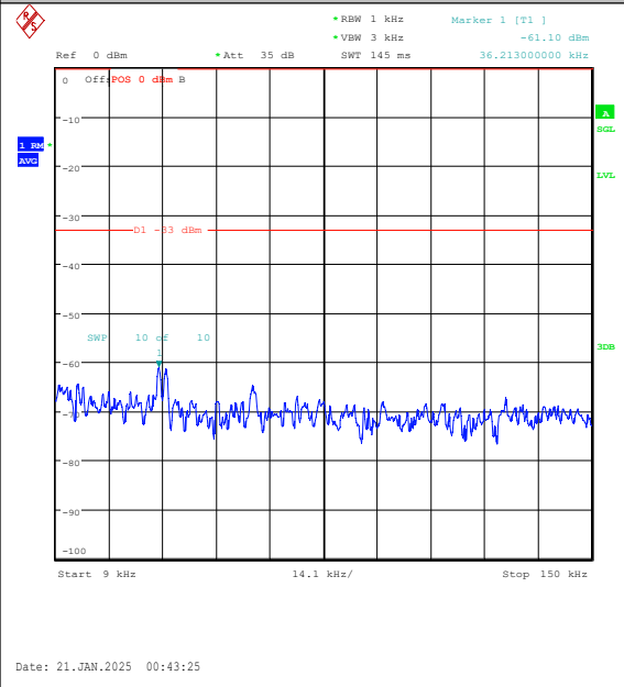
Band5-10MHz-16QAM-20525-50RB#0-0.009~0.1 5-PASS
