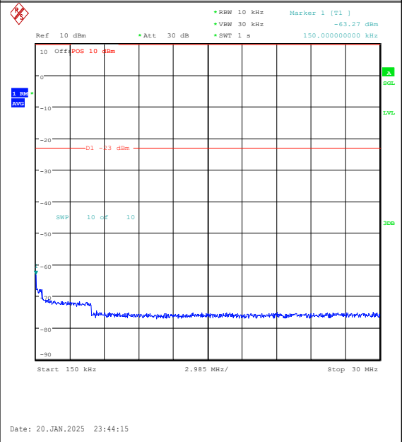
Band5-5MHz-16QAM-20425-1RB#24-0.15~30-PA SS
