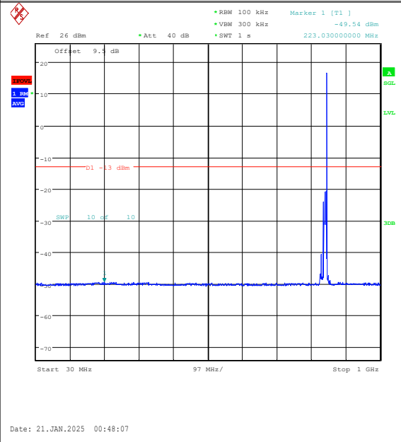
Band5-10MHz-QPSK-20600-1RB#49-30~1000-PA-SS
