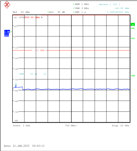
Band5-10MHz-QPSK-20525-50RB#0-3000~1000 0-PASS
