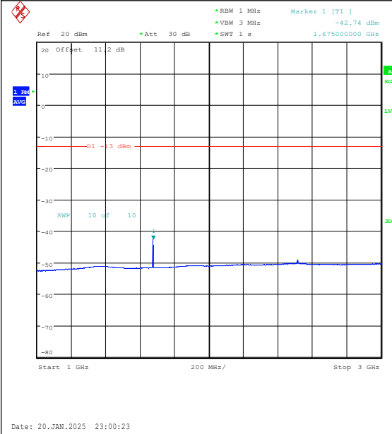
Band5-3MHz-QPSK-20525-1RB#14-1000~3000-P ASS
