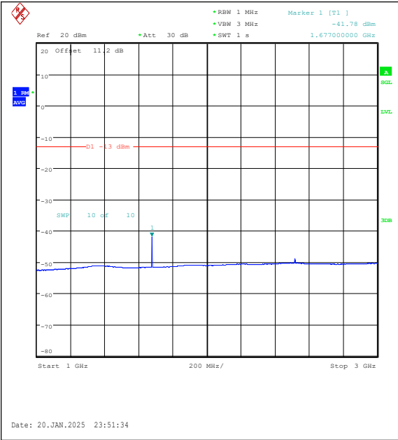
Band5-5MHz-QPSK-20525-1RB#24-1000~3000-P ASS
