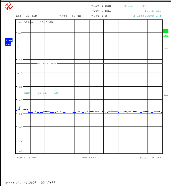
Band5-10MHz-QPSK-20525-1RB#0-3000~10000- PASS
