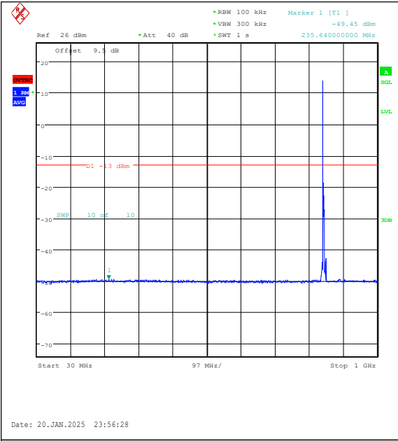
Band5-5MHz-QPSK-20625-1RB#0-30~1000-PAS S
