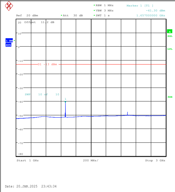
Band5-5MHz-QPSK-20425-1RB#24-1000~3000-P ASS
