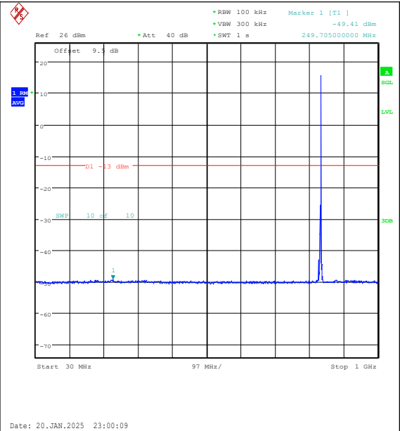
Band5-3MHz-QPSK-20525-1RB#14-30~1000-PA SS
