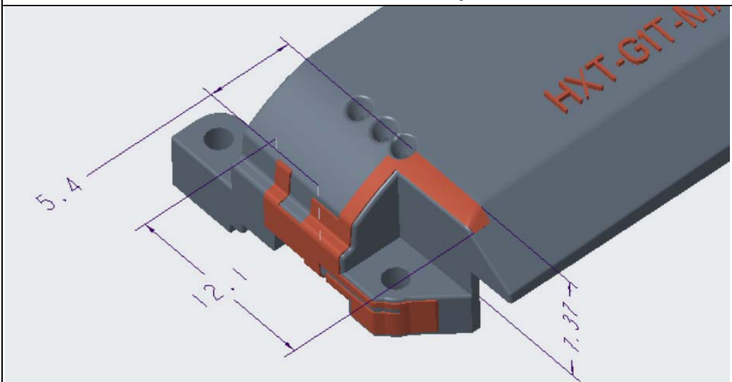
ANT5:12.1*7.37*5.4mm Monopole
