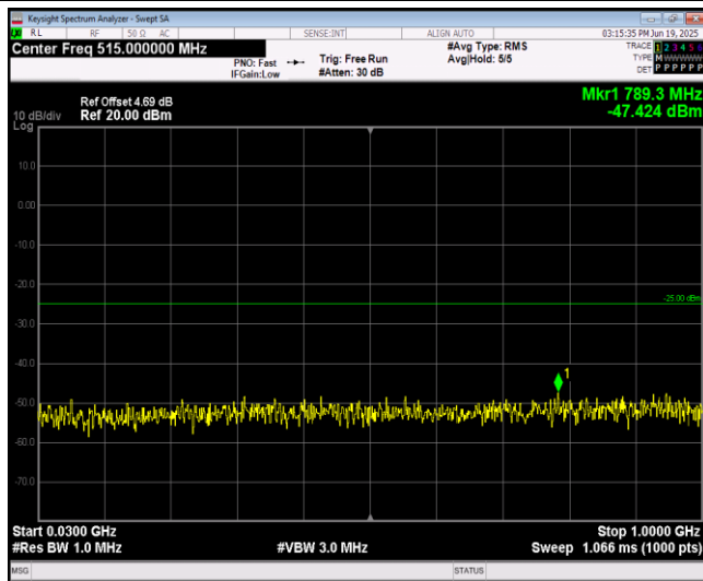
Band38-20MHz-QPSK-38000-1RB#0-Range1:30~1000MHz
