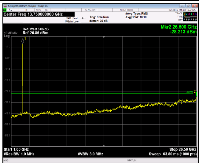
Band38-5MHz-64QAM-37775-1RB#0-Range2:1000~26500MHz
