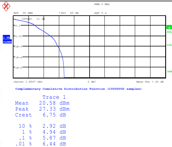
Band2-1.4MHz-QPSK-18607-1RB#0-PASS
