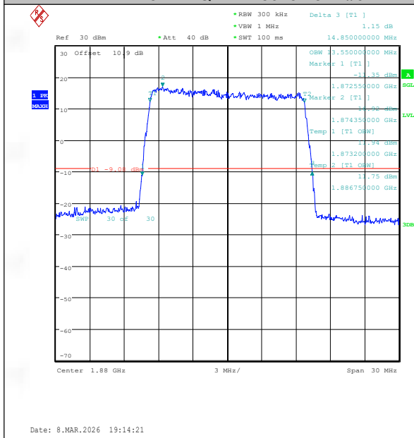
Band2-15MHz-QPSK-18900-75RB#0-PASS
