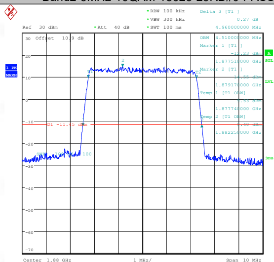
Band2-5MHz-16QAM-18625-25RB#0-PASS
