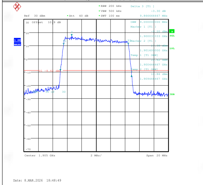
Band2-10MHz-QPSK-19150-50RB#0-PASS
