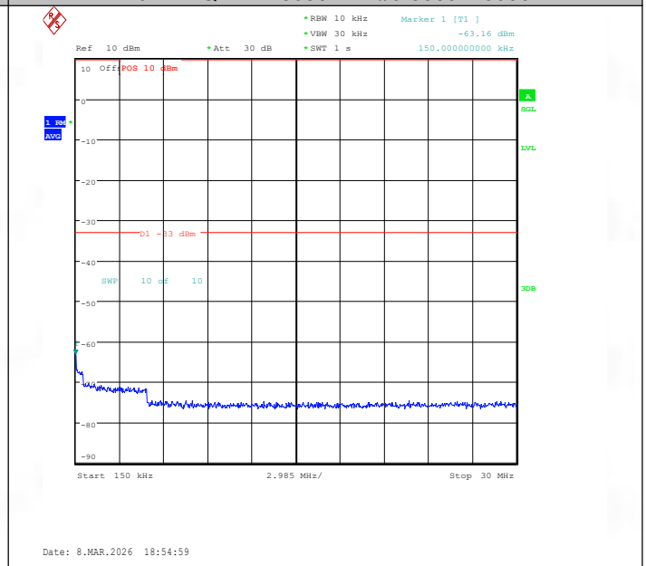
Band2-10MHz-16QAM-18650-1RB#0-0.15~30-PASS
