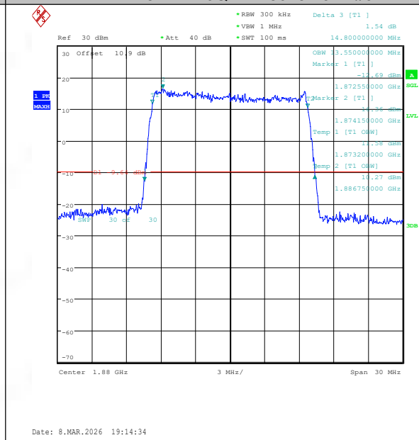
Band2-15MHz-16QAM-18900-75RB#0-PASS
