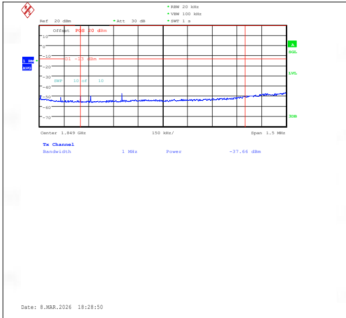
Band2-5MHz-QPSK-18625-1RB#0-1000~3000-PASS
