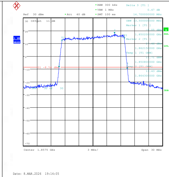
Band2-15MHz-16QAM-18675-75RB#0-PASS
