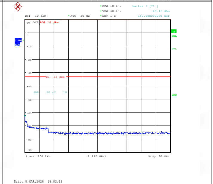
Band2-3MHz-16QAM-18615-1RB#0-0.15~30-PASS
