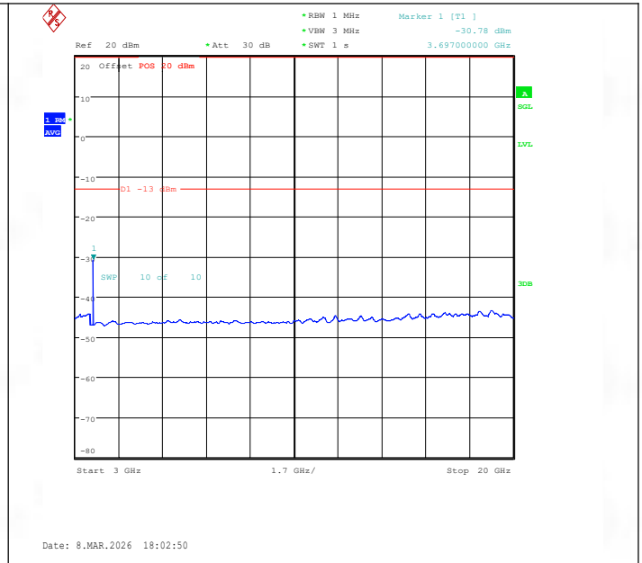
Band2-3MHz-QPSK-18615-1RB#0-3000~20000-PASS
