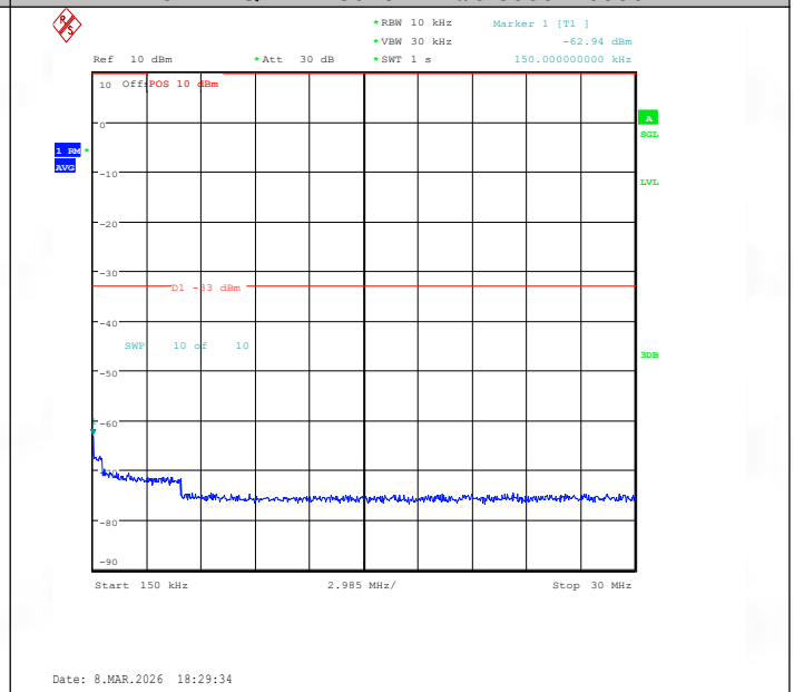
Band2-5MHz-16QAM-18625-1RB#0-0.15~30-PASS
