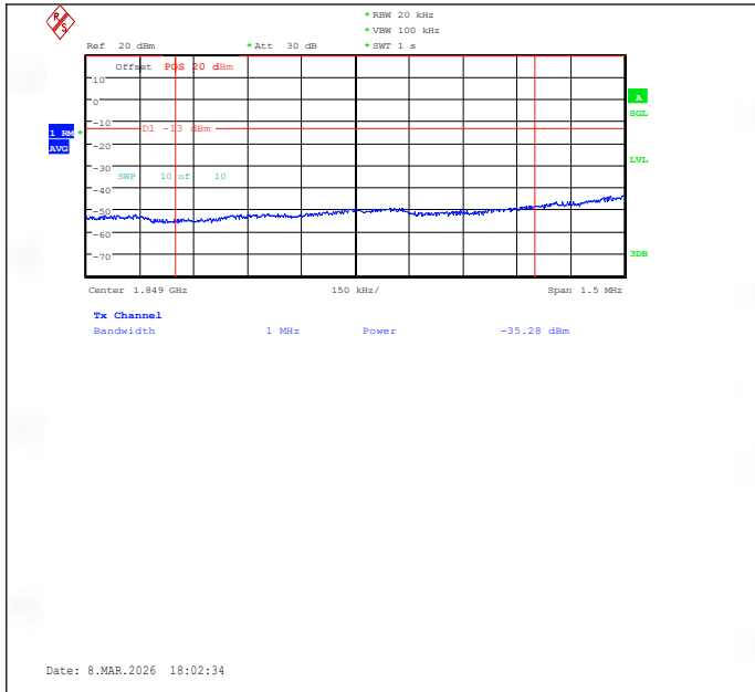
Band2-3MHz-QPSK-18615-1RB#0-1000~3000-PASS
