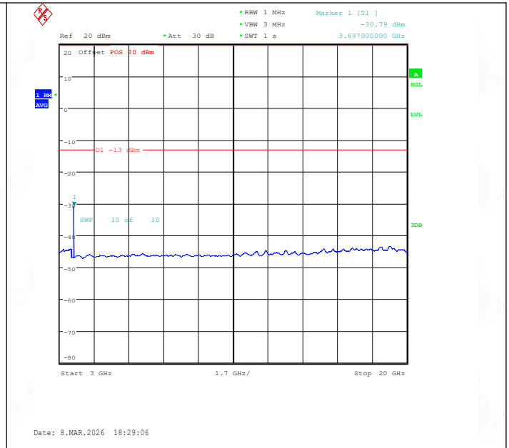
Band2-5MHz-QPSK-18625-1RB#0-3000~20000-PASS
