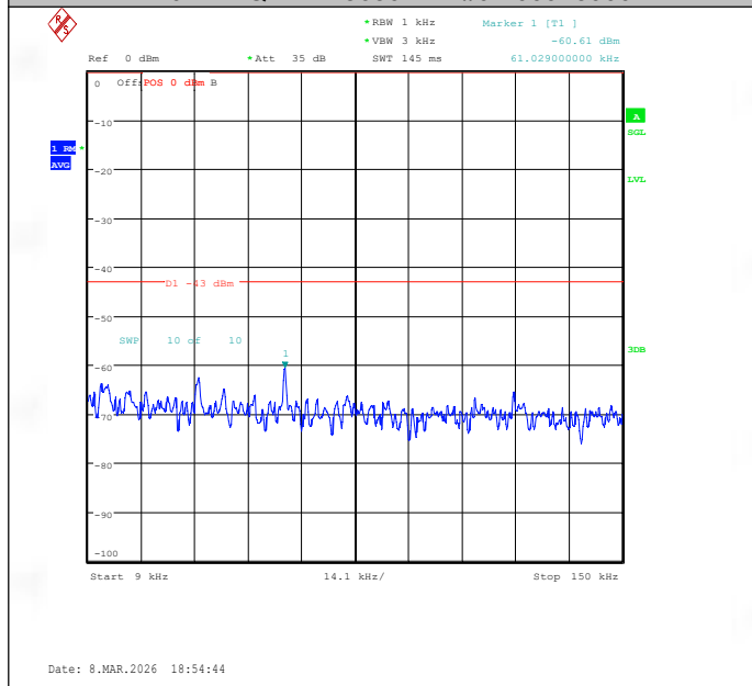
Band2-10MHz-16QAM-18650-1RB#0-0.009~0.15-PASS
