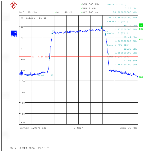
Band2-15MHz-QPSK-18675-75RB#0-PASS
