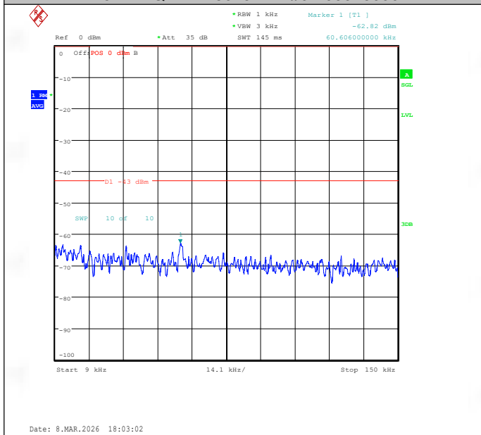
Band2-3MHz-16QAM-18615-1RB#0-0.009~0.15-PASS
