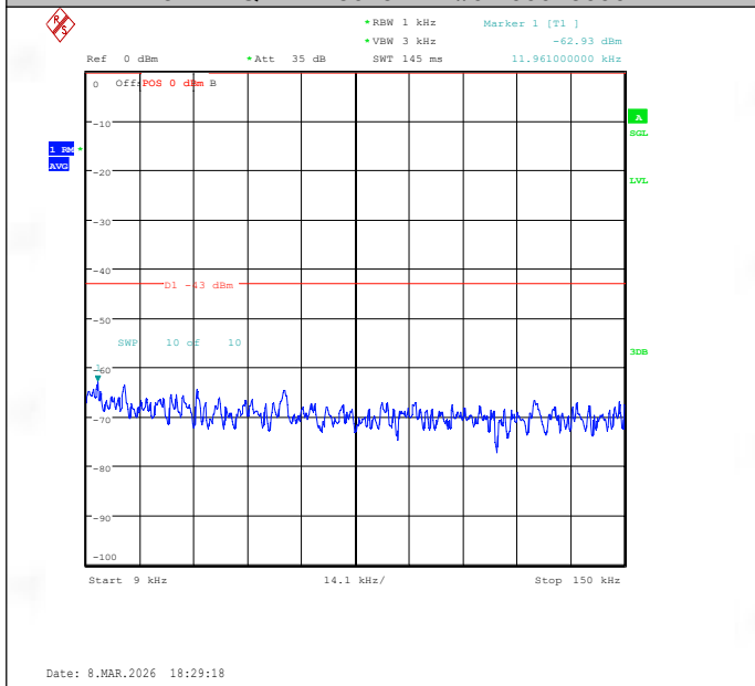
Band2-5MHz-16QAM-18625-1RB#0-0.009~0.15-PASS
