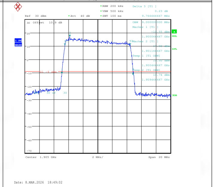
Band2-10MHz-16QAM-19150-50RB#0-PASS
