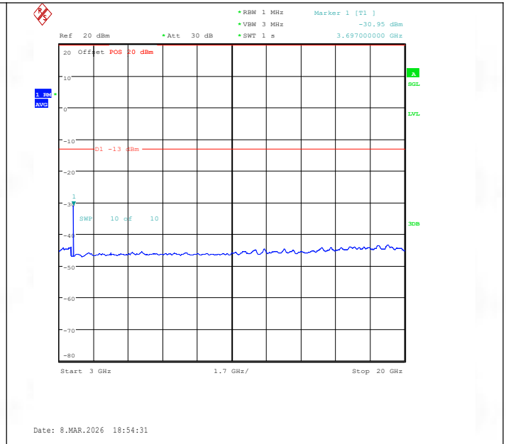
Band2-10MHz-QPSK-18650-1RB#0-3000~20000-PASS
