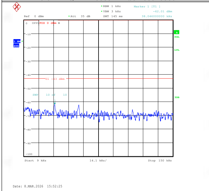
Band25-5MHz-16QAM-26065-1RB#0-0.009~0.15-PASS
