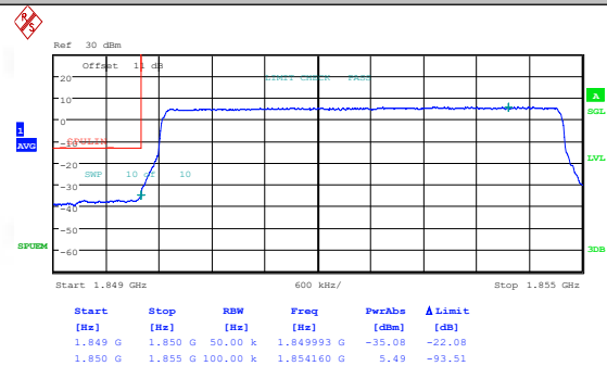
Band25-5MHz-16QAM-26065-1RB#0-PASS
