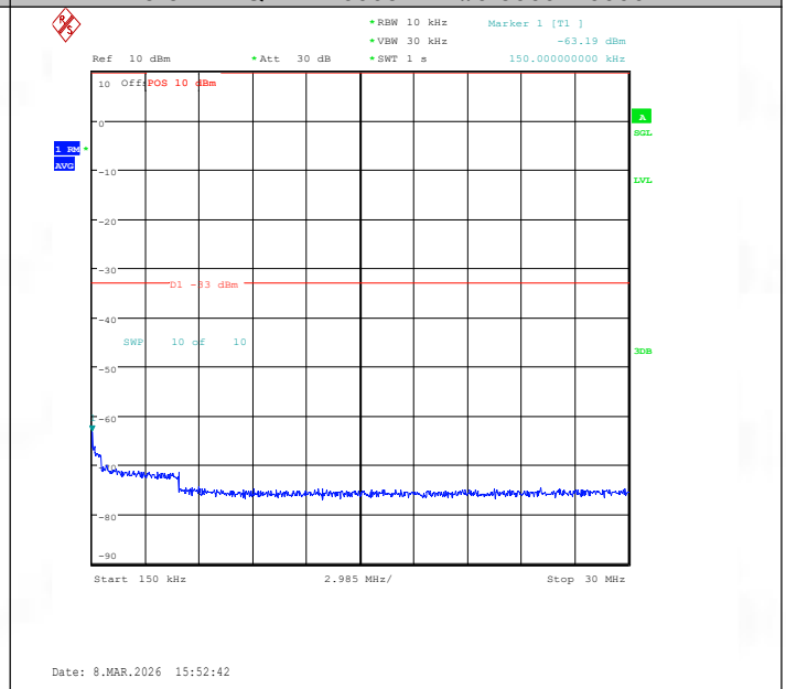
Band25-5MHz-16QAM-26065-1RB#0-0.15~30-PASS
