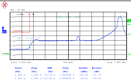
Band25-5MHz-QPSK-26065-25RB#0-PASS
