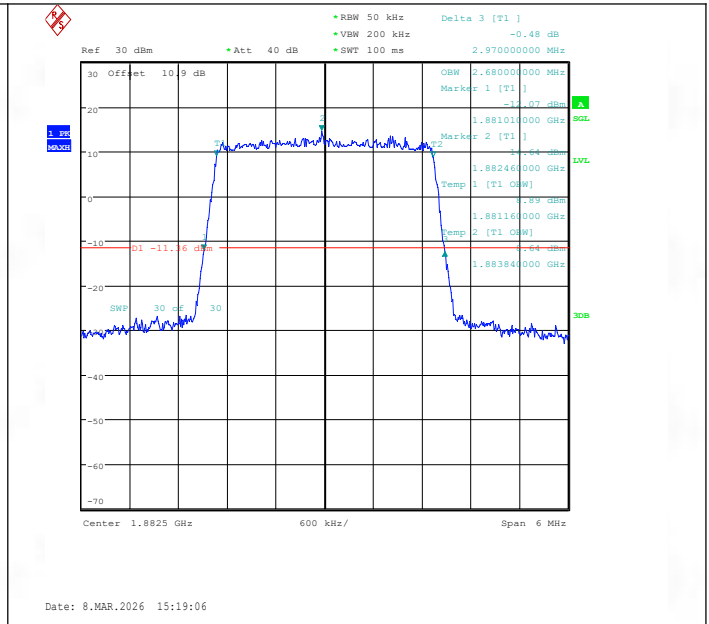
Band25-3MHz-16QAM-26365-15RB#0-PASS
