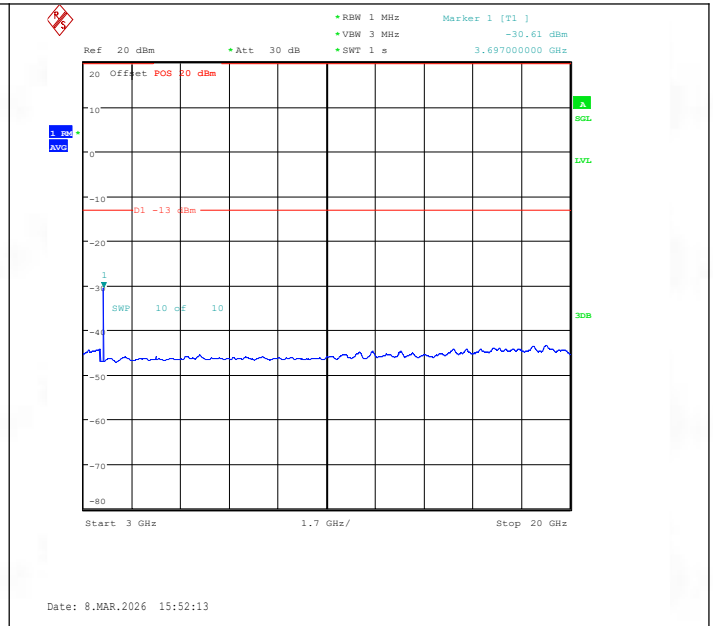
Band25-5MHz-QPSK-26065-1RB#0-3000~20000-PASS
