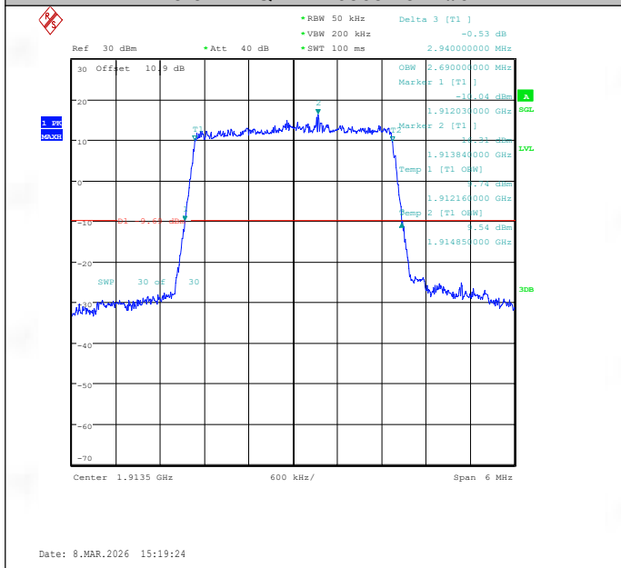
Band25-3MHz-QPSK-26675-15RB#0-PASS
