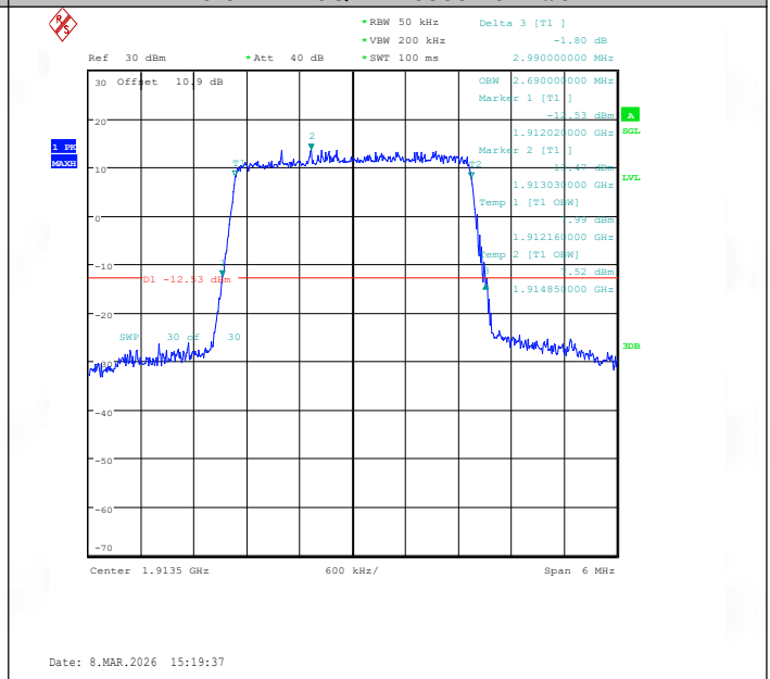
Band25-3MHz-16QAM-26675-15RB#0-PASS
