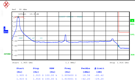
Band25-10MHz-QPSK-26640-1RB#49-PASS
