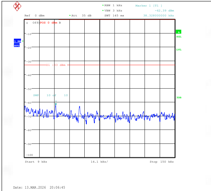
Band26(814-824)-1.4MHz-16QAM-26783-1RB#5-0.009~0.15-PASS
