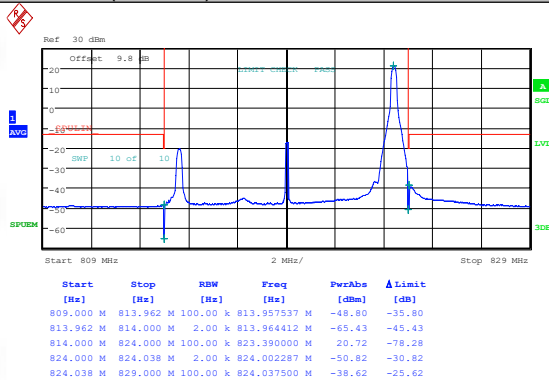
Band26(814-824)-10MHz-QPSK-26740-50RB#0-PASS
