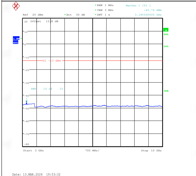
Band26(814-824)-1.4MHz-QPSK-26740-1RB#0-3000~10000-PASS
