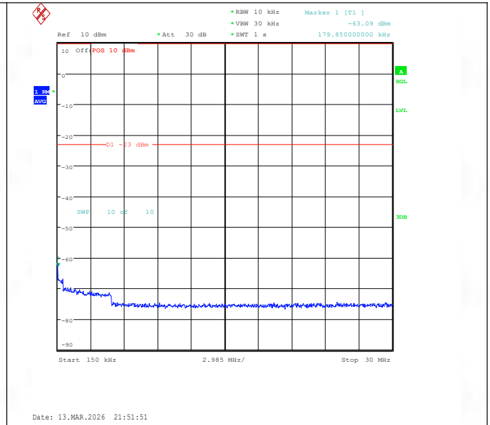
Band26(814-824)-3MHz-QPSK-26705-15RB#0-0.15~30-PASS
