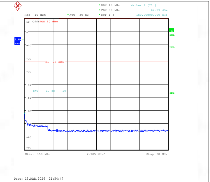
Band26(814-824)-3MHz-QPSK-26740-1RB#0-0.15~30-PASS
