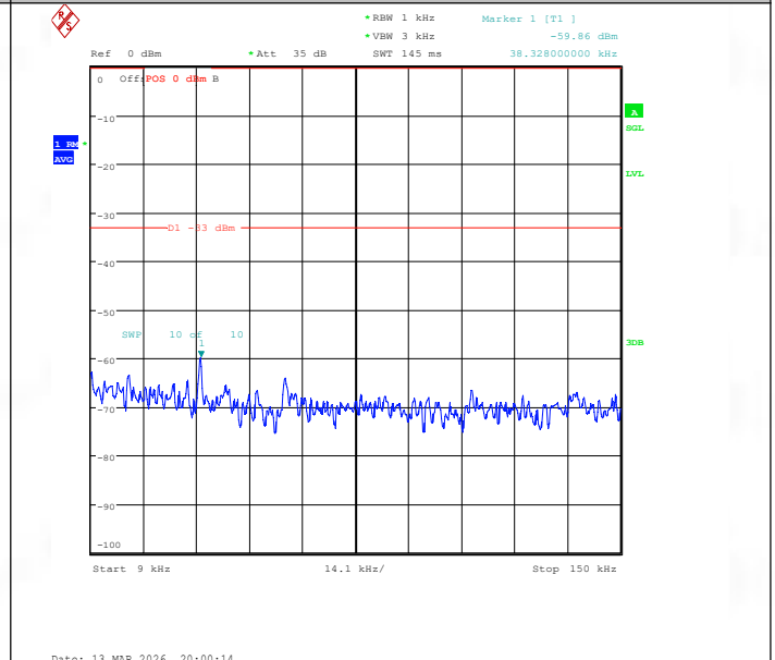
Band26(814-824)-1.4MHz-16QAM-26740-6RB#0-0.009~0.15-PASS
