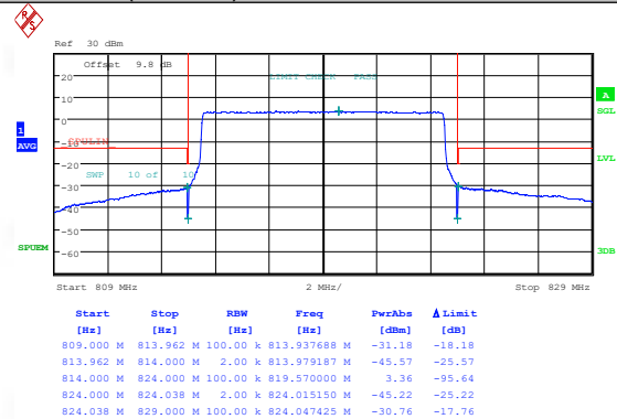
Band26(814-824)-10MHz-16QAM-26740-1RB#0-PASS
