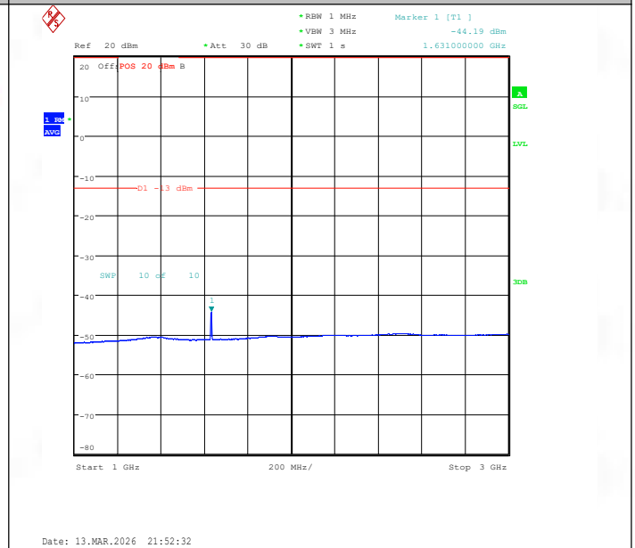
Band26(814-824)-3MHz-QPSK-26705-15RB#0-1000~3000-PASS
