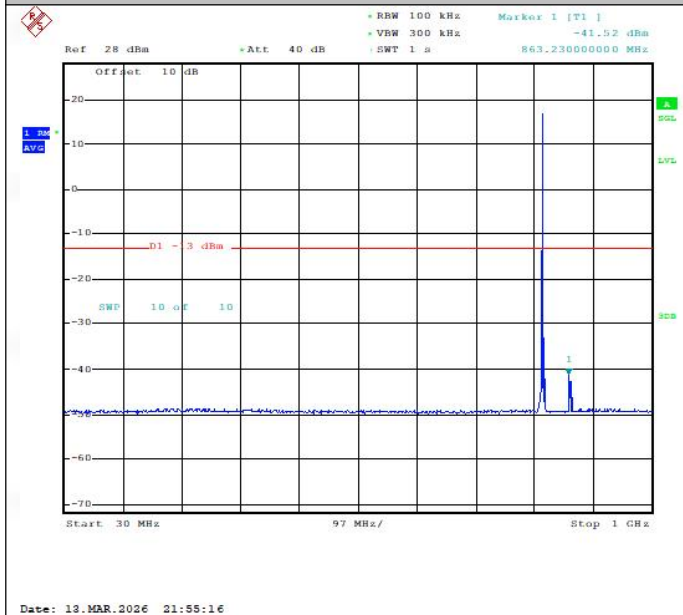
Band26(814-824)-3MHz-QPSK-26740-1RB#0-30~1000-PASS
