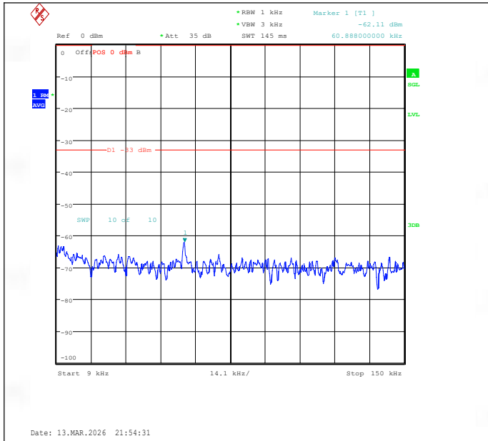
Band26(814-824)-3MHz-QPSK-26740-1RB#0-0.009~0.15-PASS
