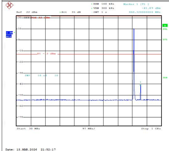
Band26(814-824)-3MHz-QPSK-26705-15RB#0-30~1000-PASS
