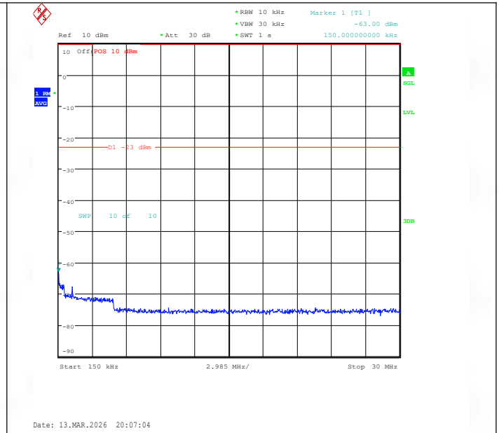
Band26(814-824)-1.4MHz-16QAM-26783-1RB#5-0.15~30-PASS
