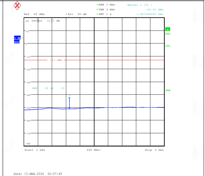
Band26(814-824)-1.4MHz-16QAM-26783-1RB#5-1000~3000-PASS
