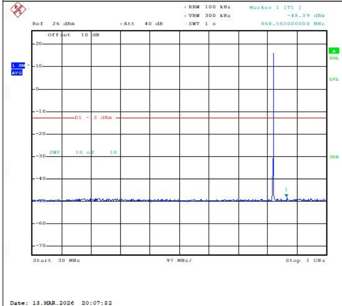
Band26(814-824)-1.4MHz-16QAM-26783-1RB#5-30~1000-PASS
