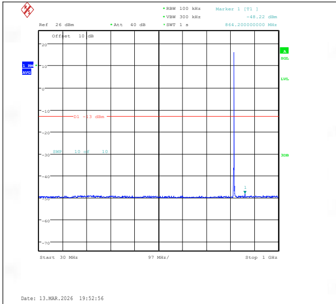
Band26(814-824)-1.4MHz-QPSK-26740-1RB#0-30~1000-PASS
