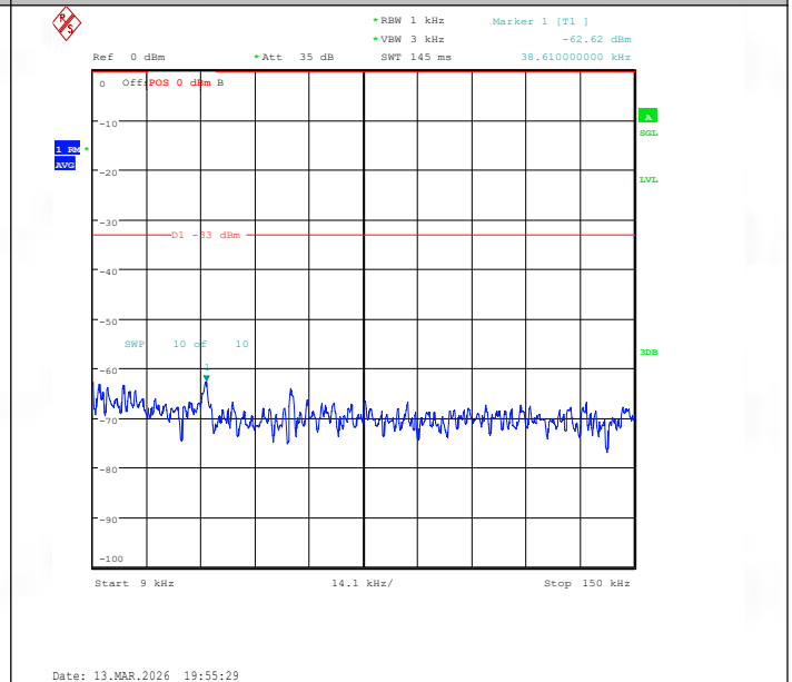
Band26(814-824)-1.4MHz-QPSK-26740-1RB#5-0.009~0.15-PASS
