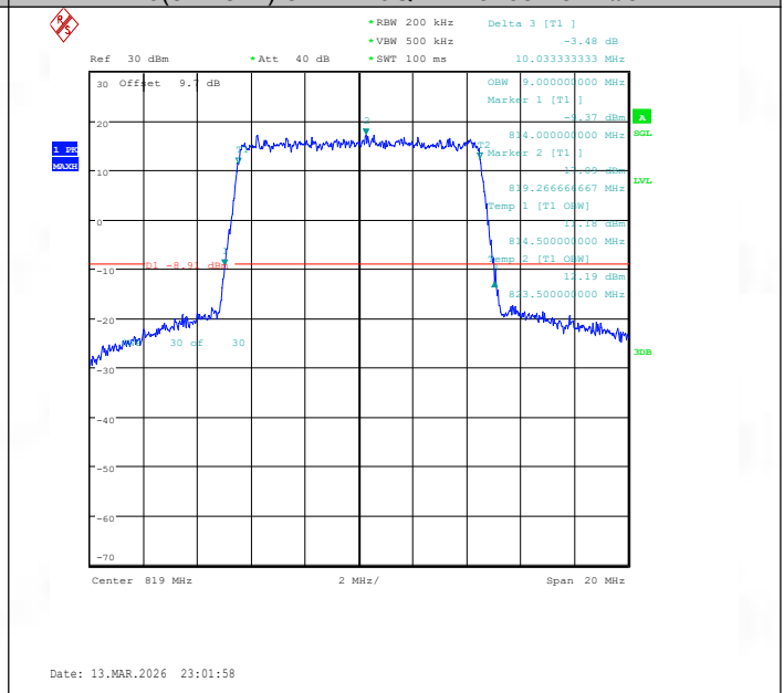
Band26(814-824)-10MHz-16QAM-26740-50RB#0-PASS
