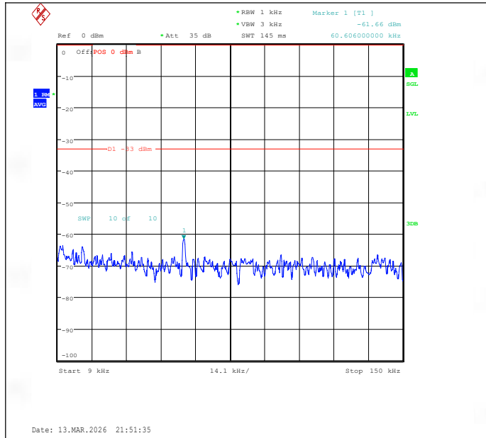
Band26(814-824)-3MHz-QPSK-26705-15RB#0-0.009~0.15-PASS
