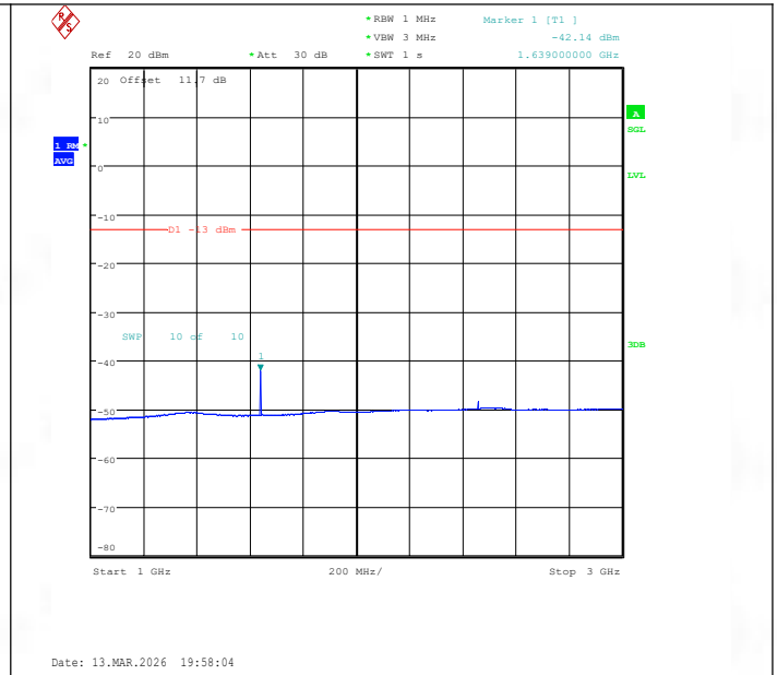
Band26(814-824)-1.4MHz-16QAM-26740-1RB#5-1000~3000-PASS
