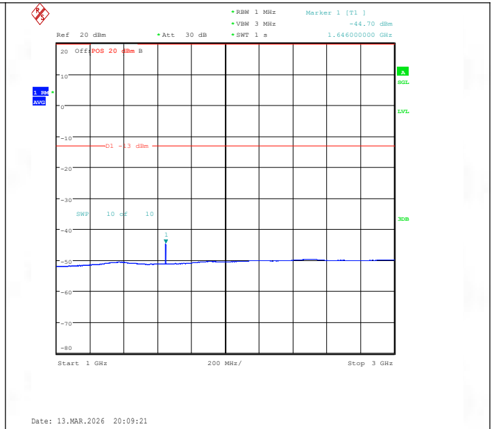
Band26(814-824)-1.4MHz-QPSK-26783-6RB#0-1000~3000-PASS
