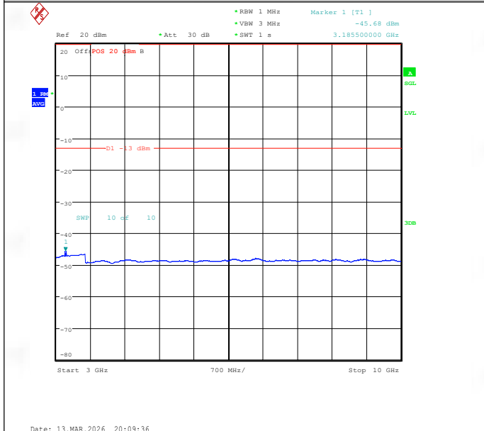
Band26(814-824)-1.4MHz-QPSK-26783-6RB#0-3000~10000-PASS
