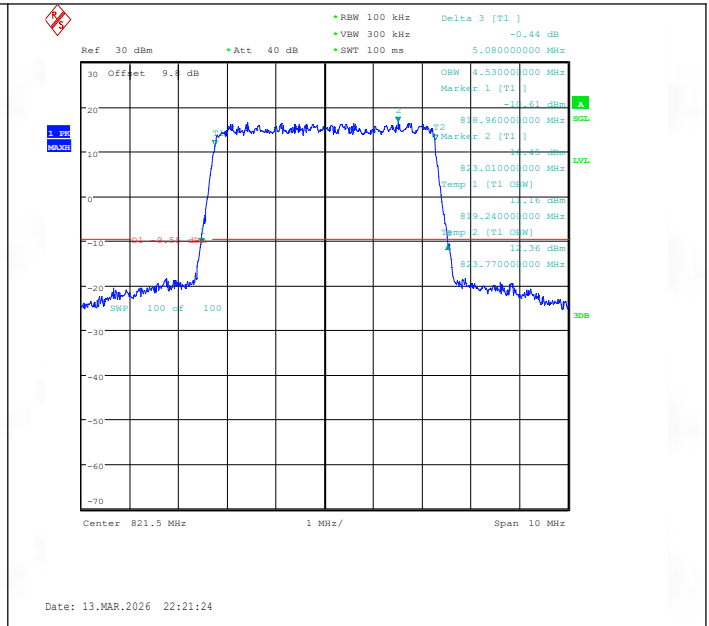
Band26(814-824)-5MHz-16QAM-26765-25RB#0-PASS
