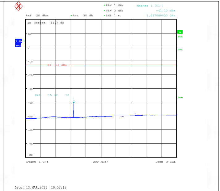
Band26(814-824)-1.4MHz-QPSK-26740-1RB#0-1000~3000-PASS
