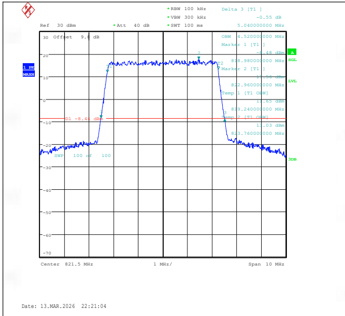
Band26(814-824)-5MHz-QPSK-26765-25RB#0-PASS
