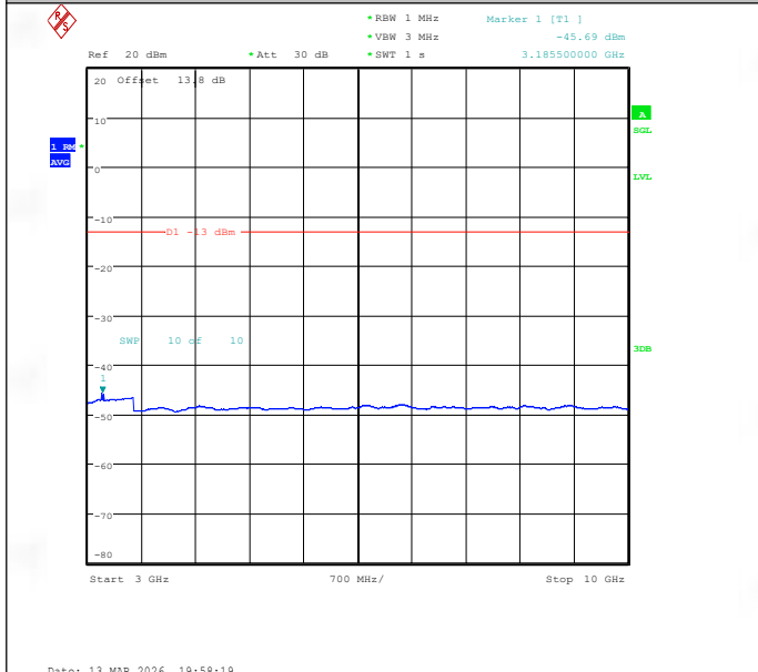
Band26(814-824)-1.4MHz-16QAM-26740-1RB#5-3000~10000-PASS
