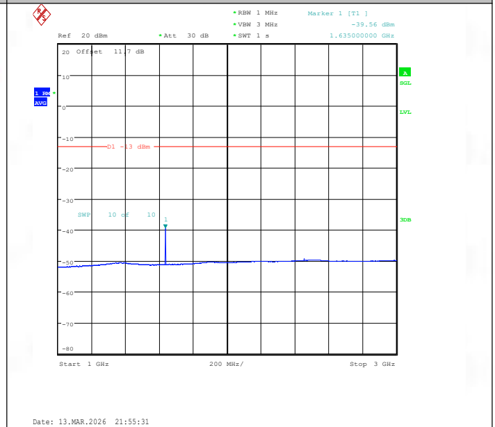
Band26(814-824)-3MHz-QPSK-26740-1RB#0-1000~3000-PASS
