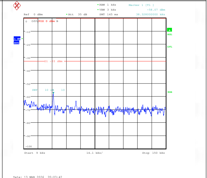
Band26(814-824)-1.4MHz-16QAM-26783-1RB#0-0.009~0.15-PASS
