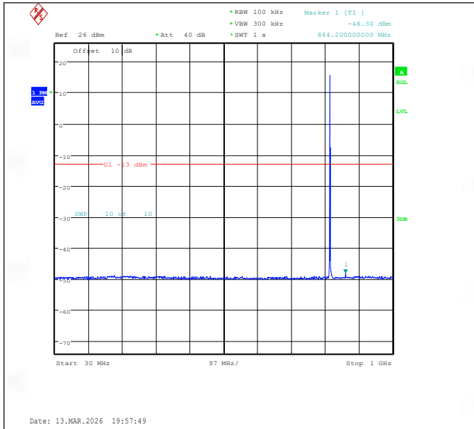
Band26(814-824)-1.4MHz-16QAM-26740-1RB#5-30~1000-PASS
