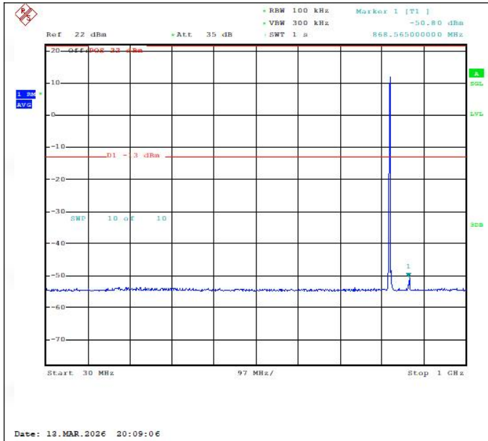
Band26(814-824)-1.4MHz-QPSK-26783-6RB#0-30~1000-PASS
