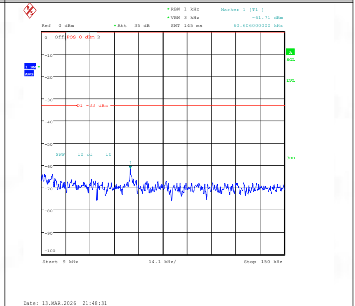
Band26(814-824)-3MHz-QPSK-26705-1RB#14-0.009~0.15-PASS
