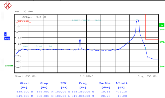
Band26(824-849)-10MHz-16QAM-26840-50RB#0-PASS
