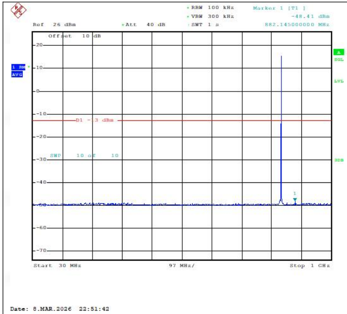
Band26(824-849)-1.4MHz-QPSK-26915-1RB#0-30~1000-PASS
