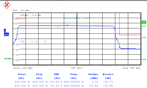
Band26(824-849)-5MHz-16QAM-27015-1RB#0-PASS
