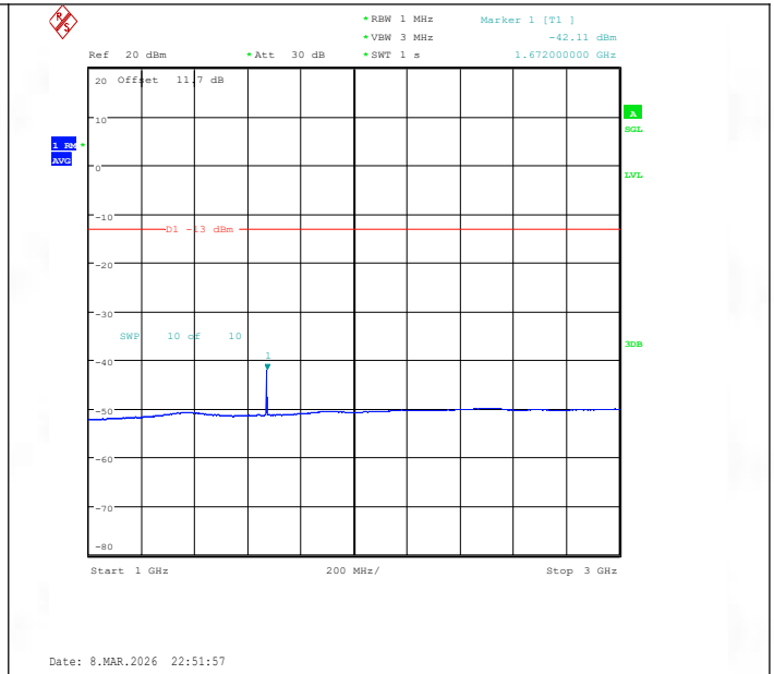
Band26(824-849)-1.4MHz-QPSK-26915-1RB#0-1000~3000-PASS
