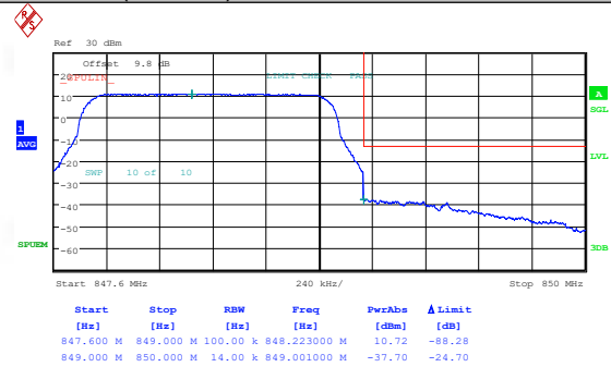
Band26(824-849)-1.4MHz-16QAM-27033-1RB#0-PASS
