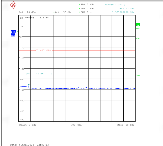
Band26(824-849)-1.4MHz-QPSK-26915-1RB#0-3000~10000-PASS
