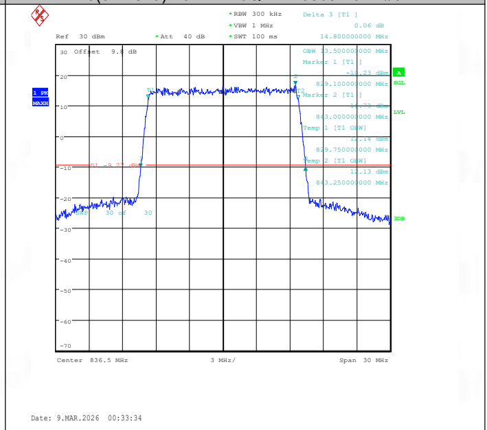
Band26(824-849)-15MHz-16QAM-26915-75RB#0-PASS
