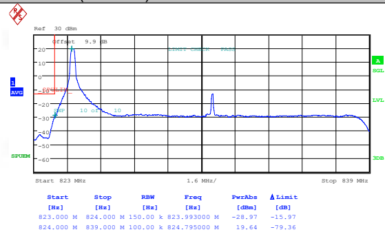
Band26(824-849)-15MHz-QPSK-26865-1RB#74-PASS
