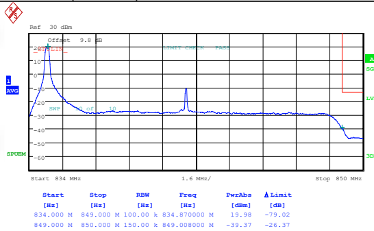
Band26(824-849)-15MHz-16QAM-26865-1RB#74-PASS
