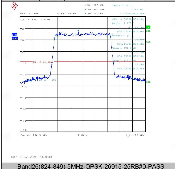
Band26(824-849)-5MHz-QPSK-26915-25RB#0-PASS
