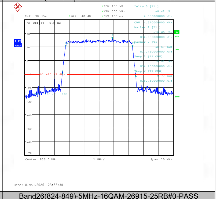
Band26(824-849)-5MHz-16QAM-26915-25RB#0-PASS
