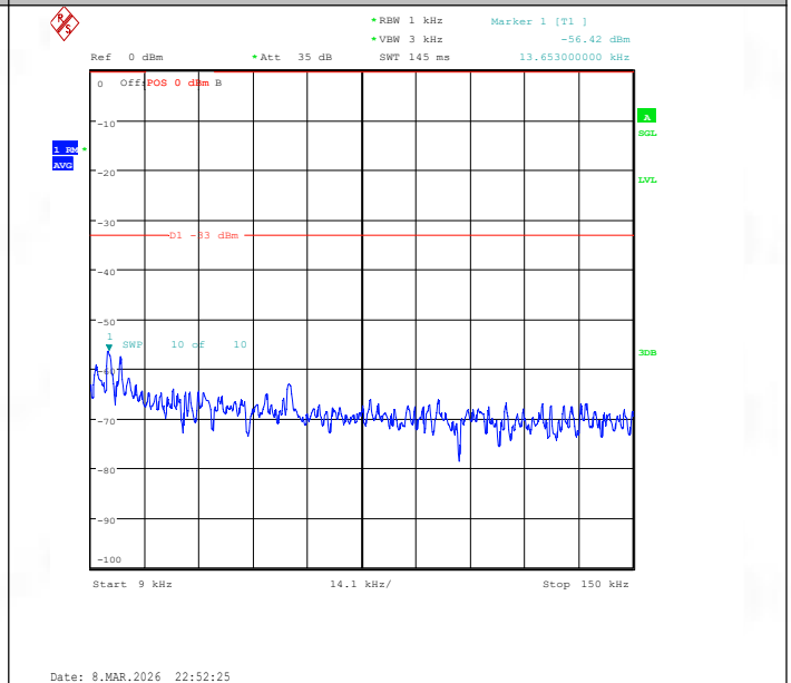
Band26(824-849)-1.4MHz-16QAM-26915-1RB#0-0.009~0.15-PASS
