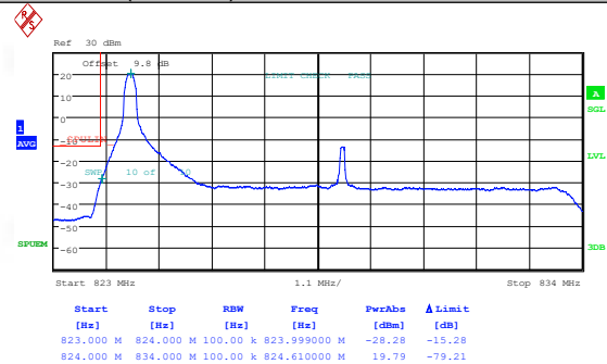
Band26(824-849)-10MHz-QPSK-26840-1RB#49-PASS
