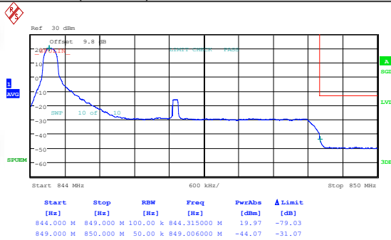
Band26(824-849)-5MHz-16QAM-26815-1RB#24-PASS
