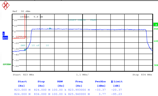
Band26(824-849)-10MHz-QPSK-26840-1RB#0-PASS
