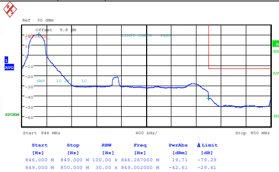
Band26(824-849)-3MHz-16QAM-26805-1RB#14-PASS
