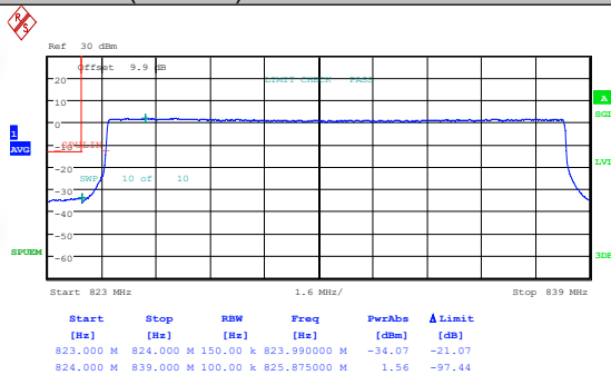
Band26(824-849)-15MHz-QPSK-26865-1RB#0-PASS
