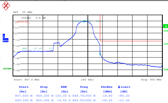
Band26(824-849)-1.4MHz-QPSK-27033-6RB#0-PASS
