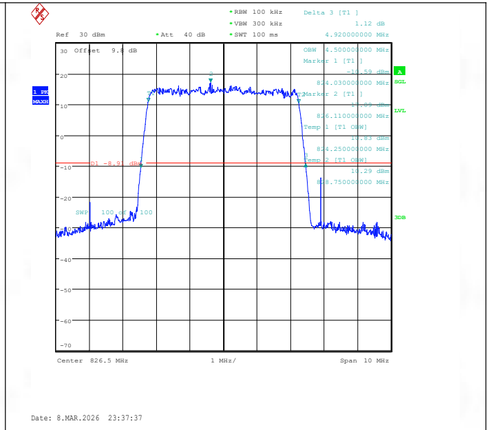
Band26(824-849)-5MHz-16QAM-26815-25RB#0-PASS
