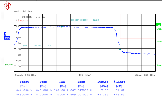
Band26(824-849)-3MHz-16QAM-27025-1RB#0-PASS
