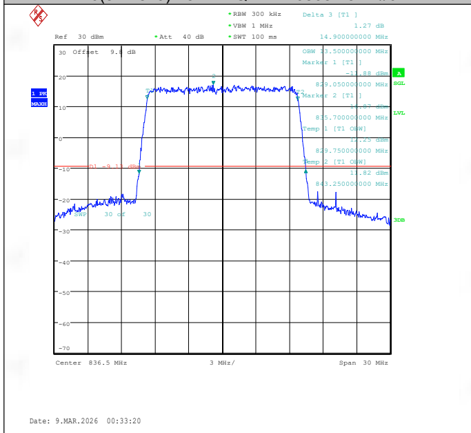
Band26(824-849)-15MHz-QPSK-26915-75RB#0-PASS
