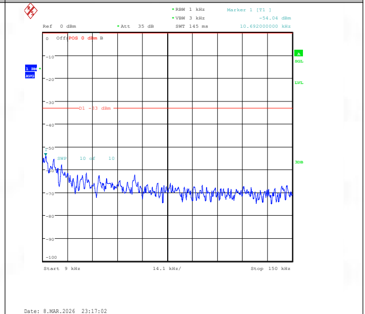
Band26(824-849)-3MHz-16QAM-26805-1RB#0-0.009~0.15-PASS
