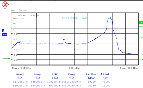
Band26(824-849)-5MHz-QPSK-27015-25RB#0-PASS
