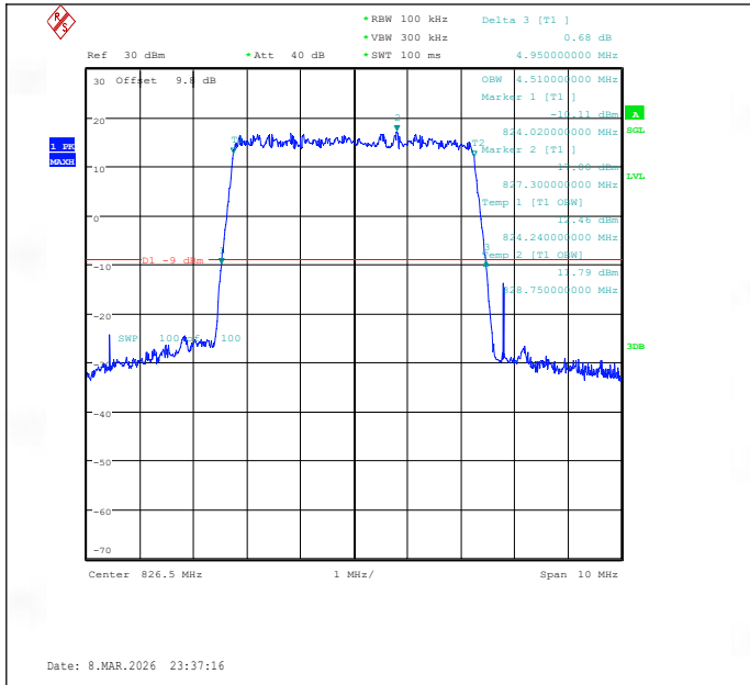
Band26(824-849)-5MHz-QPSK-26815-25RB#0-PASS
