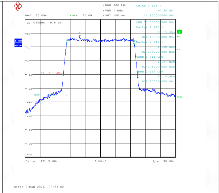
Band26(824-849)-15MHz-16QAM-26865-75RB#0-PASS
