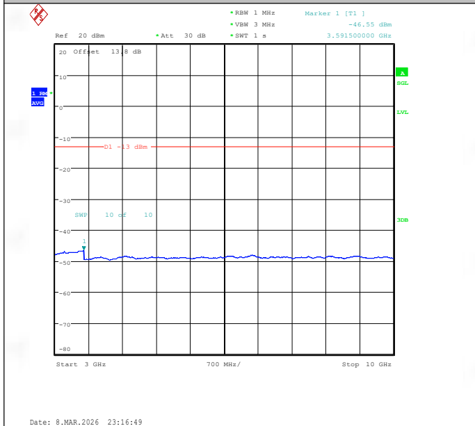
Band26(824-849)-3MHz-QPSK-26805-1RB#0-3000~10000-PASS
