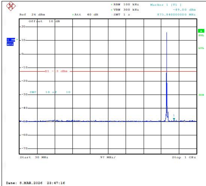
Band26(824-849)-5MHz-QPSK-26915-1RB#0-30~1000-PASS
