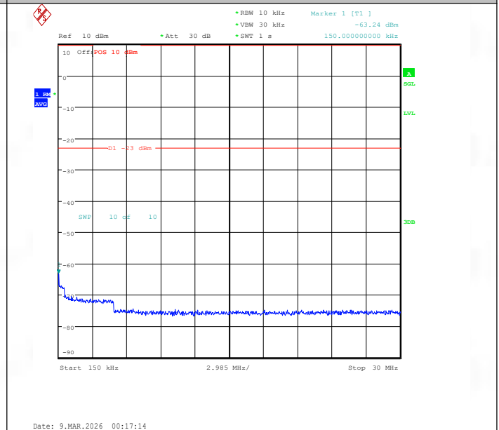
Band26(824-849)-10MHz-QPSK-26990-1RB#0-0.15~30-PASS
