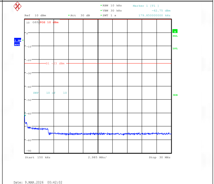
Band26(824-849)-15MHz-QPSK-26915-1RB#0-0.15~30-PASS
