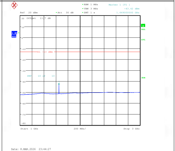
Band26(824-849)-5MHz-QPSK-26815-1RB#0-1000~3000-PASS
