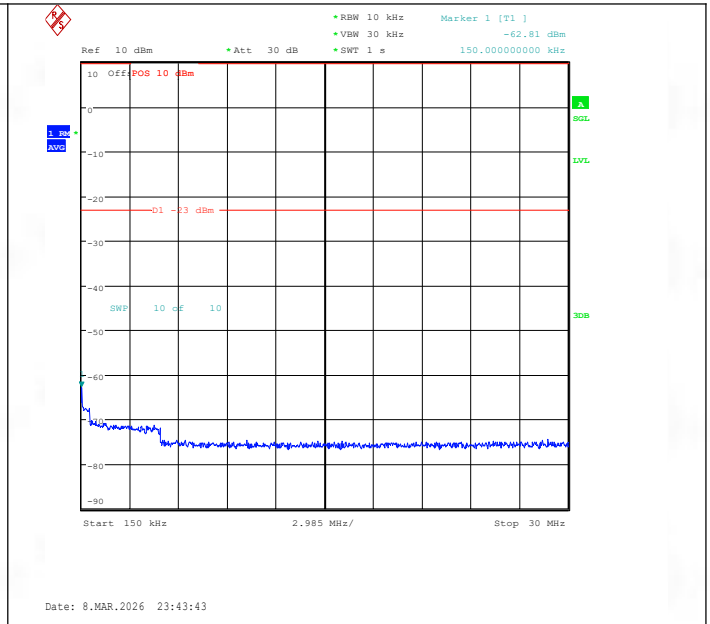
Band26(824-849)-5MHz-QPSK-26815-1RB#0-0.15~30-PASS
