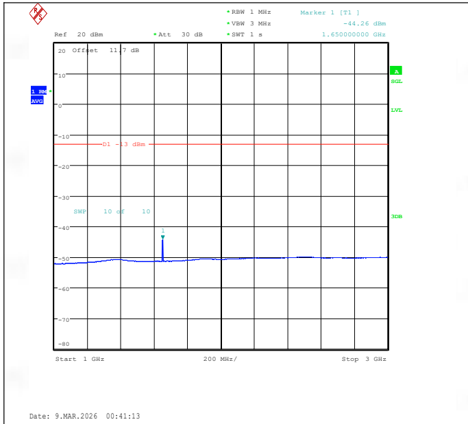
Band26(824-849)-15MHz-16QAM-26865-1RB#0-1000~3000-PASS
