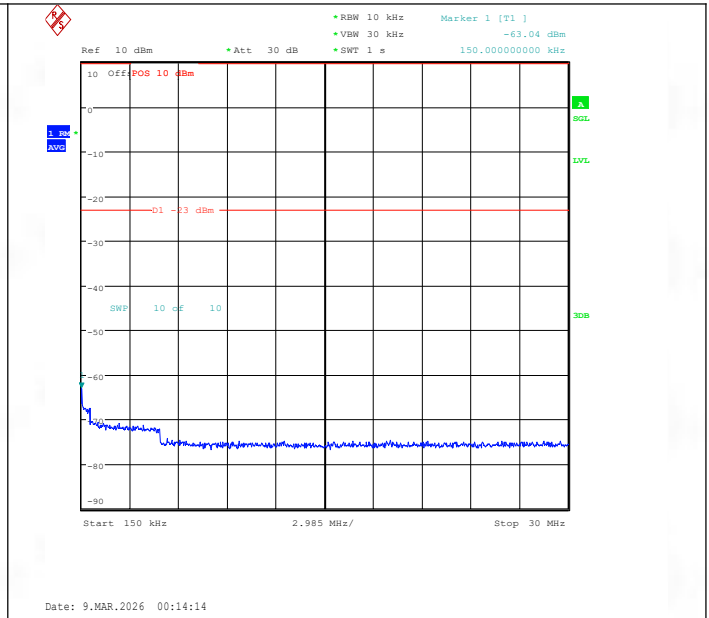
Band26(824-849)-10MHz-QPSK-26915-1RB#0-0.15~30-PASS
