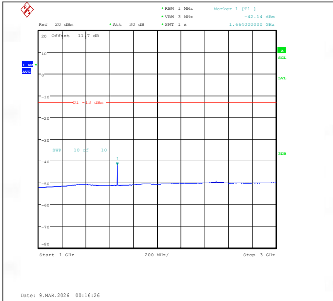
Band26(824-849)-10MHz-16QAM-26915-1RB#0-1000~3000-PASS
