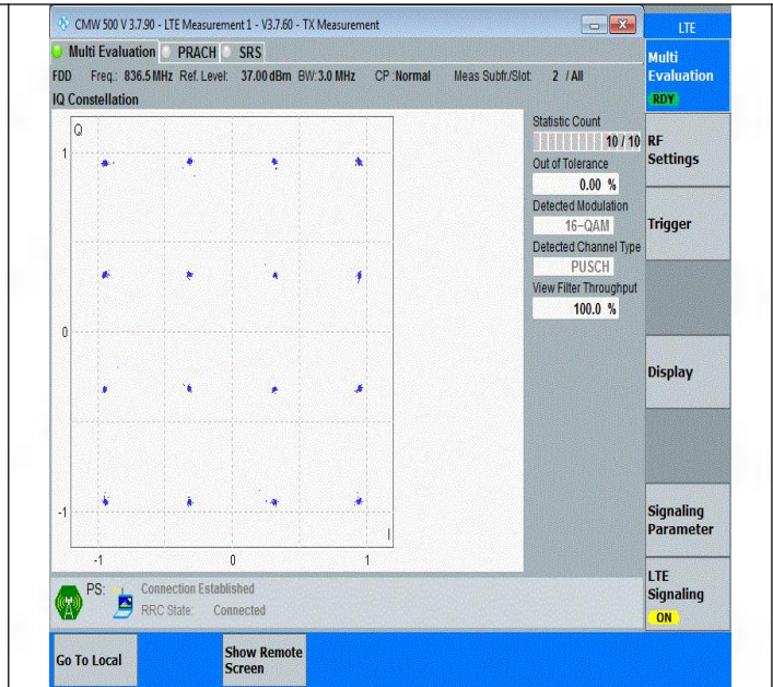
Band26(824-849)-3MHz-16QAM-26915-15RB#0-PASS
