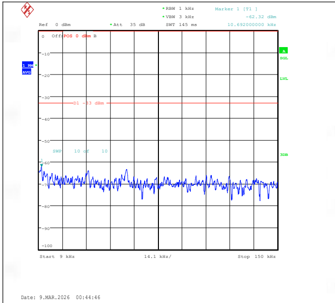
Band26(824-849)-15MHz-QPSK-26965-1RB#0-0.009~0.15-PASS
