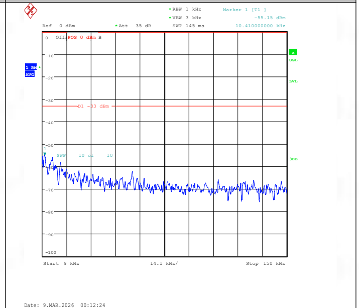
Band26(824-849)-10MHz-16QAM-26840-1RB#0-0.009~0.15-PASS
