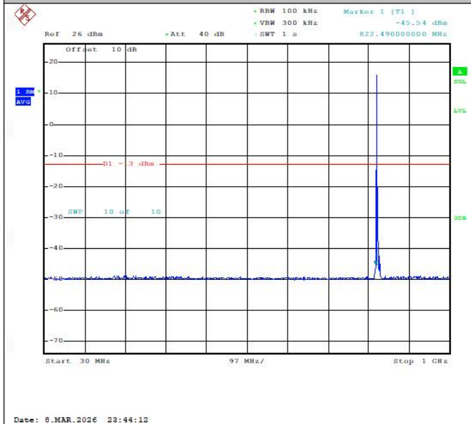
Band26(824-849)-5MHz-QPSK-26815-1RB#0-30~1000-PASS
