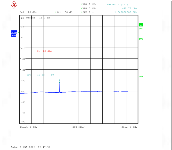
Band26(824-849)-5MHz-QPSK-26915-1RB#0-1000~3000-PASS
