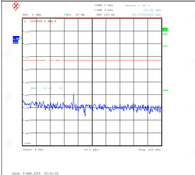
Band26(824-849)-15MHz-QPSK-26915-1RB#0-0.009~0.15-PASS
