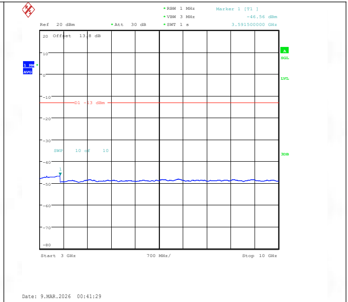
Band26(824-849)-15MHz-16QAM-26865-1RB#0-3000~10000-PASS
