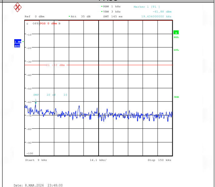
Band26(824-849)-5MHz-16QAM-26915-1RB#0-0.009~0.15-PASS
