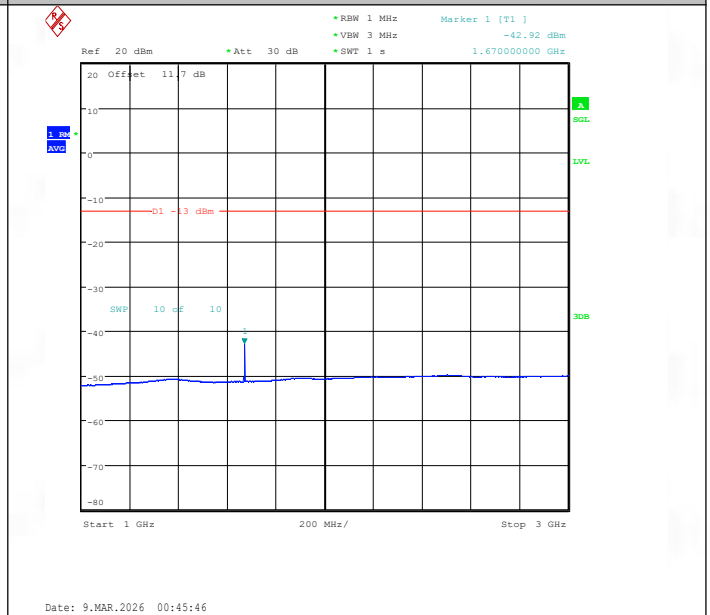
Band26(824-849)-15MHz-QPSK-26965-1RB#0-1000~3000-PASS
