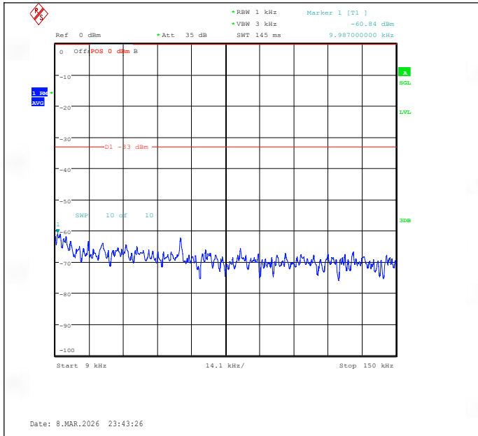
Band26(824-849)-5MHz-QPSK-26815-1RB#0-0.009~0.15-PASS
