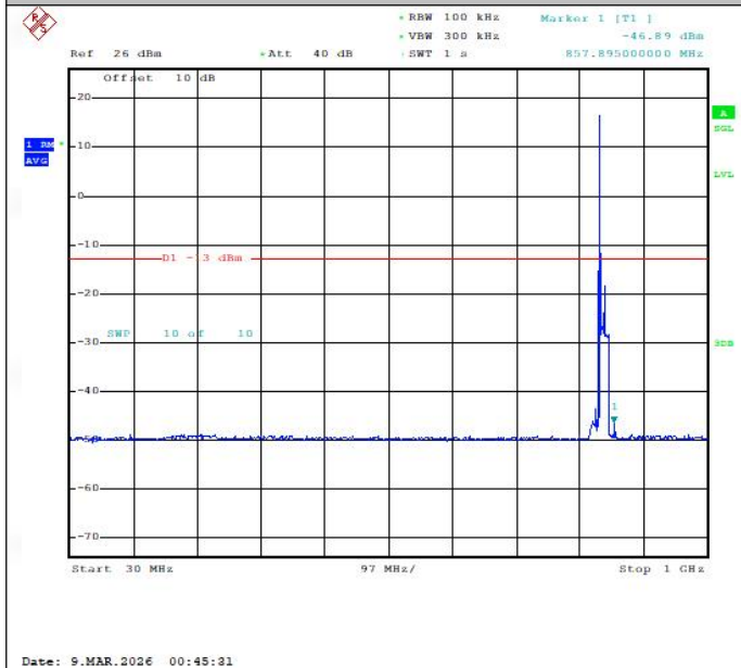
Band26(824-849)-15MHz-QPSK-26965-1RB#0-30~1000-PASS
