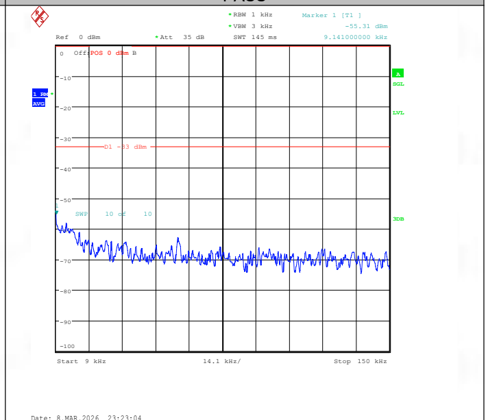
Band26(824-849)-3MHz-16QAM-27025-1RB#0-0.009~0.15-PASS
