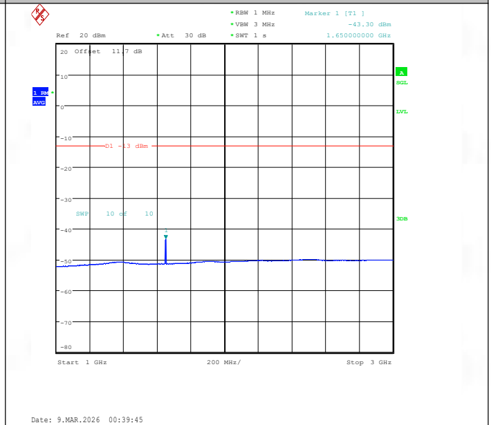
Band26(824-849)-15MHz-QPSK-26865-1RB#0-1000~3000-PASS
