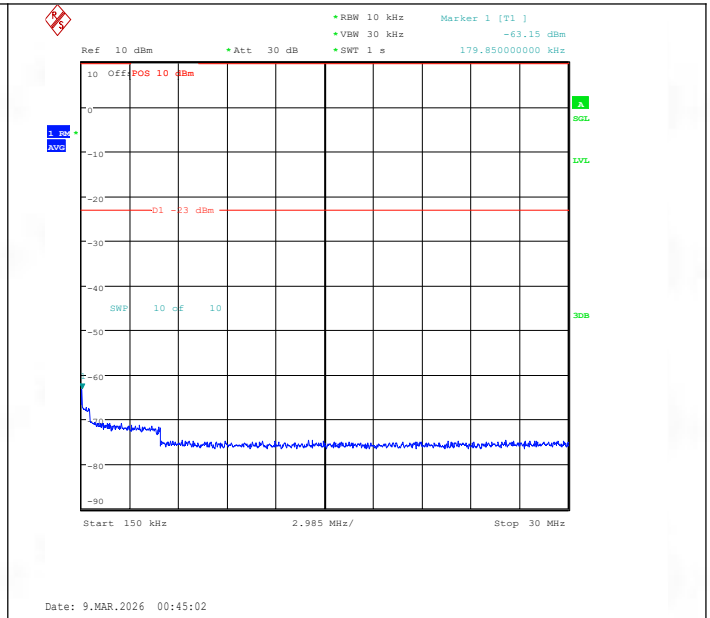
Band26(824-849)-15MHz-QPSK-26965-1RB#0-0.15~30-PASS
