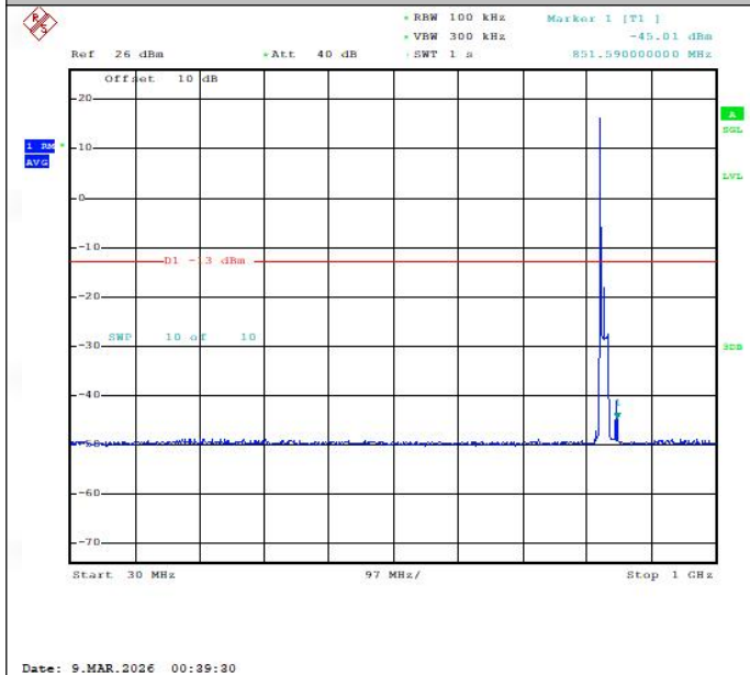
Band26(824-849)-15MHz-QPSK-26865-1RB#0-30~1000-PASS
