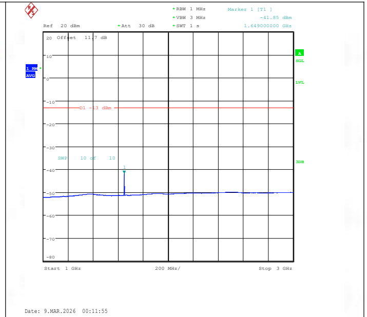
Band26(824-849)-10MHz-QPSK-26840-1RB#0-1000~3000-PASS
