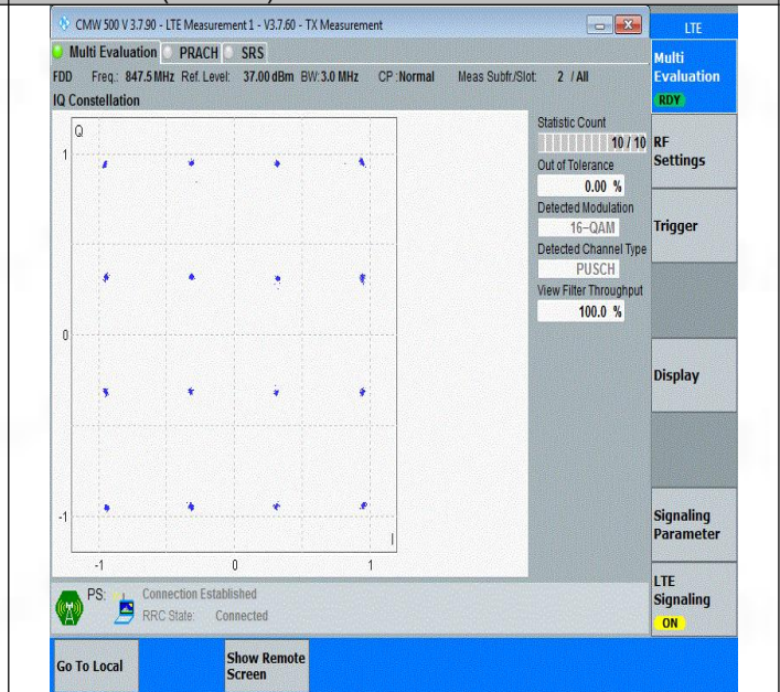
Band26(824-849)-3MHz-16QAM-27025-15RB#0-PASS
