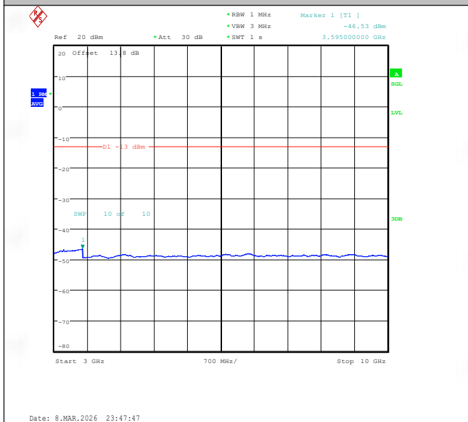
Band26(824-849)-5MHz-QPSK-26915-1RB#0-3000~10000-PASS
