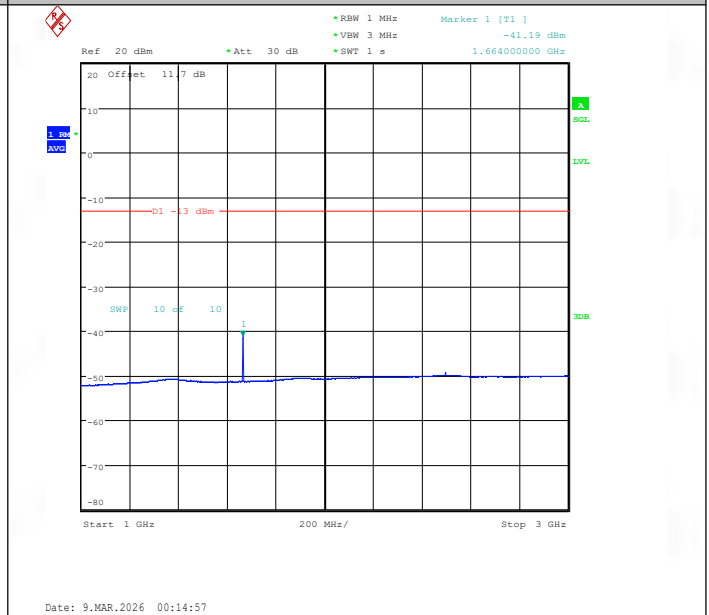
Band26(824-849)-10MHz-QPSK-26915-1RB#0-1000~3000-PASS
