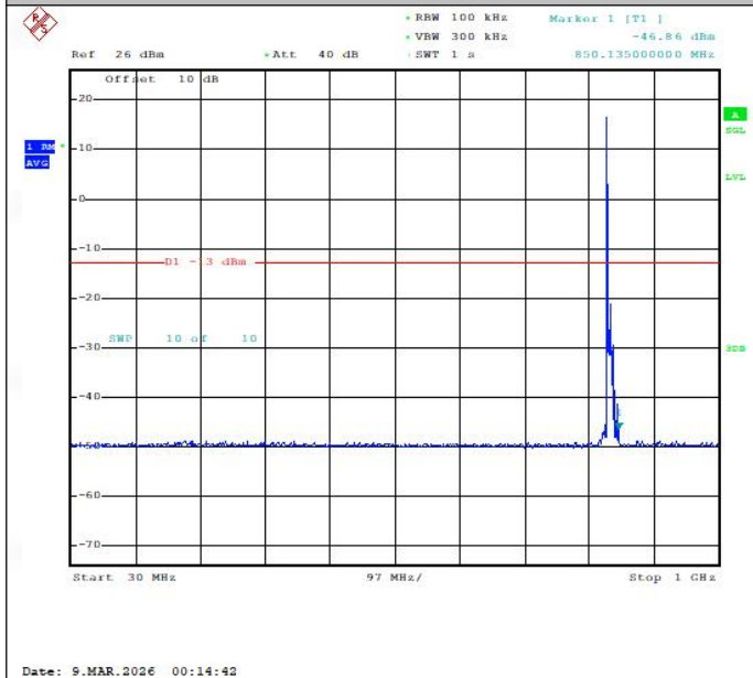
Band26(824-849)-10MHz-QPSK-26915-1RB#0-30~1000-PASS
