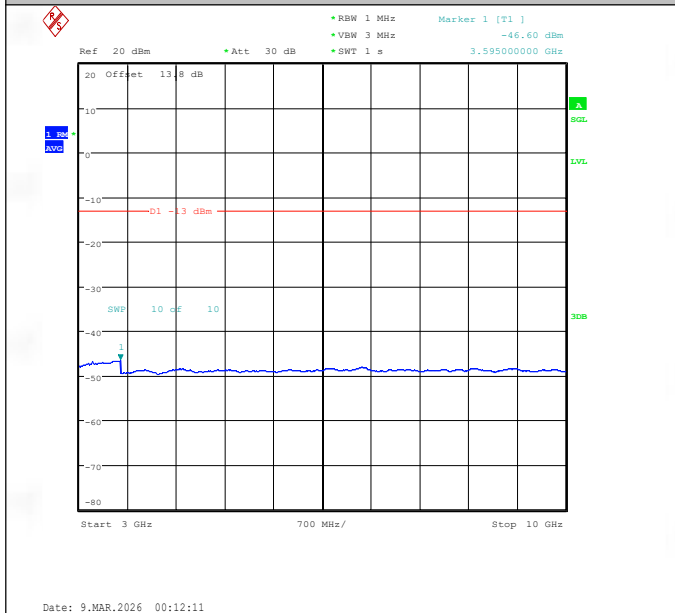
Band26(824-849)-10MHz-QPSK-26840-1RB#0-3000~10000-PASS
