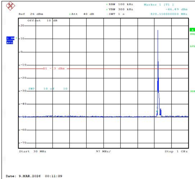
Band26(824-849)-10MHz-QPSK-26840-1RB#0-30~1000-PASS
