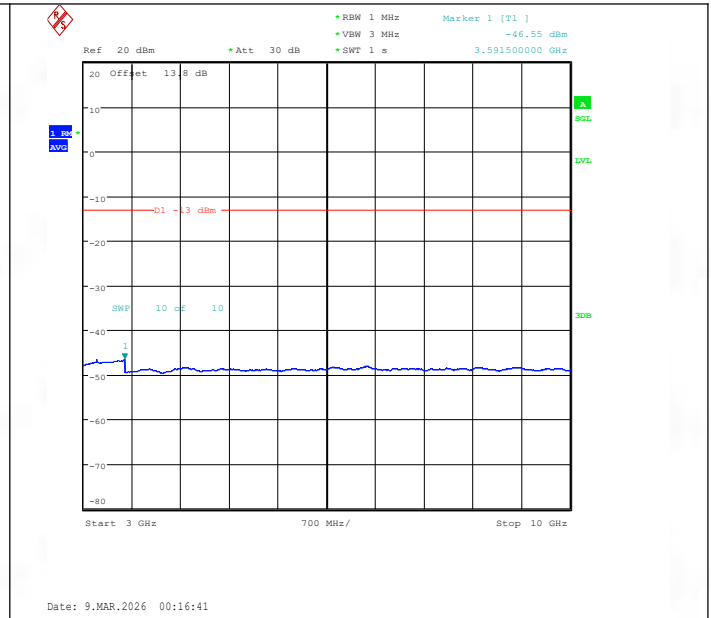
Band26(824-849)-10MHz-16QAM-26915-1RB#0-3000~10000-PASS
