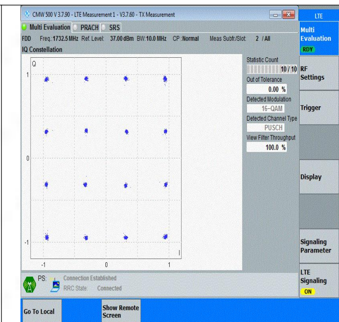
Band4-10MHz-16QAM-20175-50RB#0-PASS
