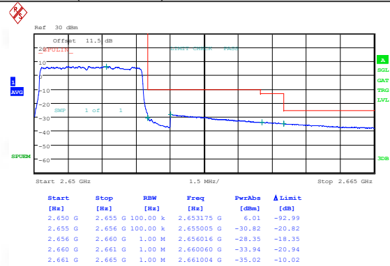
Band41(2535-2655)-5MHz-16QAM-41215-1RB#0-PASS
