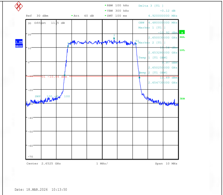
Band41(2535-2655)-5MHz-16QAM-41215-25RB#0-PASS
