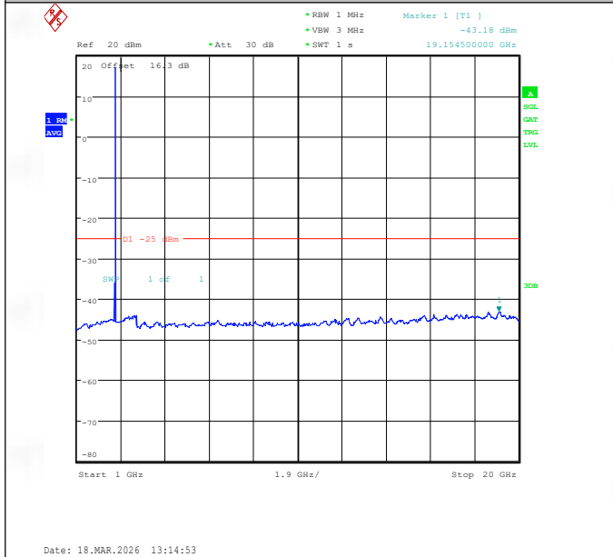
Band41(2535-2655)-10MHz-16QAM-41190-1RB#49-1000~20000-PASS
