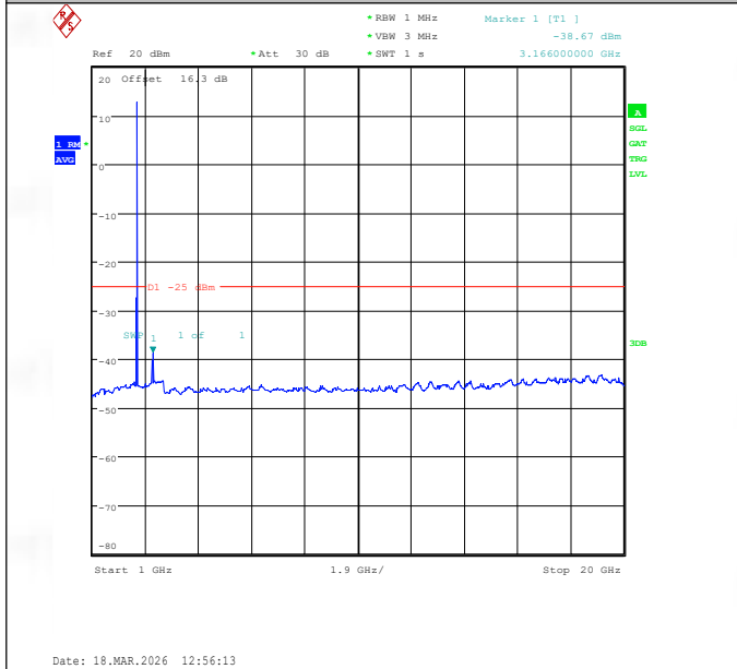
Band41(2535-2655)-10MHz-QPSK-40590-1RB#49-1000~20000-PASS
