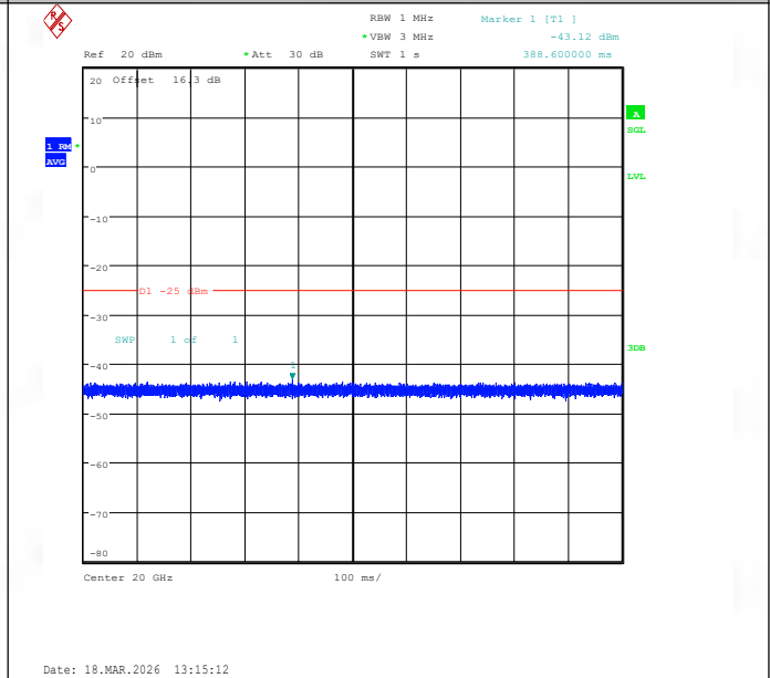
Band41(2535-2655)-10MHz-16QAM-41190-1RB#49-20000~27000-PASS
