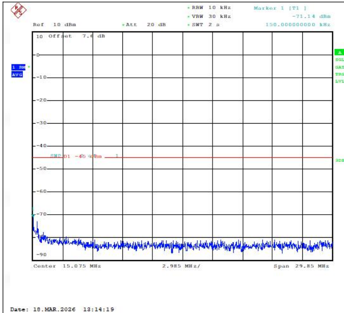
Band41(2535-2655)-10MHz-16QAM-41190-1RB#49-0.15~30-PASS
