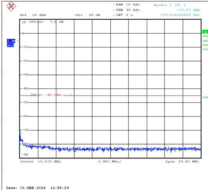
Band41(2535-2655)-10MHz-QPSK-40590-1RB#49-0.15~30-PASS
