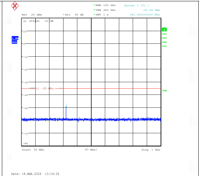
Band41(2535-2655)-10MHz-16QAM-41190-1RB#49-30~1000-PASS
