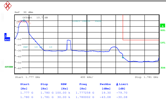
Band66-3MHz-QPSK-132657-1RB#14-PASS
