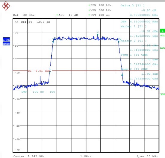
Band66-5MHz-QPSK-131997-25RB#0-PASS
