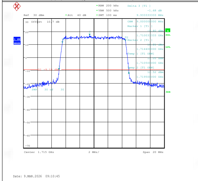
Band66-10MHz-QPSK-132022-50RB#0-PASS
