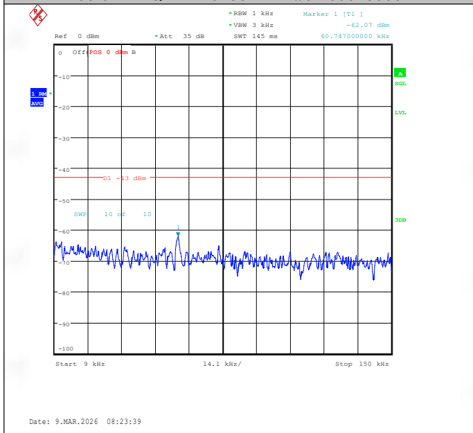
Band66-3MHz-16QAM-131987-1RB#0-0.009~0.15-PASS
