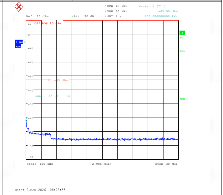
Band66-3MHz-16QAM-131987-1RB#0-0.15~30-PASS
