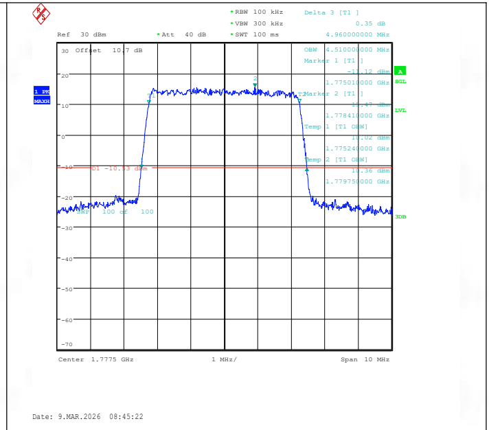
Band66-5MHz-16QAM-132647-25RB#0-PASS
