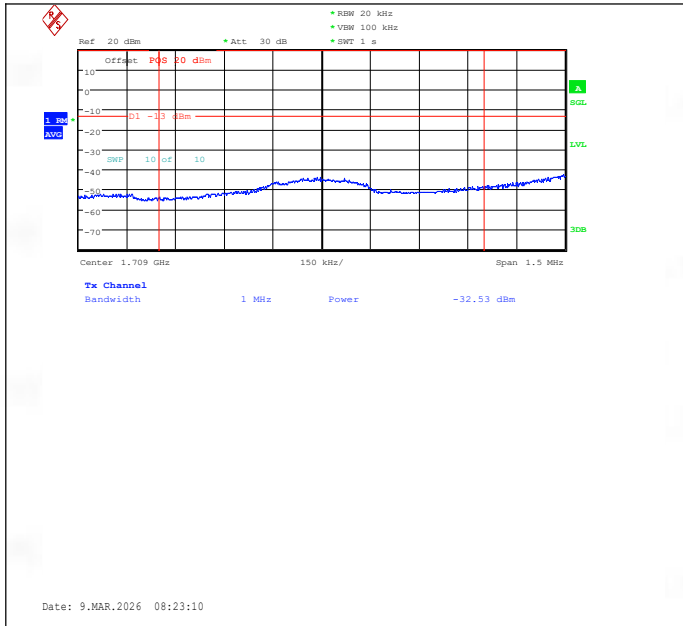
Band66-3MHz-QPSK-131987-1RB#0-1000~3000-PASS
