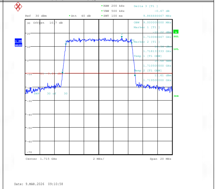
Band66-10MHz-16QAM-132022-50RB#0-PASS
