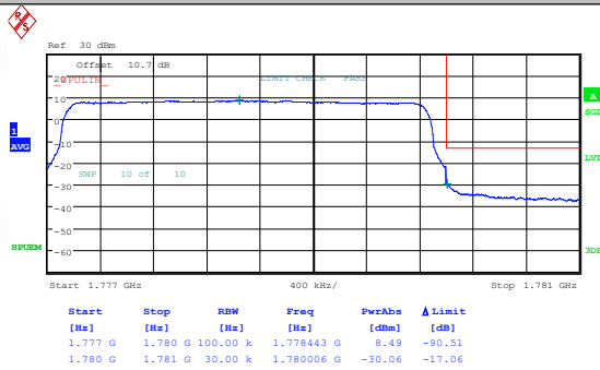
Band66-3MHz-QPSK-132657-1RB#0-PASS
