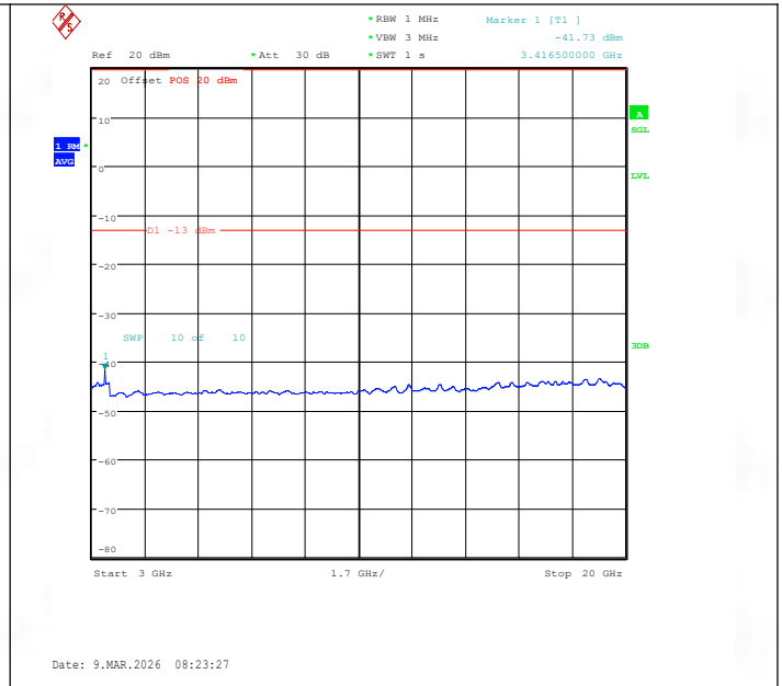
Band66-3MHz-QPSK-131987-1RB#0-3000~20000-PASS
