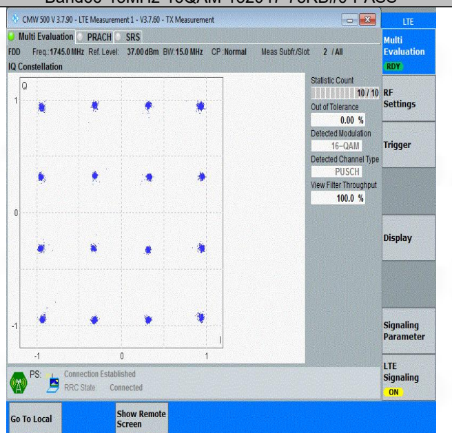
Band66-15MHz-16QAM-132322-75RB#0-PASS
