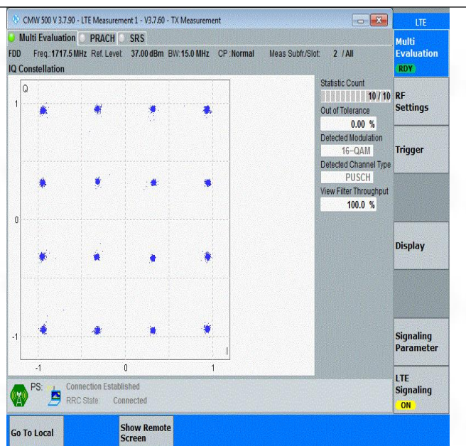
Band66-15MHz-16QAM-132047-75RB#0-PASS
