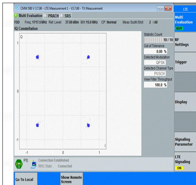
Band66-15MHz-QPSK-132047-75RB#0-PASS
