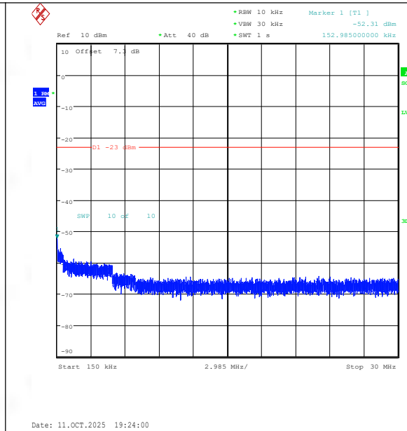
EGPRS850-190-8-0.15~30MHz-PASS
