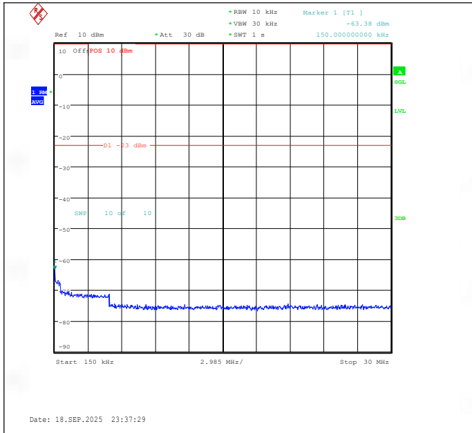
Band19-10MHz-16QAM-24100-50RB#0-0.15~30-PASS
