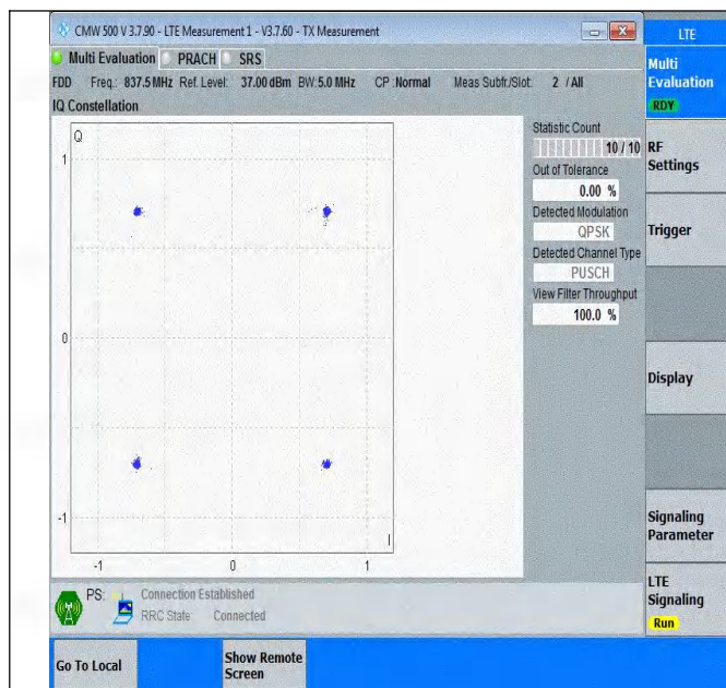
Band19-5MHz-QPSK-24075-25RB#0-PASS
