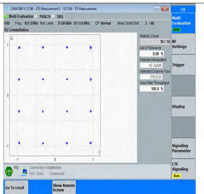
Band19-5MHz-16QAM-24075-25RB#0-PASS
