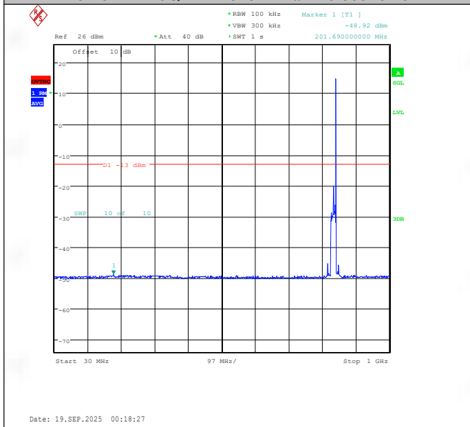
Band19-15MHz-16QAM-24075-1RB#74-30~1000-PASS
