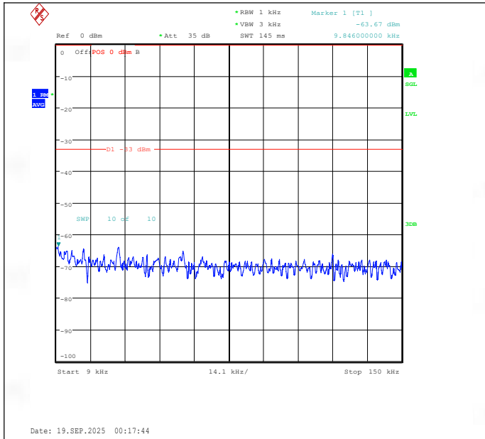
Band19-15MHz-16QAM-24075-1RB#74-0.009~0.15-PASS
