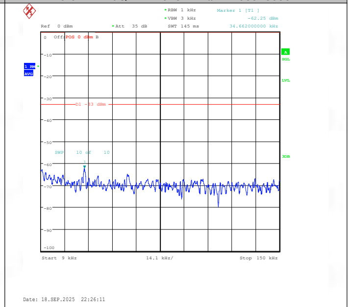
Band19-5MHz-16QAM-24075-25RB#0-0.009~0.15-PASS
