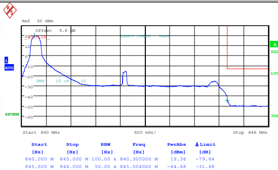
Band19-5MHz-16QAM-24025-1RB#24-PASS
