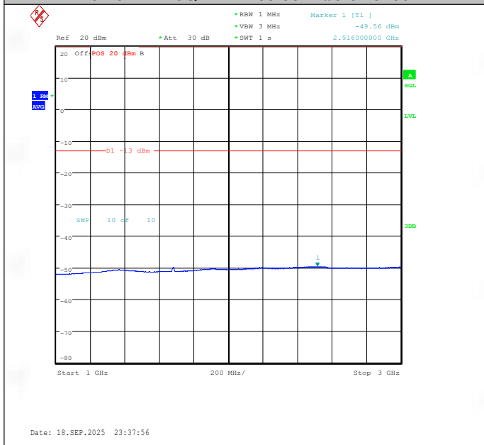
Band19-10MHz-16QAM-24100-50RB#0-1000~3000-PASS
