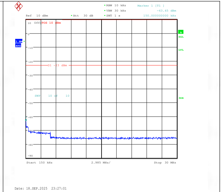
Band19-10MHz-16QAM-24075-1RB#49-0.15~30-PASS
