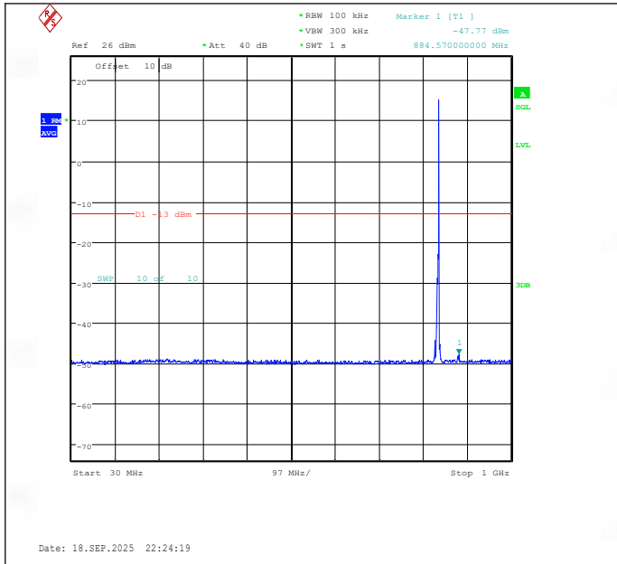
Band19-5MHz-16QAM-24075-1RB#24-30~1000-PASS
