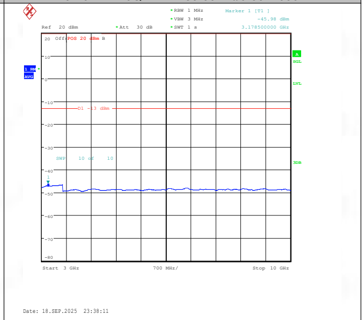
Band19-10MHz-16QAM-24100-50RB#0-3000~10000-PASS
