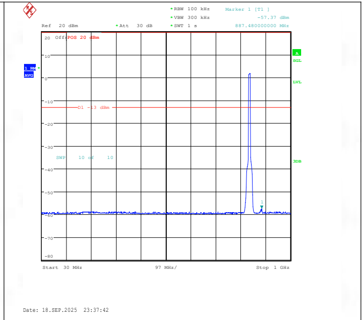
Band19-10MHz-16QAM-24100-50RB#0-30~1000-PASS
