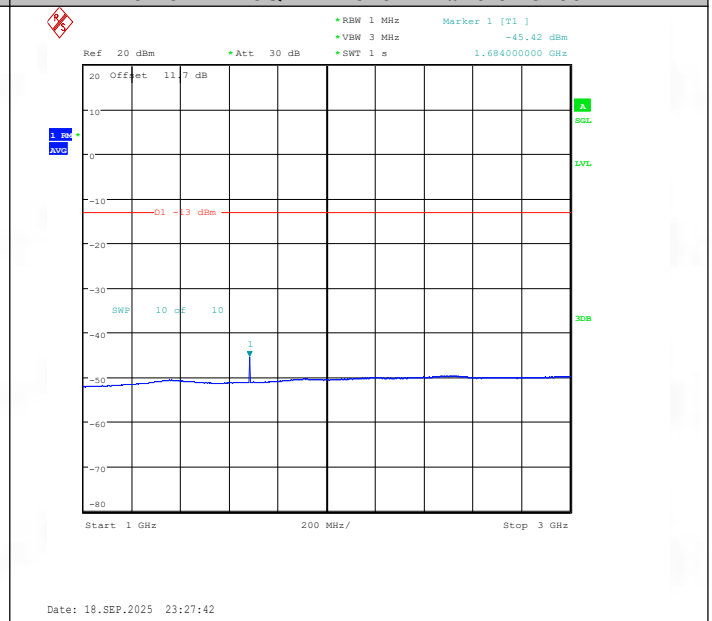
Band19-10MHz-16QAM-24075-1RB#49-1000~3000-PASS
