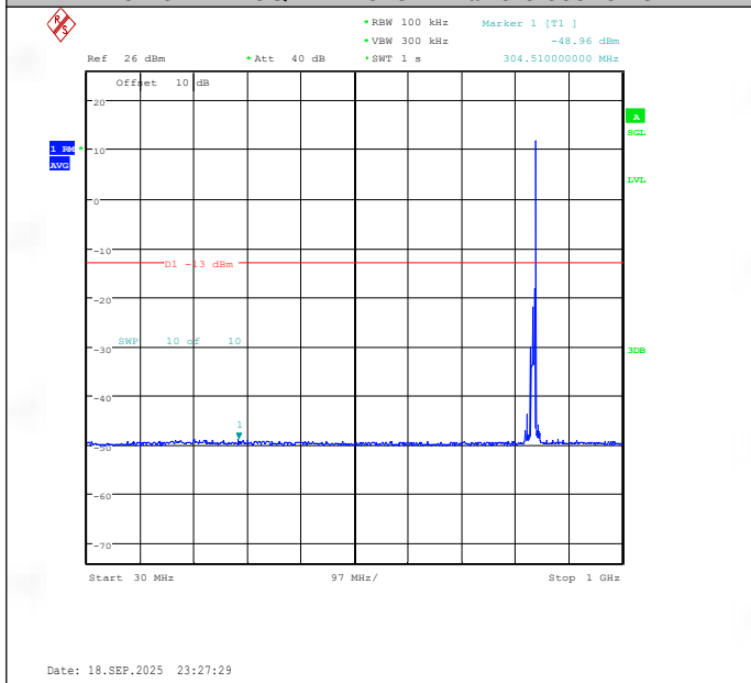
Band19-10MHz-16QAM-24075-1RB#49-30~1000-PASS
