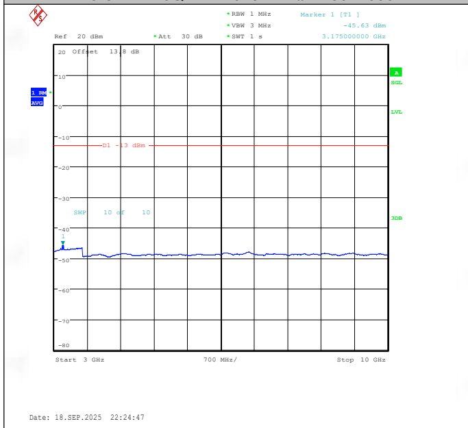
Band19-5MHz-16QAM-24075-1RB#24-3000~10000-PASS
