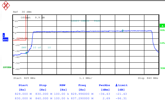
Band19-10MHz-QPSK-24050-1RB#0-PASS
