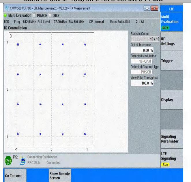
Band19-5MHz-16QAM-24125-25RB#0-PASS
