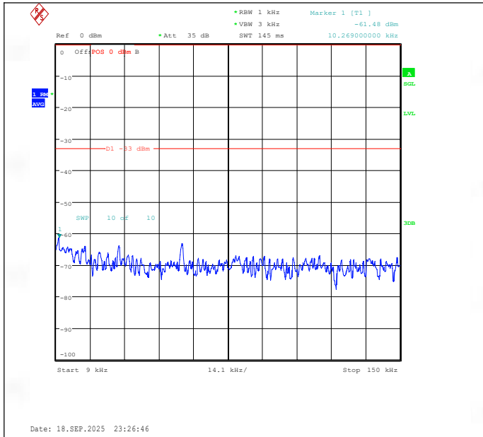
Band19-10MHz-16QAM-24075-1RB#49-0.009~0.15-PASS
