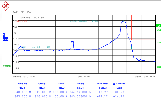
Band19-5MHz-QPSK-24125-25RB#0-PASS
