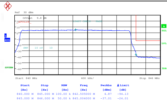
Band19-5MHz-16QAM-24125-1RB#0-PASS
