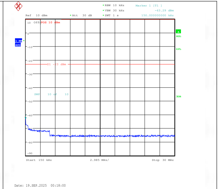
Band19-15MHz-16QAM-24075-1RB#74-0.15~30-PASS
