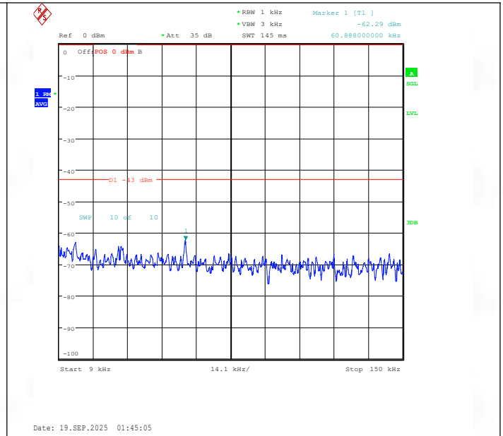
Band25-15MHz-16QAM-26365-1RB#0-0.009~0.15-PASS
