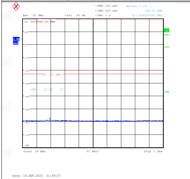
Band25-15MHz-QPSK-26365-75RB#0-30~1000-PASS
