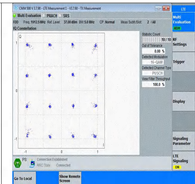
Band25-5MHz-16QAM-26665-25RB#0-PASS
