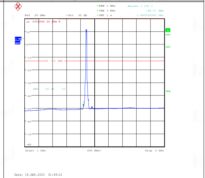
Band25-15MHz-QPSK-26365-75RB#0-1000~3000-PASS
