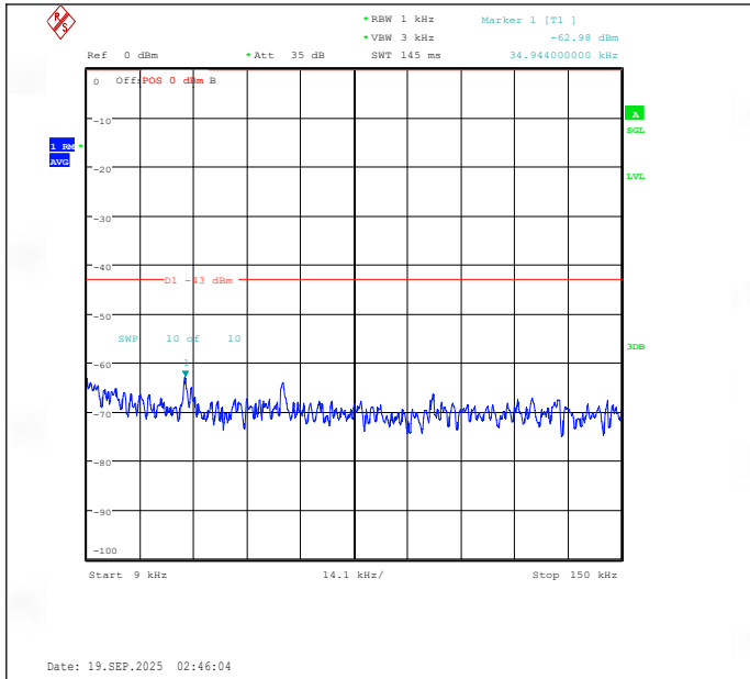
Band25-20MHz-16QAM-26365-1RB#99-0.009~0.15-PASS
