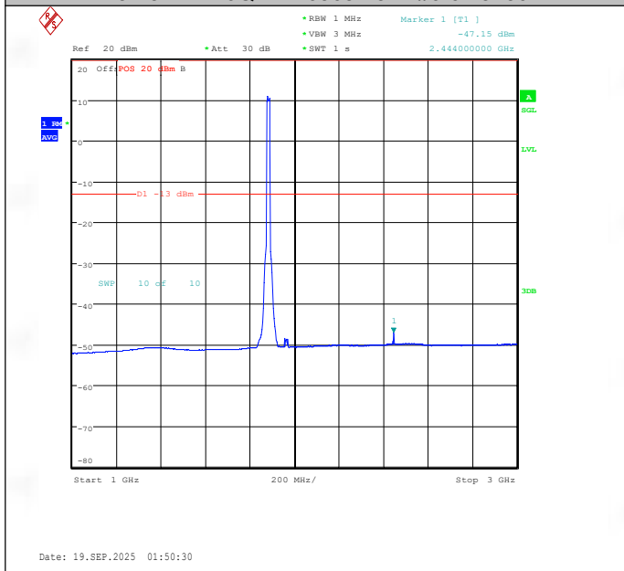
Band25-15MHz-16QAM-26365-75RB#0-1000~3000-PASS
