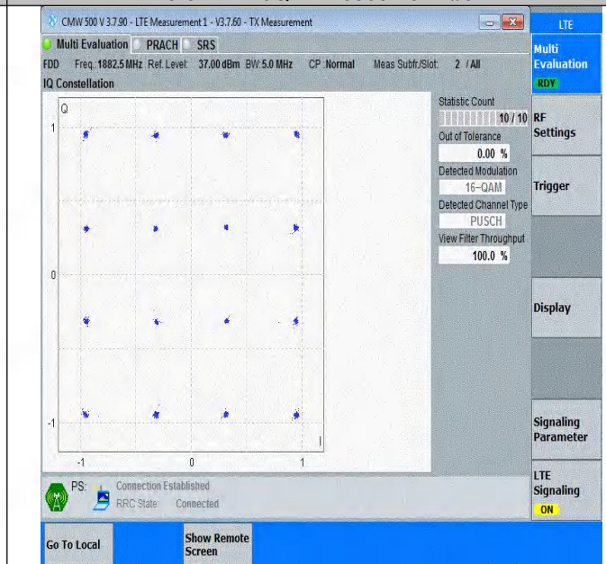
Band25-5MHz-16QAM-26365-25RB#0-PASS
