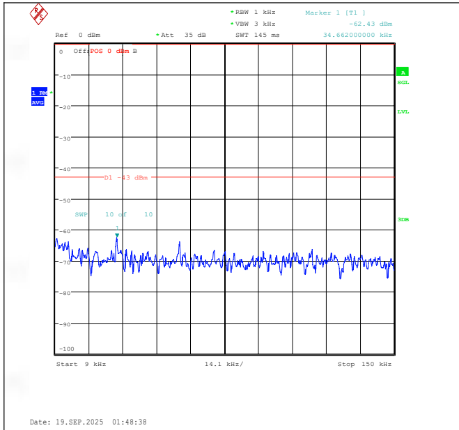
Band25-15MHz-QPSK-26365-75RB#0-0.009~0.15-PASS
