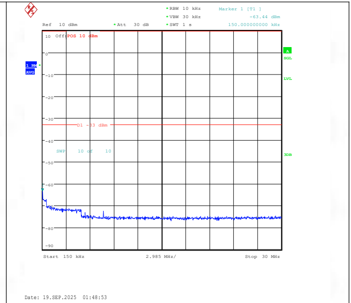
Band25-15MHz-QPSK-26365-75RB#0-0.15~30-PASS
