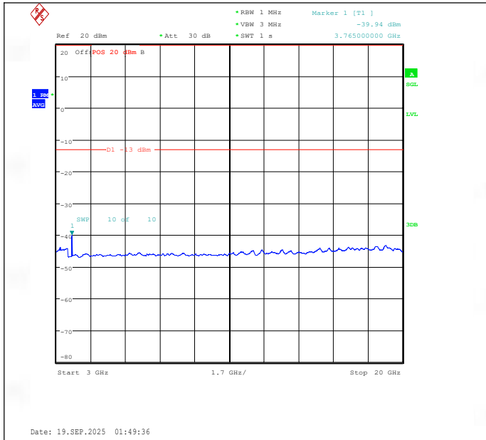
Band25-15MHz-QPSK-26365-75RB#0-3000~20000-PASS
