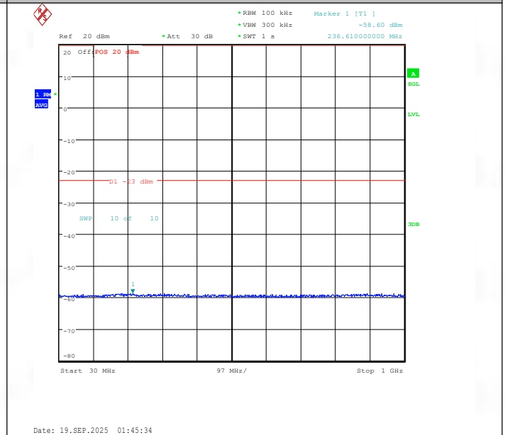
Band25-15MHz-16QAM-26365-1RB#0-30~1000-PASS
