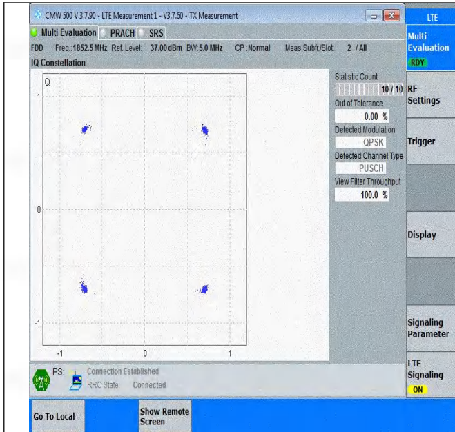
Band25-5MHz-QPSK-26065-25RB#0-PASS
