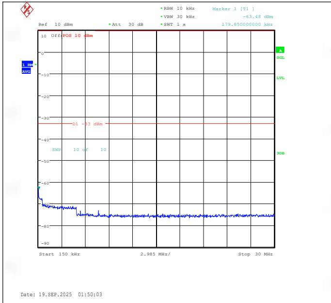
Band25-15MHz-16QAM-26365-75RB#0-0.15~30-PASS
