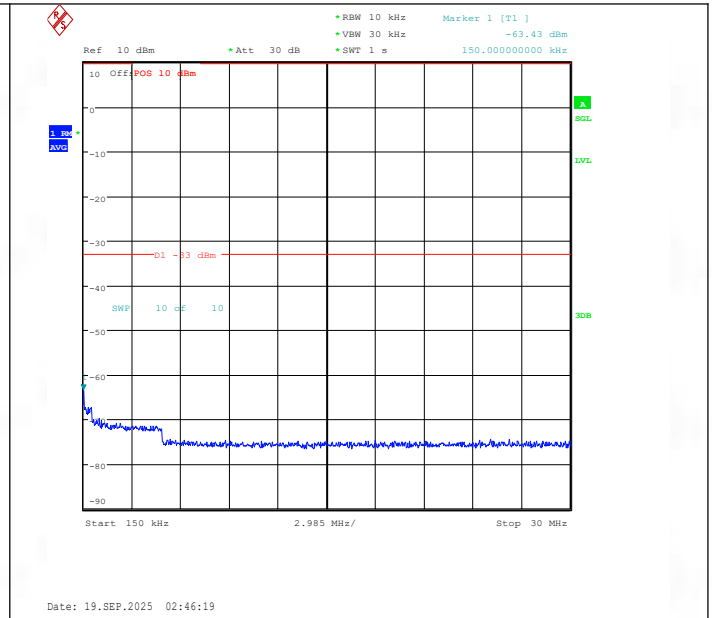
Band25-20MHz-16QAM-26365-1RB#99-0.15~30-PASS
