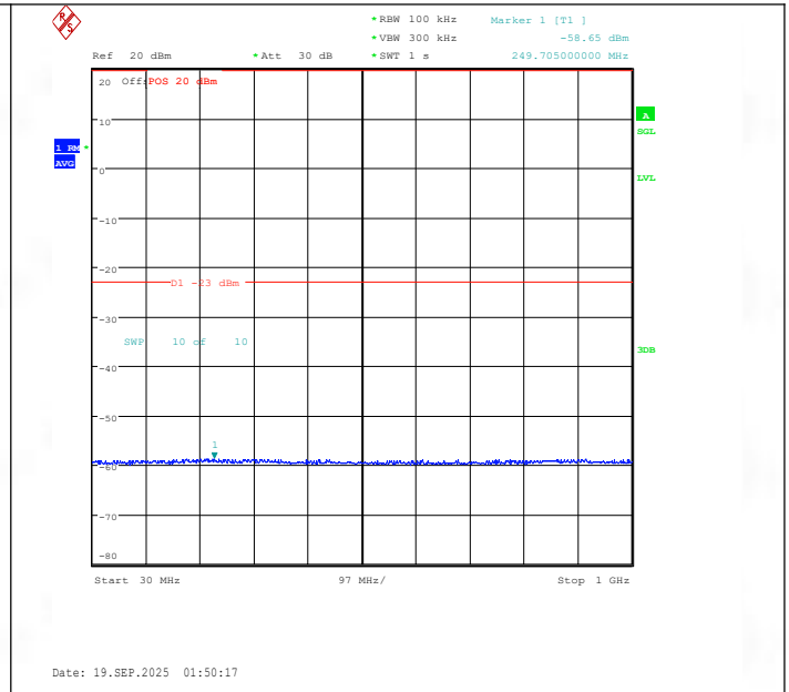
Band25-15MHz-16QAM-26365-75RB#0-30~1000-PASS
