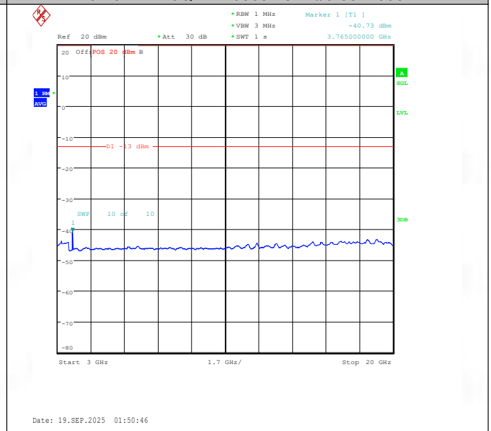
Band25-15MHz-16QAM-26365-75RB#0-3000~20000-PASS
