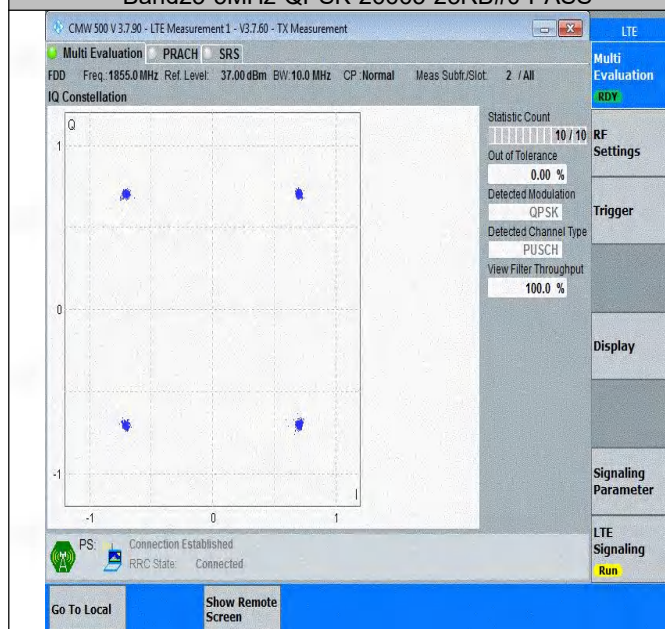
Band25-10MHz-QPSK-26090-50RB#0-PASS
