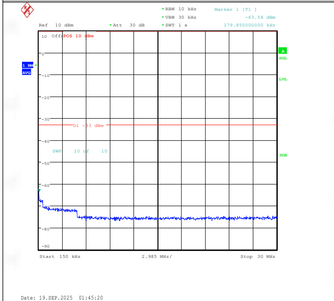
Band25-15MHz-16QAM-26365-1RB#0-0.15~30-PASS
