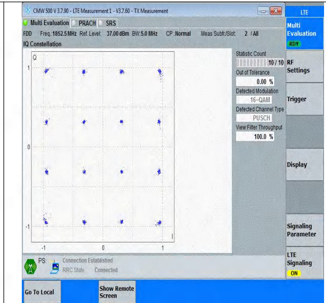
Band25-5MHz-16QAM-26065-25RB#0-PASS
