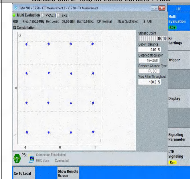
Band25-10MHz-16QAM-26090-50RB#0-PASS
