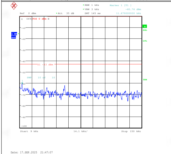
Band25-3MHz-QPSK-26055-1RB#0-0.009~0.15-PASS
