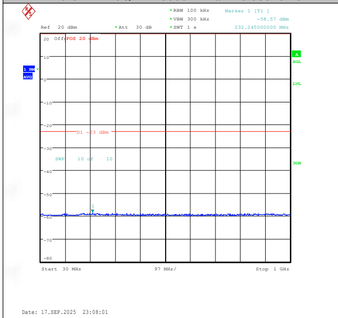
Band25-5MHz-16QAM-26665-1RB#24-30~1000-PASS
