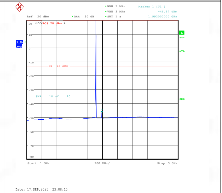
Band25-5MHz-16QAM-26665-1RB#24-1000~3000-PASS
