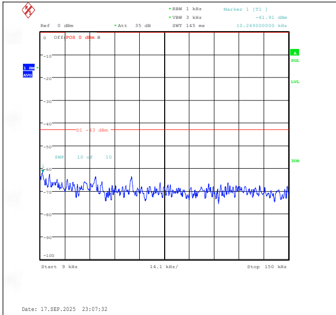
Band25-5MHz-16QAM-26665-1RB#24-0.009~0.15-PASS
