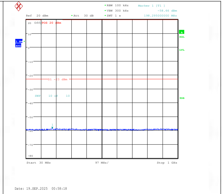
Band25-10MHz-16QAM-26640-50RB#0-30~1000-PASS
