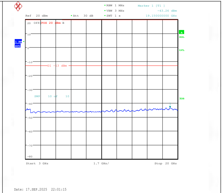
Band25-3MHz-16QAM-26365-15RB#0-3000~20000-PASS
