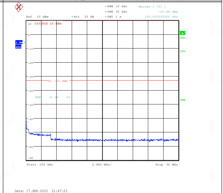
Band25-3MHz-QPSK-26055-1RB#0-0.15~30-PASS
