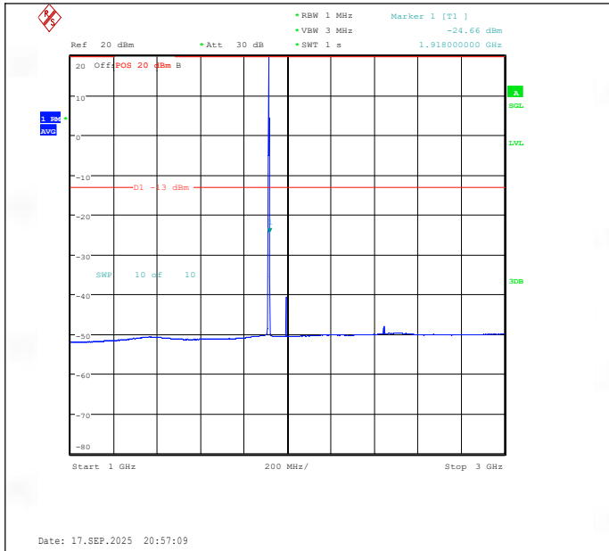
Band25-1.4MHz-16QAM-26683-6RB#0-1000~3000-PASS
