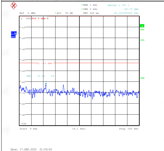
Band25-3MHz-QPSK-26365-15RB#0-0.009~0.15-PASS
