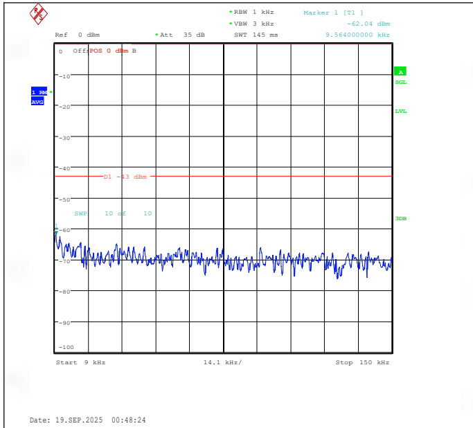
Band25-10MHz-16QAM-26365-1RB#49-0.009~0.15-PASS
