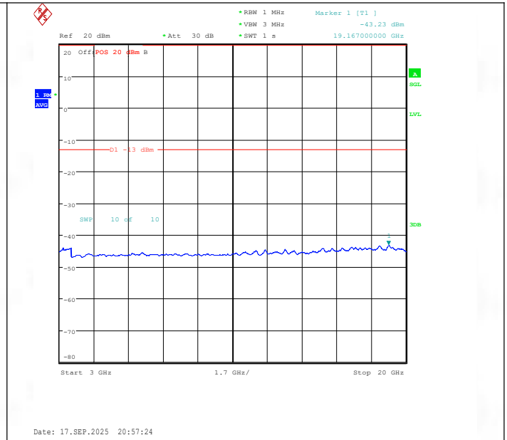
Band25-1.4MHz-16QAM-26683-6RB#0-3000~20000-PASS
