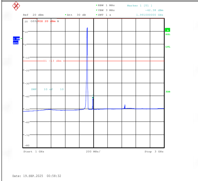
Band25-10MHz-16QAM-26640-50RB#0-1000~3000-PASS
