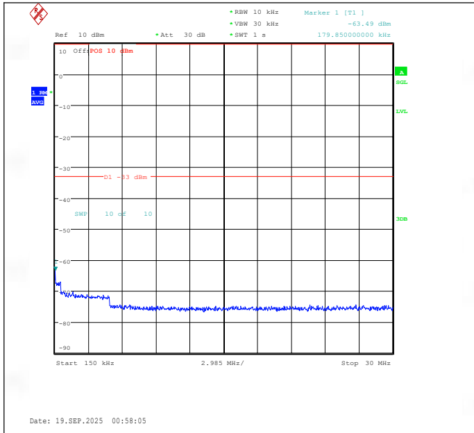
Band25-10MHz-16QAM-26640-50RB#0-0.15~30-PASS
