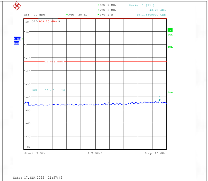
Band25-3MHz-QPSK-26365-1RB#14-3000~20000-PASS
