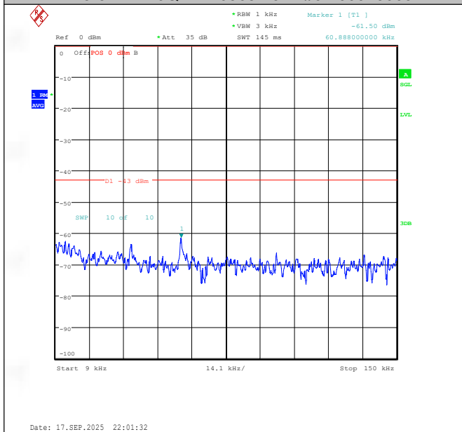
Band25-3MHz-QPSK-26675-1RB#0-0.009~0.15-PASS
