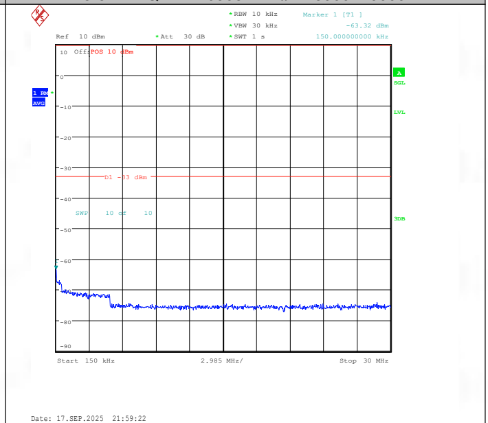
Band25-3MHz-QPSK-26365-15RB#0-0.15~30-PASS
