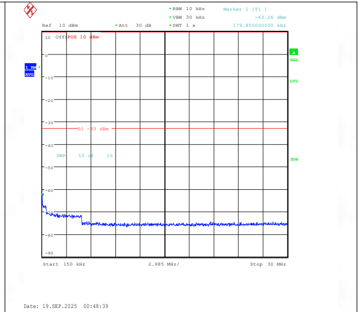
Band25-10MHz-16QAM-26365-1RB#49-0.15~30-PASS
