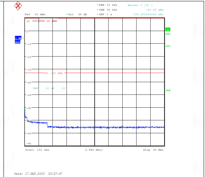
Band25-5MHz-16QAM-26665-1RB#24-0.15~30-PASS
