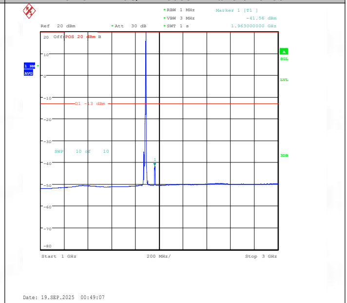
Band25-10MHz-16QAM-26365-1RB#49-1000~3000-PASS
