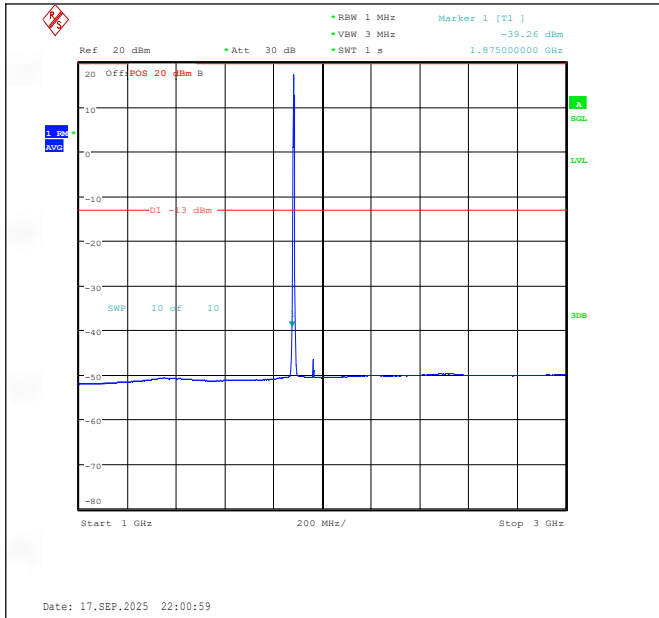
Band25-3MHz-16QAM-26365-15RB#0-1000~3000-PASS
