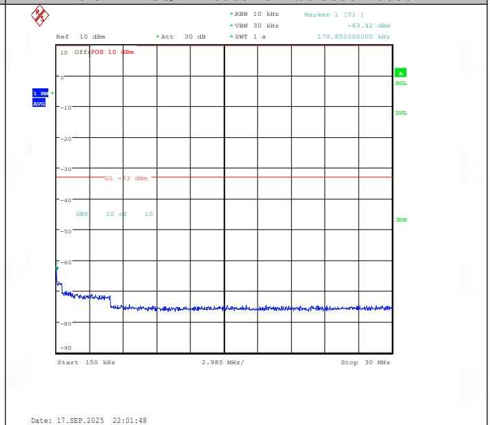
Band25-3MHz-QPSK-26675-1RB#0-0.15~30-PASS
