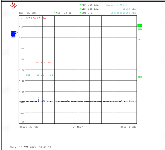
Band25-10MHz-16QAM-26365-1RB#49-30~1000-PASS
