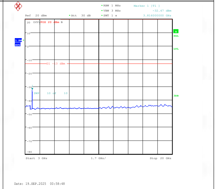
Band25-10MHz-16QAM-26640-50RB#0-3000~20000-PASS
