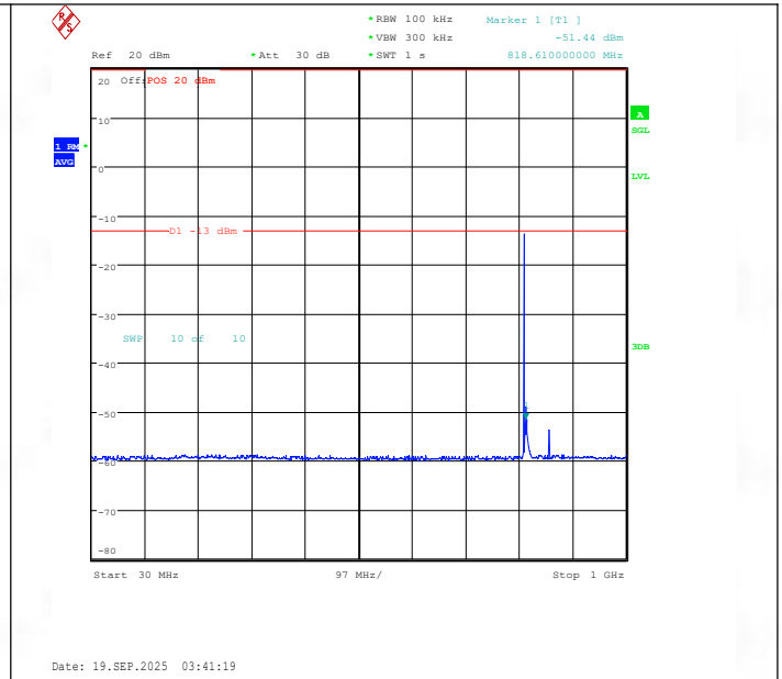
Band26(814-824)-1.4MHz-16QAM-26697-1RB#0-30~1000-PASS
