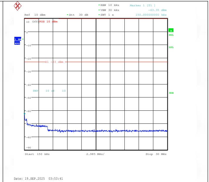
Band26(814-824)-1.4MHz-QPSK-26740-6RB#0-0.15~30-PASS
