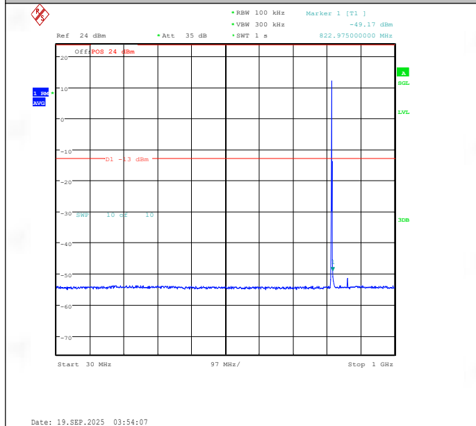
Band26(814-824)-1.4MHz-QPSK-26740-6RB#0-30~1000-PASS
