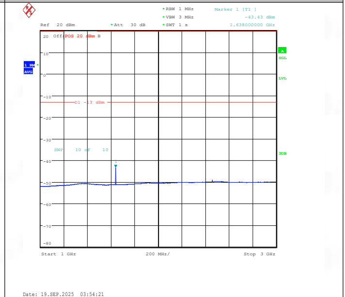
Band26(814-824)-1.4MHz-QPSK-26740-6RB#0-1000~3000-PASS
