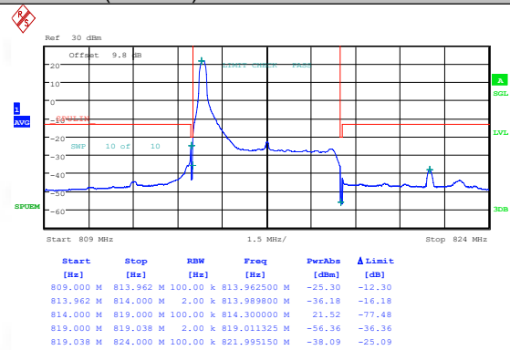
Band26(814-824)-3MHz-16QAM-26775-1RB#14-PASS
