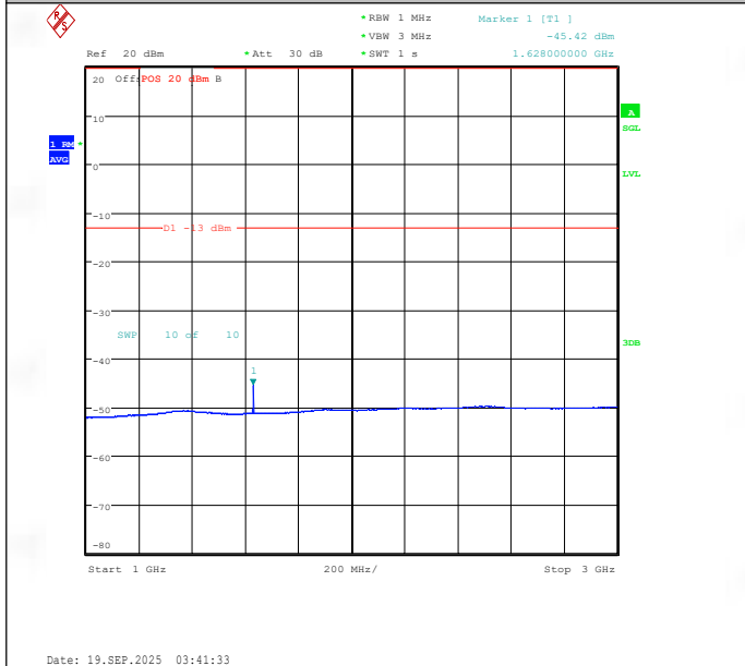
Band26(814-824)-1.4MHz-16QAM-26697-1RB#0-1000~3000-PASS
