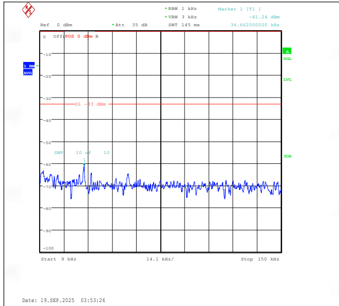
Band26(814-824)-1.4MHz-QPSK-26740-6RB#0-0.009~0.15-PASS
