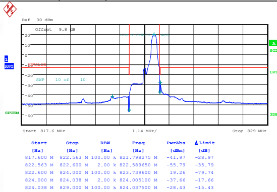
Band26(814-824)-1.4MHz-QPSK-26783-6RB#0-PASS
