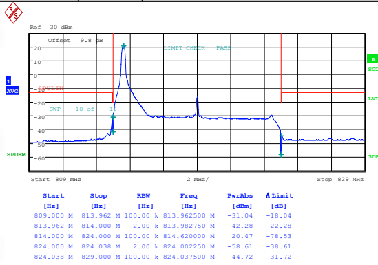
Band26(814-824)-10MHz-QPSK-26740-1RB#49-PASS
