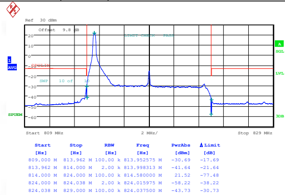
Band26(814-824)-5MHz-16QAM-26765-1RB#24-PASS
