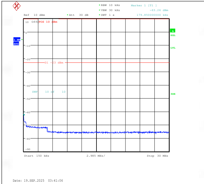
Band26(814-824)-1.4MHz-16QAM-26697-1RB#0-0.15~30-PASS
