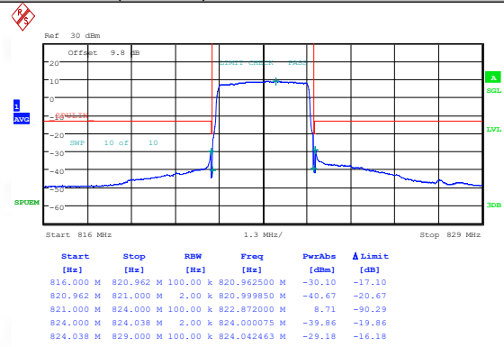
Band26(814-824)-3MHz-QPSK-26775-1RB#0-PASS
