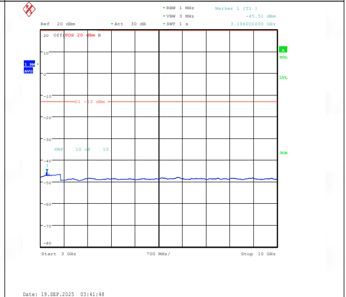
Band26(814-824)-1.4MHz-16QAM-26697-1RB#0-3000~10000-PASS
