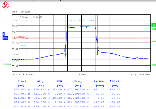
Band26(814-824)-3MHz-16QAM-26775-1RB#0-PASS
