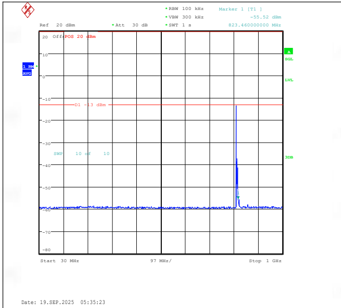
Band26(814-824)-3MHz-QPSK-26705-1RB#0-30~1000-PASS
