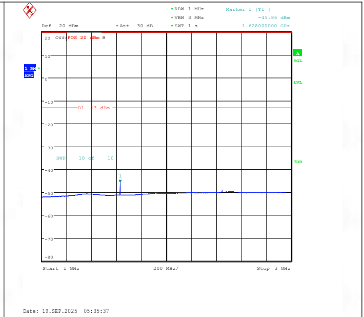
Band26(814-824)-3MHz-QPSK-26705-1RB#0-1000~3000-PASS
