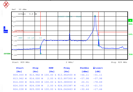
Band26(814-824)-10MHz-QPSK-26740-50RB#0-PASS
