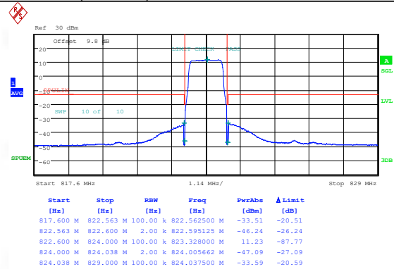
Band26(814-824)-1.4MHz-16QAM-26783-1RB#0-PASS
