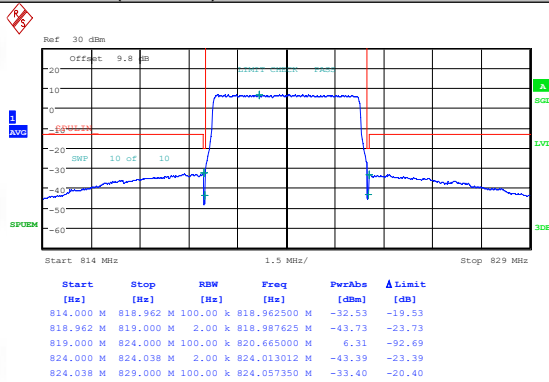
Band26(814-824)-5MHz-16QAM-26765-1RB#0-PASS
