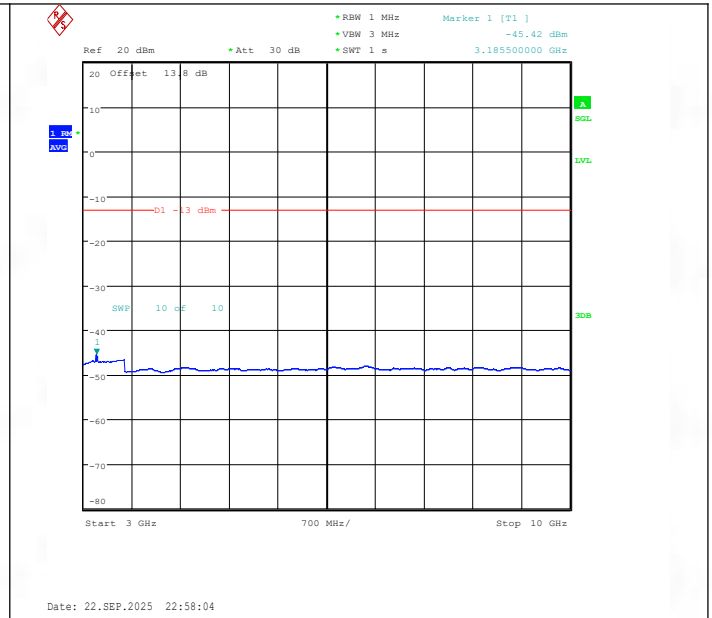
Band26(824-849)-1.4MHz-QPSK-26797-1RB#5-3000~10000-PASS
