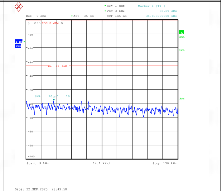
Band26(824-849)-3MHz-QPSK-26805-1RB#14-0.009~0.15-PASS
