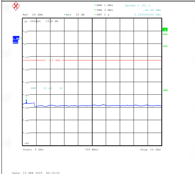
Band26(824-849)-3MHz-16QAM-27025-1RB#14-3000~10000-PASS
