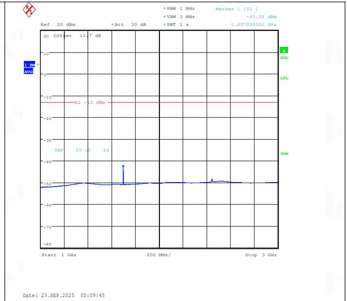
Band26(824-849)-3MHz-16QAM-27025-1RB#14-1000~3000-PASS
