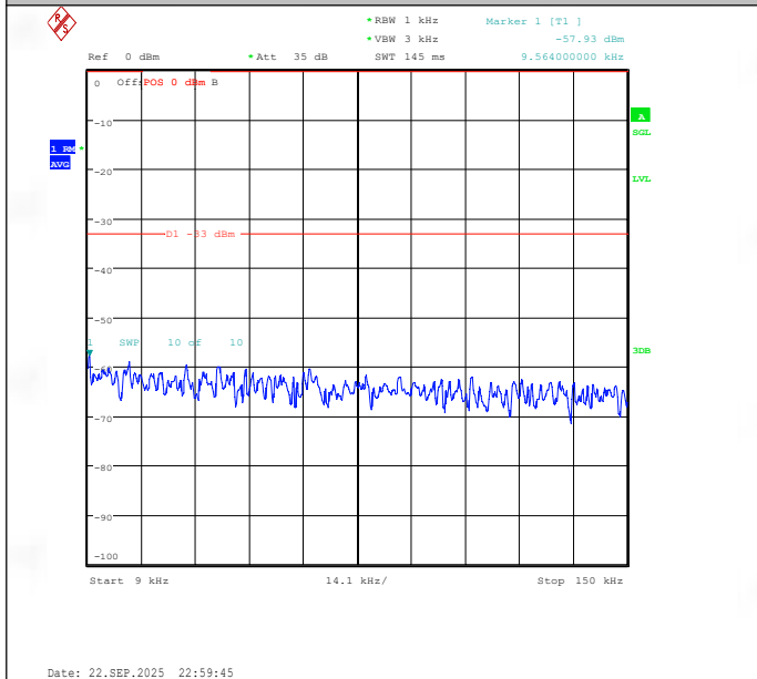
Band26(824-849)-1.4MHz-QPSK-26797-6RB#0-0.009~0.15-PASS
