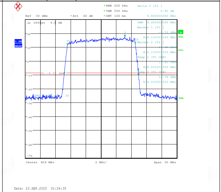
Band26(824-849)-10MHz-16QAM-26840-50RB#0-PASS
