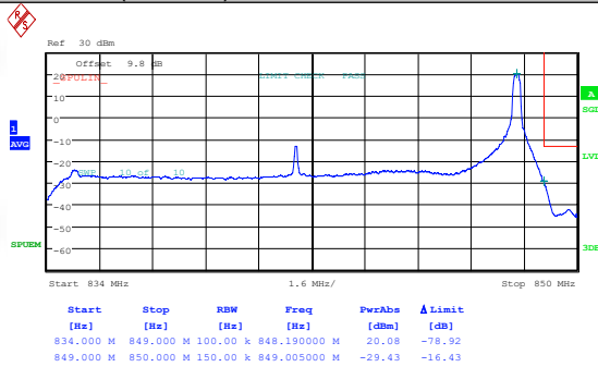
Band26(824-849)-15MHz-QPSK-26965-75RB#0-PASS
