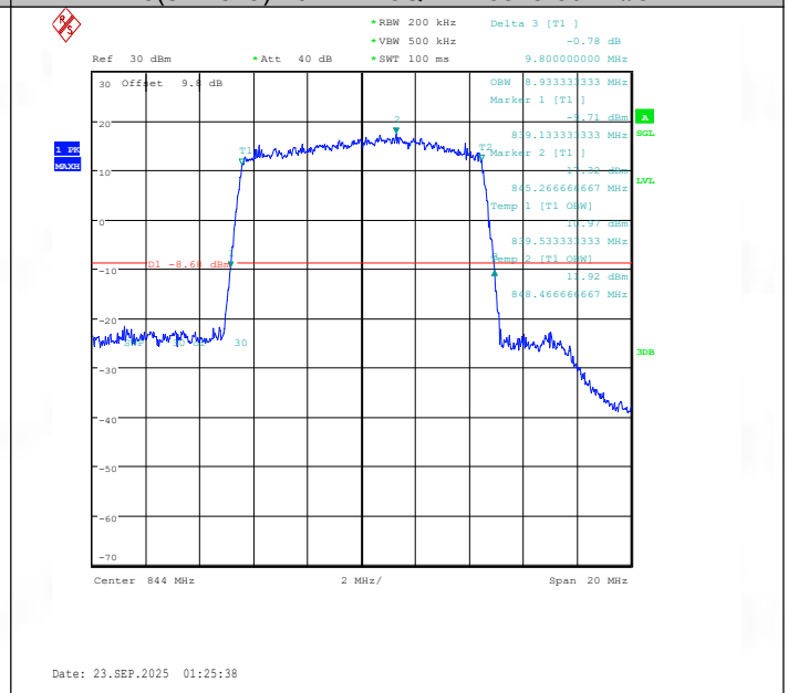
Band26(824-849)-10MHz-16QAM-26990-50RB#0-PASS
