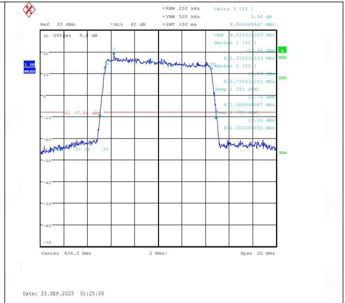
Band26(824-849)-10MHz-16QAM-26915-50RB#0-PASS
