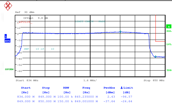
Band26(824-849)-15MHz-16QAM-26965-1RB#0-PASS
