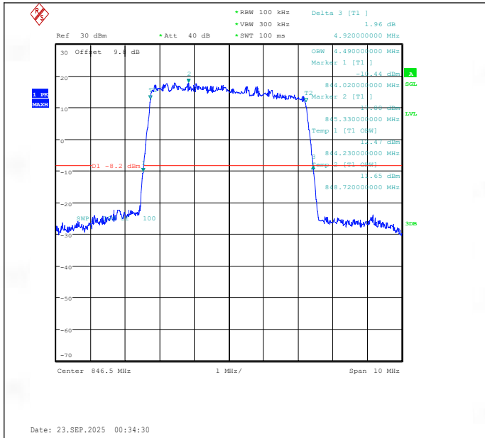
Band26(824-849)-5MHz-QPSK-27015-25RB#0-PASS
