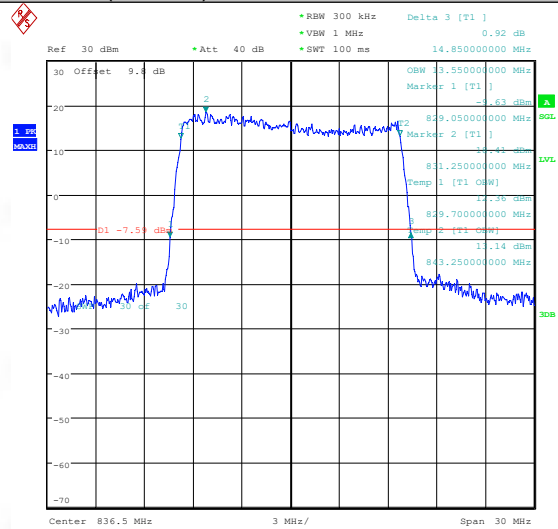
Band26(824-849)-15MHz-16QAM-26865-75RB#0-PASS
