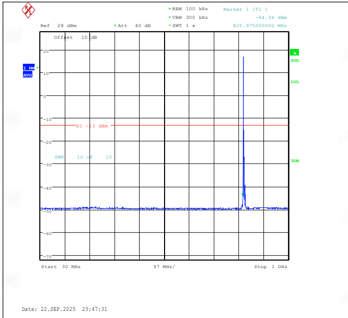
Band26(824-849)-3MHz-QPSK-26805-1RB#0-30~1000-PASS
