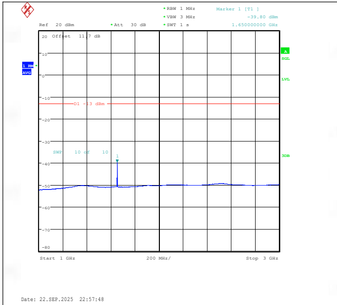
Band26(824-849)-1.4MHz-QPSK-26797-1RB#5-1000~3000-PASS
