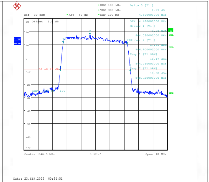
Band26(824-849)-5MHz-16QAM-27015-25RB#0-PASS
