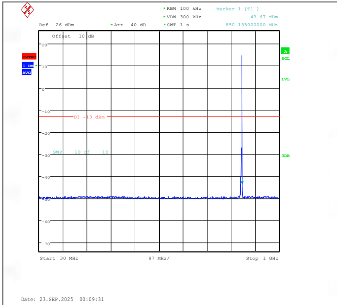
Band26(824-849)-3MHz-16QAM-27025-1RB#14-30~1000-PASS
