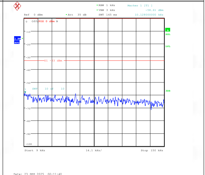
Band26(824-849)-3MHz-16QAM-27025-15RB#0-0.009~0.15-PASS
