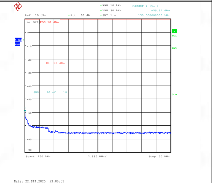
Band26(824-849)-1.4MHz-QPSK-26797-6RB#0-0.15~30-PASS
