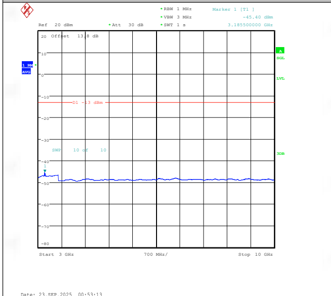
Band26(824-849)-5MHz-16QAM-26915-1RB#24-3000~10000-PASS
