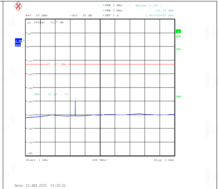
Band26(824-849)-10MHz-16QAM-26840-1RB#49-1000~3000-PASS
