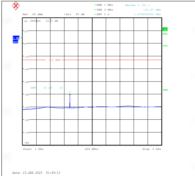
Band26(824-849)-10MHz-16QAM-26990-1RB#0-1000~3000-PASS
