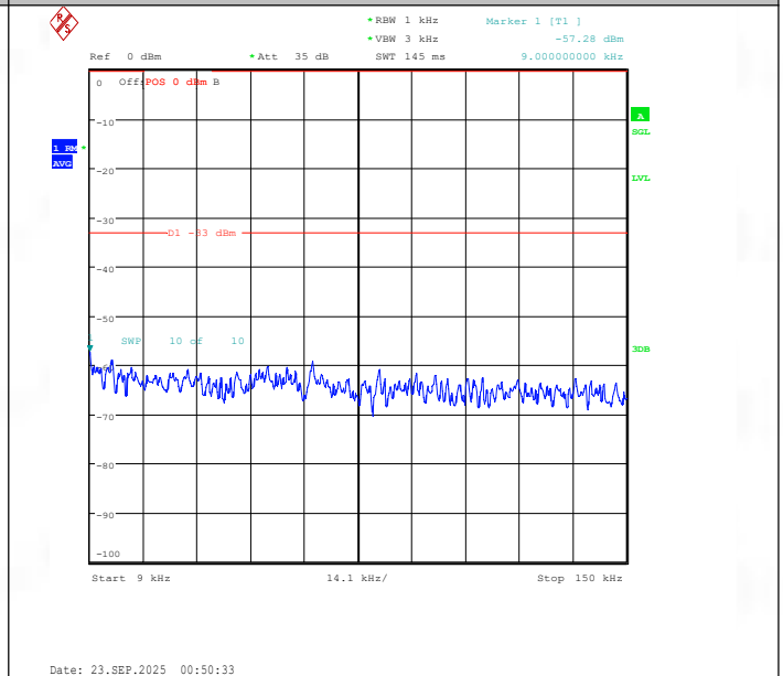
Band26(824-849)-5MHz-QPSK-26915-1RB#24-0.009~0.15-PASS
