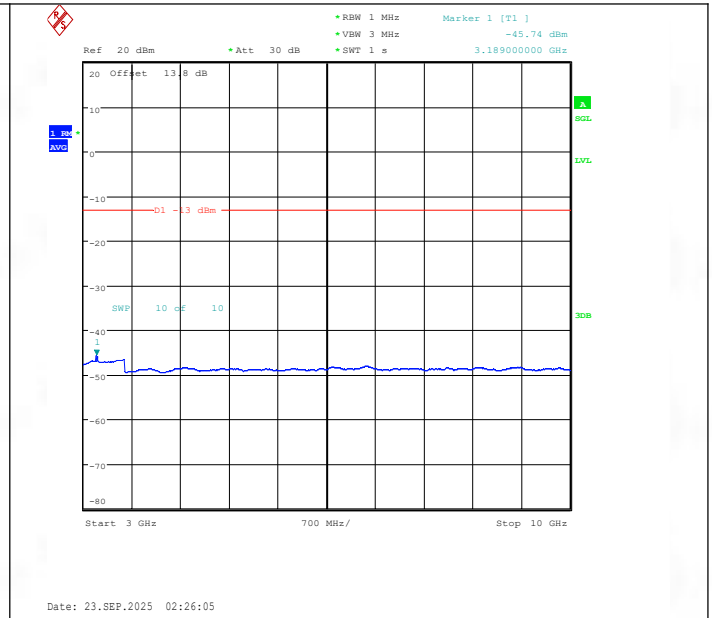
Band26(824-849)-15MHz-QPSK-26865-1RB#74-3000~10000-PASS
