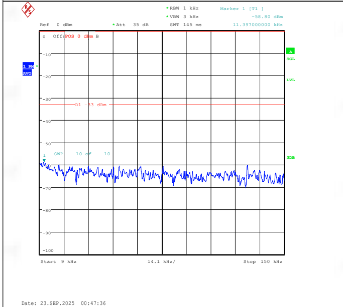
Band26(824-849)-5MHz-QPSK-26915-1RB#0-0.009~0.15-PASS
