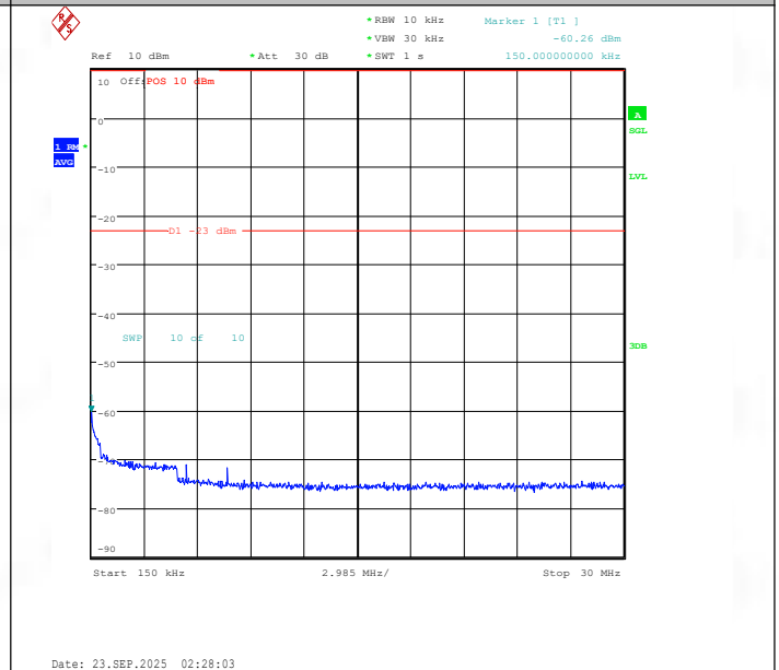
Band26(824-849)-15MHz-QPSK-26865-75RB#0-0.15~30-PASS
