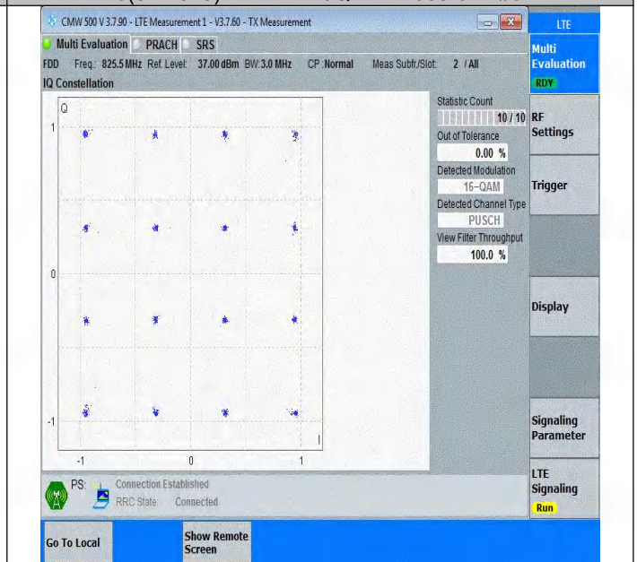
Band26(824-849)-3MHz-16QAM-26805-15RB#0-PASS
