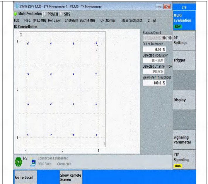
Band26(824-849)-1.4MHz-16QAM-27033-6RB#0-PASS
