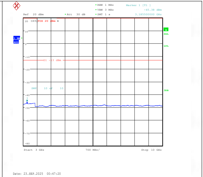
Band26(824-849)-5MHz-16QAM-26815-25RB#0-3000~10000-PASS
