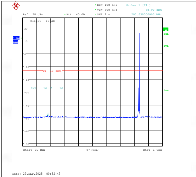
Band26(824-849)-5MHz-16QAM-26915-1RB#24-30~1000-PASS
