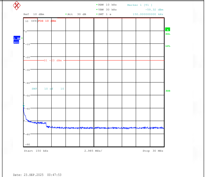
Band26(824-849)-5MHz-QPSK-26915-1RB#0-0.15~30-PASS
