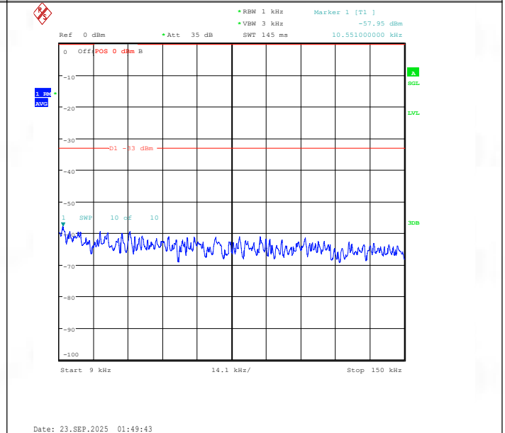
Band26(824-849)-10MHz-QPSK-26990-1RB#49-0.009~0.15-PASS
