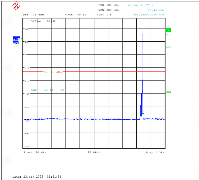
Band26(824-849)-10MHz-16QAM-26990-1RB#49-30~1000-PASS
