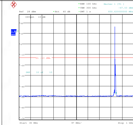
Band26(824-849)-10MHz-16QAM-26990-1RB#0-0.009~0.15-PASS
