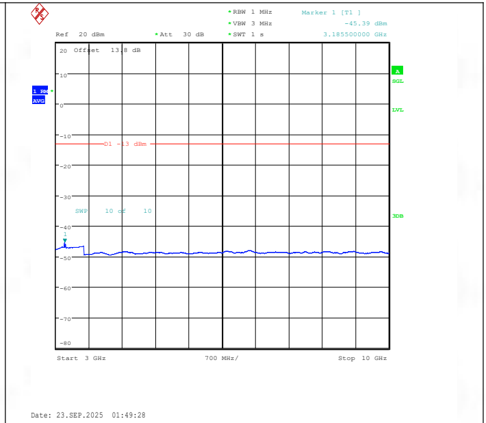
Band26(824-849)-10MHz-16QAM-26990-1RB#0-3000~10000-PASS
