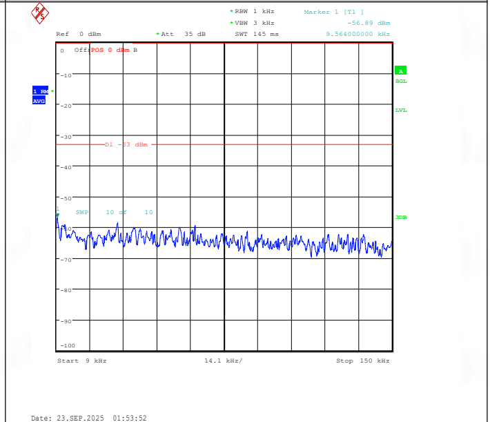
Band26(824-849)-10MHz-16QAM-26990-50RB#0-0.009~0.15-PASS
