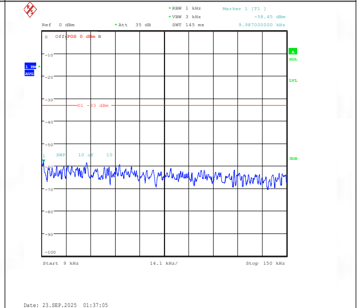
Band26(824-849)-10MHz-16QAM-26840-50RB#0-0.009~0.15-PASS
