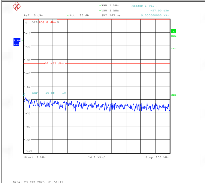
Band26(824-849)-10MHz-16QAM-26990-1RB#49-0.009~0.15-PASS
