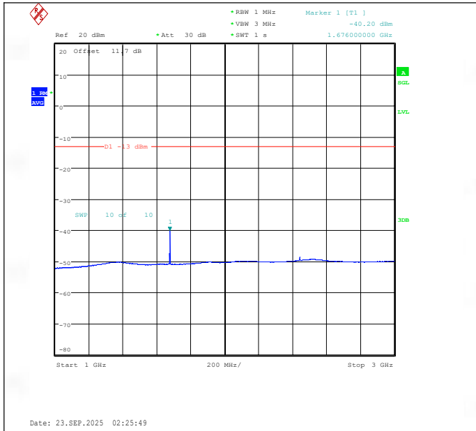
Band26(824-849)-15MHz-QPSK-26865-1RB#74-1000~3000-PASS
