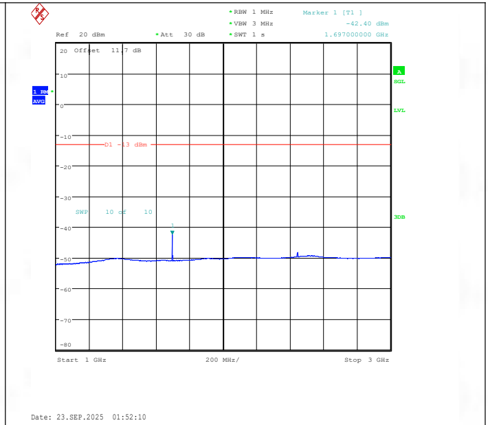
Band26(824-849)-10MHz-16QAM-26990-1RB#49-1000~3000-PASS
