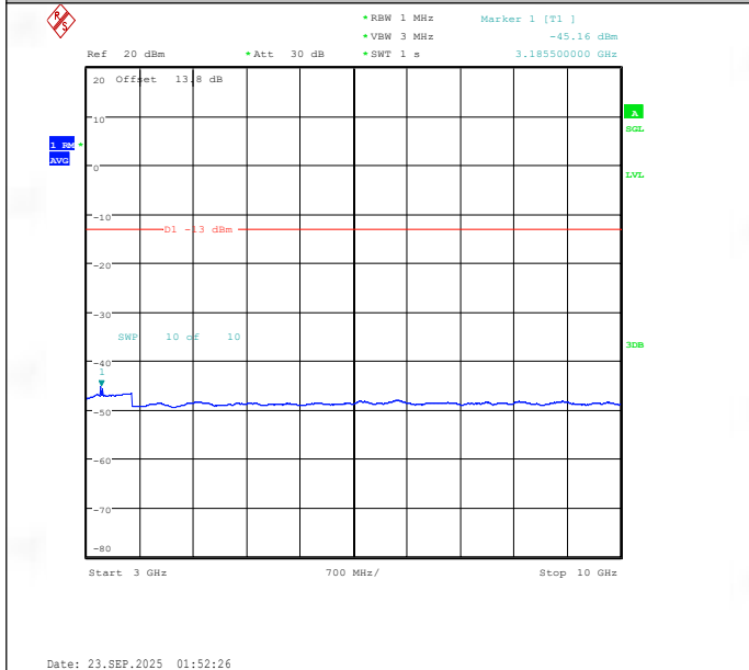
Band26(824-849)-10MHz-16QAM-26990-1RB#49-3000~10000-PASS
