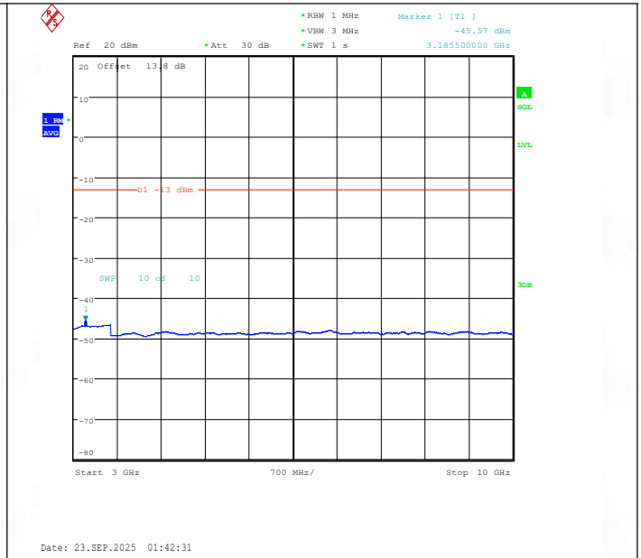
Band26(824-849)-10MHz-QPSK-26915-1RB#49-3000~10000-PASS
