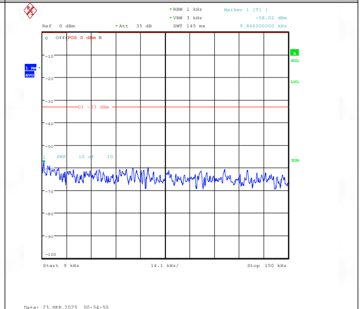
Band26(824-849)-5MHz-16QAM-26915-25RB#0-0.009~0.15-PASS
