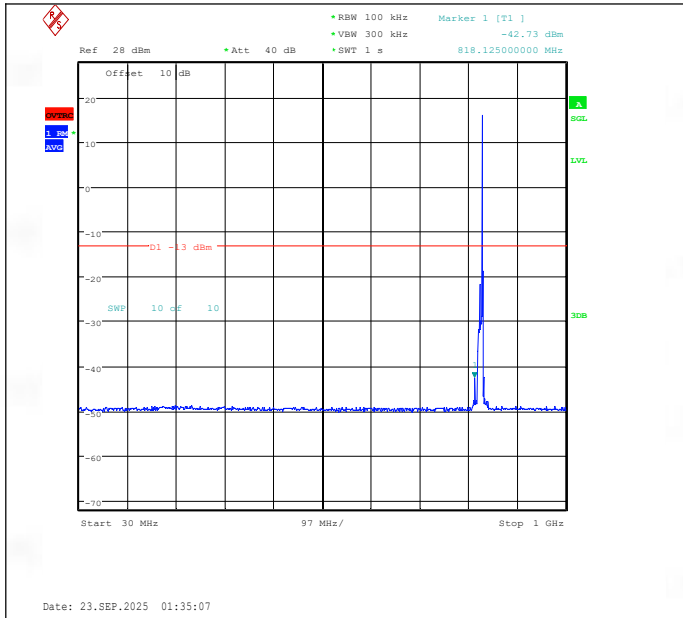
Band26(824-849)-10MHz-16QAM-26840-1RB#49-30~1000-PASS
