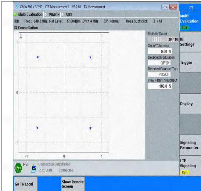
Band26(824-849)-1.4MHz-QPSK-27033-6RB#0-PASS
