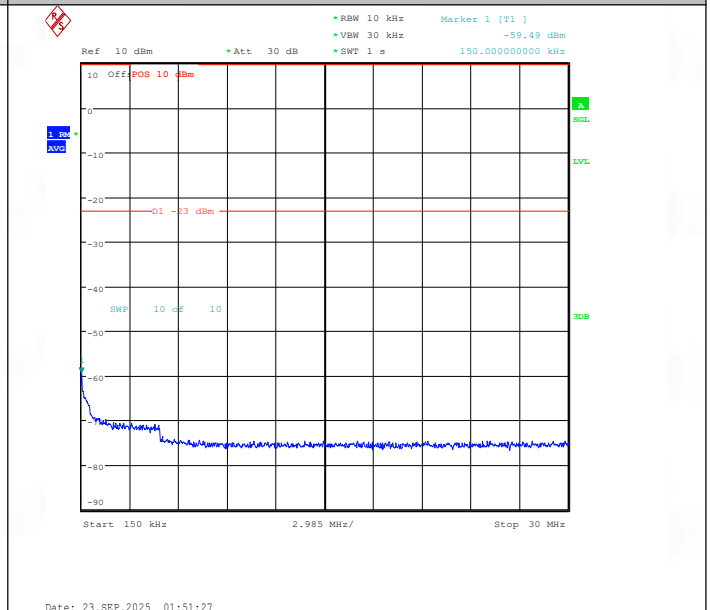
Band26(824-849)-10MHz-16QAM-26990-1RB#49-0.15~30-PASS
