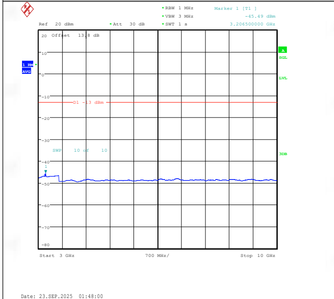
Band26(824-849)-10MHz-QPSK-26990-1RB#0-3000~10000-PASS
