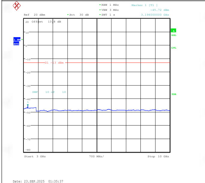
Band26(824-849)-10MHz-16QAM-26840-1RB#49-3000~10000-PASS
