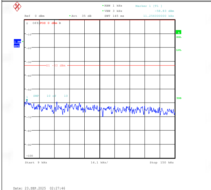
Band26(824-849)-15MHz-QPSK-26865-75RB#0-0.009~0.15-PASS
