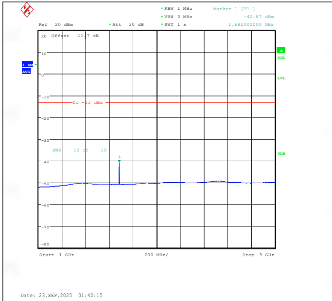
Band26(824-849)-10MHz-QPSK-26915-1RB#49-1000~3000-PASS
