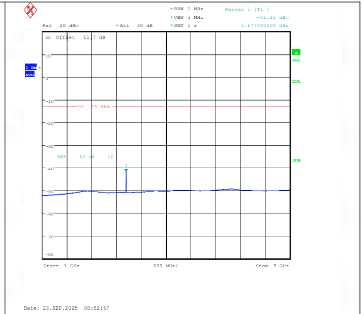
Band26(824-849)-5MHz-16QAM-26915-1RB#24-1000~3000-PASS
