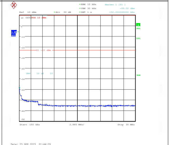
Band26(824-849)-10MHz-QPSK-26915-50RB#0-0.15~30-PASS
