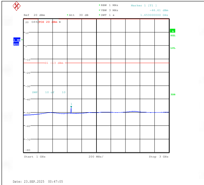
Band26(824-849)-5MHz-16QAM-26815-25RB#0-1000~3000-PASS
