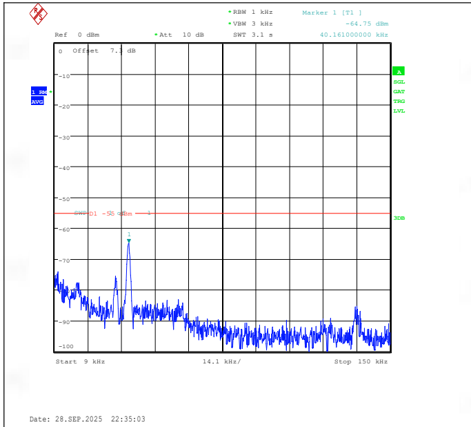
Band38-10MHz-16QAM-38000-1RB#49-0.009~0.15-PASS
