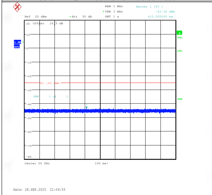
Band38-5MHz-QPSK-38225-25RB#0-20000~27000-PASS
