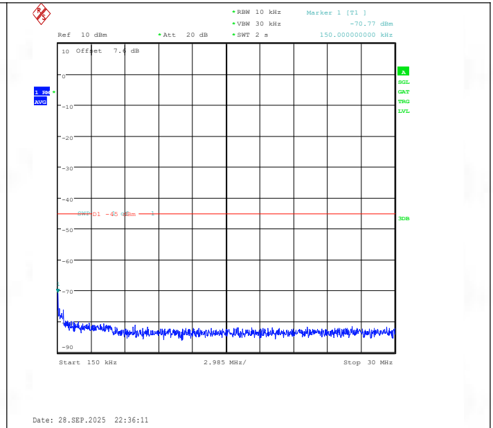
Band38-10MHz-16QAM-38000-1RB#49-0.15~30-PASS
