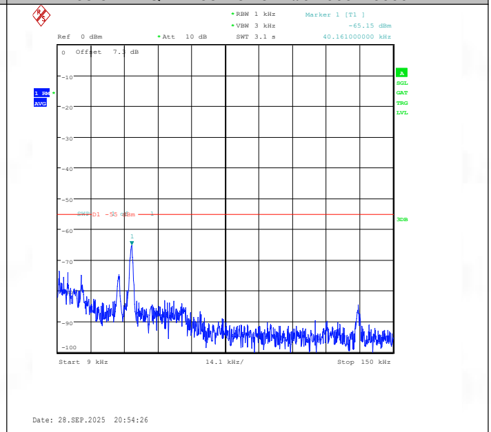
Band38-5MHz-16QAM-38225-1RB#0-0.009~0.15-PASS
