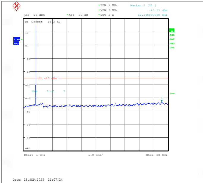
Band38-5MHz-16QAM-38225-25RB#0-1000~20000-PASS
