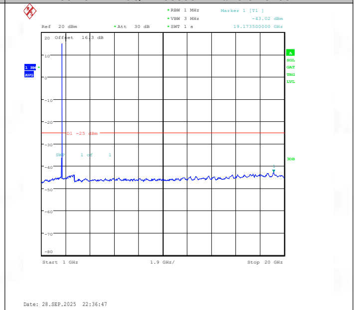
Band38-10MHz-16QAM-38000-1RB#49-1000~20000-PASS
