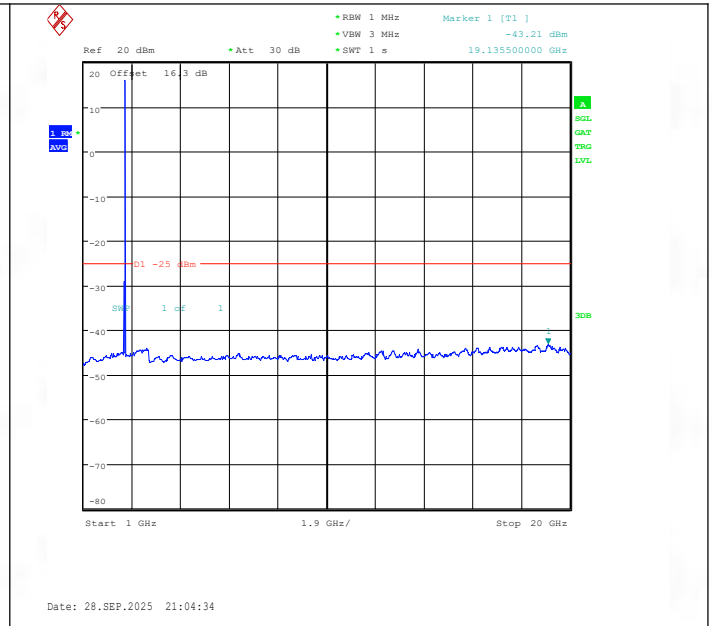
Band38-5MHz-QPSK-38225-25RB#0-1000~20000-PASS
