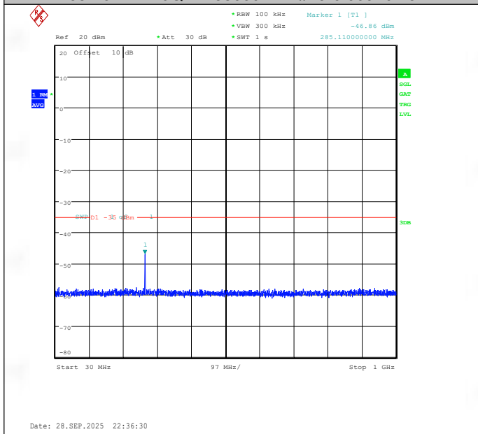
Band38-10MHz-16QAM-38000-1RB#49-30~1000-PASS
