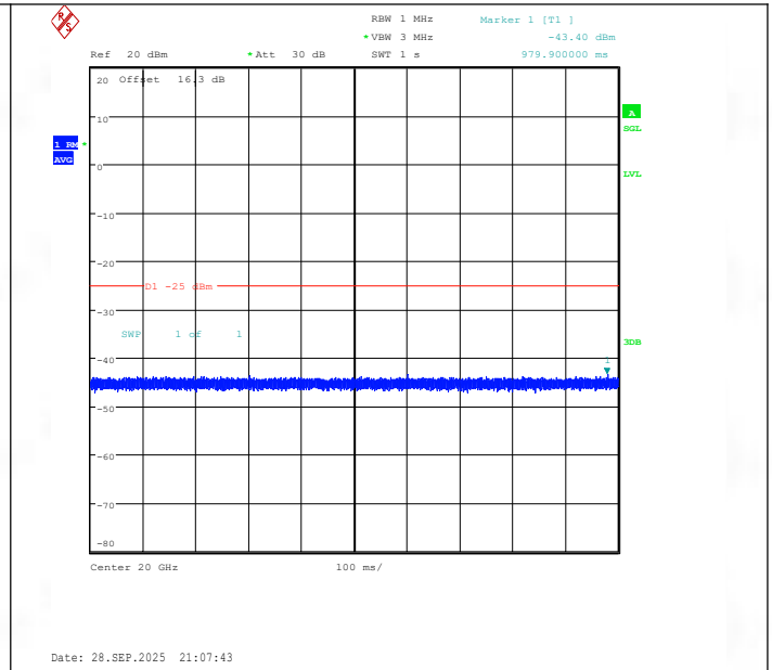
Band38-5MHz-16QAM-38225-25RB#0-20000~27000-PASS
