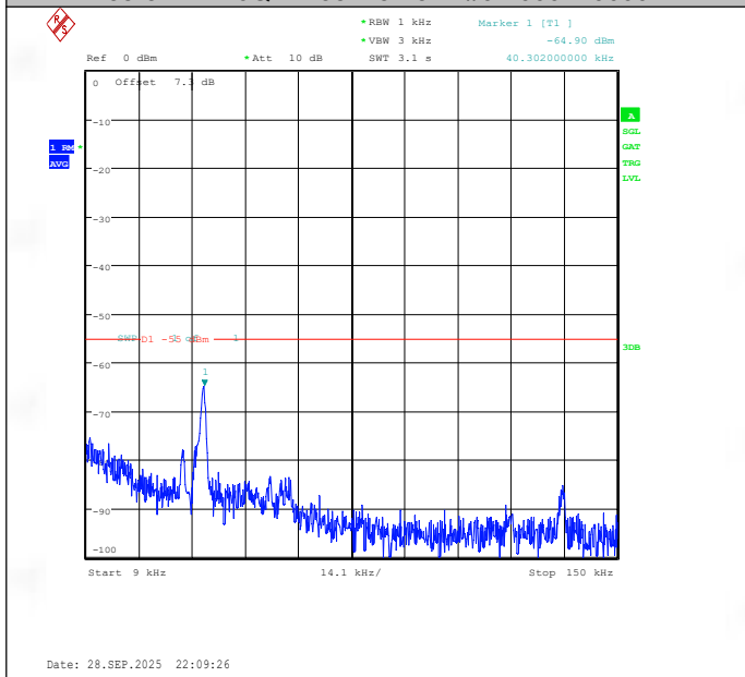
Band38-10MHz-QPSK-37800-1RB#0-0.009~0.15-PASS
