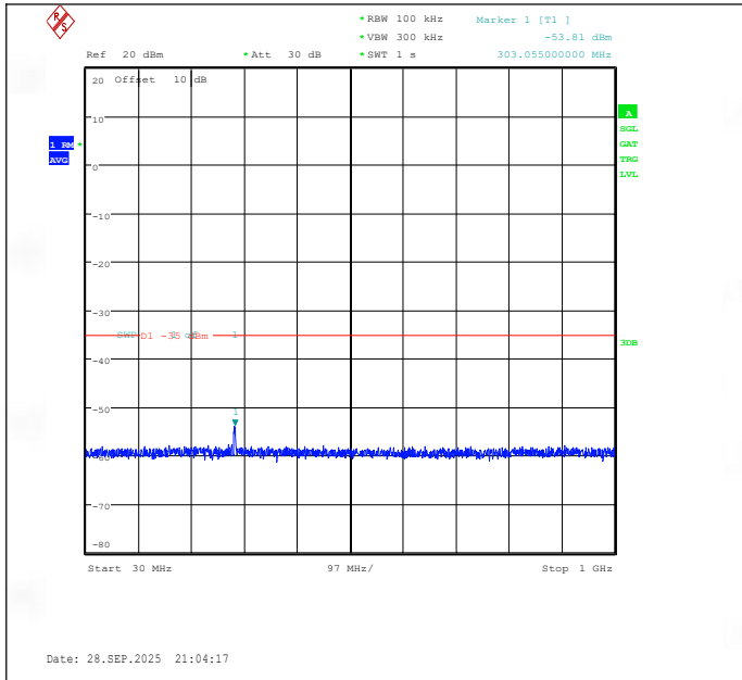
Band38-5MHz-QPSK-38225-25RB#0-30~1000-PASS
