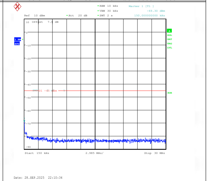
Band38-10MHz-QPSK-37800-1RB#0-0.15~30-PASS
