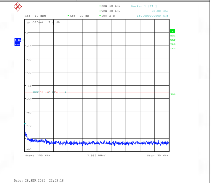
Band38-10MHz-16QAM-38200-1RB#49-0.15~30-PASS
