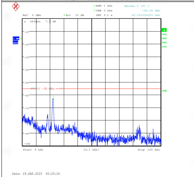
Band38-15MHz-16QAM-38000-1RB#74-0.009~0.15-PASS
