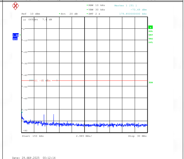
Band38-15MHz-QPSK-37825-75RB#0-0.15~30-PASS
