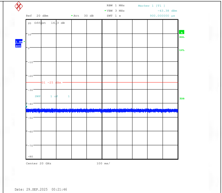
Band38-15MHz-16QAM-38000-1RB#0-20000~27000-PASS
