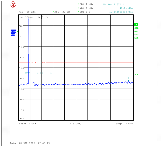
Band38-10MHz-16QAM-38200-1RB#0-1000~20000-PASS
