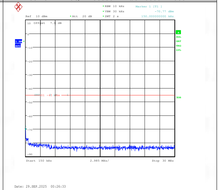
Band38-15MHz-16QAM-38000-1RB#74-0.15~30-PASS
