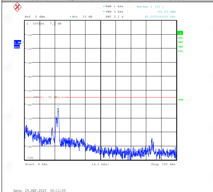
Band38-15MHz-QPSK-37825-75RB#0-0.009~0.15-PASS
