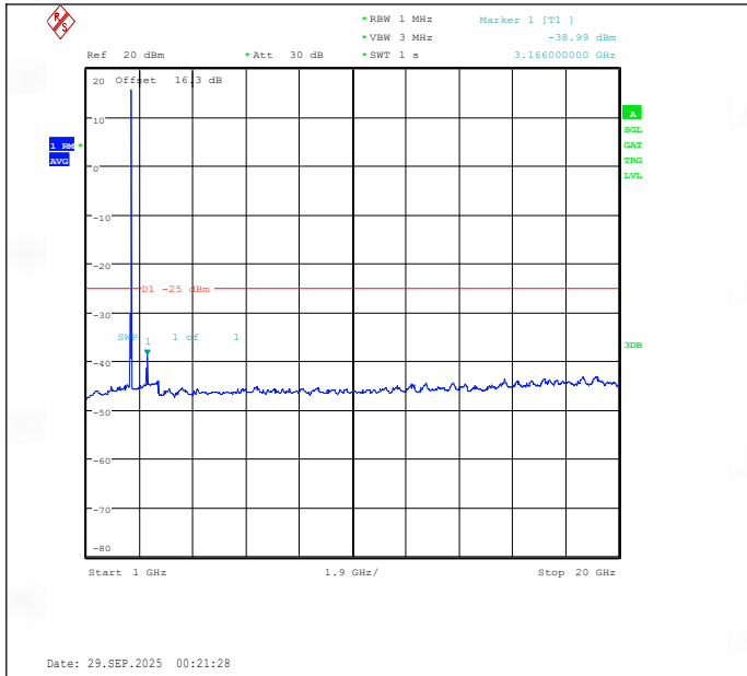
Band38-15MHz-16QAM-38000-1RB#0-1000~20000-PASS
