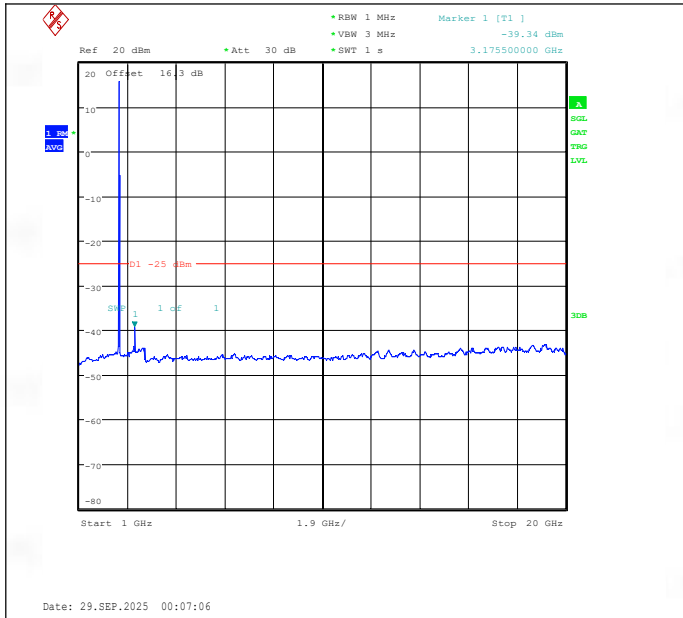
Band38-15MHz-QPSK-37825-1RB#74-1000~20000-PASS
