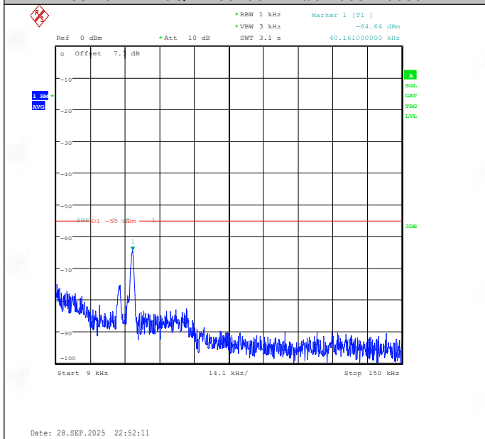
Band38-10MHz-16QAM-38200-1RB#49-0.009~0.15-PASS
