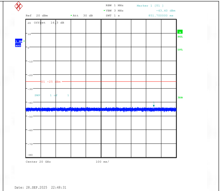
Band38-10MHz-16QAM-38200-1RB#0-20000~27000-PASS
