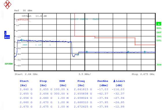
Band41(2535-2655)-15MHz-16QAM-41165-1RB#0-PASS
