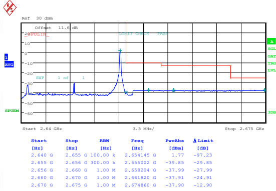
Band41(2535-2655)-15MHz-QPSK-41165-75RB#0-PASS
