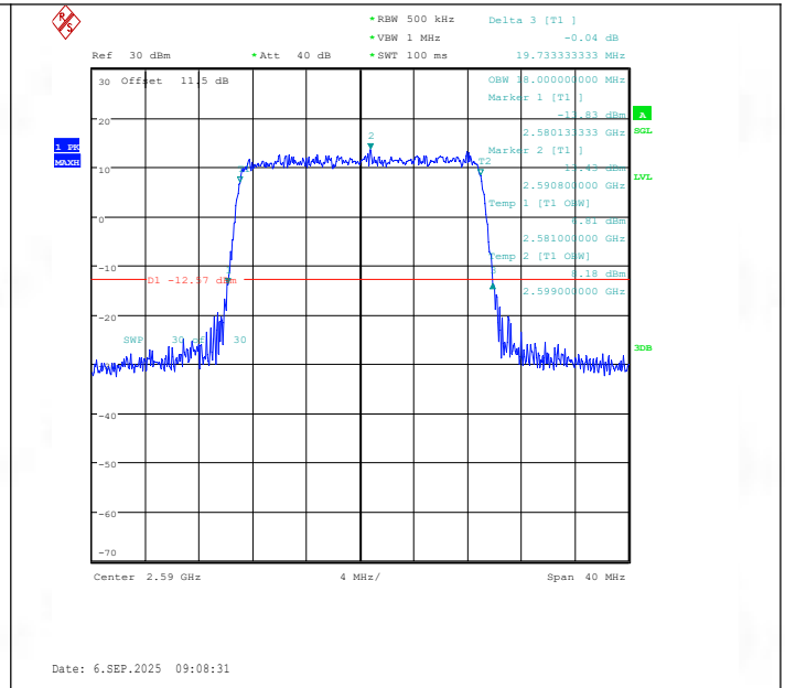
Band41(2535-2655)-20MHz-16QAM-40590-100RB#0-PASS
