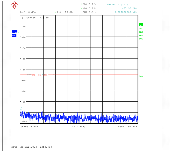
Band41(2535-2655)-20MHz-QPSK-40590-1RB#99-0.009~0.15-PASS
