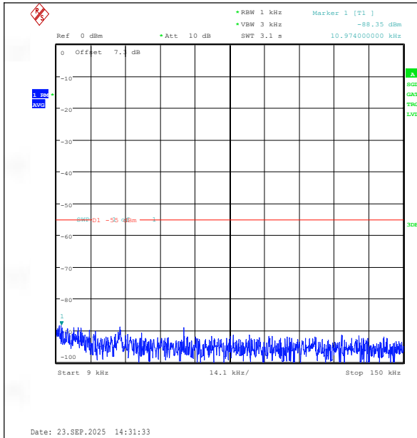
Band41(2535-2655)-10MHz-QPSK-40090-50RB#0-0.009~0.15-PASS
