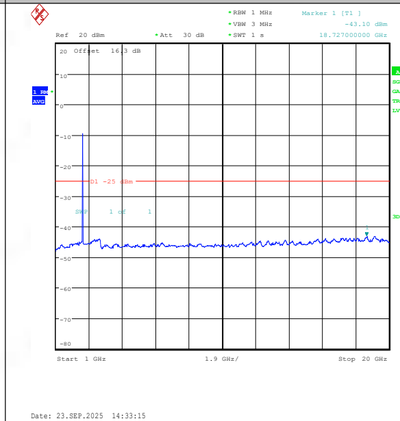
Band41(2535-2655)-10MHz-QPSK-40090-50RB#0-1000~20000-PASS
