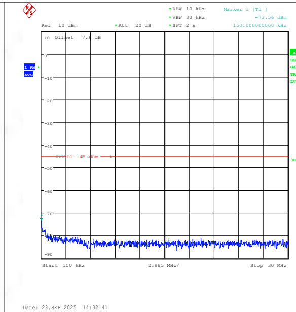
Band41(2535-2655)-10MHz-QPSK-40090-50RB#0-0.15~30-PASS
