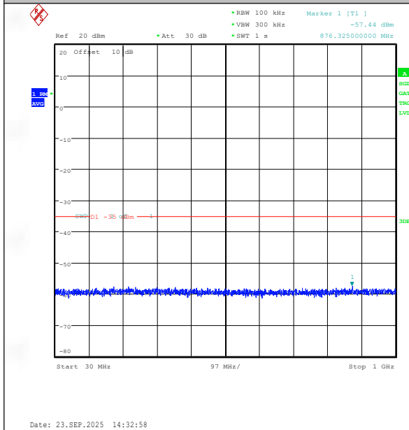
Band41(2535-2655)-10MHz-QPSK-40090-50RB#0-30~1000-PASS
