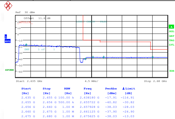
Band41(2535-2655)-20MHz-16QAM-41140-1RB#0-PASS
