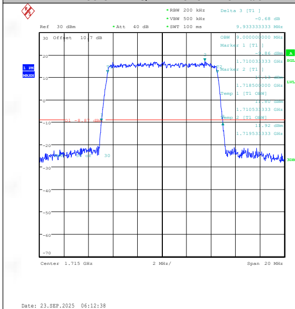
Band66-10MHz-QPSK-132022-50RB#0-PASS
