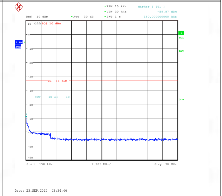
Band66-1.4MHz-QPSK-132665-6RB#0-0.15~30-PASS
