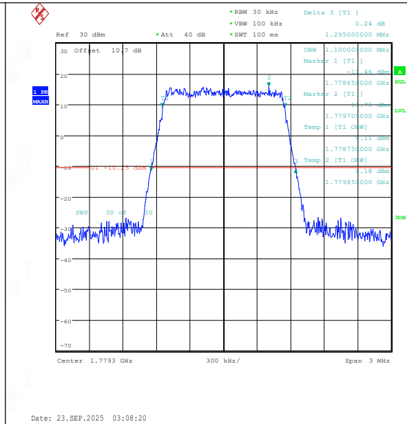
Band66-1.4MHz-16QAM-132665-6RB#0-PASS
