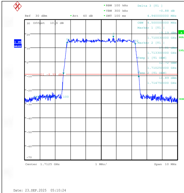
Band66-5MHz-QPSK-131997-25RB#0-PASS
