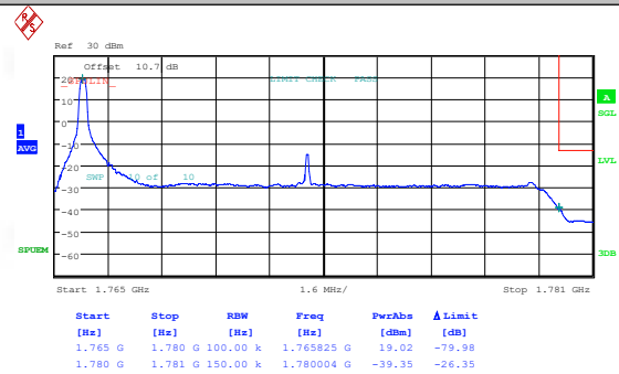
Band66-15MHz-QPSK-132597-1RB#74-PASS
