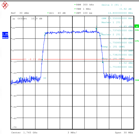
Band66-15MHz-QPSK-132047-75RB#0-PASS
