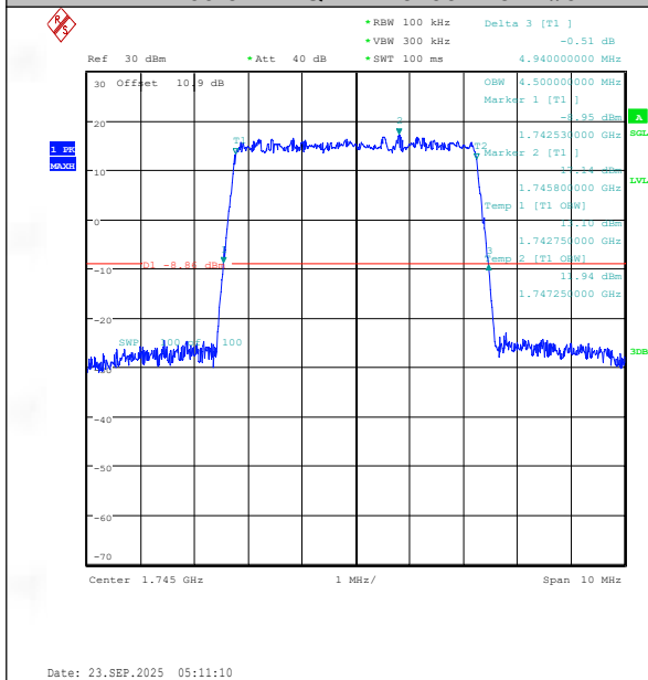
Band66-5MHz-QPSK-132322-25RB#0-PASS
