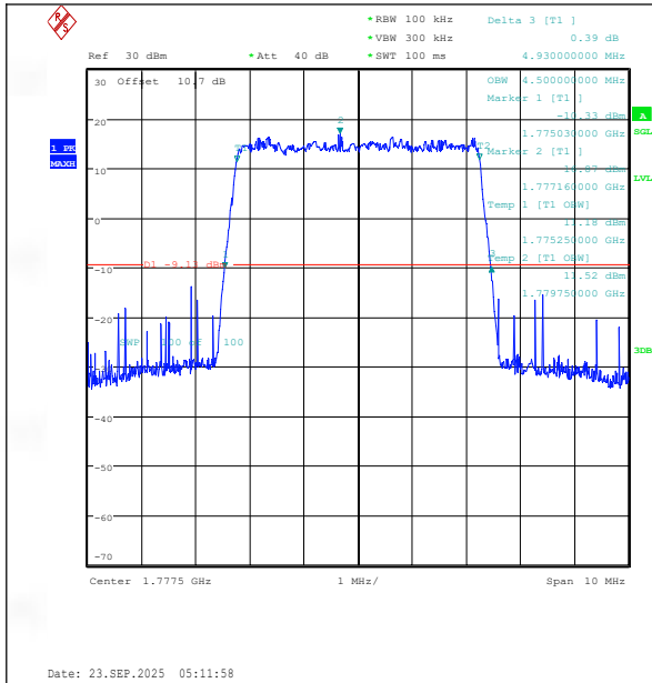
Band66-5MHz-QPSK-132647-25RB#0-PASS
