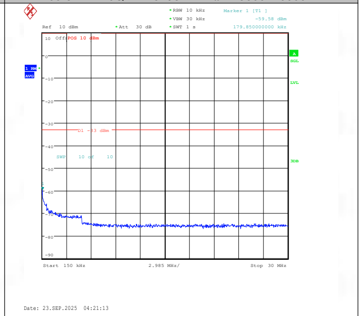
Band66-3MHz-16QAM-131987-15RB#0-0.15~30-PASS
