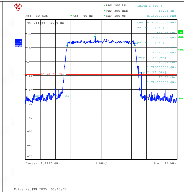
Band66-5MHz-16QAM-131997-25RB#0-PASS
