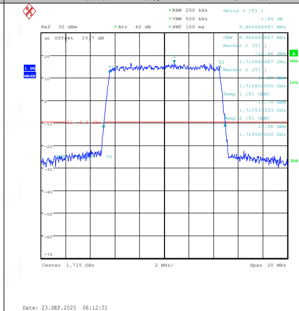
Band66-10MHz-16QAM-132022-50RB#0-PASS
