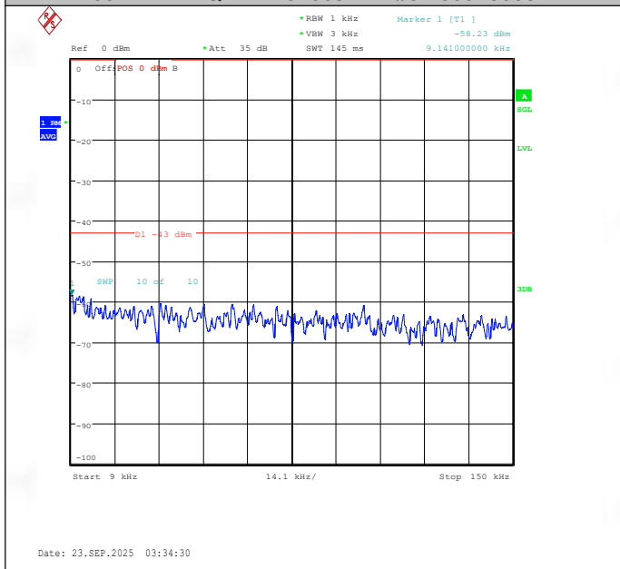
Band66-1.4MHz-QPSK-132665-6RB#0-0.009~0.15-PASS
