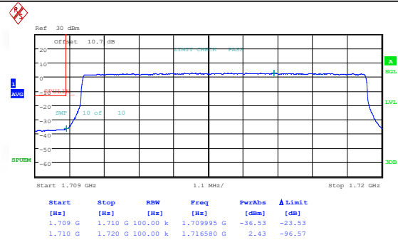
Band66-10MHz-16QAM-132022-1RB#0-PASS
