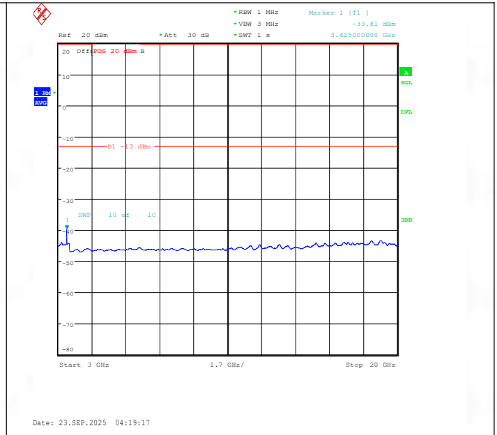
Band66-3MHz-16QAM-131987-1RB#14-3000~20000-PASS
