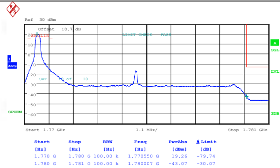
Band66-10MHz-QPSK-132622-1RB#49-PASS
