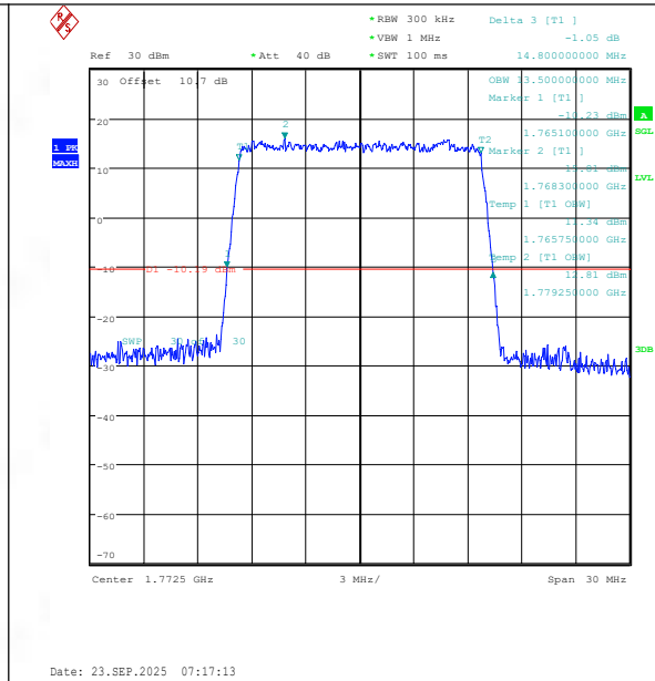
Band66-15MHz-16QAM-132597-75RB#0-PASS
