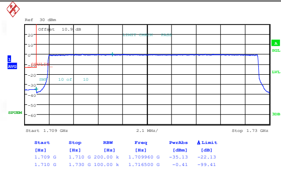
Band66-20MHz-16QAM-132072-1RB#0-PASS
