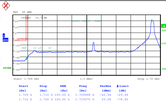
Band66-10MHz-QPSK-132022-50RB#0-PASS
