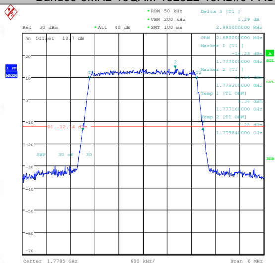
Band66-3MHz-16QAM-132322-15RB#0-PASS
