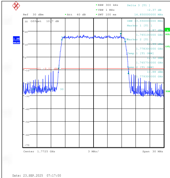
Band66-15MHz-QPSK-132597-75RB#0-PASS
