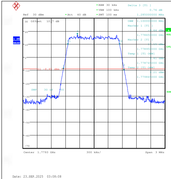
Band66-1.4MHz-QPSK-132665-6RB#0-PASS
