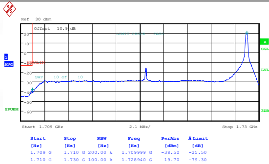
Band66-20MHz-QPSK-132072-100RB#0-PASS
