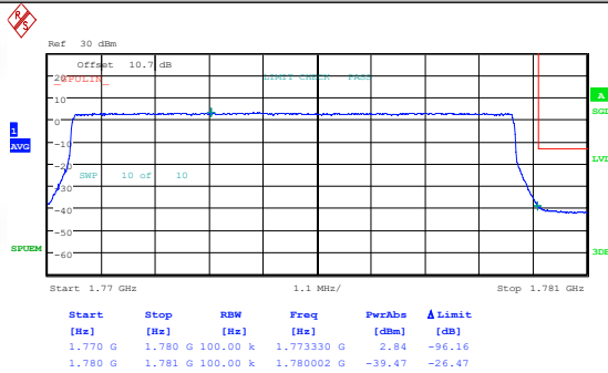
Band66-10MHz-QPSK-132622-1RB#0-PASS
