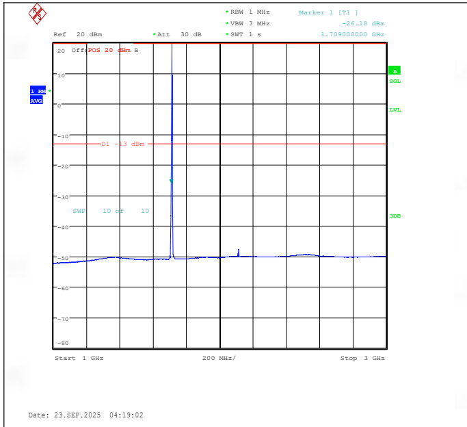
Band66-3MHz-16QAM-131987-1RB#14-1000~3000-PASS
