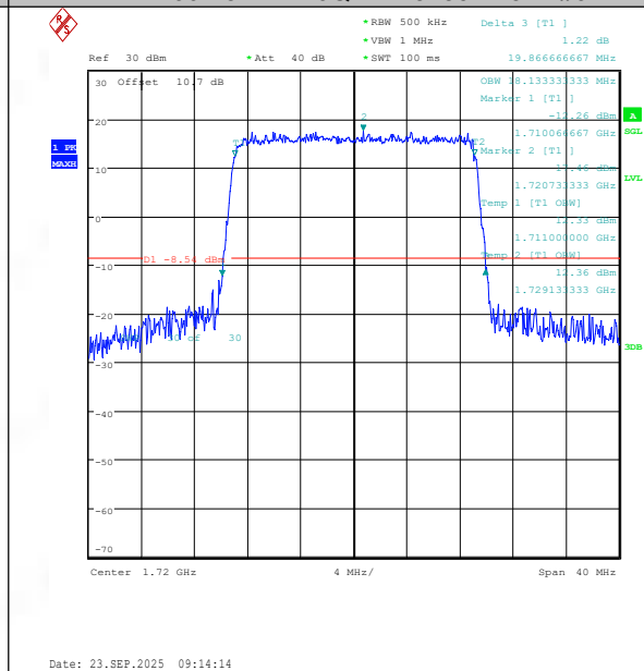
Band66-20MHz-16QAM-132072-100RB#0-PASS
