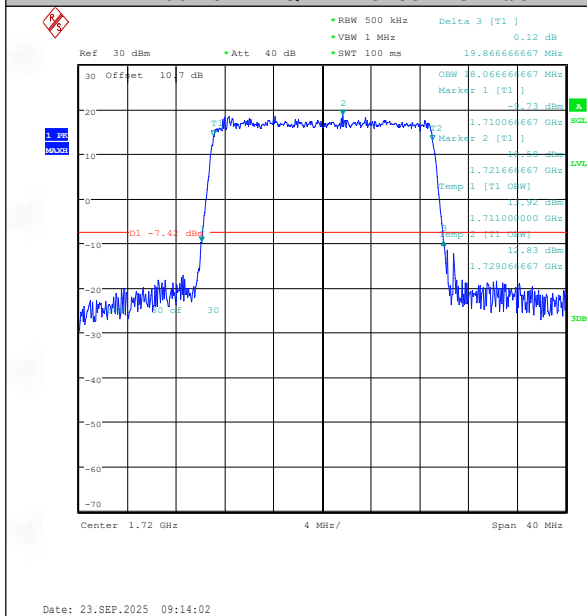
Band66-20MHz-QPSK-132072-100RB#0-PASS
