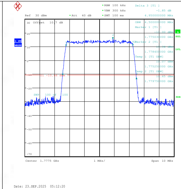
Band66-5MHz-16QAM-132647-25RB#0-PASS
