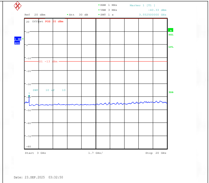
Band66-1.4MHz-QPSK-132665-1RB#5-3000~20000-PASS
