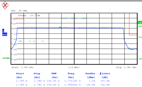
Band66-15MHz-QPSK-132597-1RB#0-PASS
