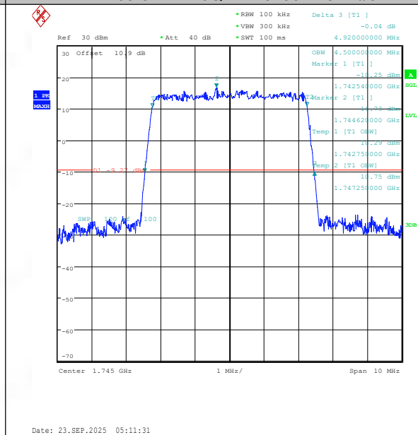
Band66-5MHz-16QAM-132322-25RB#0-PASS
