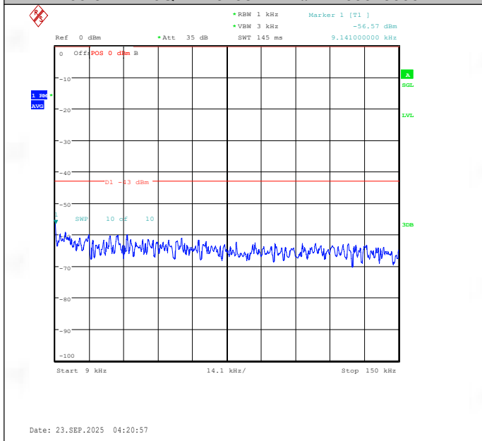
Band66-3MHz-16QAM-131987-15RB#0-0.009~0.15-PASS
