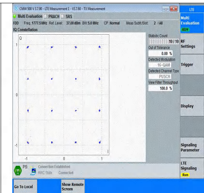
Band66-5MHz-16QAM-132647-25RB#0-PASS
