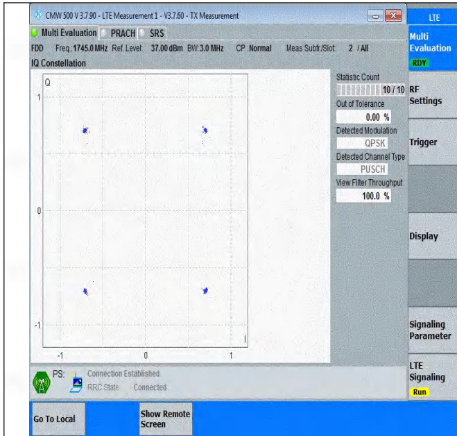
Band66-3MHz-QPSK-132322-15RB#0-PASS
