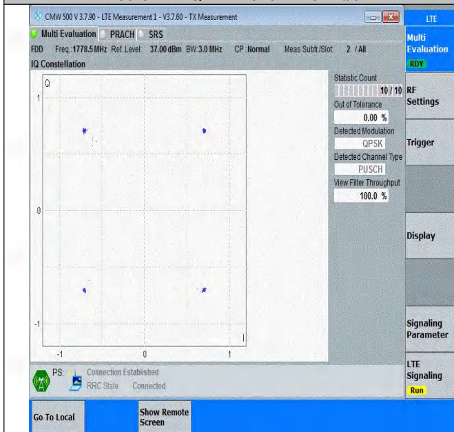
Band66-3MHz-QPSK-132657-15RB#0-PASS
