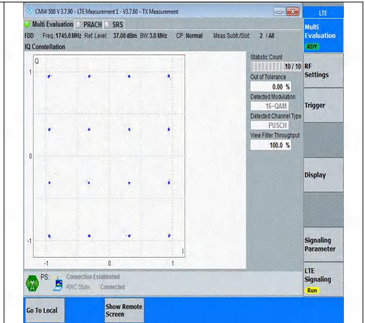
Band66-3MHz-16QAM-132322-15RB#0-PASS
