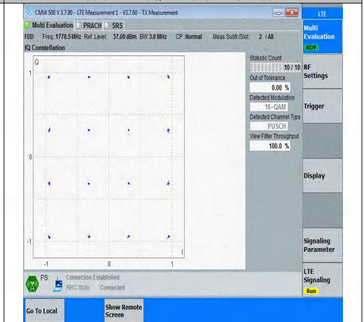
Band66-3MHz-16QAM-132657-15RB#0-PASS
