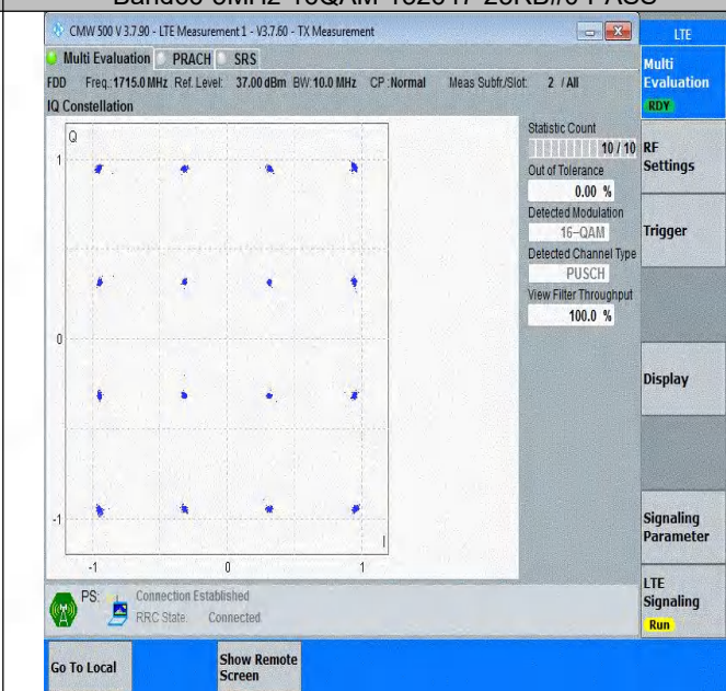
Band66-10MHz-16QAM-132022-50RB#0-PASS
