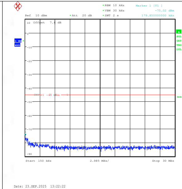
Band41(2535-2655)-15MHz-16QAM-41165-1RB#74-0.15~30-PASS
