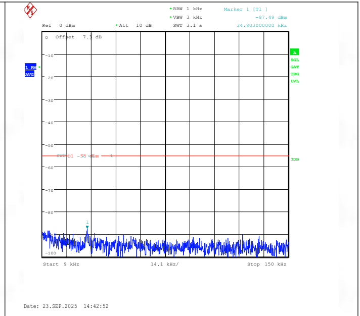
Band41(2535-2655)-10MHz-QPSK-40590-1RB#49-0.009~0.15-PASS
