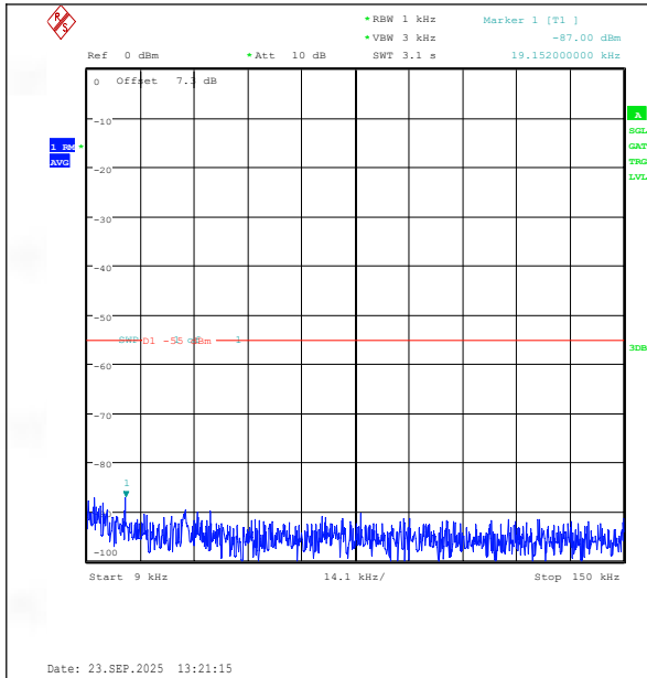
Band41(2535-2655)-15MHz-16QAM-41165-1RB#74-0.009~0.15-PASS
