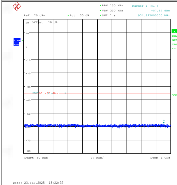
Band41(2535-2655)-15MHz-16QAM-41165-1RB#74-30~1000-PASS
