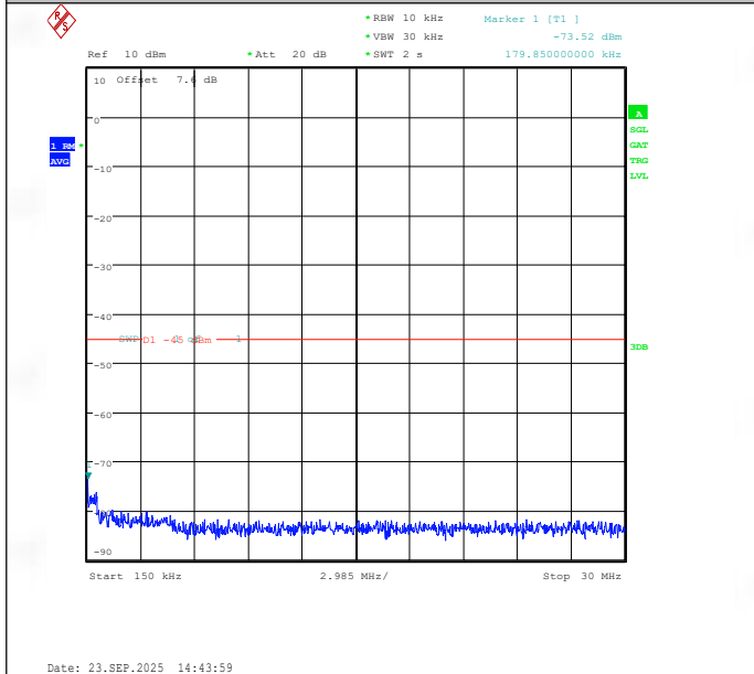
Band41(2535-2655)-10MHz-QPSK-40590-1RB#49-0.15~30-PASS
