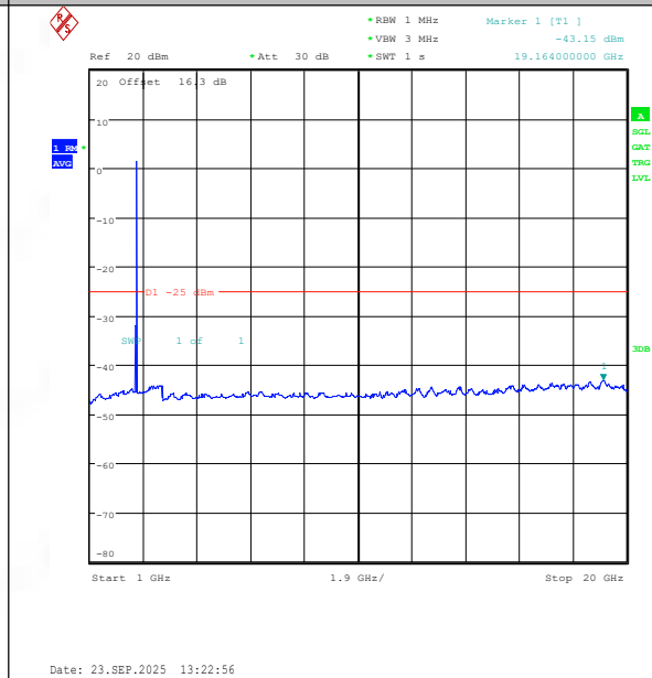
Band41(2535-2655)-15MHz-16QAM-41165-1RB#74-1000~20000-PASS
