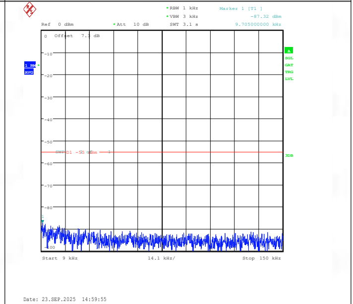
Band41(2535-2655)-10MHz-QPSK-41190-1RB#49-0.009~0.15-PASS
