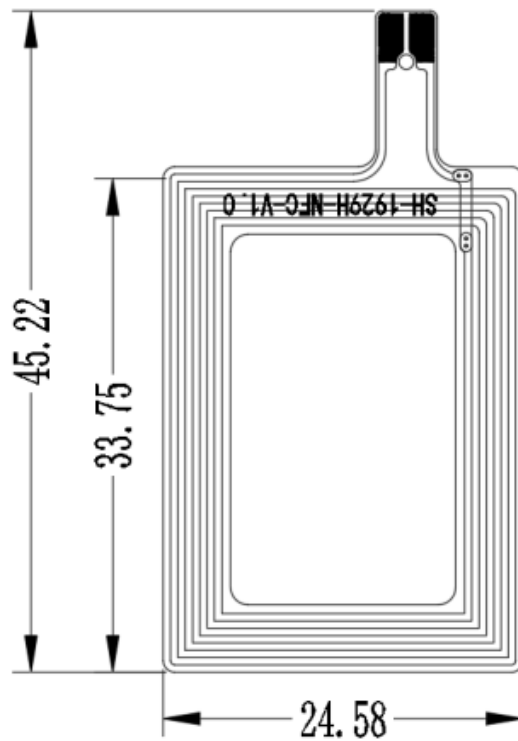
NFC:45.22*24.58mm PIFA
