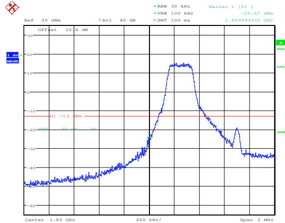
Band25-1.4MHz-16QAM-26047-1RB#5
