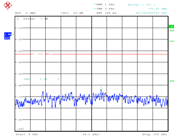
Band25-1.4MHz-QPSK-26683-1RB#0-Range1:0.009~0.15MHz
