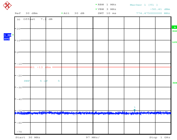
Band25-1.4MHz-QPSK-26683-1RB#0-Range3:30~1000MHz
