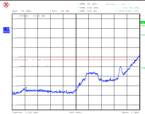
Band25-1.4MHz-16QAM-26047-1RB#5
