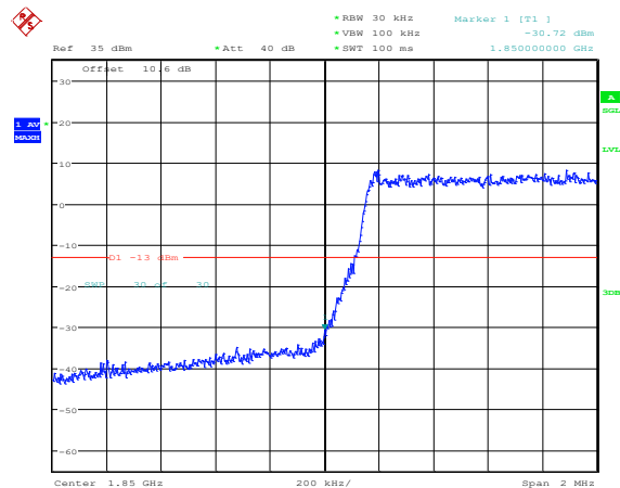
Band25-1.4MHz-16QAM-26047-6RB#0
