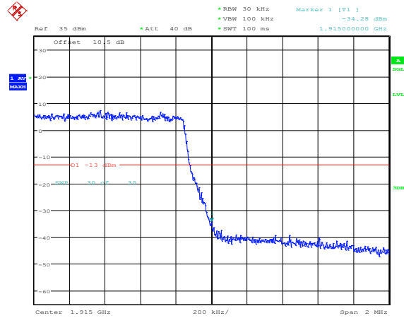
Band25-1.4MHz-16QAM-26683-6RB#0
