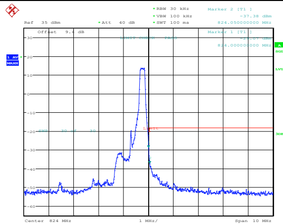
Band26-1.4MHz-16QAM-26783-1RB#5
