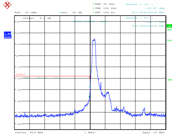
Band26-1.4MHz-16QAM-26697-1RB#5
