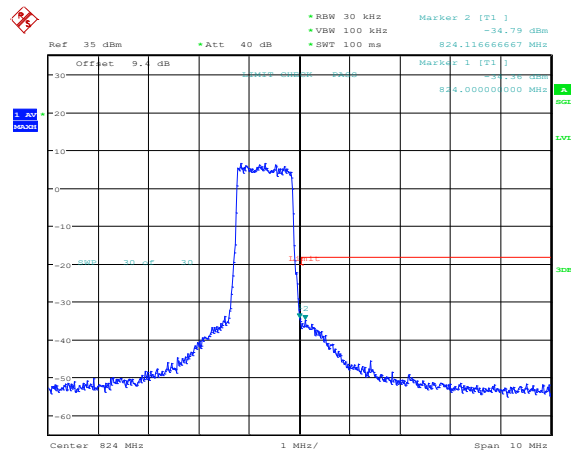
Band26-1.4MHz-16QAM-26783-6RB#0
