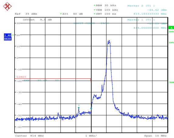
Band26-1.4MHz-16QAM-26697-1RB#5
