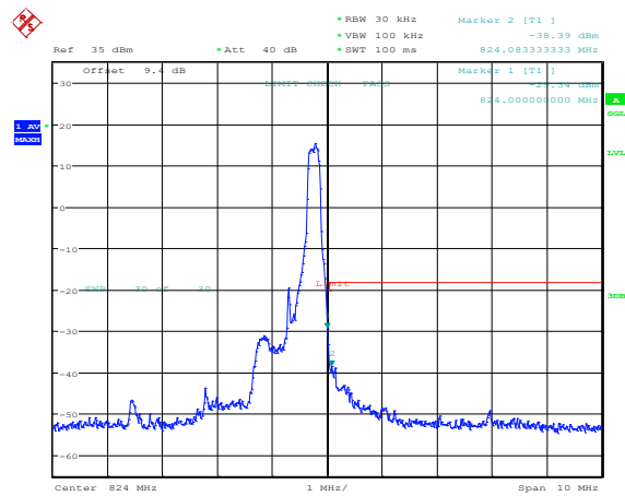
Band26-1.4MHz-QPSK-26783-1RB#5
