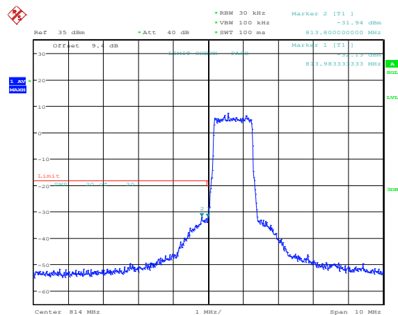
Band26-1.4MHz-16QAM-26697-6RB#0
