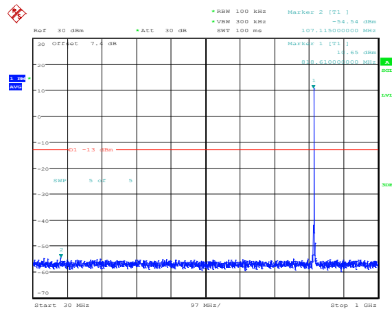
Band26-1.4MHz-QPSK-26740-1RB#0-Range3:30~1000MHz
