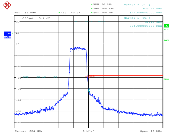
Band26-1.4MHz-QPSK-26783-6RB#0
