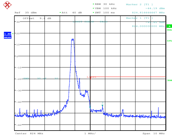
Band26-1.4MHz-QPSK-26783-1RB#5
