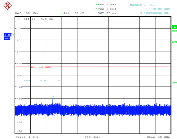
Band26-1.4MHz-QPSK-26740-1RB#0-Range4:1000~10000MHz
