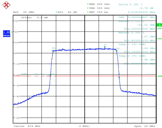
Band26-10MHz-QPSK-26740-50RB#0
