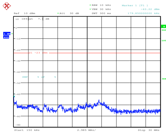
Band4-10MHz-16QAM-20175-1RB#0-Range2:0.15~30MHz
