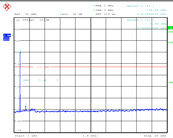
Band4-15MHz-16QAM-20175-1RB#0-Range4:1000~20000MHz
