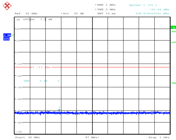
Band4-10MHz-16QAM-20350-1RB#0-Range3:30~1000MHz
