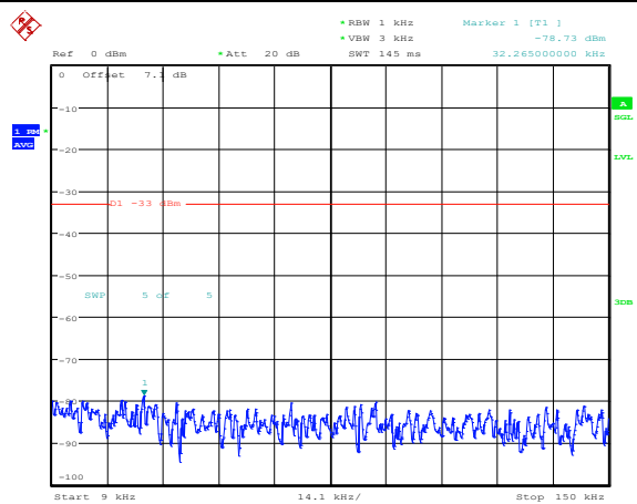
Band4-15MHz-QPSK-20325-1RB#0-Range1:0.009~0.15MHz
