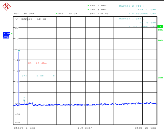
Band4-15MHz-QPSK-20175-1RB#0-Range4:1000~20000MHz
