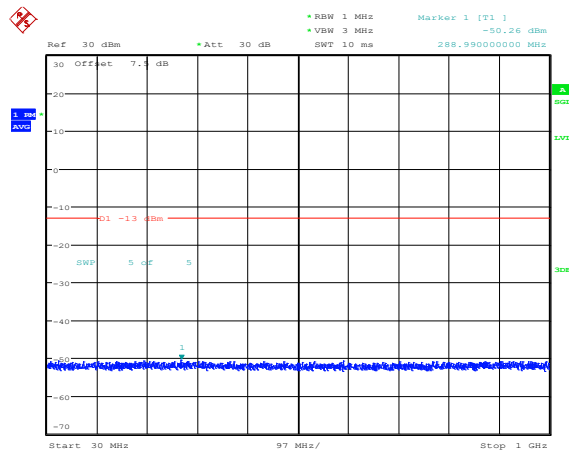
Band4-15MHz-QPSK-20325-1RB#0-Range3:30~1000MHz
