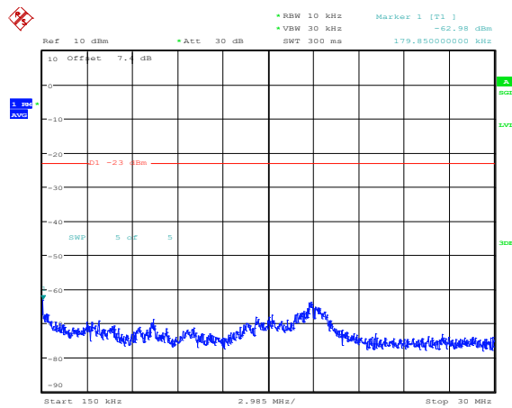
Band4-15MHz-16QAM-20025-1RB#0-Range2:0.15~30MHz
