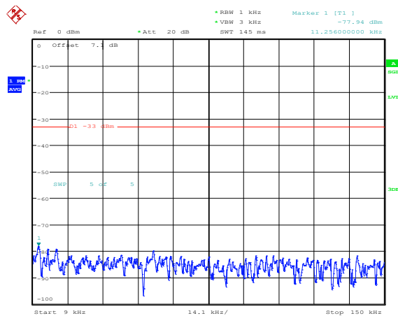
Band4-5MHz-16QAM-20375-1RB#0-Range1:0.009~0.15MHz
