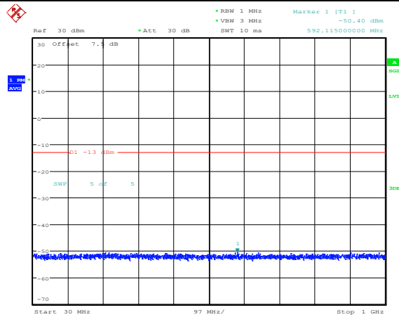
Band4-1.4MHz-QPSK-20393-1RB#0-Range3:30~1000MHz
