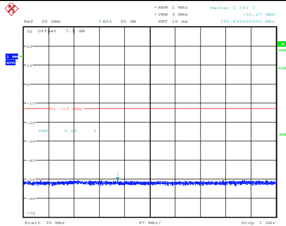
Band4-15MHz-16QAM-20025-1RB#0-Range3:30~1000MHz
