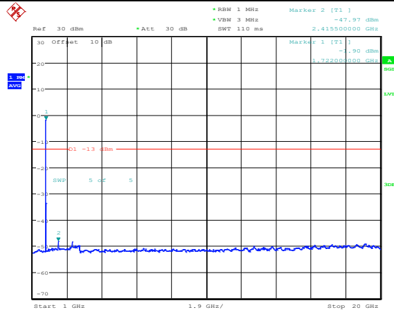
Band4-10MHz-16QAM-20175-1RB#0-Range4:1000~20000MHz
