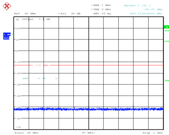
Band4-3MHz-16QAM-20385-1RB#0-Range3:30~1000MHz
