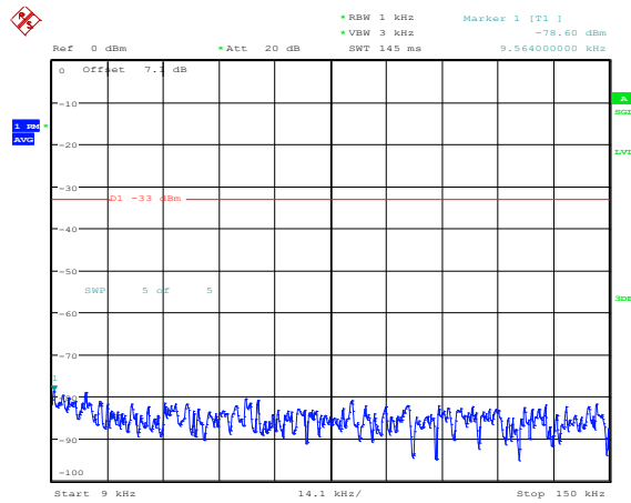
Band4-5MHz-16QAM-20175-1RB#0-Range1:0.009~0.15MHz
