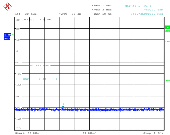
Band4-15MHz-16QAM-20325-1RB#0-Range3:30~1000MHz
