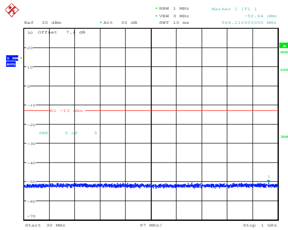
Band66-1.4MHz-QPSK-132665-1RB#0-Range3:30~1000MHz
