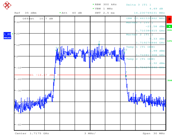
Band66-15MHz-QPSK-132047-75RB#0
