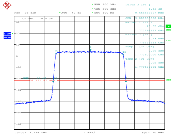
Band66-10MHz-16QAM-132622-50RB#0
