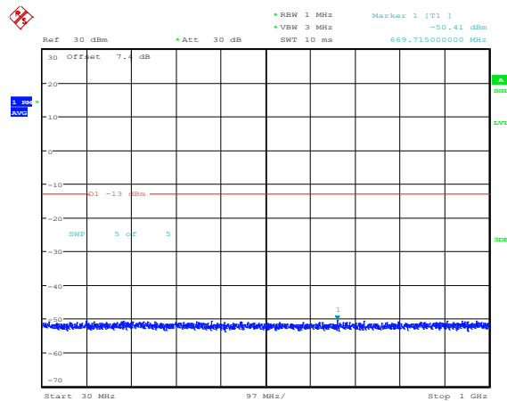
Band66-1.4MHz-16QAM-131979-1RB#0-Range3:30~1000MHz
