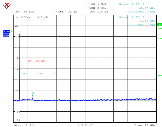
Band66-1.4MHz-QPSK-132665-1RB#0-Range4:1000~20000MHz
