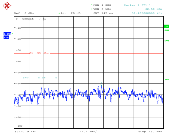
Band66-1.4MHz-QPSK-132322-1RB#0-Range1:0.009~0.15MHz
