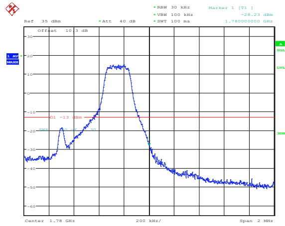
Band66-1.4MHz-16QAM-132665-1RB#5
