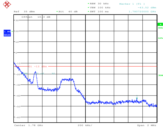
Band66-1.4MHz-16QAM-132665-1RB#5
