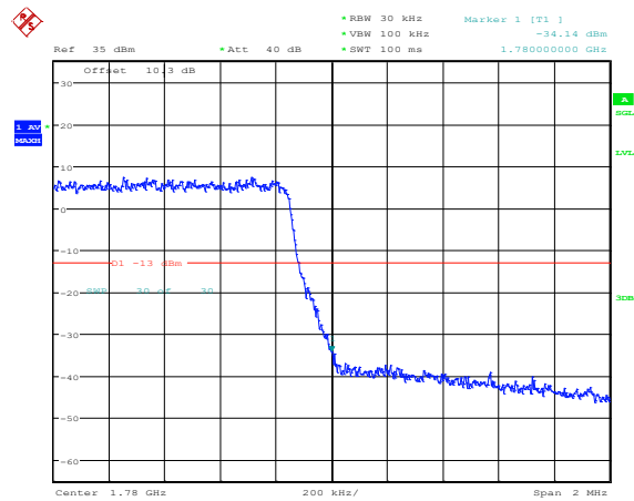
Band66-1.4MHz-16QAM-132665-6RB#0
