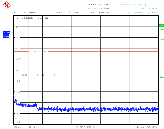
Band66-1.4MHz-QPSK-132322-1RB#0-Range2:0.15~30MHz
