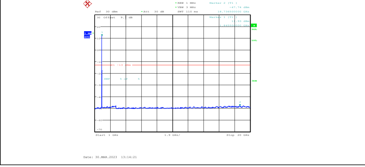
Band2-15MHz-16QAM-18675-1RB#0-Range4:1000~20000MHz
