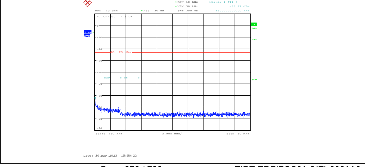
Band5-1.4MHz-16QAM-20407-1RB#0-Range2:0.15~30MHz
