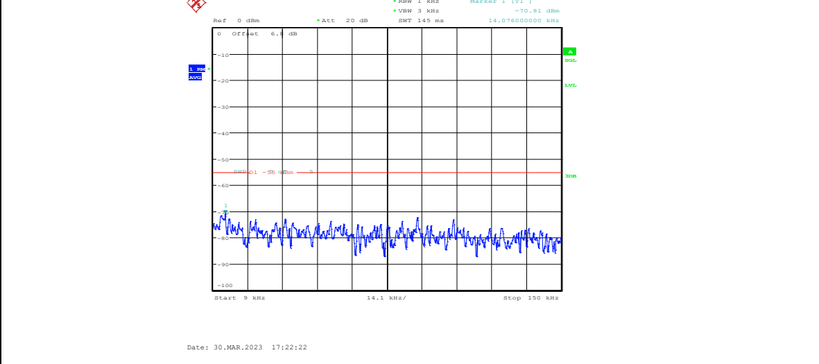
Band7-10MHz-16QAM-21400-1RB#0-Range1:0.009~0.15MHz
