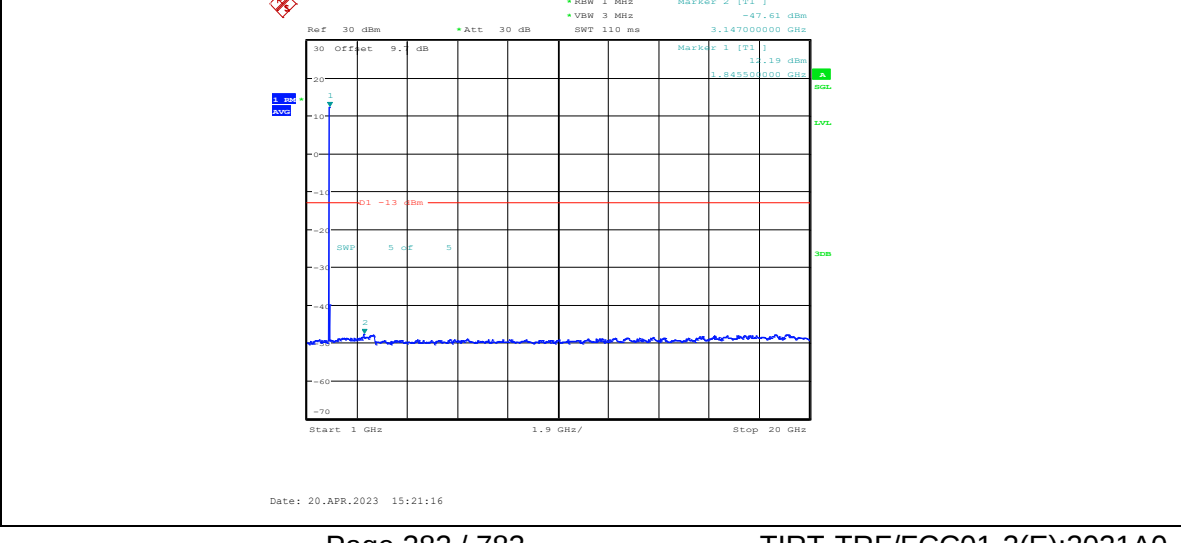
Band25-3MHz-QPSK-26055-1RB#0-Range4:1000~20000MHz
