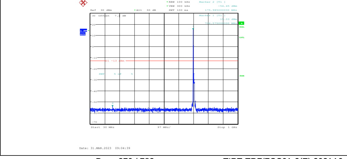
Band17-10MHz-QPSK-23800-1RB#0-Range3:30~1000MHz
