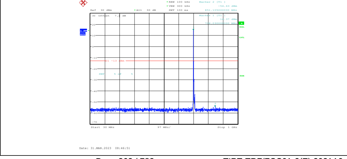
Band17-5MHz-QPSK-23790-1RB#0-Range3:30~1000MHz
