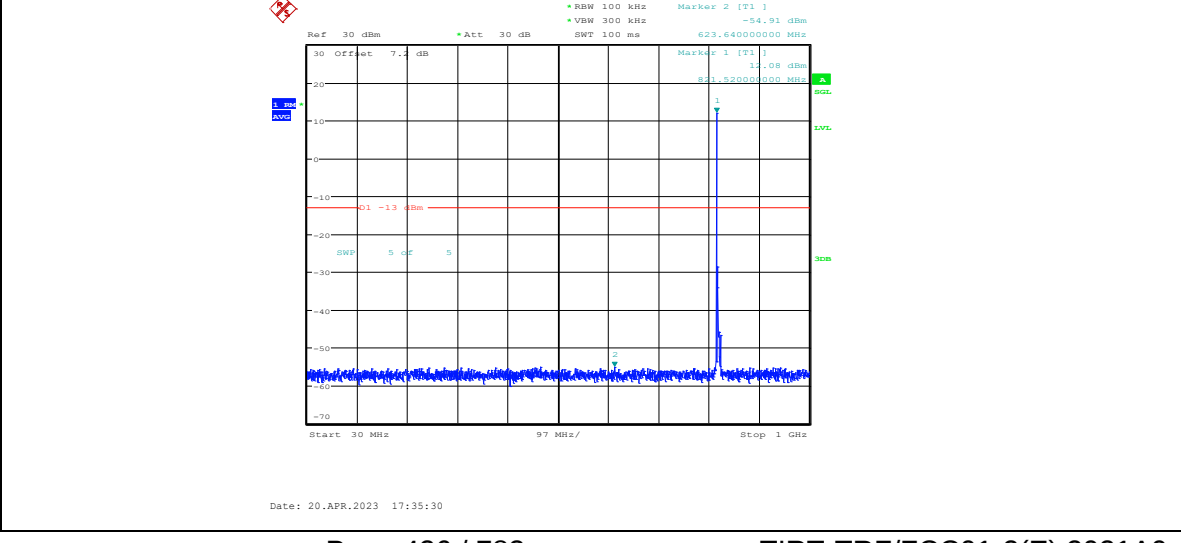
Band26-3MHz-QPSK-26775-1RB#0-Range3:30~1000MHz
