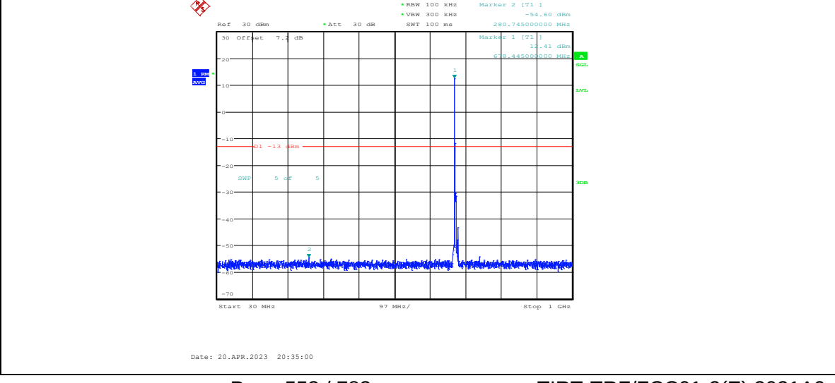
Band71-5MHz-QPSK-133297-1RB#0-Range3:30~1000MHz
