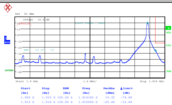
Band25_15MHz_16QAM_26615_1RB#0
