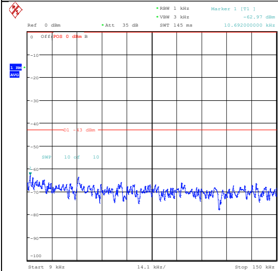
Band25_5MHz_16QAM_26365_1RB#0_1000~3000_1000~3000
