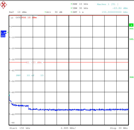
Band25_5MHz_16QAM_26365_1RB#0_3000~20000_3000~20000
