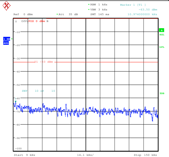
Band26_10MHz_QPSK_26915_1RB#0_1000~3000_0_1000~3000
